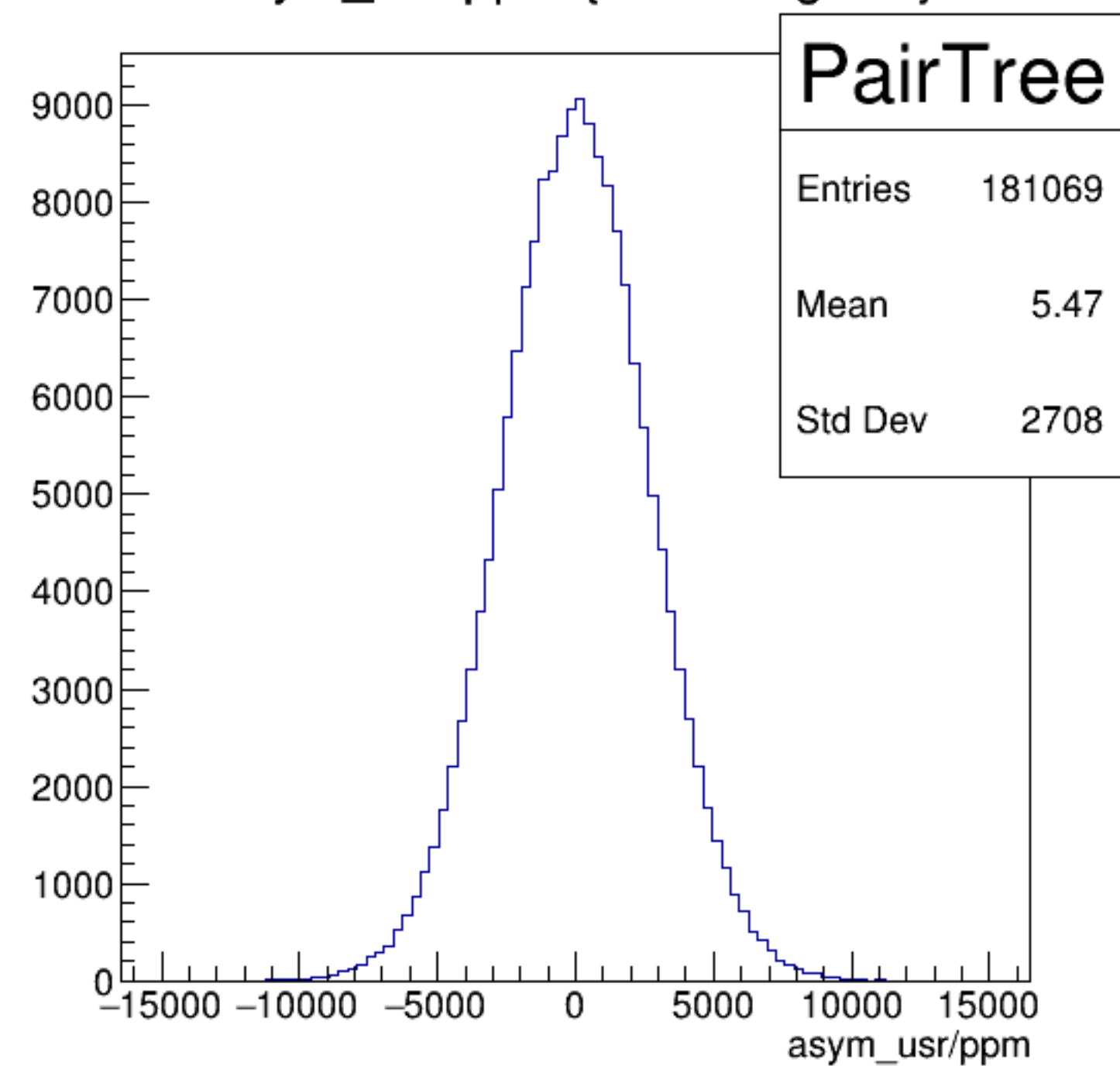
asym_usr/ppm {ErrorFlag==0}
