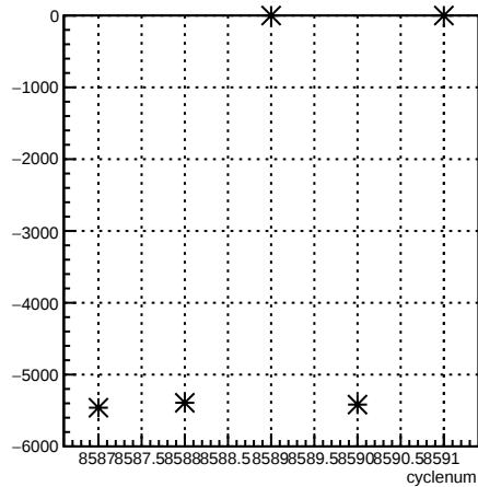
usr_coil3:cyclenum {run == 7288}
