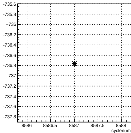
usl_coil6:cyclenum {run == 7288}
