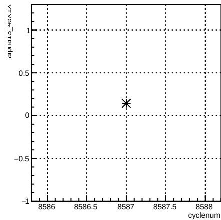
alpha13_4eX1X:cyclenum {run == 7288}
