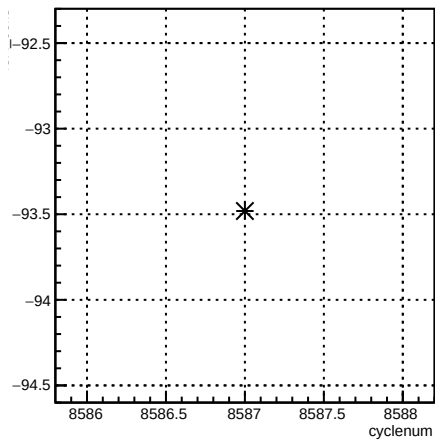
4eX_coil3:cyclenum {run == 7288}
