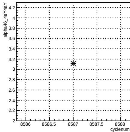
alpha46_4eY4aY:cyclenum {run == 7288}
