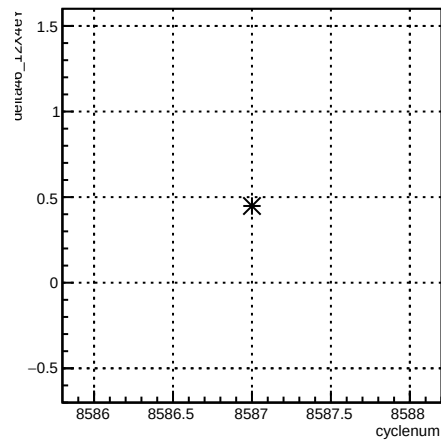
delta46_12X4eY:cyclenum {run == 7288}
