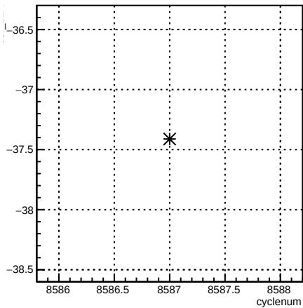
usr_12X:cyclenum {run == 7288}
