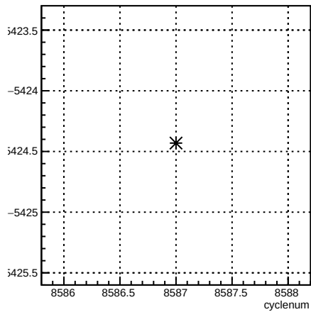
usr_coil7:cyclenum {run == 7288}
