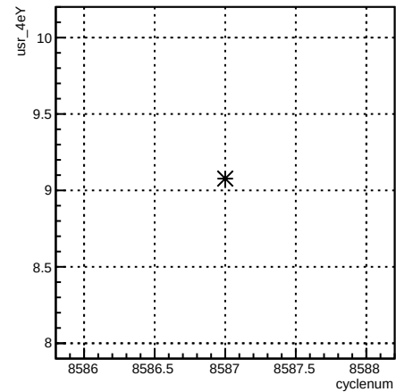
usr_4eY:cyclenum {run == 7288}
