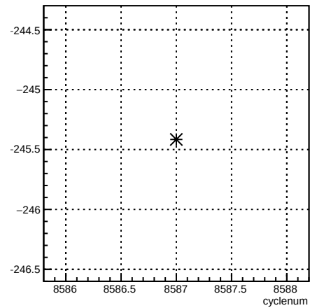
12X_coil6:cyclenum {run == 7288}
