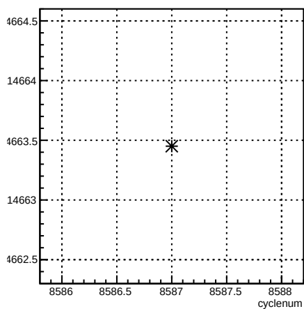
usl_coil7:cyclenum {run == 7288}
