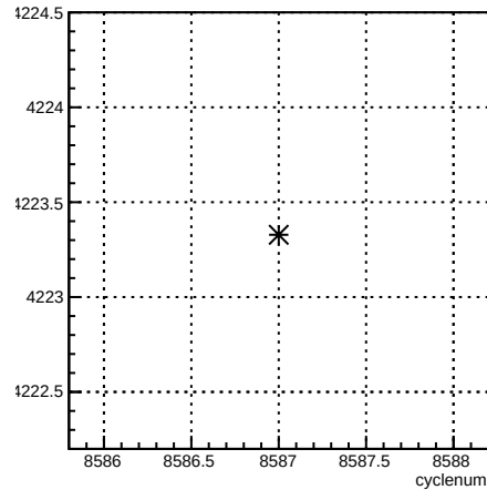
usl_coil4:cyclenum {run == 7288}
