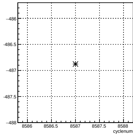
4eX_coil1:cyclenum {run == 7288}
