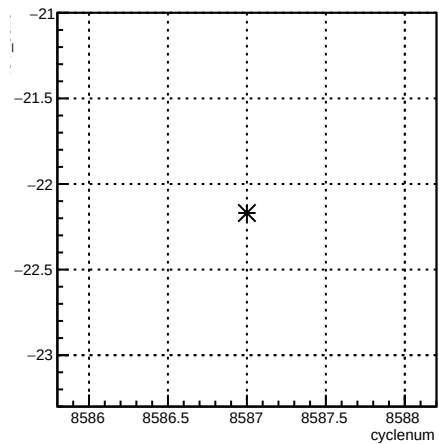
4eY_coil6:cyclenum {run == 7288}
