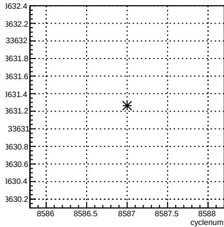
usl_coil1:cyclenum {run == 7288}
