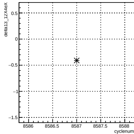
delta13_12X4eX:cyclenum {run == 7288}
