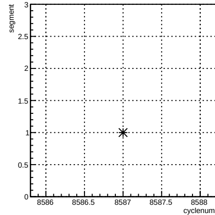
segment:cyclenum {run == 7288}
