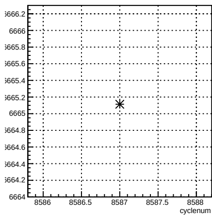
usl_coil3:cyclenum {run == 7288}
