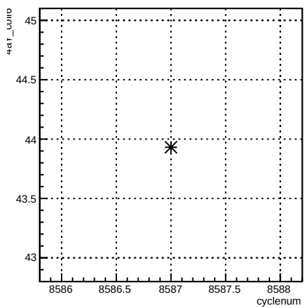
4aY_coil6:cyclenum {run == 7288}
