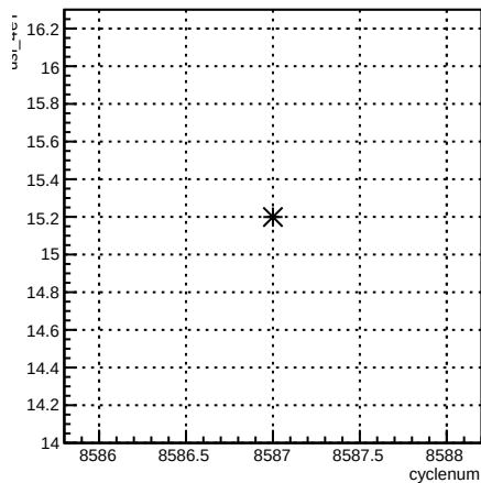
usl_4eY:cyclenum {run == 7288}
