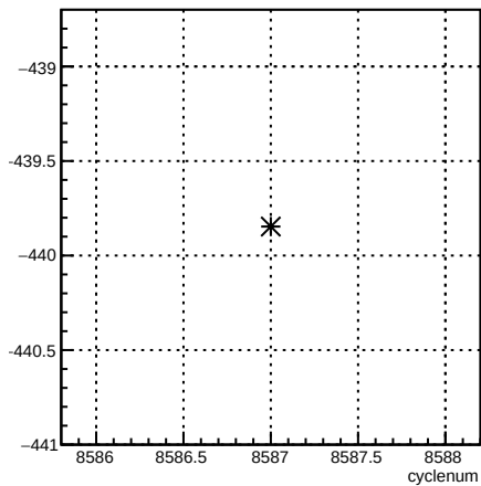
12X_coil7:cyclenum {run == 7288}
