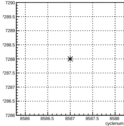
run:cyclenum {run == 7288}
