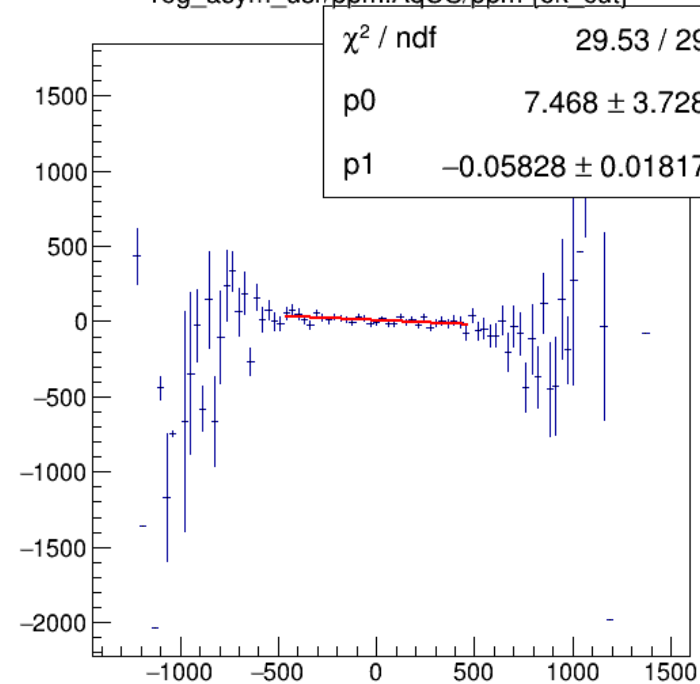
reg_asym_usr/ppm:AqUS/ppm {ok_cut}
