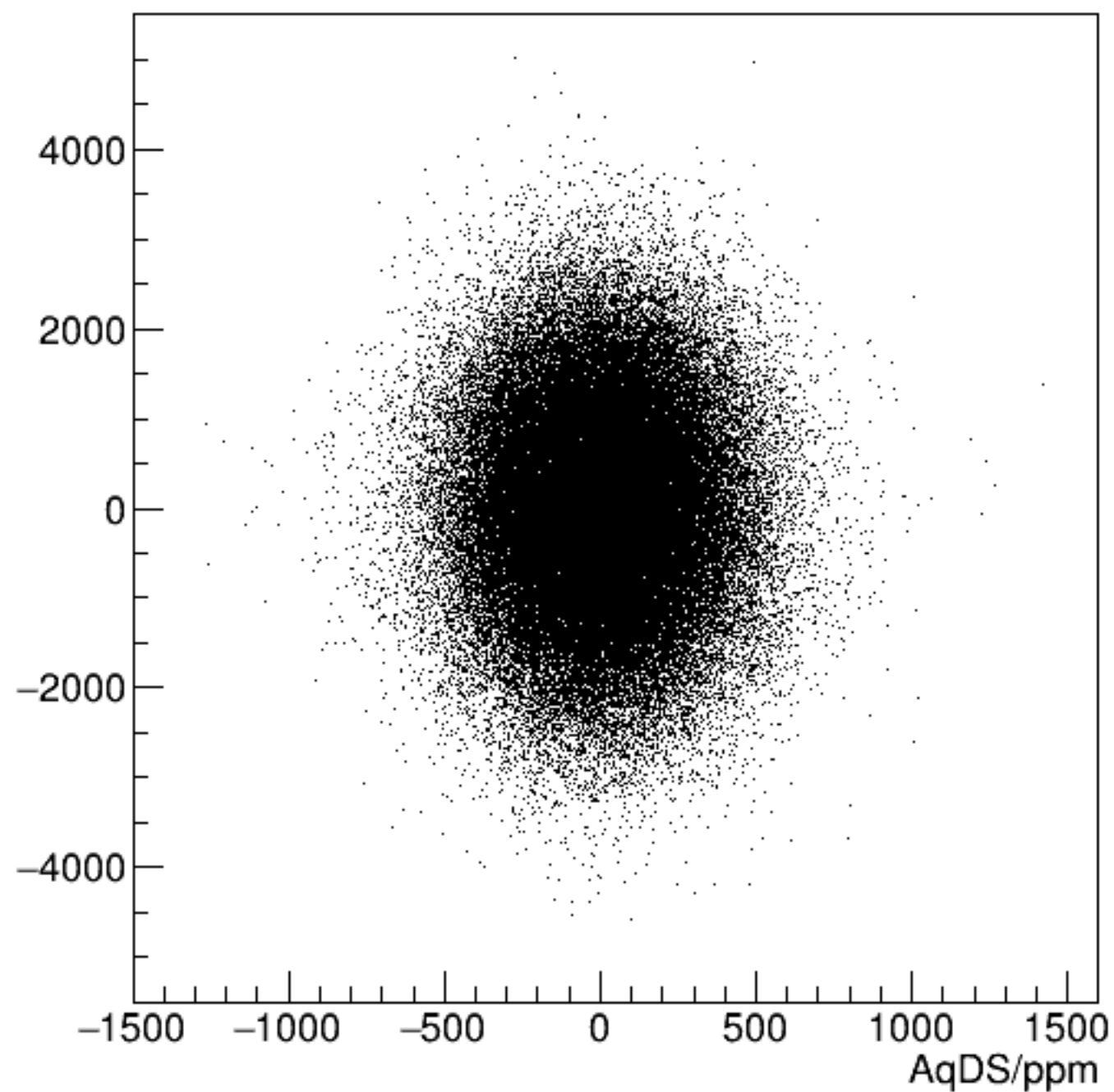
reg_asym_usl/ppm:AqDS/ppm {ok_cut}
