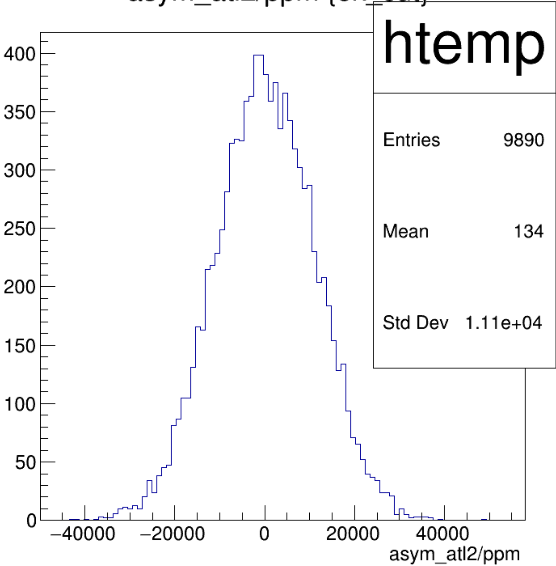
asym_atl2/ppm {ok_cut}
