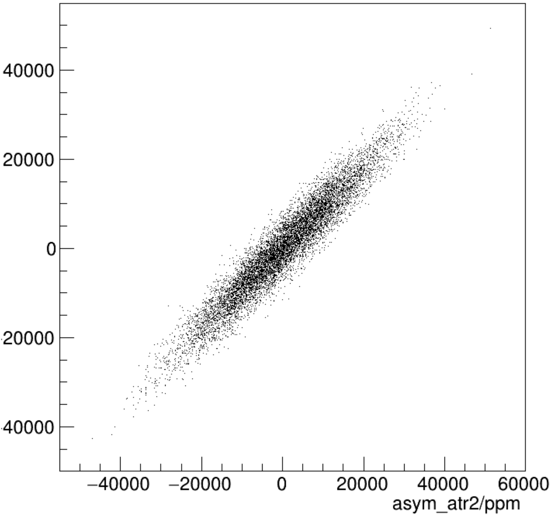
asym_atl2/ppm:asym_atr2/ppm {ok_cut}
