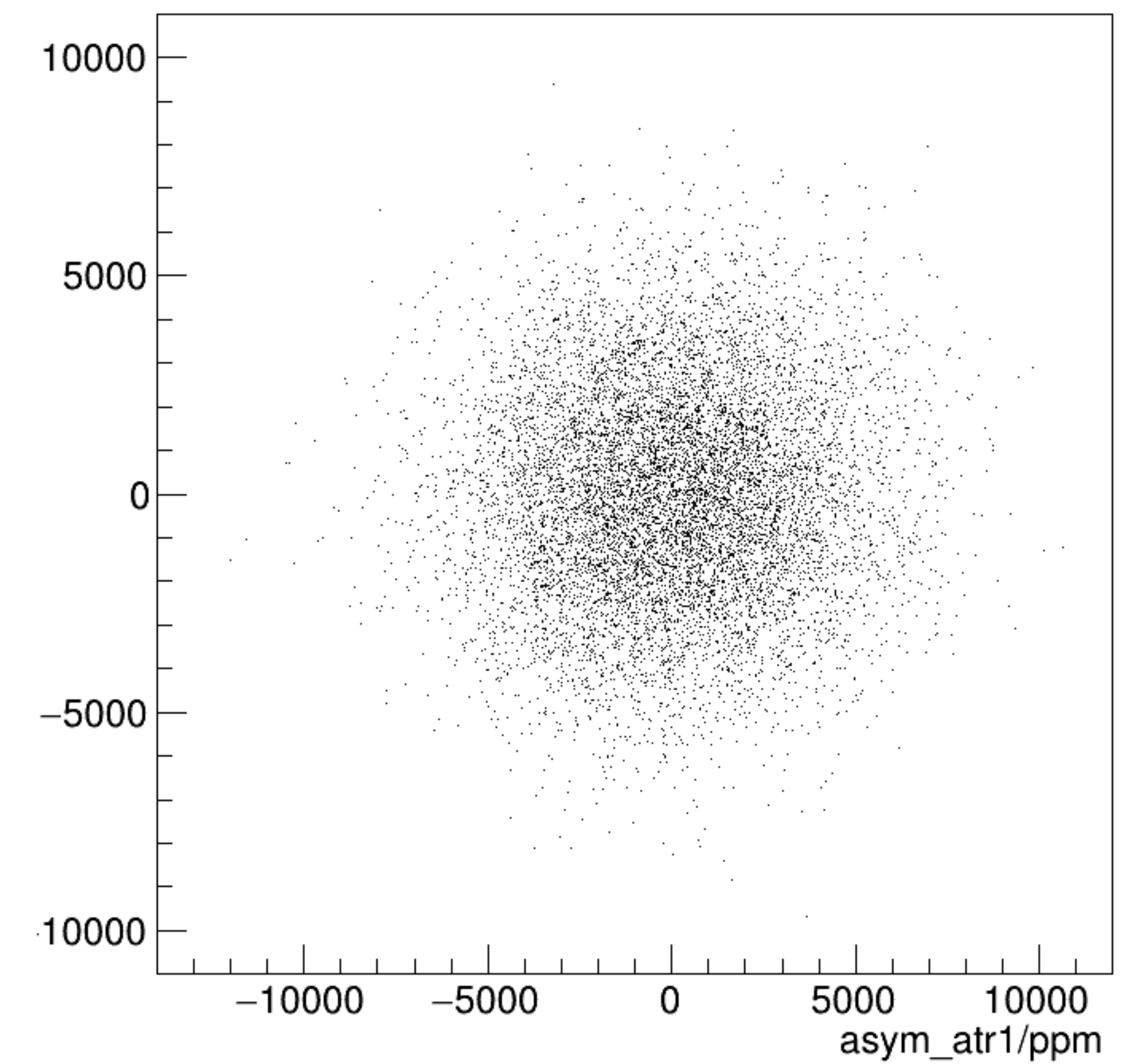
asym_atl1/ppm:asym_atr1/ppm {ok_cut}
