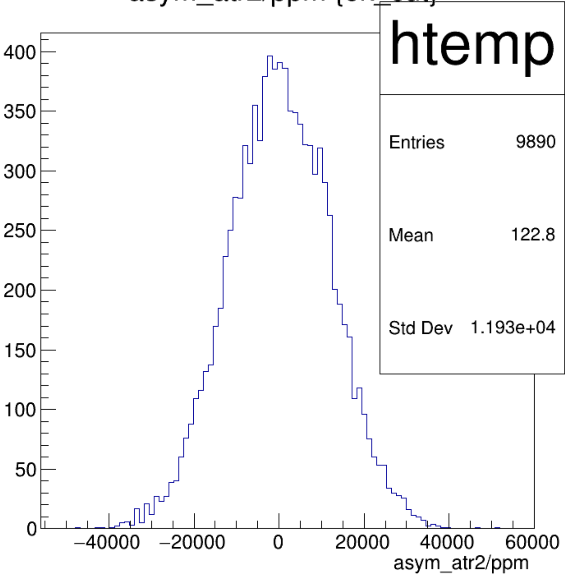
asym_atr2/ppm {ok_cut}
