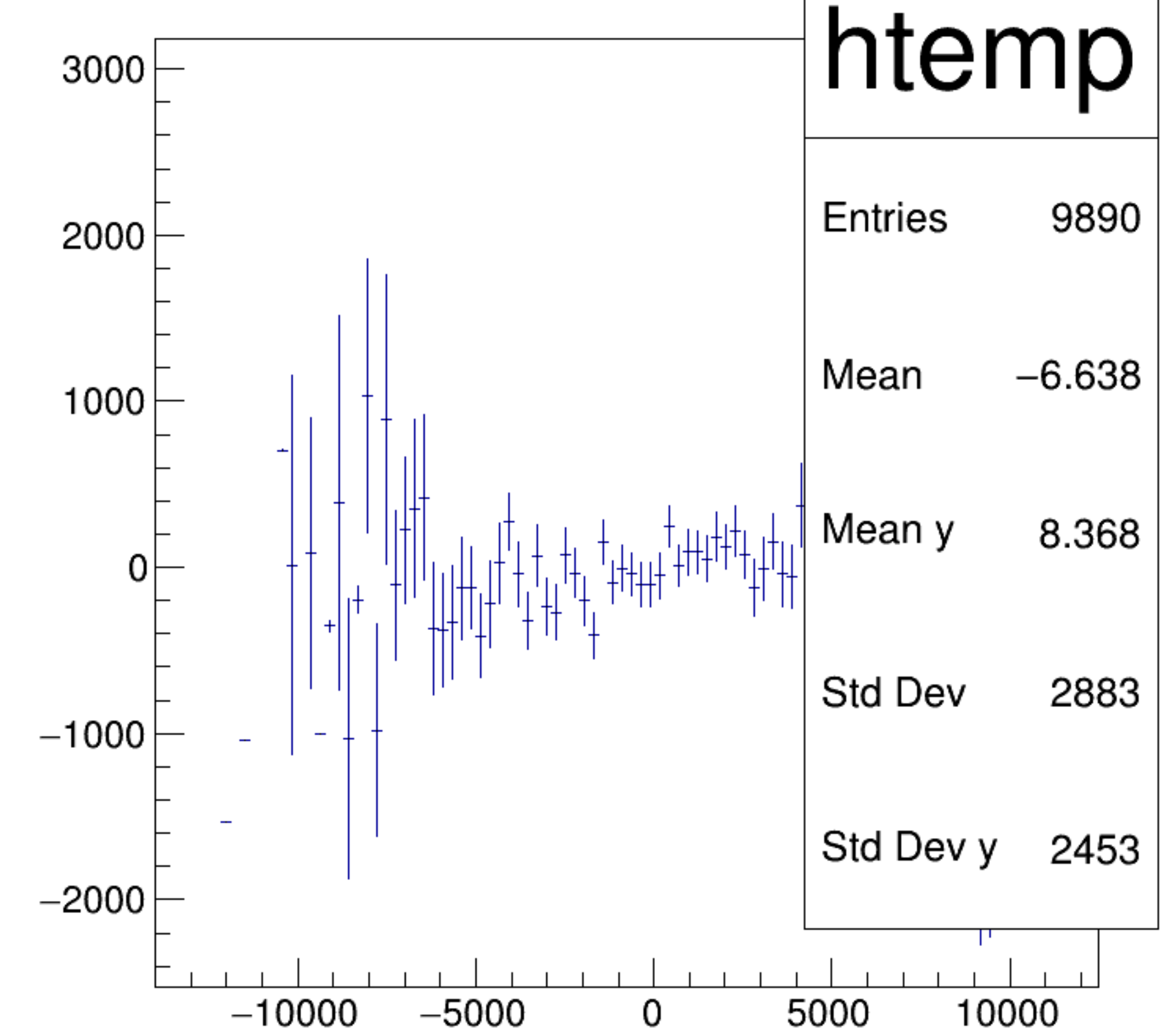
asym_atl1/ppm:asym_atr1/ppm {ok_cut}
