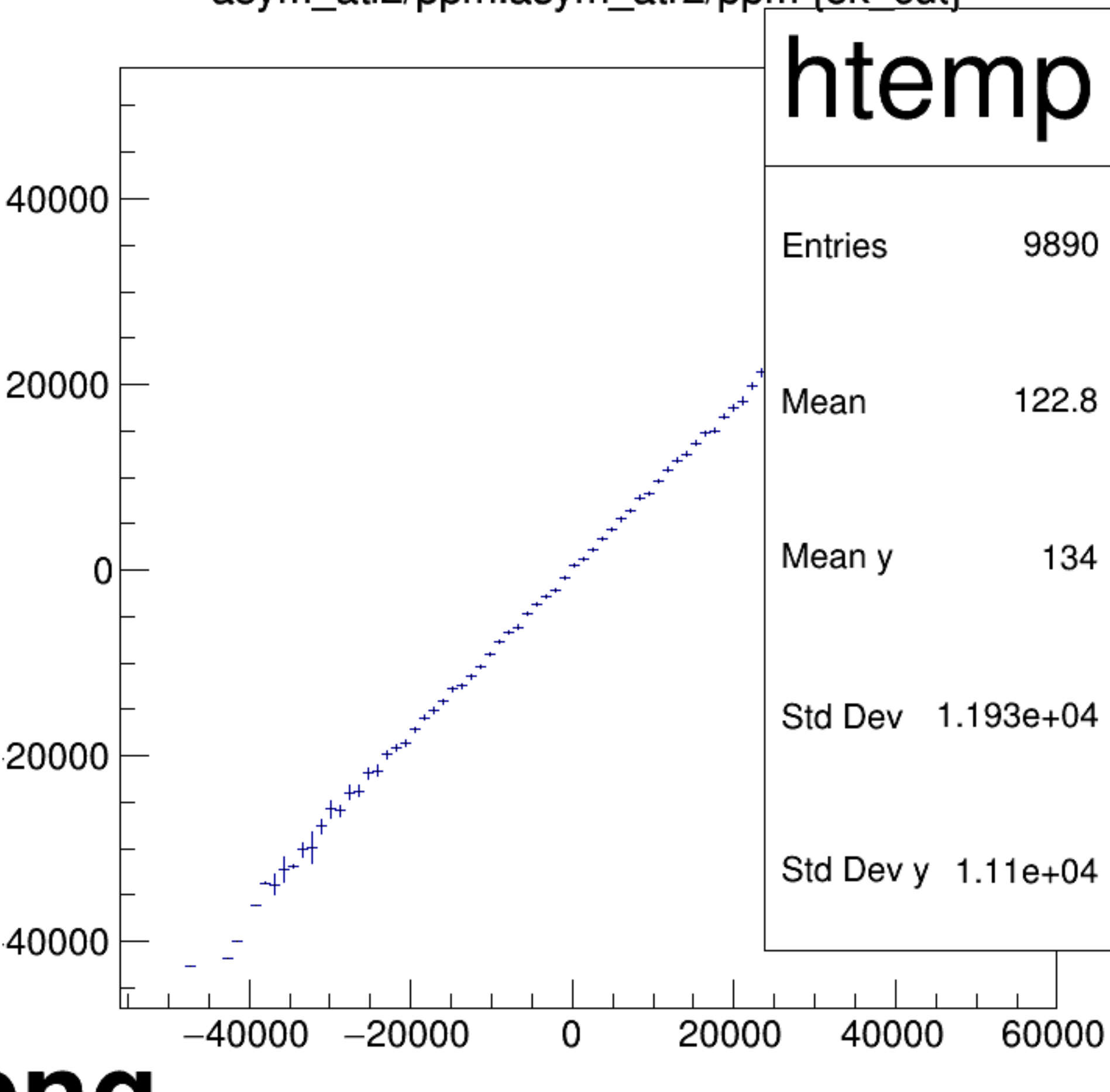
asym_atl2/ppm:asym_atr2/ppm {ok_cut}
