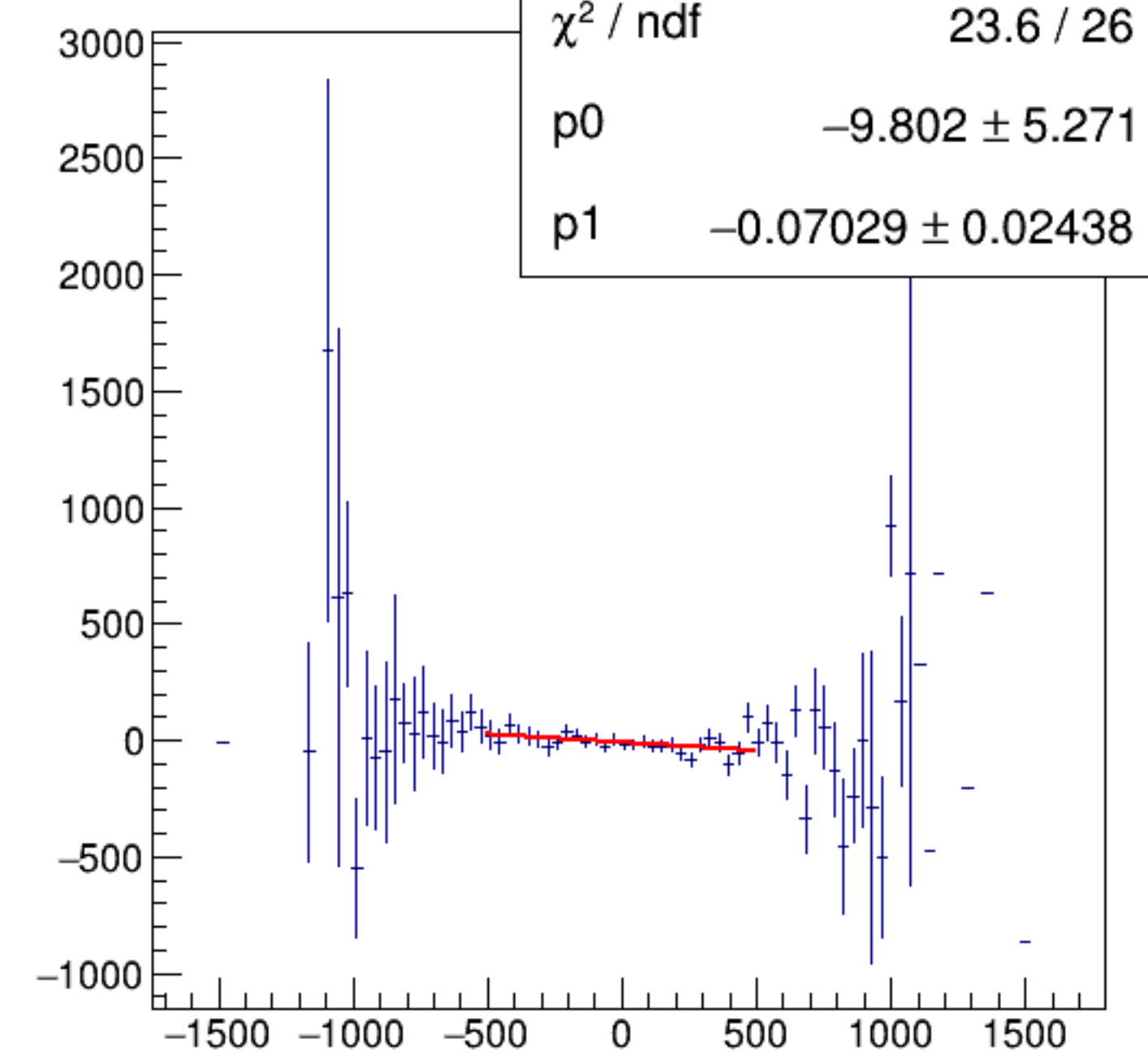
reg_asym_usr/ppm:AqUS/ppm {ok_cut}
