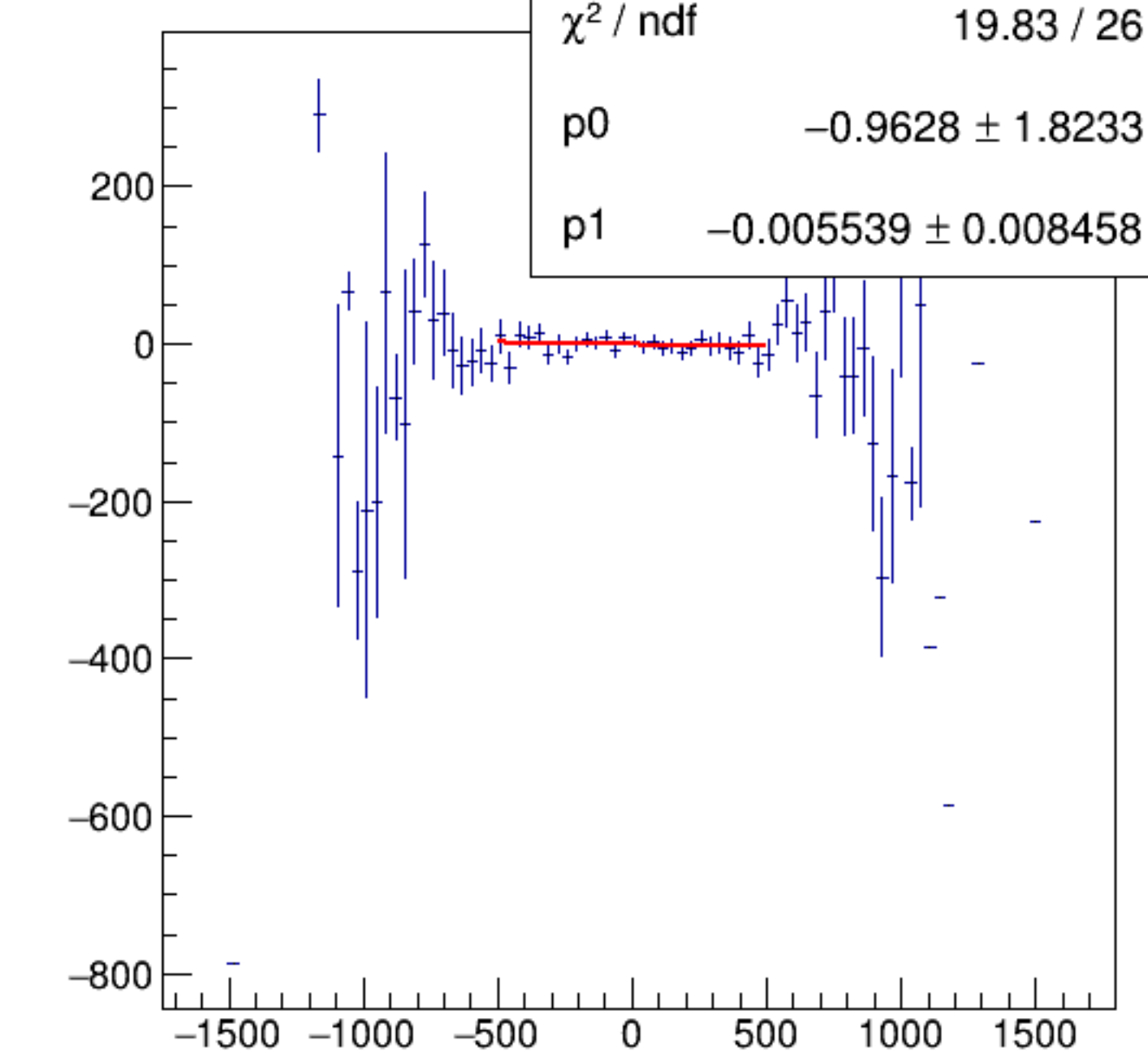
reg_asym_dsr/ppm:AqUS/ppm {ok_cut}
