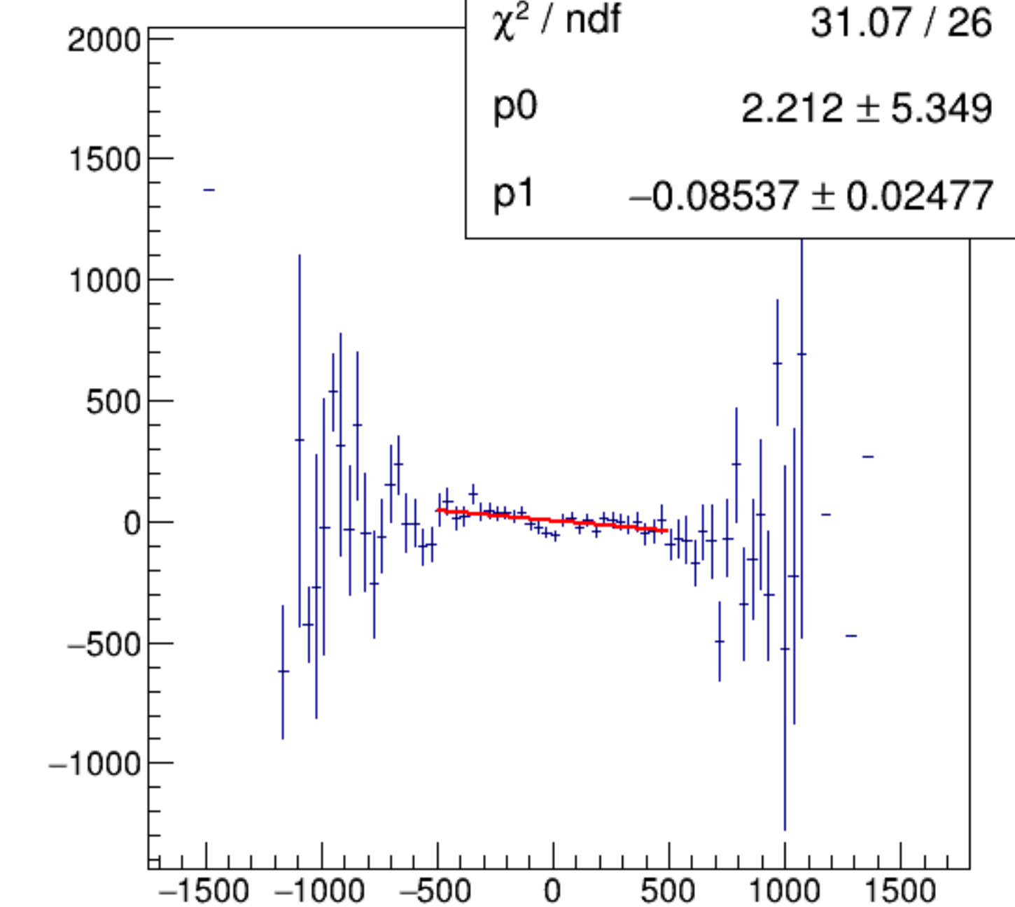
reg_asym_usl/ppm:AqUS/ppm {ok_cut}
