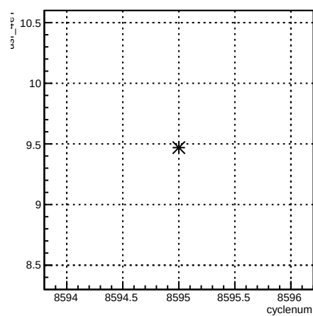
usr_4eY:cyclenum {run == 7292}
