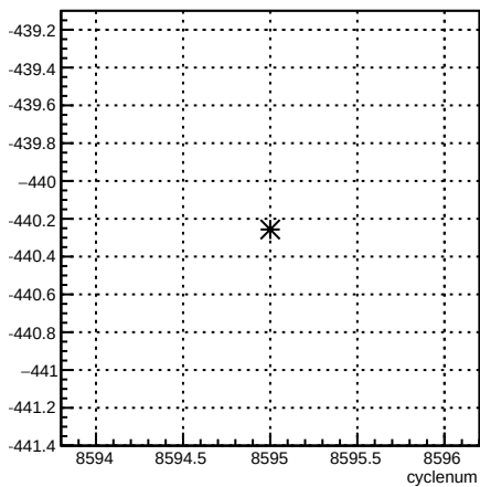
12X_coil7:cyclenum {run == 7292}
