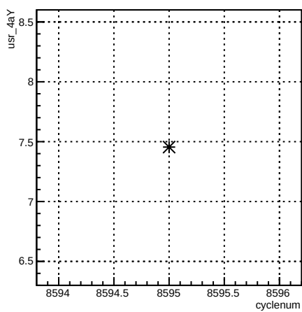
usr_4aY:cyclenum {run == 7292}
