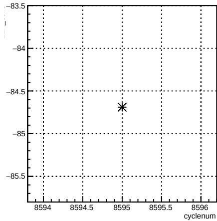
12X_coil3:cyclenum {run == 7292}
