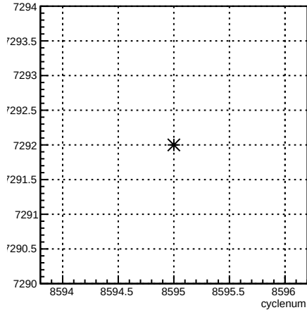
run:cyclenum {run == 7292}
