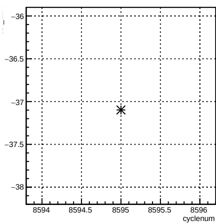
usr_12X:cyclenum {run == 7292}
