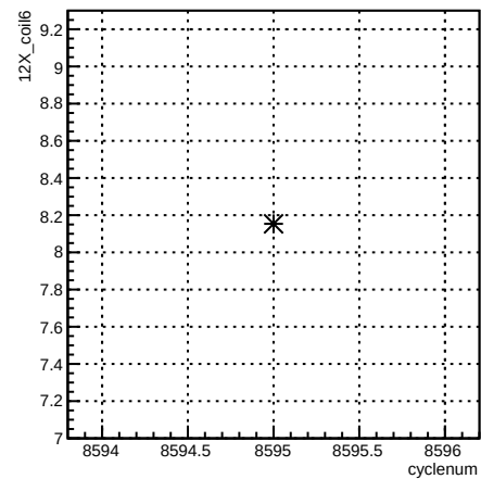
12X_coil6:cyclenum {run == 7292}
