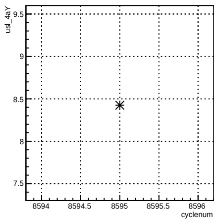
usl_4aY:cyclenum {run == 7292}
