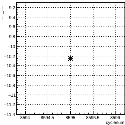
4eY_coil7:cyclenum {run == 7292}
