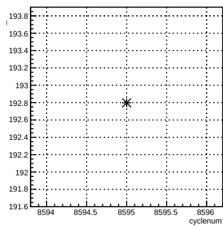
usr_4eX:cyclenum {run == 7292}
