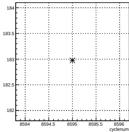
4eY_coil4:cyclenum {run == 7292}
