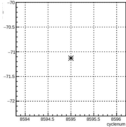
4eX_coil3:cyclenum {run == 7292}
