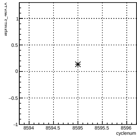
alpha13_4eX1X:cyclenum {run == 7292}
