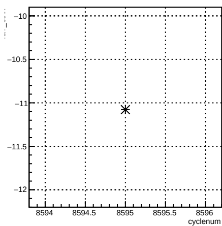
4aY_coil7:cyclenum {run == 7292}
