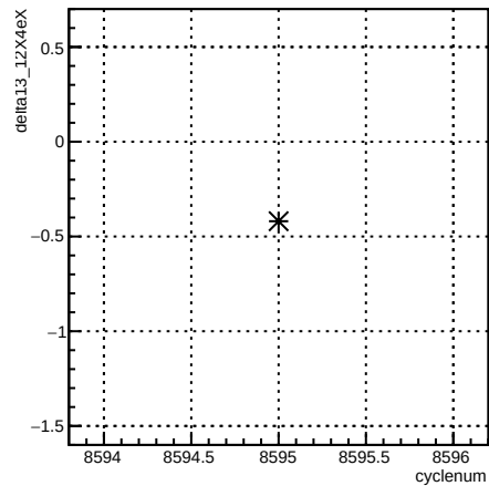
delta13_12X4eX:cyclenum {run == 7292}
