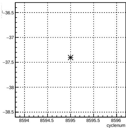
usl_12X:cyclenum {run == 7292}
