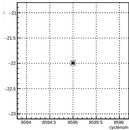
4eY_coil6:cyclenum {run == 7292}
