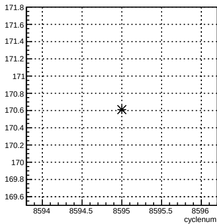
4aY_coil4:cyclenum {run == 7292}
