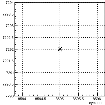
run:cyclenum {run == 7292}
