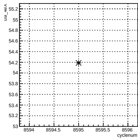
usl_4eX:cyclenum {run == 7292}
