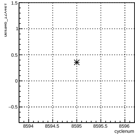
delta46_12X4eY:cyclenum {run == 7292}
