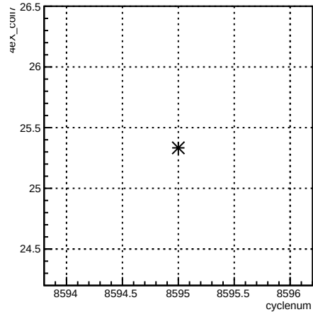
4eX_coil7:cyclenum {run == 7292}
