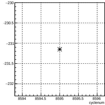
12X_coil1:cyclenum {run == 7292}
