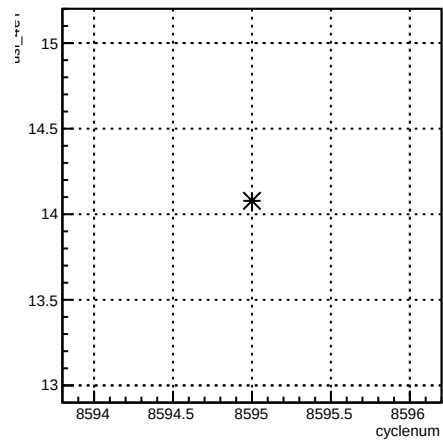
usl_4eY:cyclenum {run == 7292}
