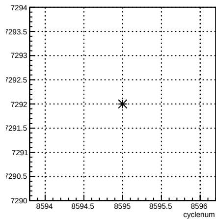
run:cyclenum {run == 7292}
