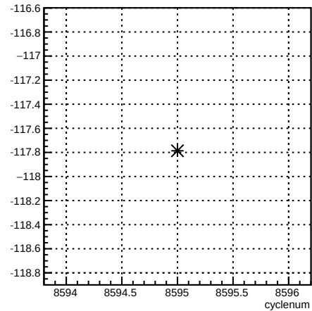
usl_1X:cyclenum {run == 7292}
