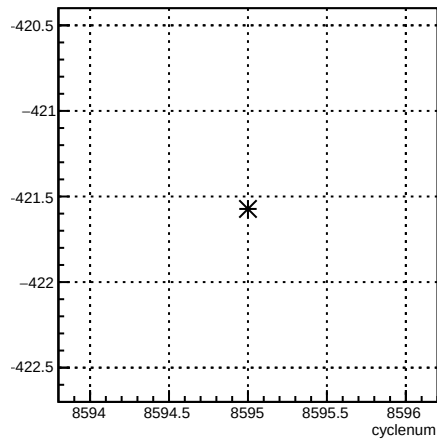
4eX_coil1:cyclenum {run == 7292}
