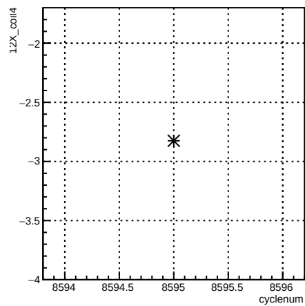
12X_coil4:cyclenum {run == 7292}
