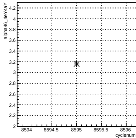
alpha46_4eY4aY:cyclenum {run == 7292}
