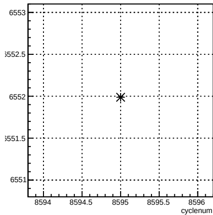
usl_coil7:cyclenum {run == 7292}
