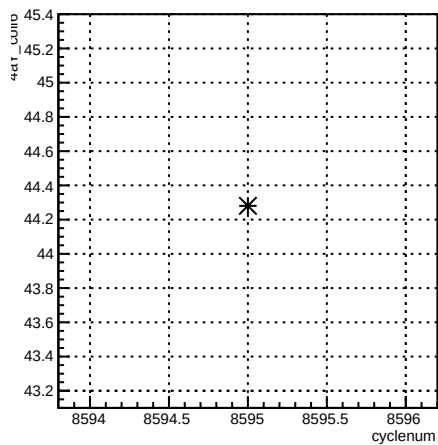
4aY_coil6:cyclenum {run == 7292}
