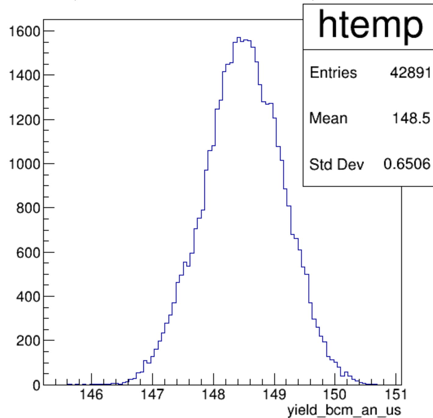
yield_bcm_an_us {ErrorFlag==0}
