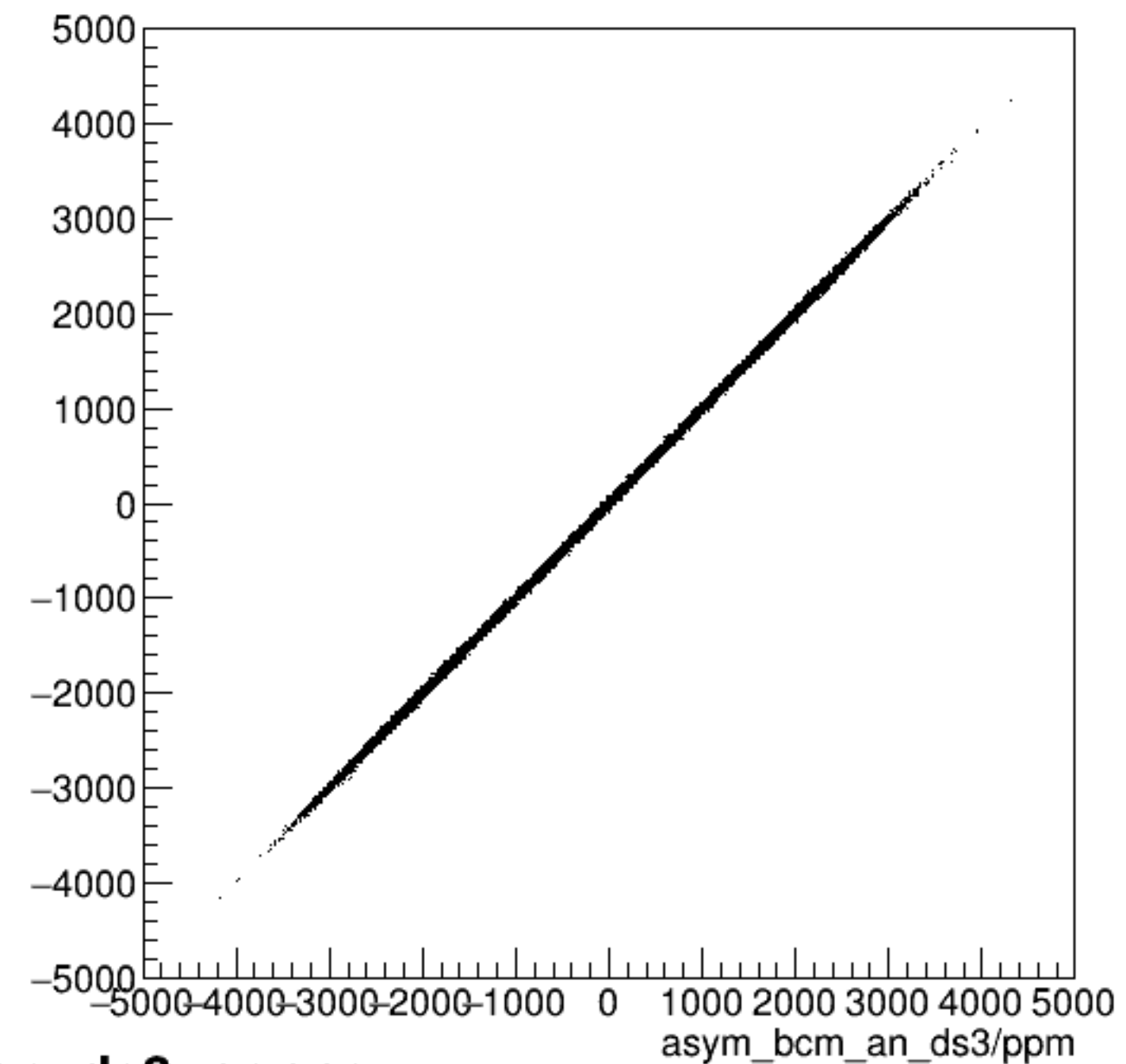
run7292_000_asym_bcm_an_us_vs_asym_bcm_an_ds3_pr.png
