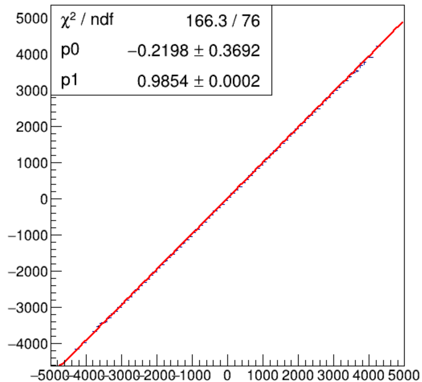
run7292_000_asym_bcm_dg_us_vs_asym_bcm_dg_ds_pr.png
