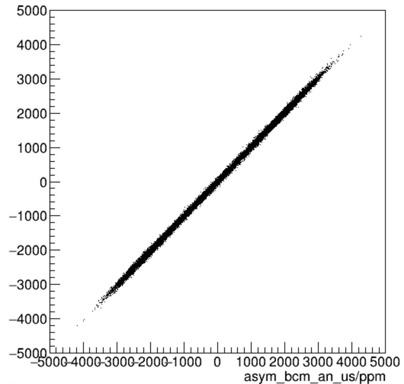
run7292_000_asym_bcm_dg_ds_vs_asym_bcm_an_us_pr.png
