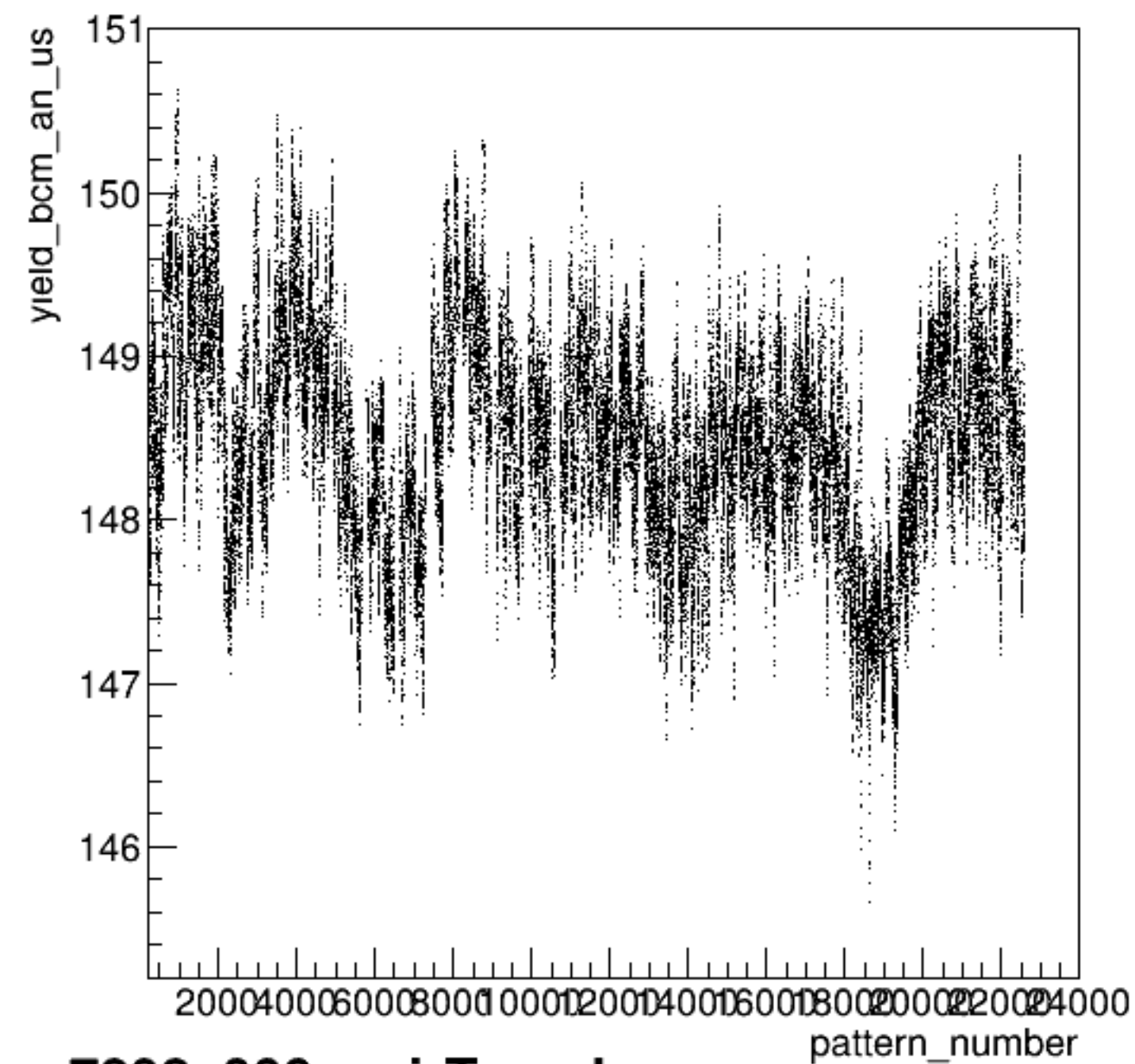
yield_bcm_an_us:pattern_number {ErrorFlag==0}
