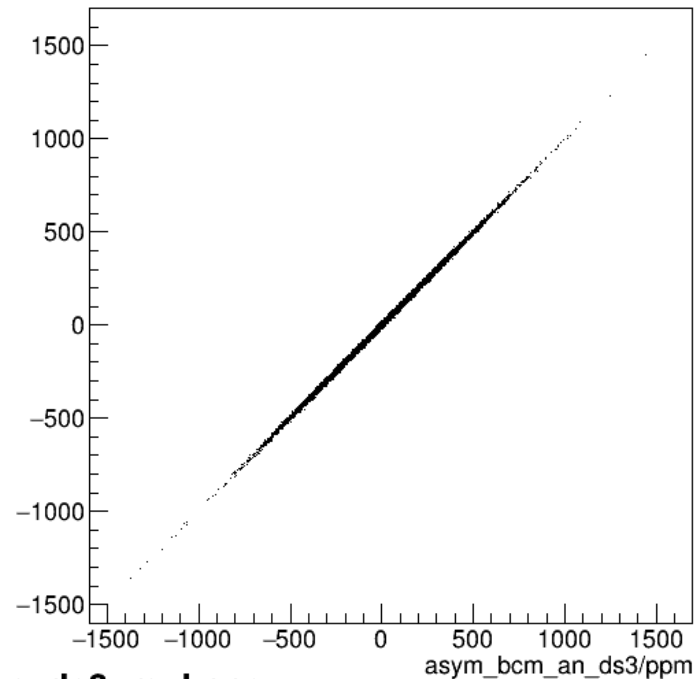
run7292_000_asym_bcm_an_ds_vs_asym_bcm_an_ds3_mul.png
