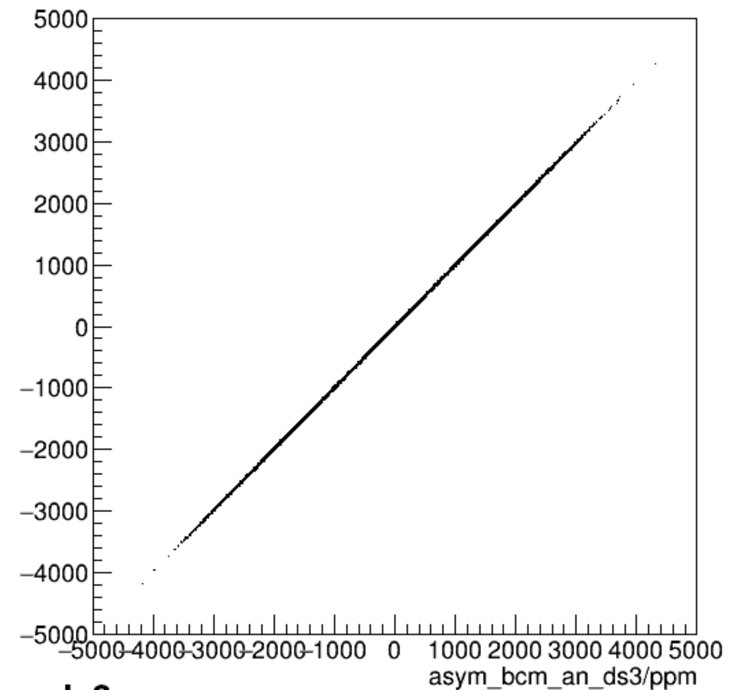
run7292_000_asym_bcm_an_ds_vs_asym_bcm_an_ds3_pr.png
