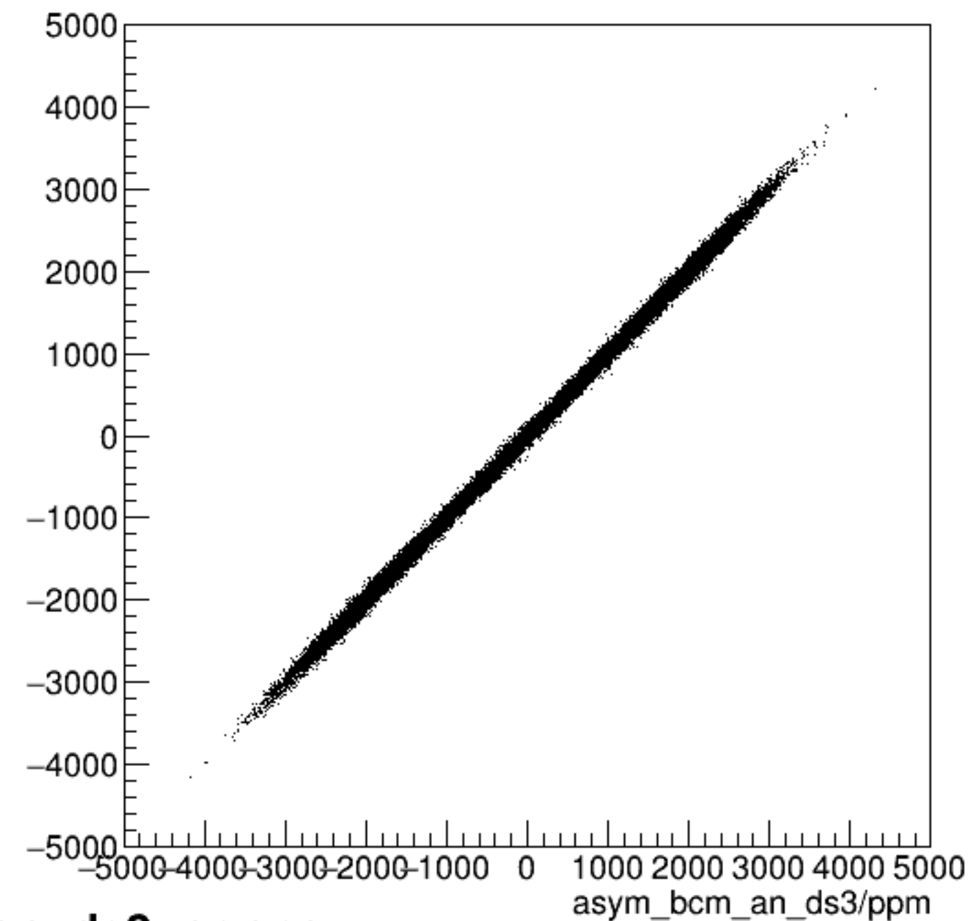
run7292_000_asym_bcm_dg_us_vs_asym_bcm_an_ds3_pr.png
