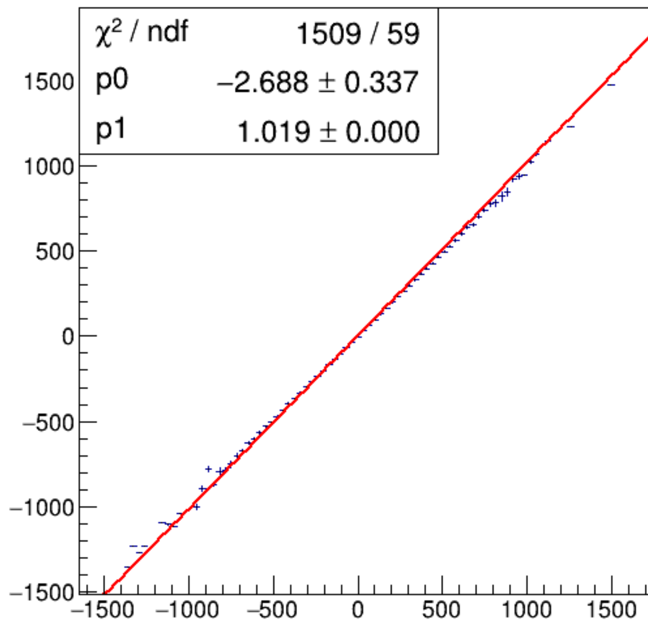
run7292_000_asym_bcm_dg_us_vs_asym_bcm_dg_ds_mul.png
