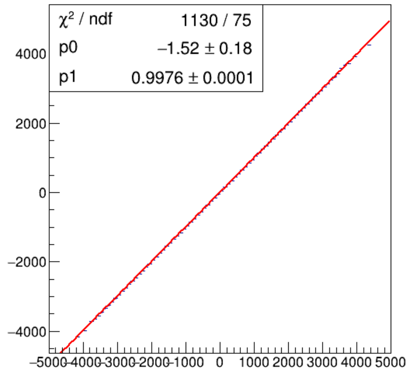
run7292_000_asym_bcm_an_us_vs_asym_bcm_an_ds3_pr.png
