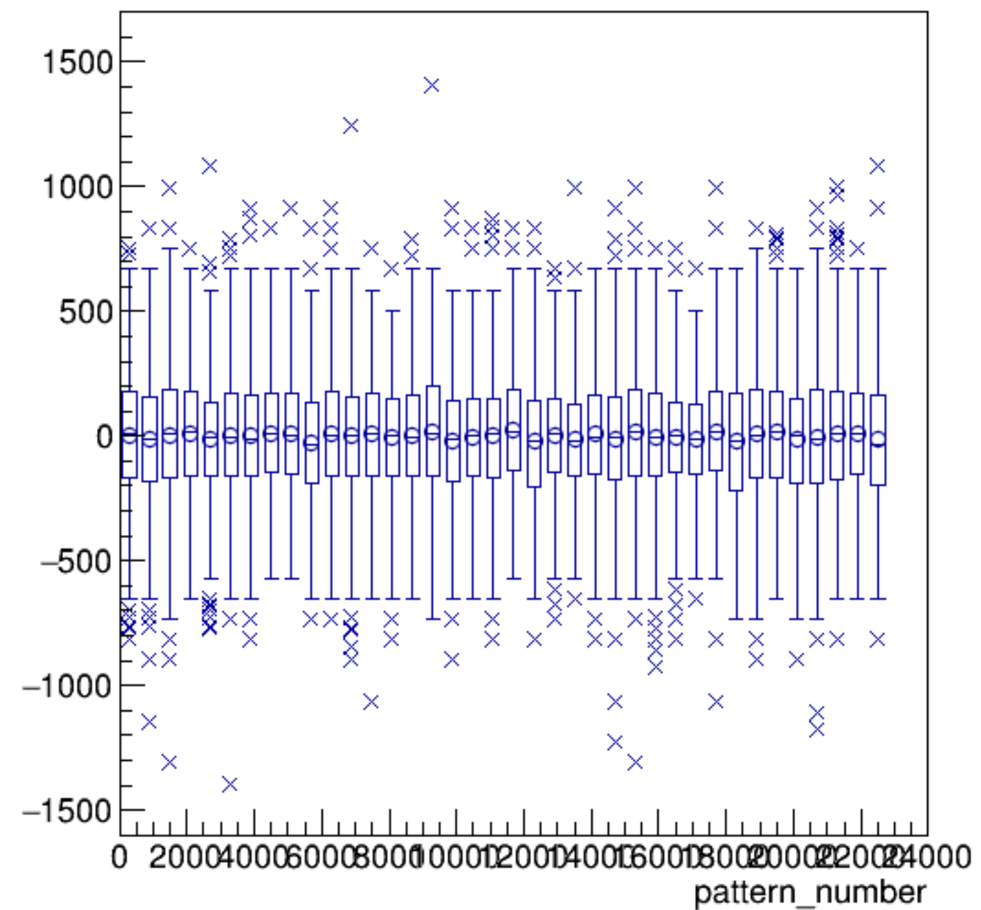
asym_bcm_an_us/ppm:pattern_number {ErrorFlag==0}
