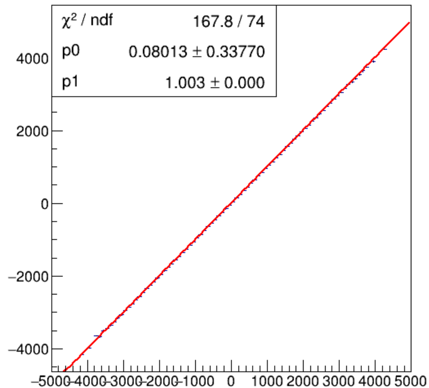
run7292_000_asym_bcm_dg_us_vs_asym_bcm_an_ds_pr.png
