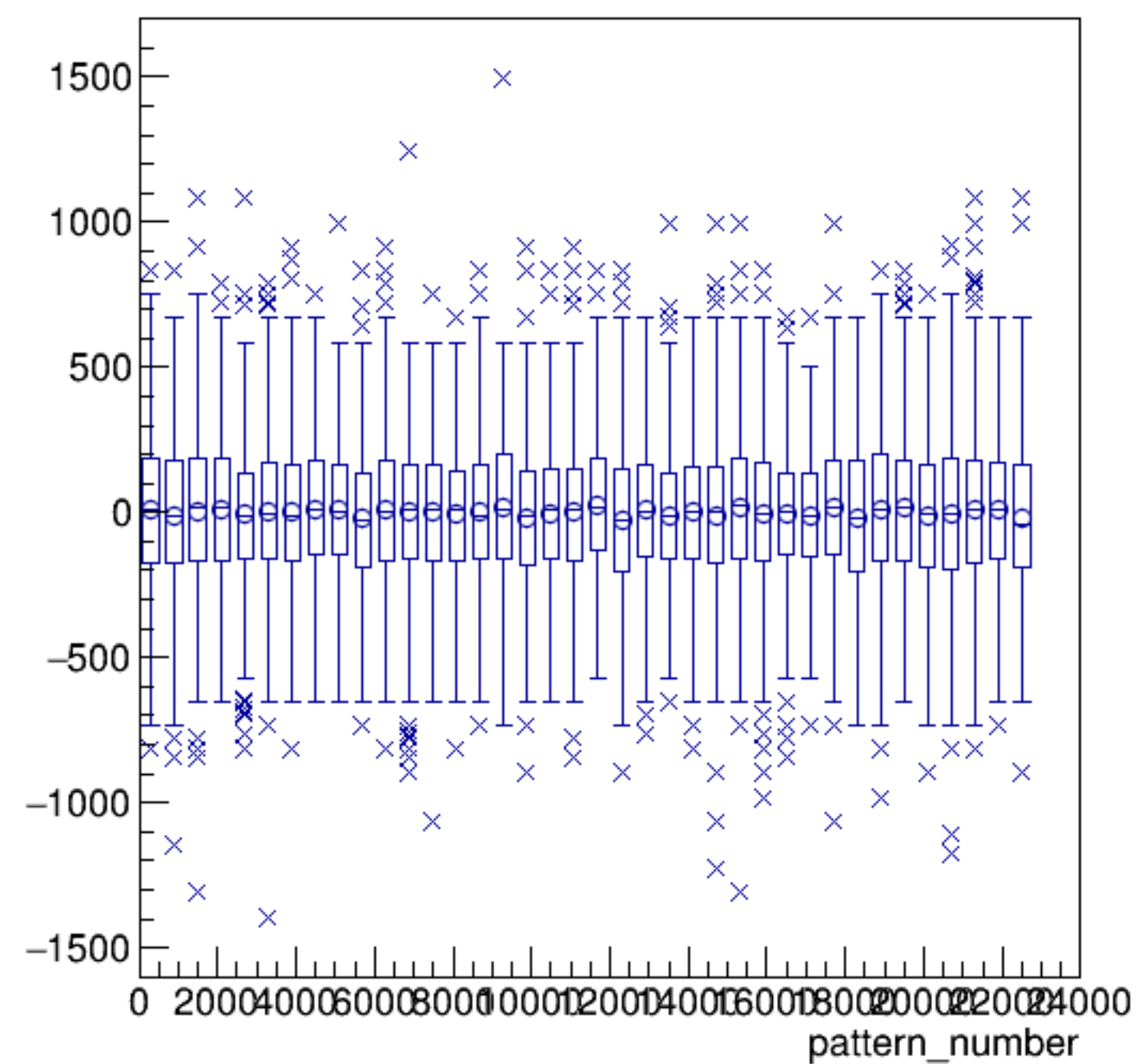
asym_bcm_dg_ds/ppm:pattern_number {ErrorFlag==0}
