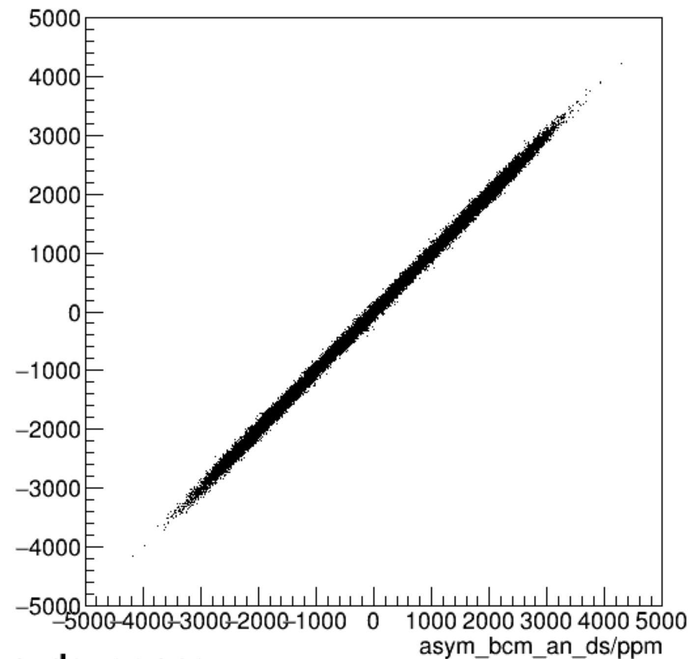
run7292_000_asym_bcm_dg_us_vs_asym_bcm_an_ds_pr.png
