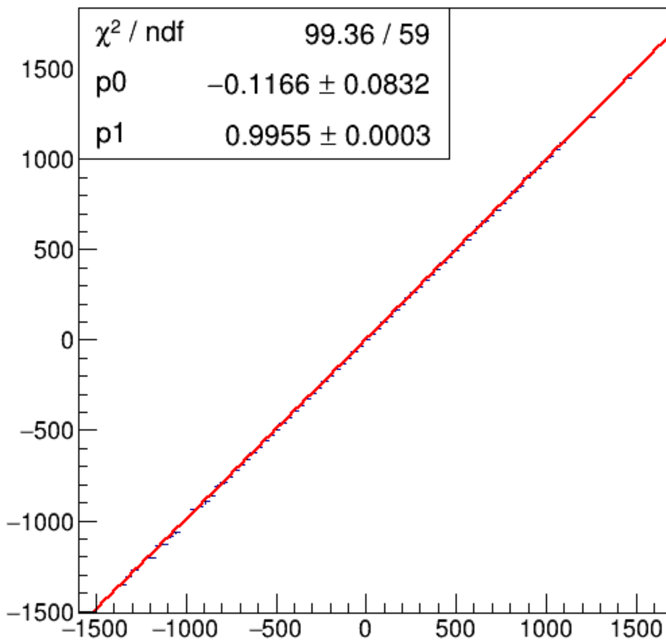
run7292_000_asym_bcm_an_ds_vs_asym_bcm_an_ds3_mul.png
