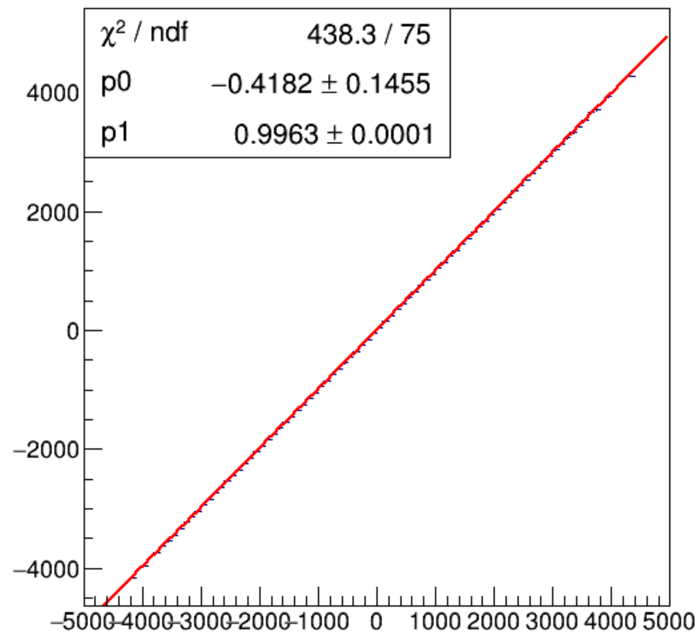
run7292_000_asym_bcm_an_ds_vs_asym_bcm_an_ds3_pr.png
