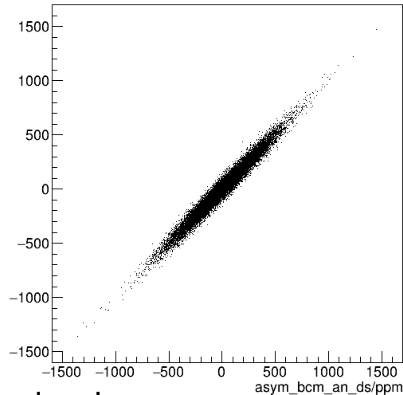
run7292_000_asym_bcm_dg_us_vs_asym_bcm_an_ds_mul.png
