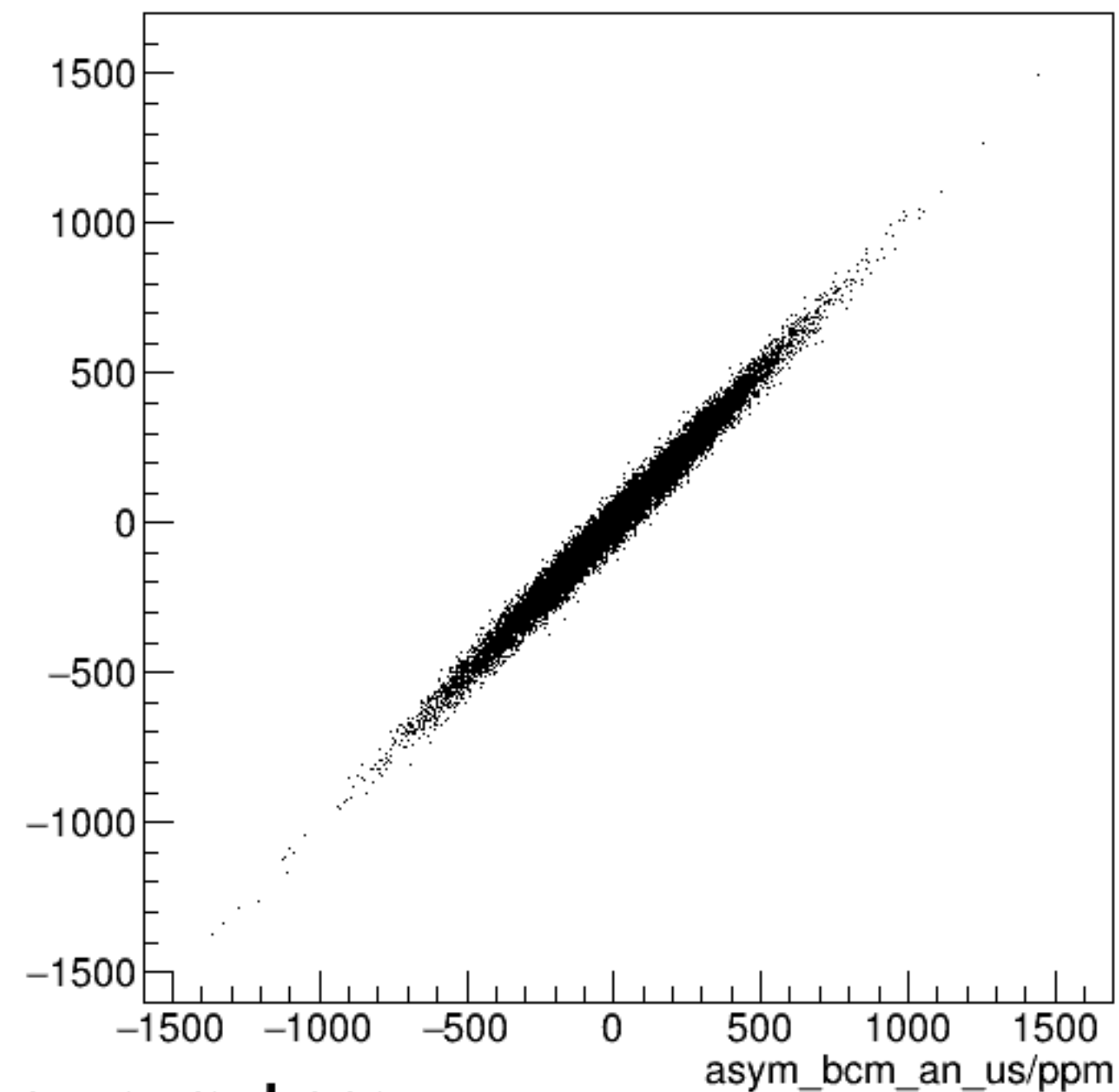
run7292_000_asym_bcm_dg_ds_vs_asym_bcm_an_us_mul.png
