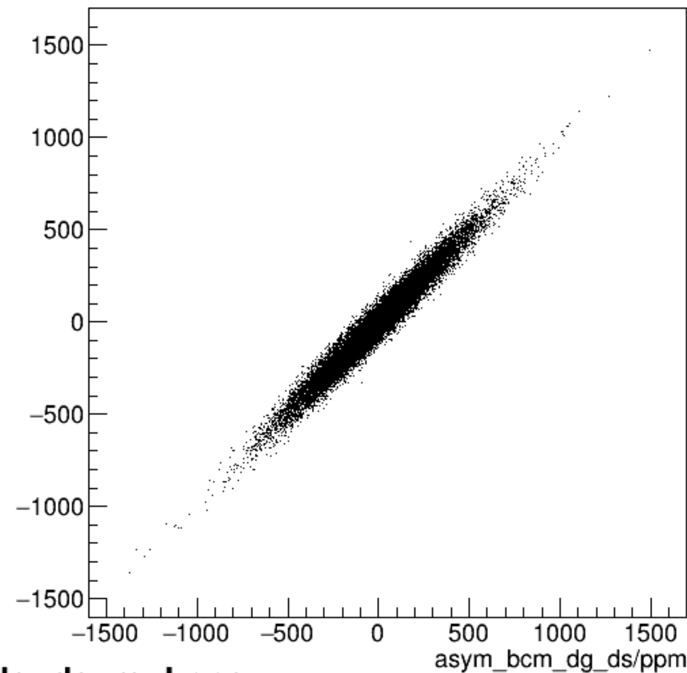
run7292_000_asym_bcm_dg_us_vs_asym_bcm_dg_ds_mul.png
