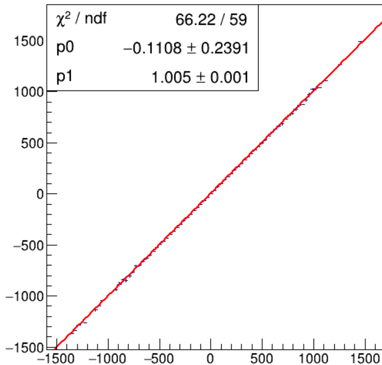
run7292_000_asym_bcm_dg_ds_vs_asym_bcm_an_us_mul.png
