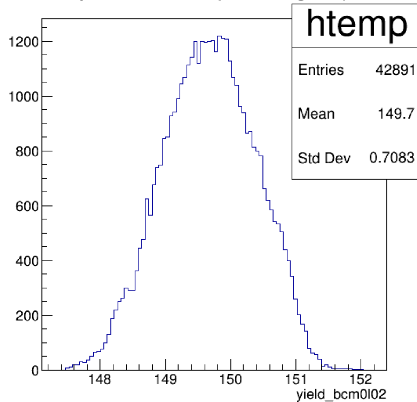
yield_bcm0l02 {ErrorFlag==0}
