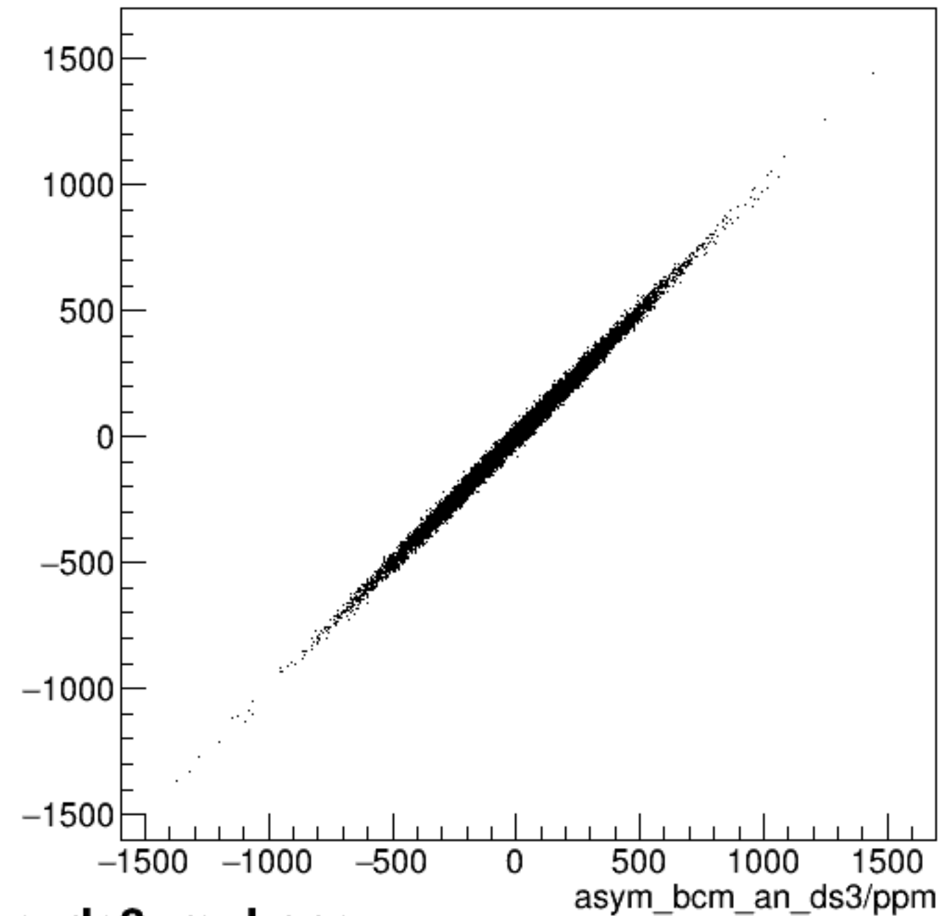
run7292_000_asym_bcm_an_us_vs_asym_bcm_an_ds3_mul.png
