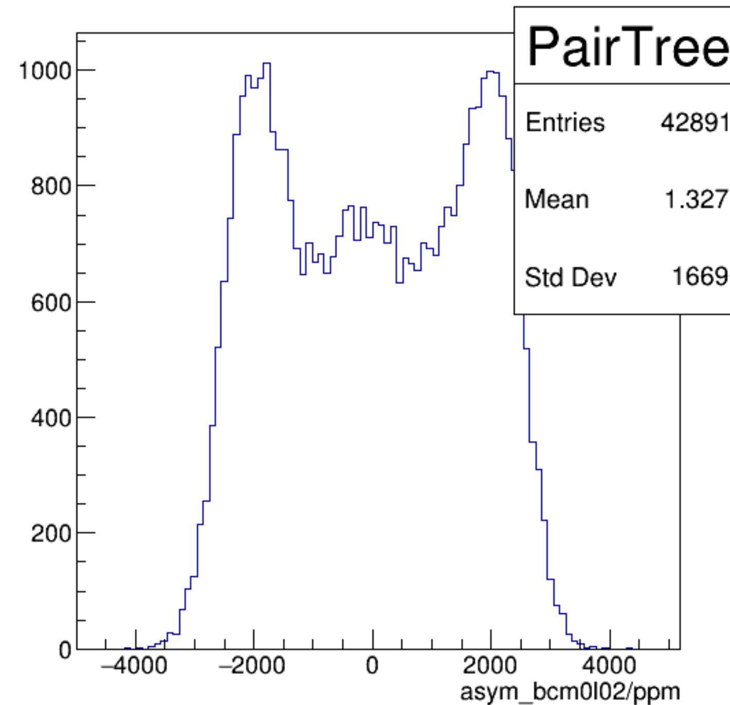
asym_bcm0l02/ppm {ErrorFlag==0}
