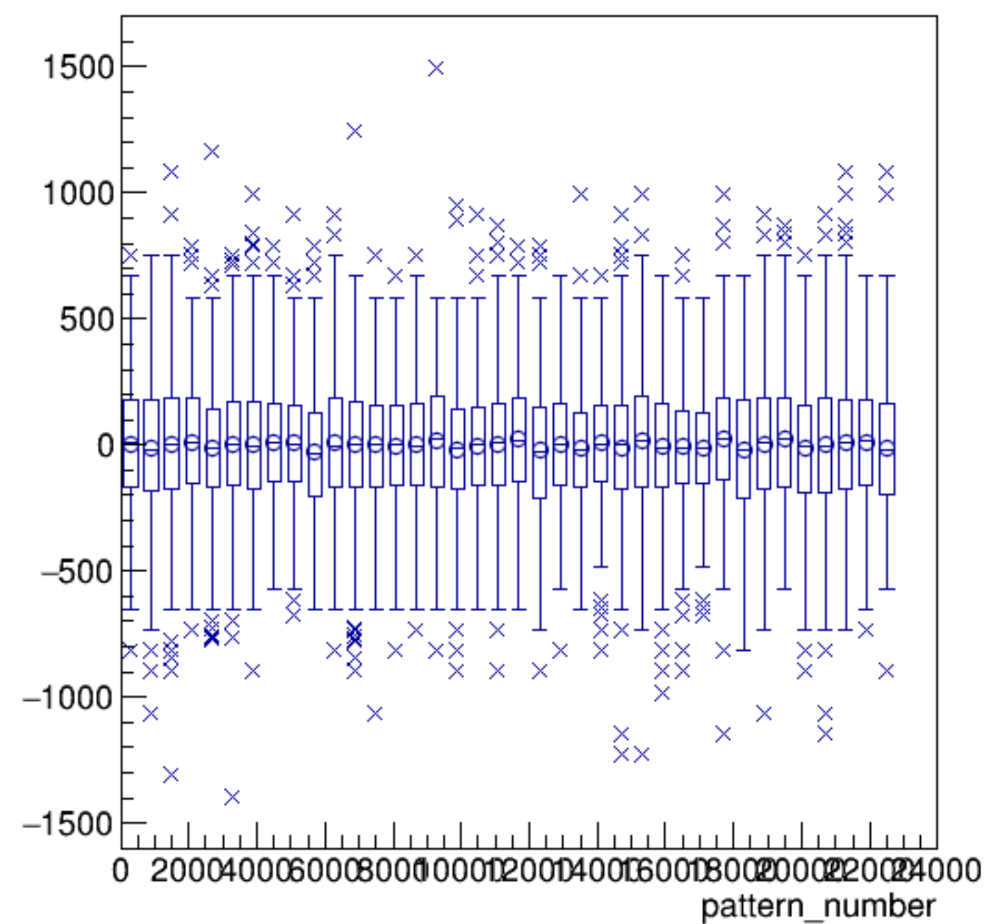
asym_bcm_dg_us/ppm:pattern_number {ErrorFlag==0}
