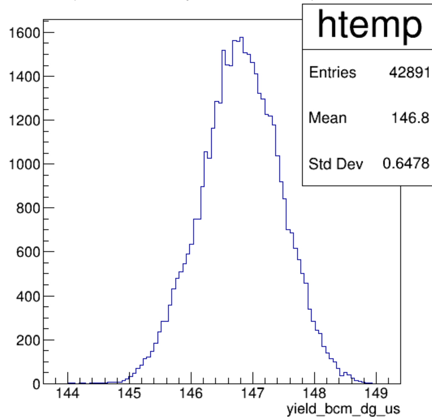
yield_bcm_dg_us {ErrorFlag==0}
