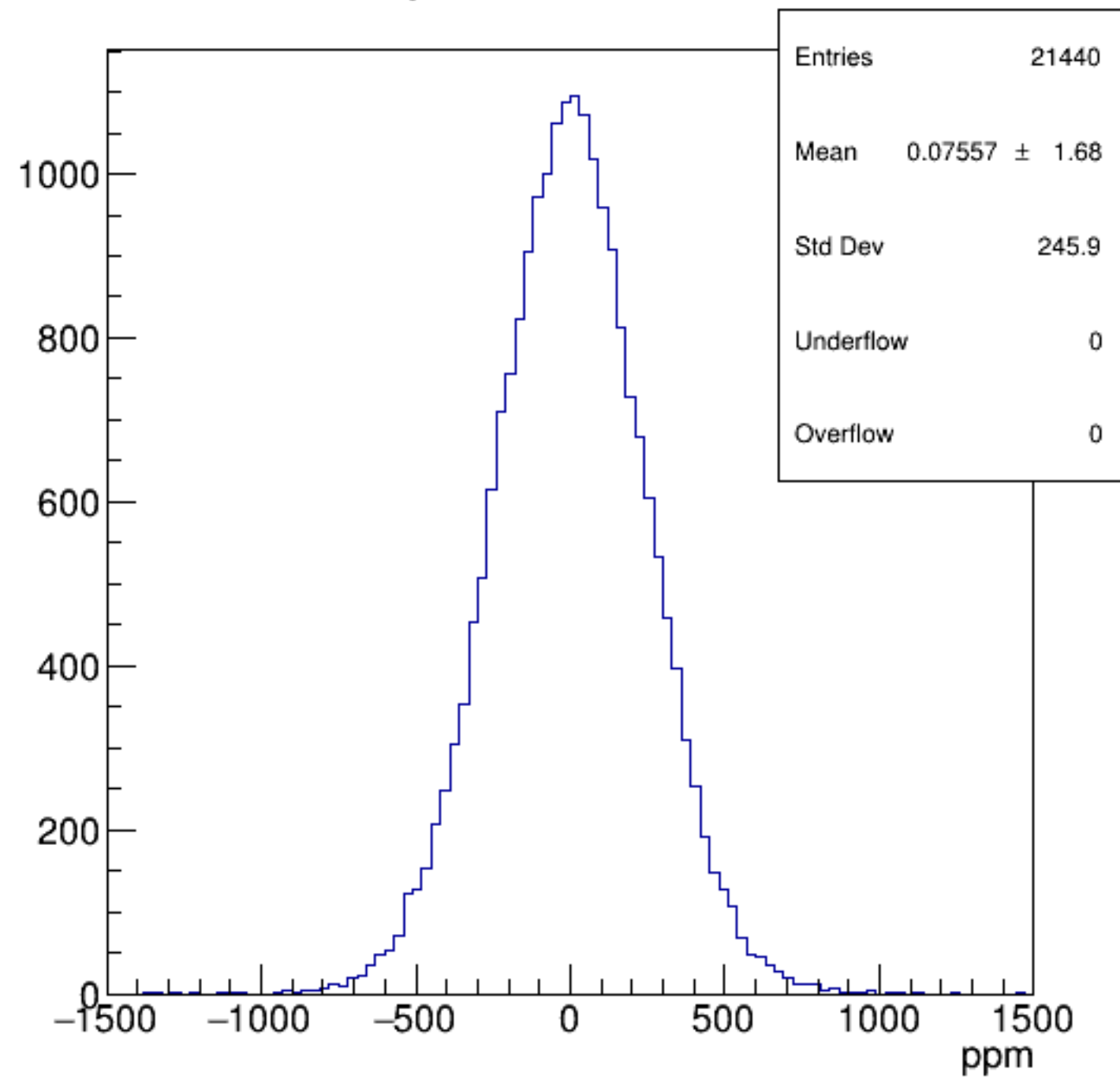
asym_bcm_an_us
