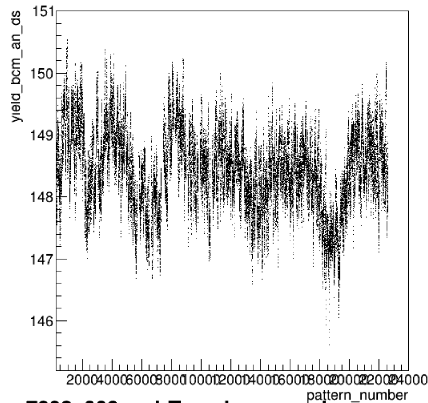
yield_bcm_an_ds:pattern_number {ErrorFlag==0}
