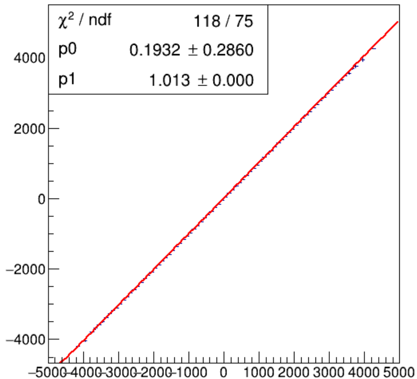
run7292_000_asym_bcm_dg_ds_vs_asym_bcm_an_us_pr.png
