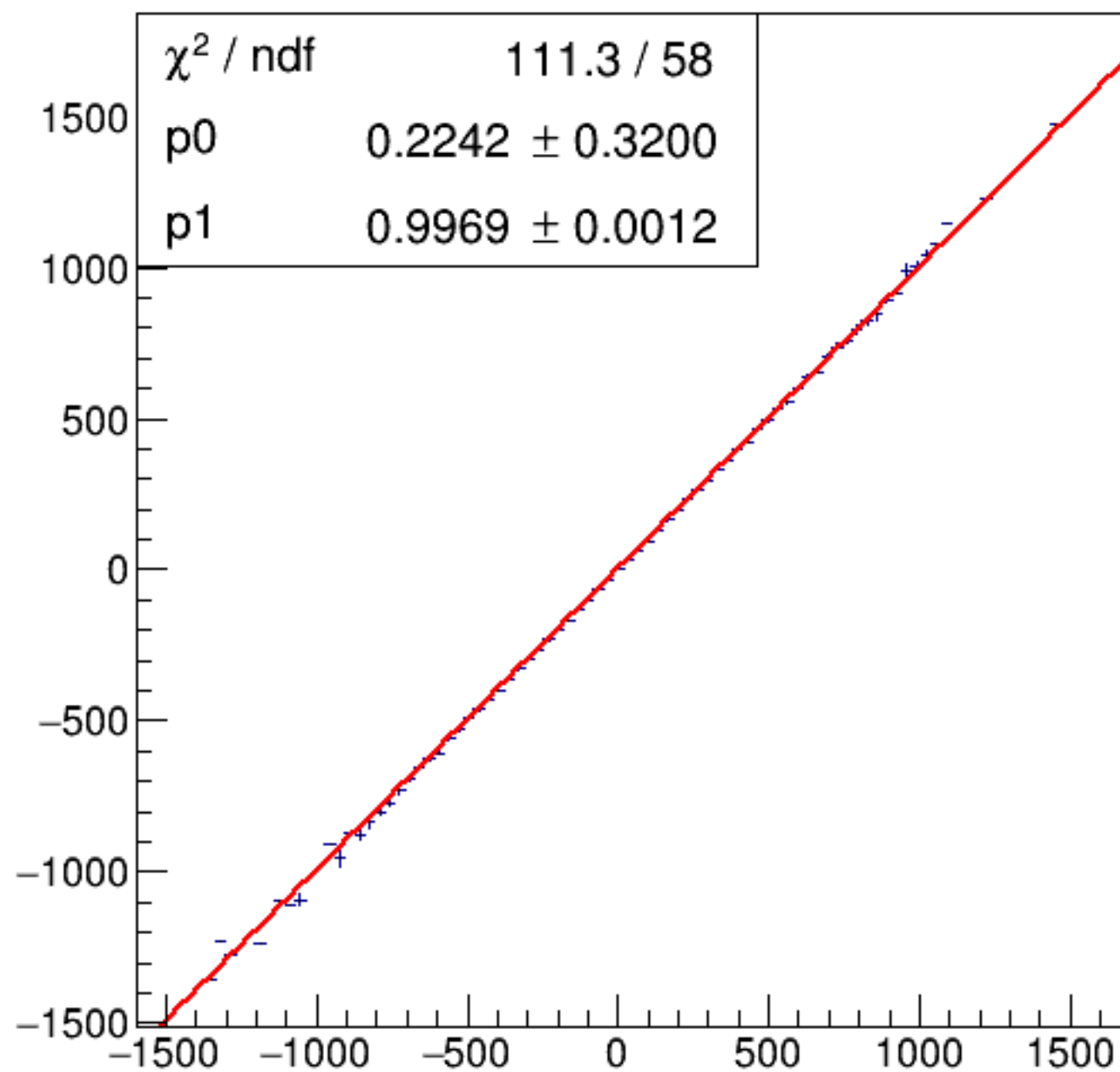
run7292_000_asym_bcm_dg_us_vs_asym_bcm_an_ds_mul.png
