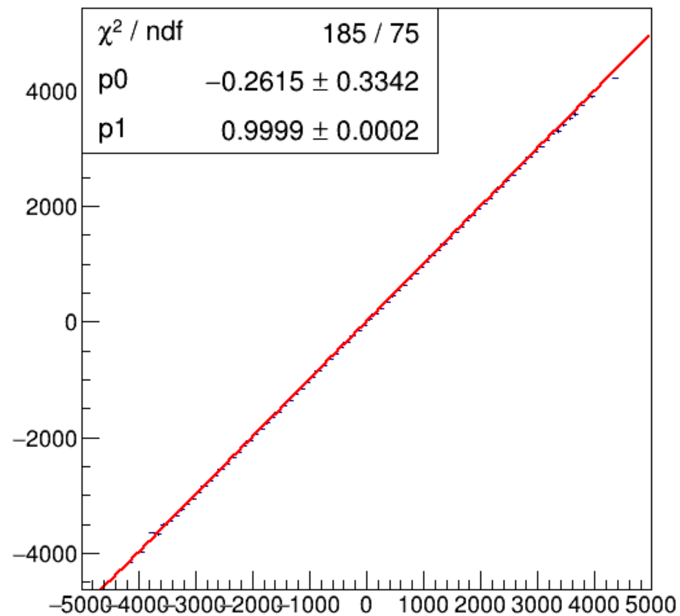
run7292_000_asym_bcm_dg_us_vs_asym_bcm_an_ds3_pr.png
