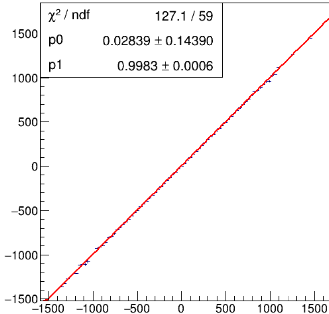
run7292_000_asym_bcm_an_us_vs_asym_bcm_an_ds3_mul.png
