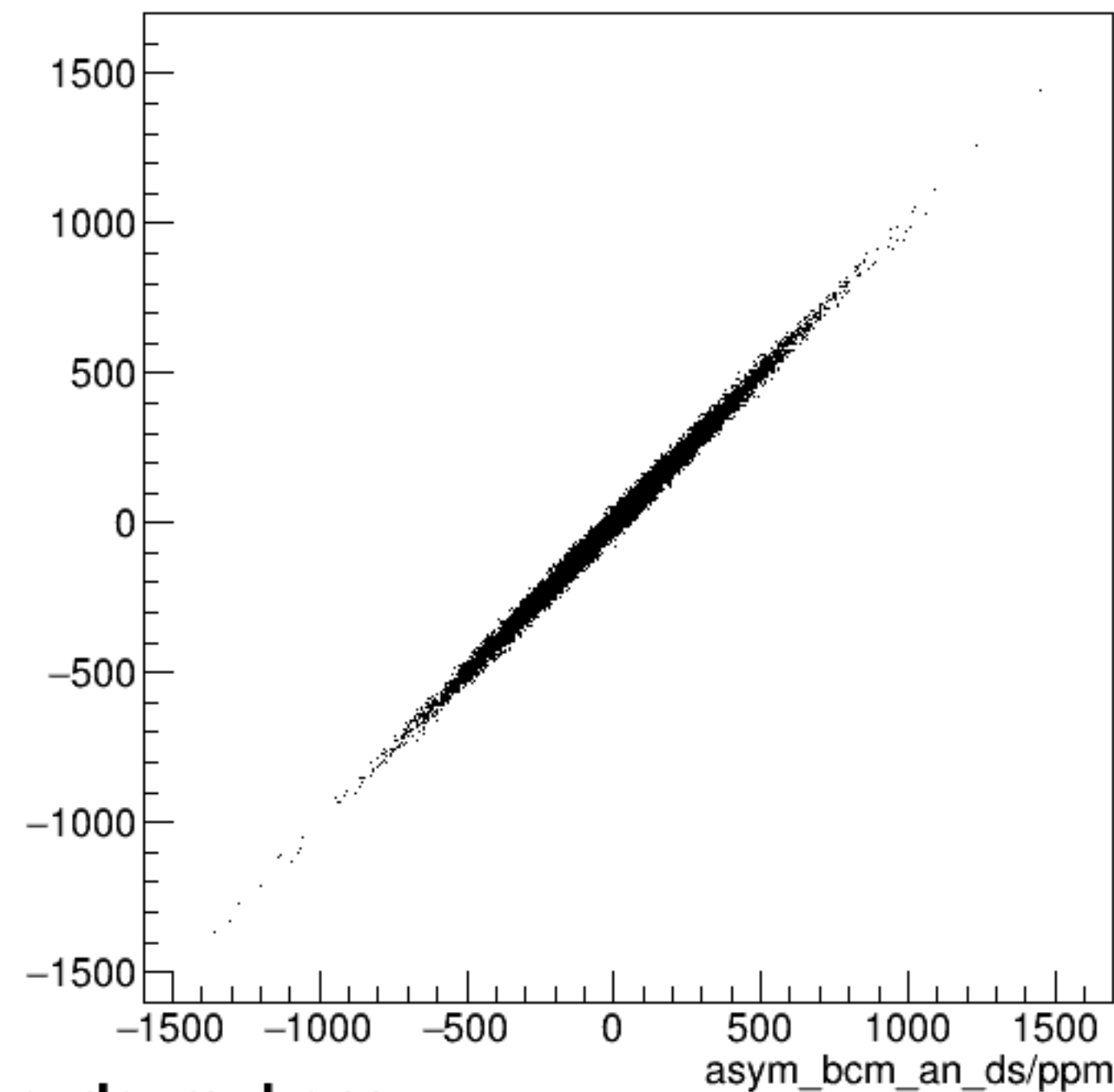
run7292_000_asym_bcm_an_us_vs_asym_bcm_an_ds_mul.png
