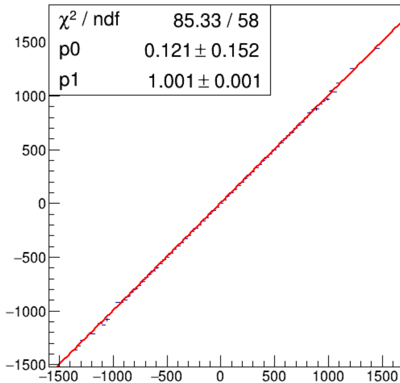
run7292_000_asym_bcm_an_us_vs_asym_bcm_an_ds_mul.png
