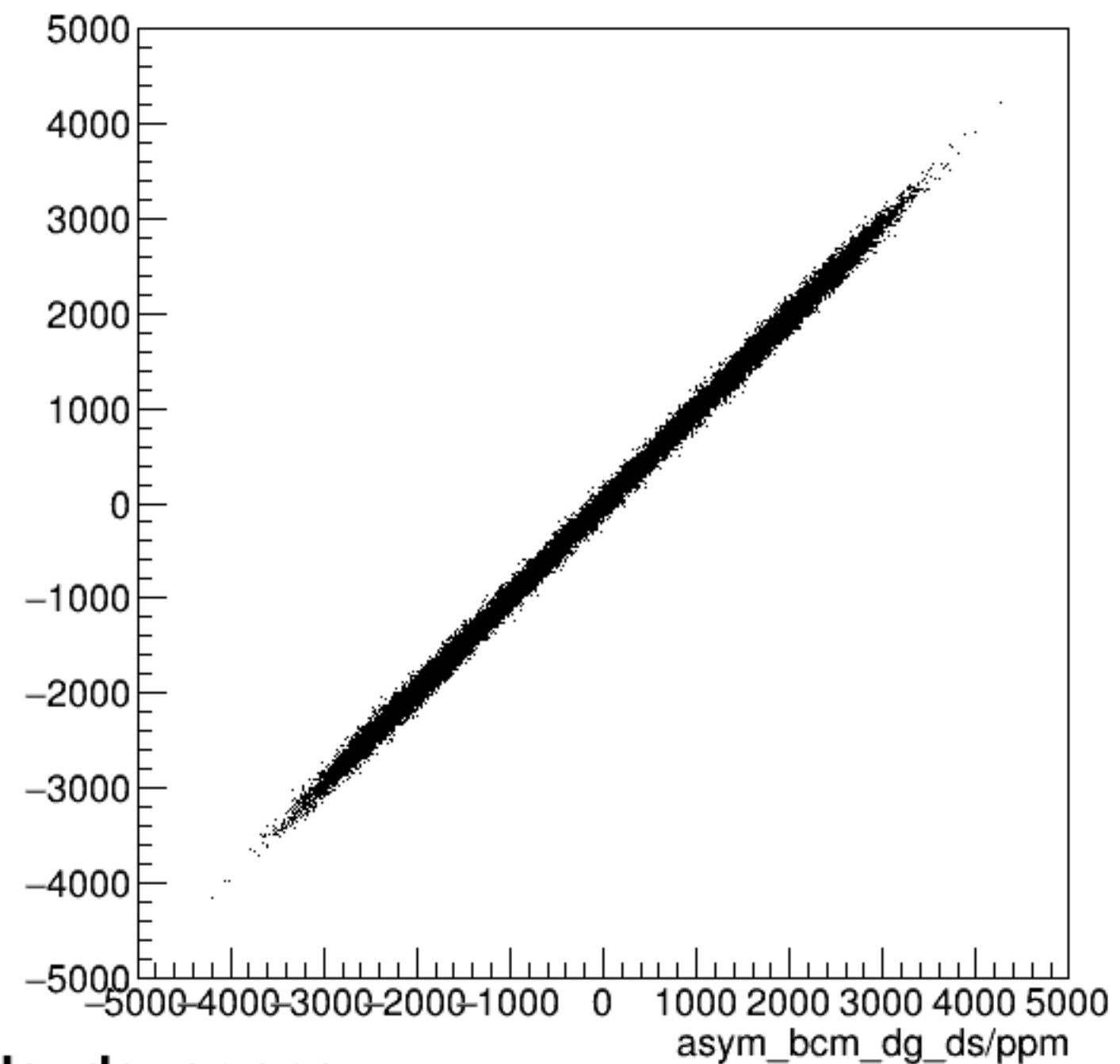
run7292_000_asym_bcm_dg_us_vs_asym_bcm_dg_ds_pr.png
