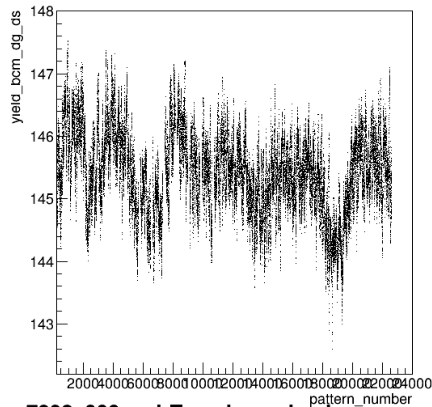
yield_bcm_dg_ds:pattern_number {ErrorFlag==0}
