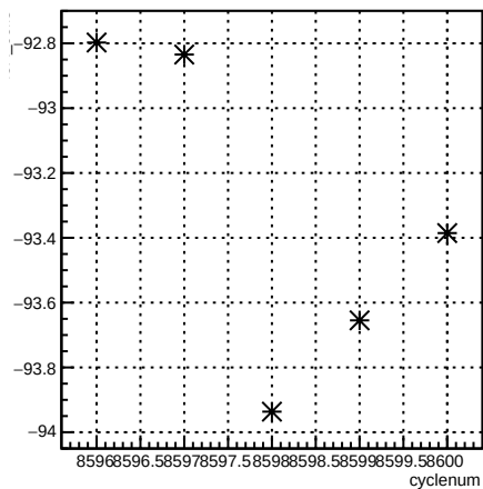
4eX_coil3:cyclenum {run == 7293}
