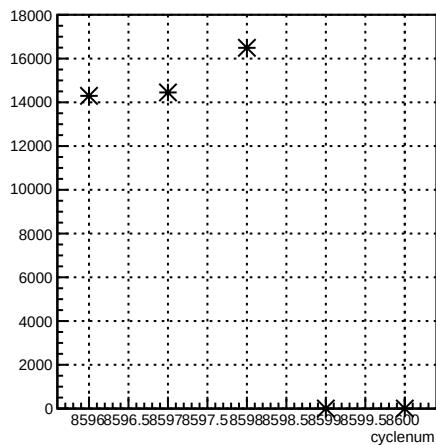
usl_coil7:cyclenum {run == 7293}
