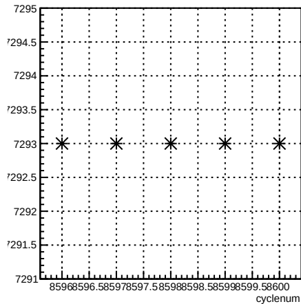
run:cyclenum {run == 7293}
