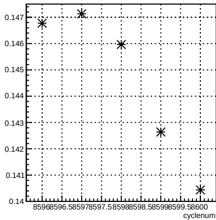
delta46_12X4eY:cyclenum {run == 7293}
