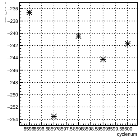
12X_coil1:cyclenum {run == 7293}
