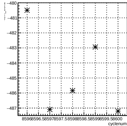
4eX_coil1:cyclenum {run == 7293}
