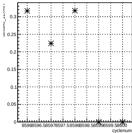
delta46_12X4eY:cyclenum {run == 7293}
