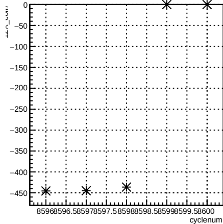
12X_coil7:cyclenum {run == 7293}
