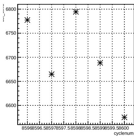
usl_coil3:cyclenum {run == 7293}
