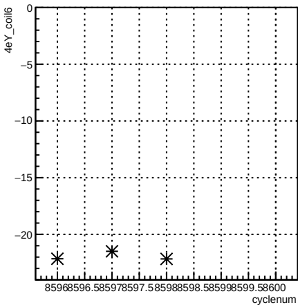
4eY_coil6:cyclenum {run == 7293}
