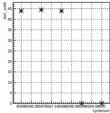
4aY_coil6:cyclenum {run == 7293}
