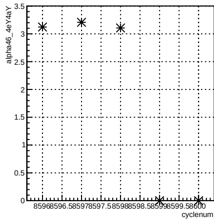
alpha46_4eY4aY:cyclenum {run == 7293}
