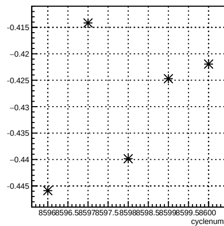
delta13_12X4eX:cyclenum {run == 7293}
