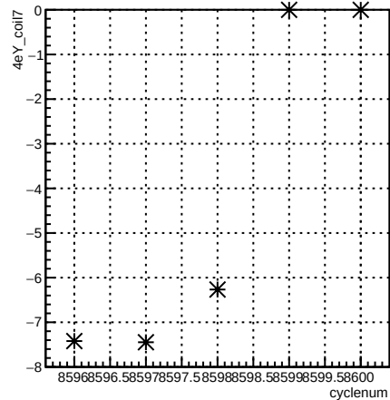
4eY_coil7:cyclenum {run == 7293}
