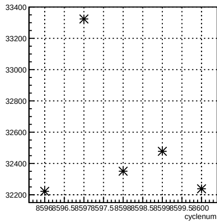
usl_coil1:cyclenum {run == 7293}
