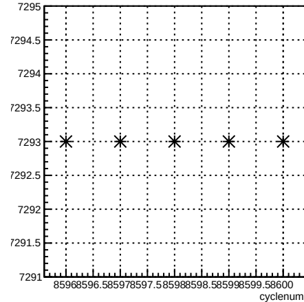
run:cyclenum {run == 7293}
