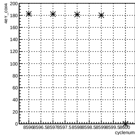
4eY_coil4:cyclenum {run == 7293}
