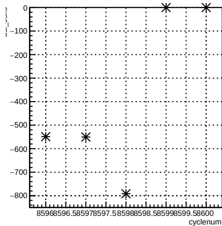
usl_coil6:cyclenum {run == 7293}
