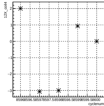
12X_coil4:cyclenum {run == 7293}
