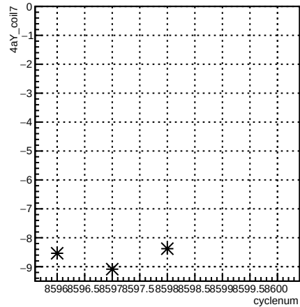
4aY_coil7:cyclenum {run == 7293}
