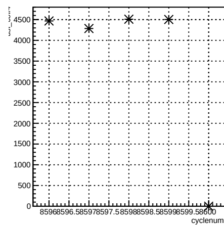
usl_coil4:cyclenum {run == 7293}
