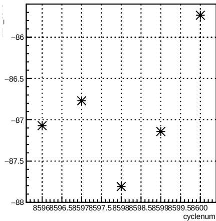
12X_coil3:cyclenum {run == 7293}
