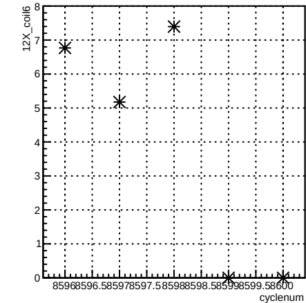
12X_coil6:cyclenum {run == 7293}
