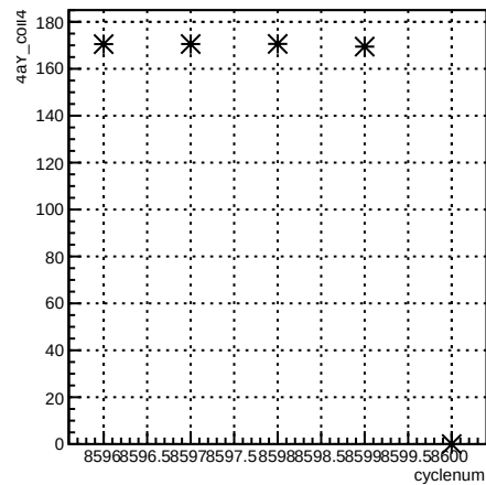
4aY_coil4:cyclenum {run == 7293}
