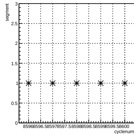
segment:cyclenum {run == 7293}
