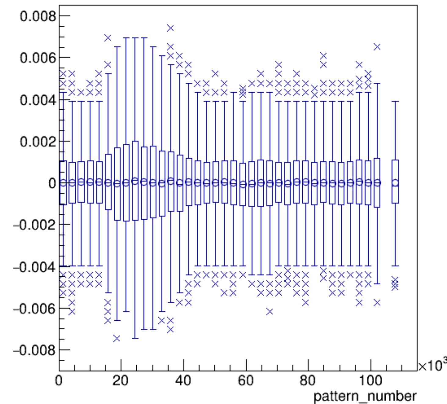
asym_bcm_an_diff*yield_bcm_an_diff:pattern_number {ErrorFlag==0}
