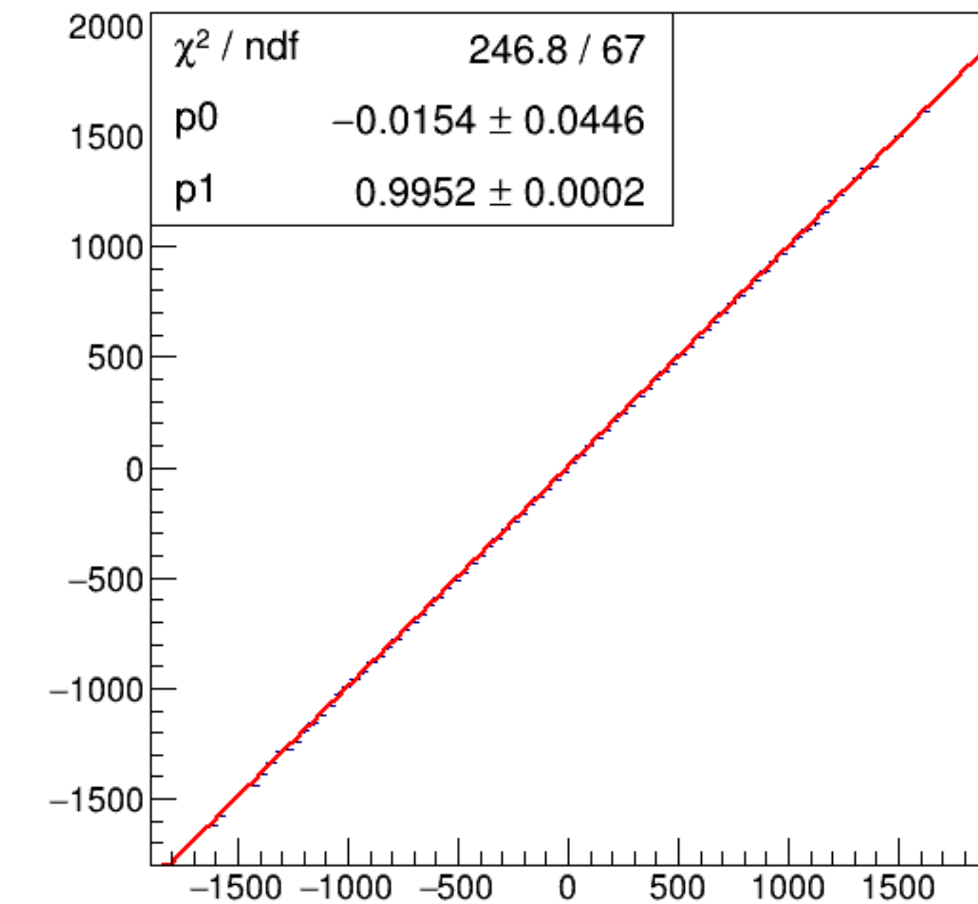
run7293_000_asym_bcm_an_ds_vs_asym_bcm_an_ds3_mul.png
