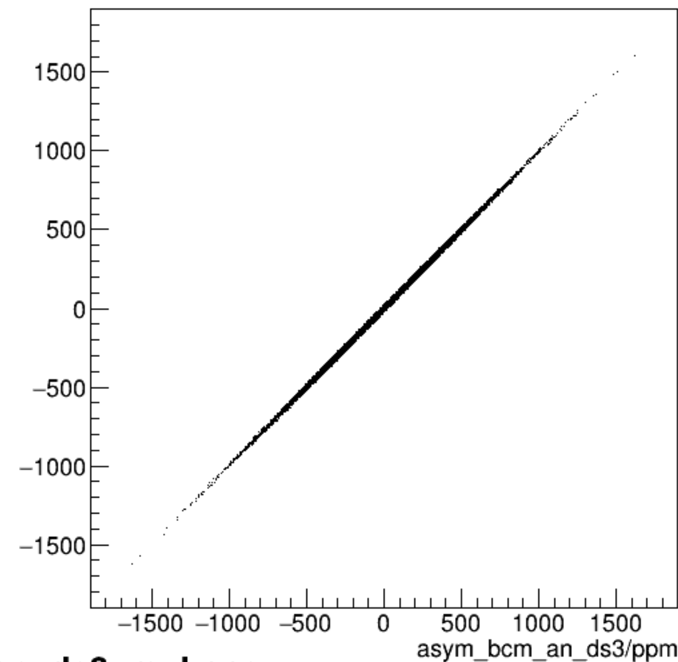
run7293_000_asym_bcm_an_ds_vs_asym_bcm_an_ds3_mul.png
