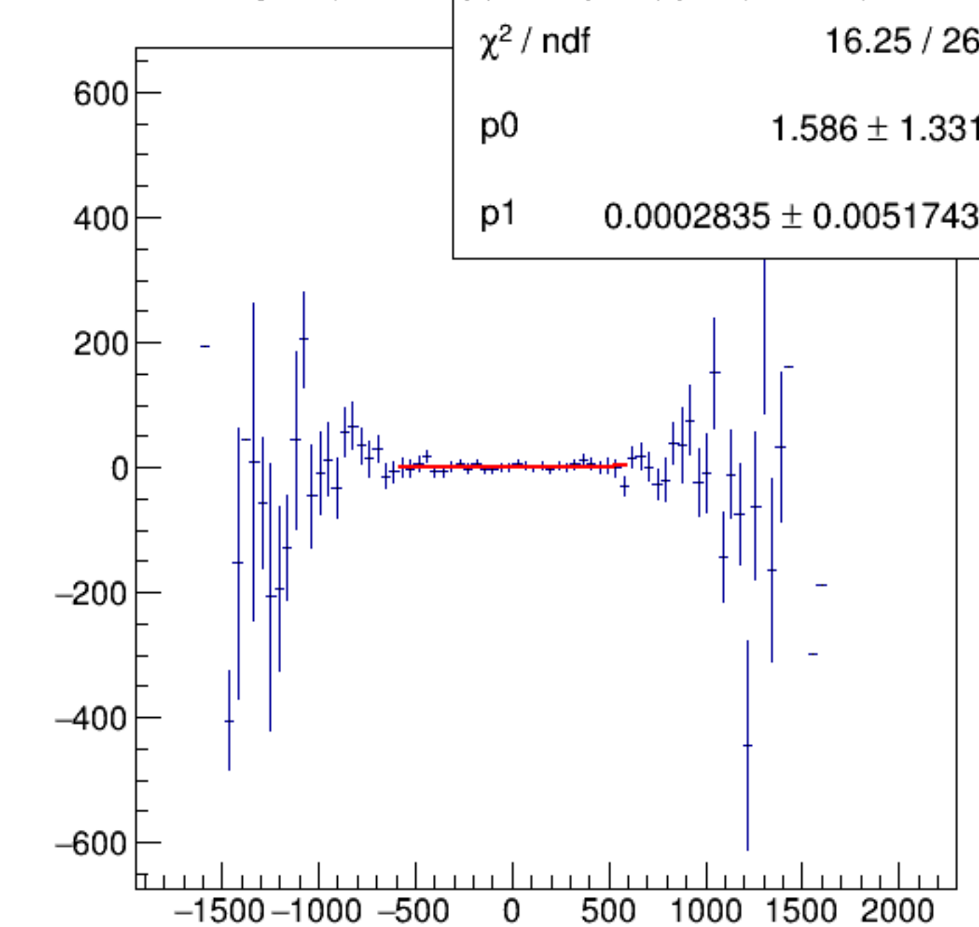
reg_asym_dsr/ppm:AqUS/ppm {ok_cut}
