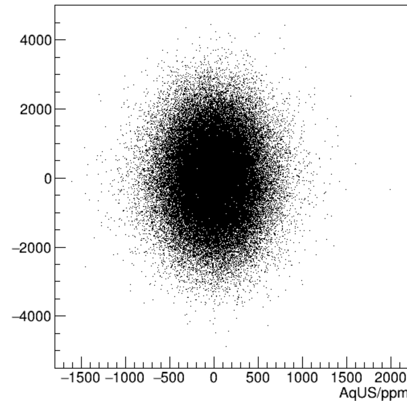
reg_asym_usr/ppm:AqUS/ppm {ok_cut}
