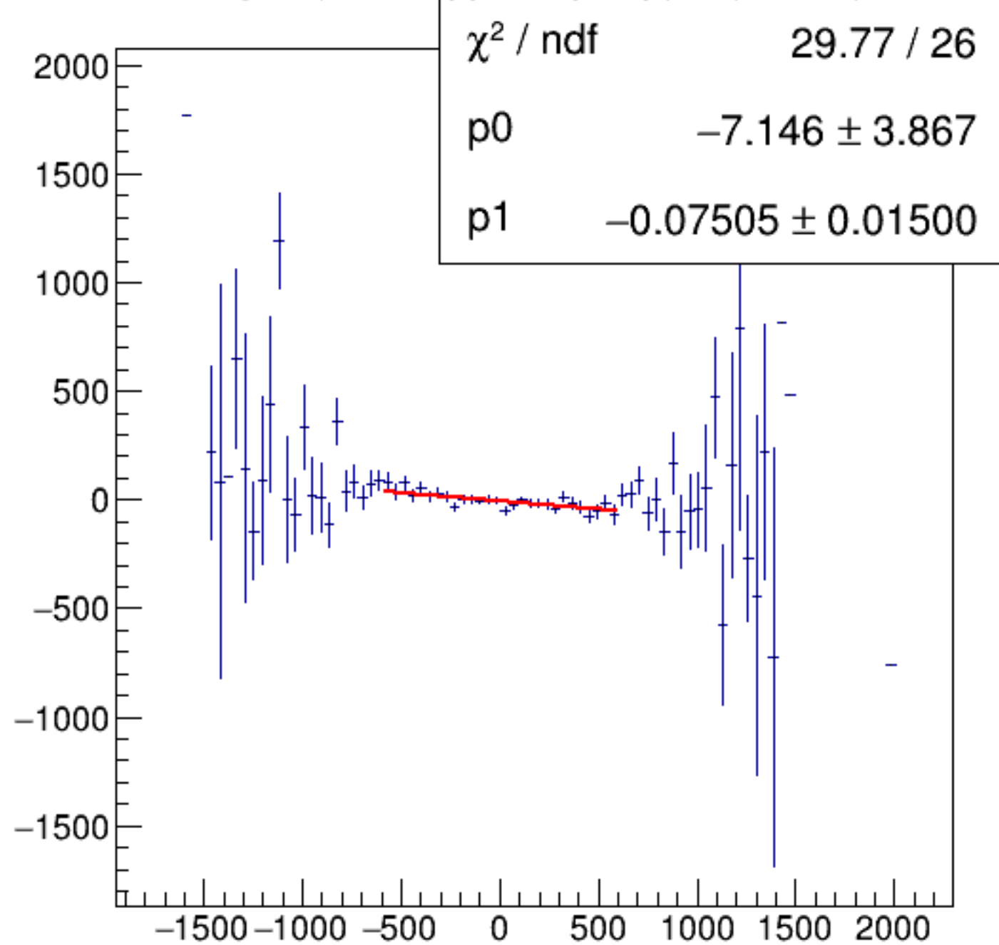
reg_asym_usl/ppm:AqUS/ppm {ok_cut}
