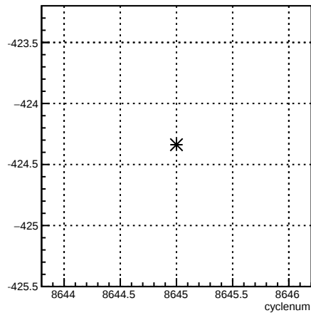
4eX_coil1:cyclenum {run == 7307}
