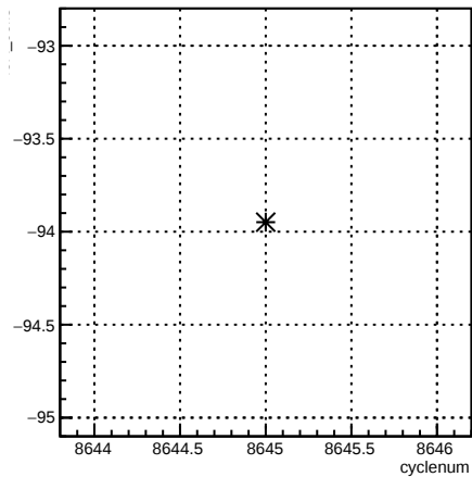
4eX_coil3:cyclenum {run == 7307}
