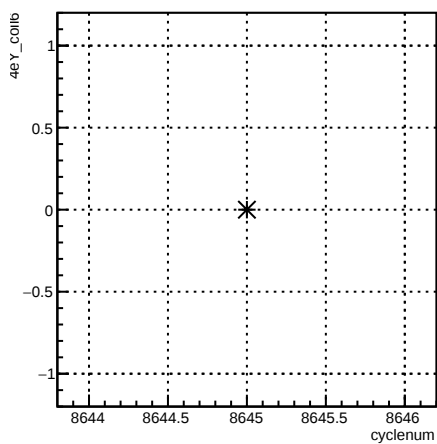
4eY_coil6:cyclenum {run == 7307}
