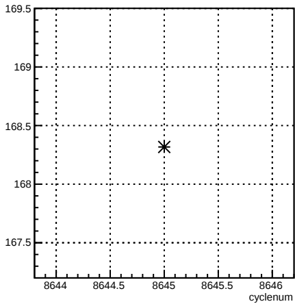
4aY_coil4:cyclenum {run == 7307}
