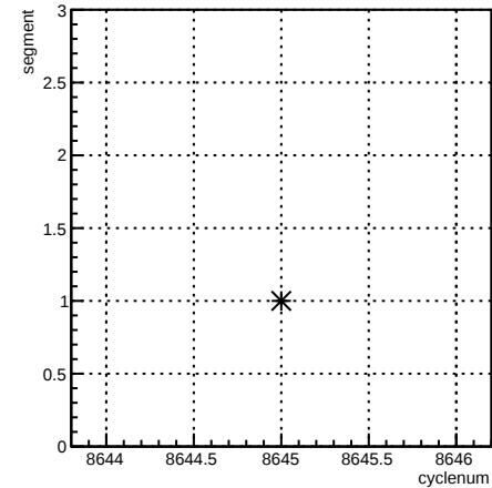
segment:cyclenum {run == 7307}
