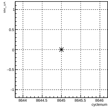
usl_4eY:cyclenum {run == 7307}
