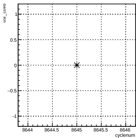
usr_coil6:cyclenum {run == 7307}
