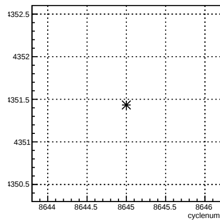
usl_coil4:cyclenum {run == 7307}
