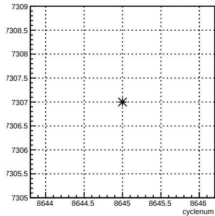
run:cyclenum {run == 7307}
