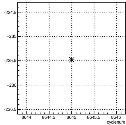
12X_coil6:cyclenum {run == 7307}
