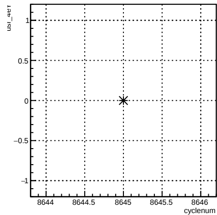
usr_4eY:cyclenum {run == 7307}
