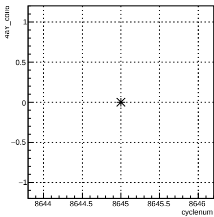
4aY_coil6:cyclenum {run == 7307}
