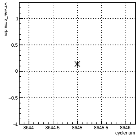
alpha13_4eX1X:cyclenum {run == 7307}
