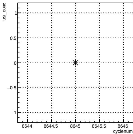
usl_coil6:cyclenum {run == 7307}
