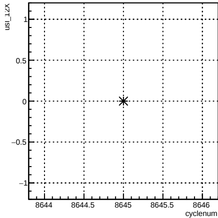
usl_12X:cyclenum {run == 7307}
