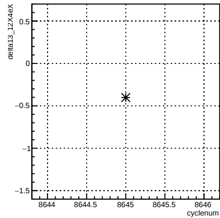
delta13_12X4eX:cyclenum {run == 7307}
