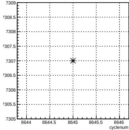
run:cyclenum {run == 7307}
