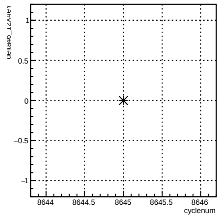
delta46_12X4eY:cyclenum {run == 7307}
