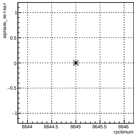
alpha46_4eY4aY:cyclenum {run == 7307}
