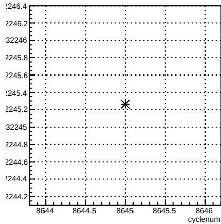
usl_coil1:cyclenum {run == 7307}
