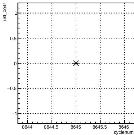
usl_coil7:cyclenum {run == 7307}
