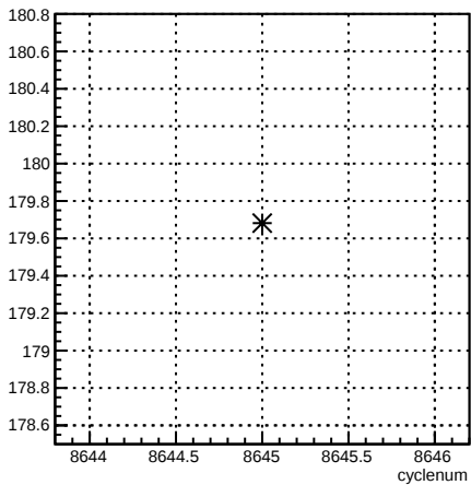
4eY_coil4:cyclenum {run == 7307}
