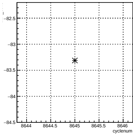
12X_coil7:cyclenum {run == 7307}
