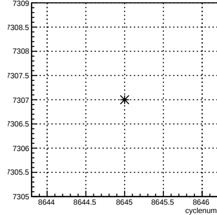
run:cyclenum {run == 7307}
