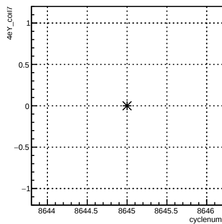
4eY_coil7:cyclenum {run == 7307}
