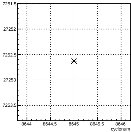
usr_coil1:cyclenum {run == 7307}
