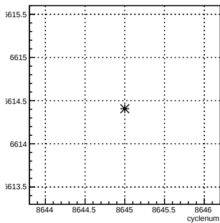
usl_coil3:cyclenum {run == 7307}
