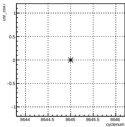
usr_coil7:cyclenum {run == 7307}
