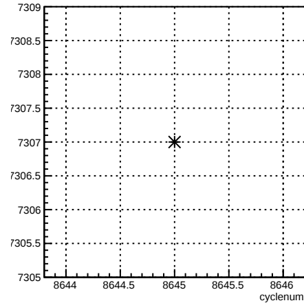
run:cyclenum {run == 7307}
