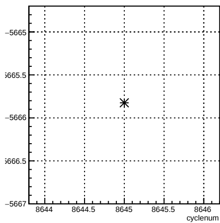
usr_coil3:cyclenum {run == 7307}
