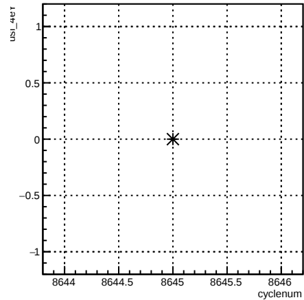
usl_4eY:cyclenum {run == 7307}
