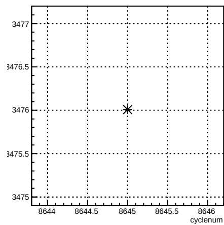
usr_coil4:cyclenum {run == 7307}
