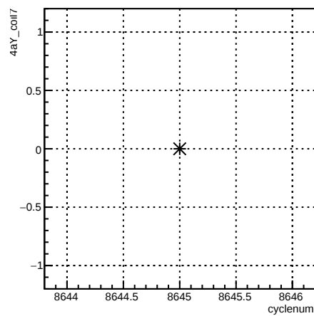
4aY_coil7:cyclenum {run == 7307}
