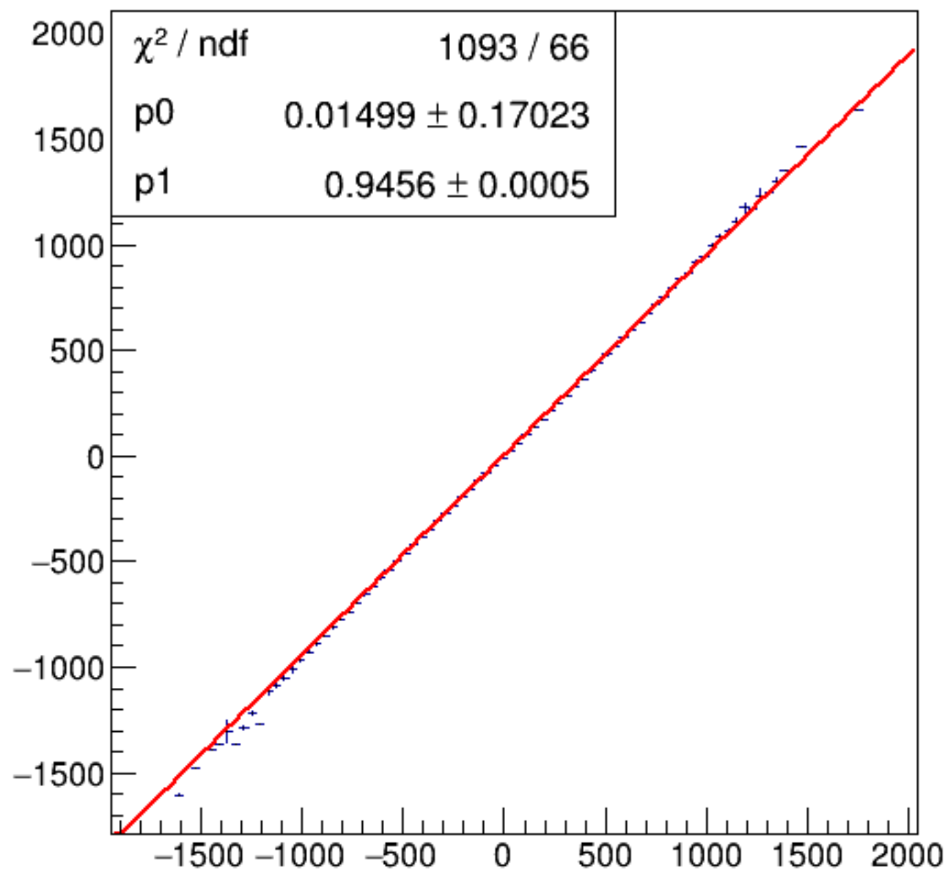
run7314_000_asym_bcm_dg_ds_vs_asym_bcm_an_us_pr.png
