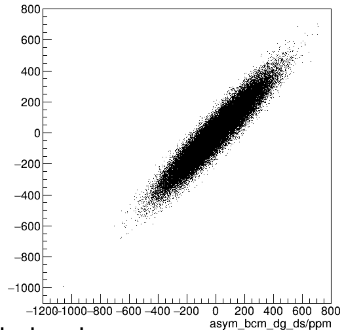
run7314_000_asym_bcm_dg_us_vs_asym_bcm_dg_ds_mul.png
