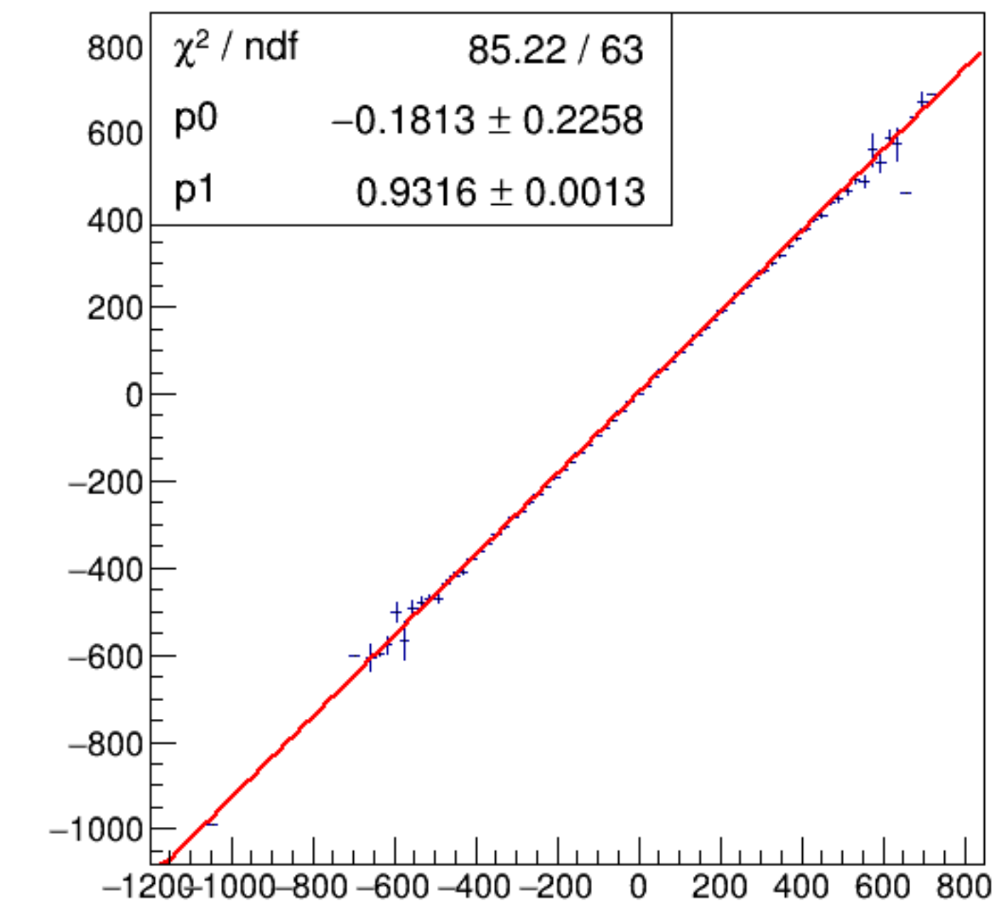
run7314_000_asym_bcm_dg_us_vs_asym_bcm_dg_ds_mul.png
