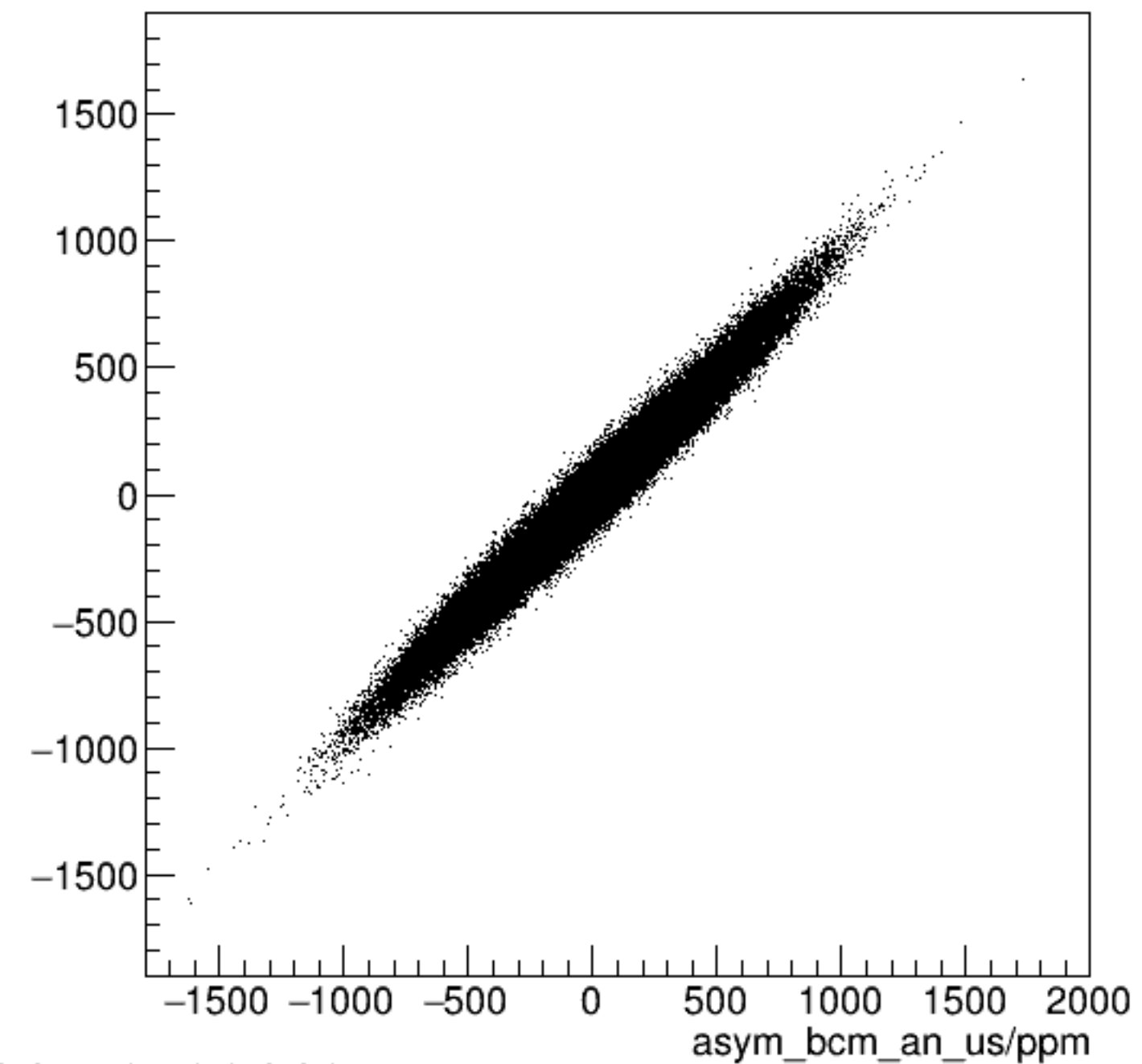
run7314_000_asym_bcm_dg_ds_vs_asym_bcm_an_us_pr.png
