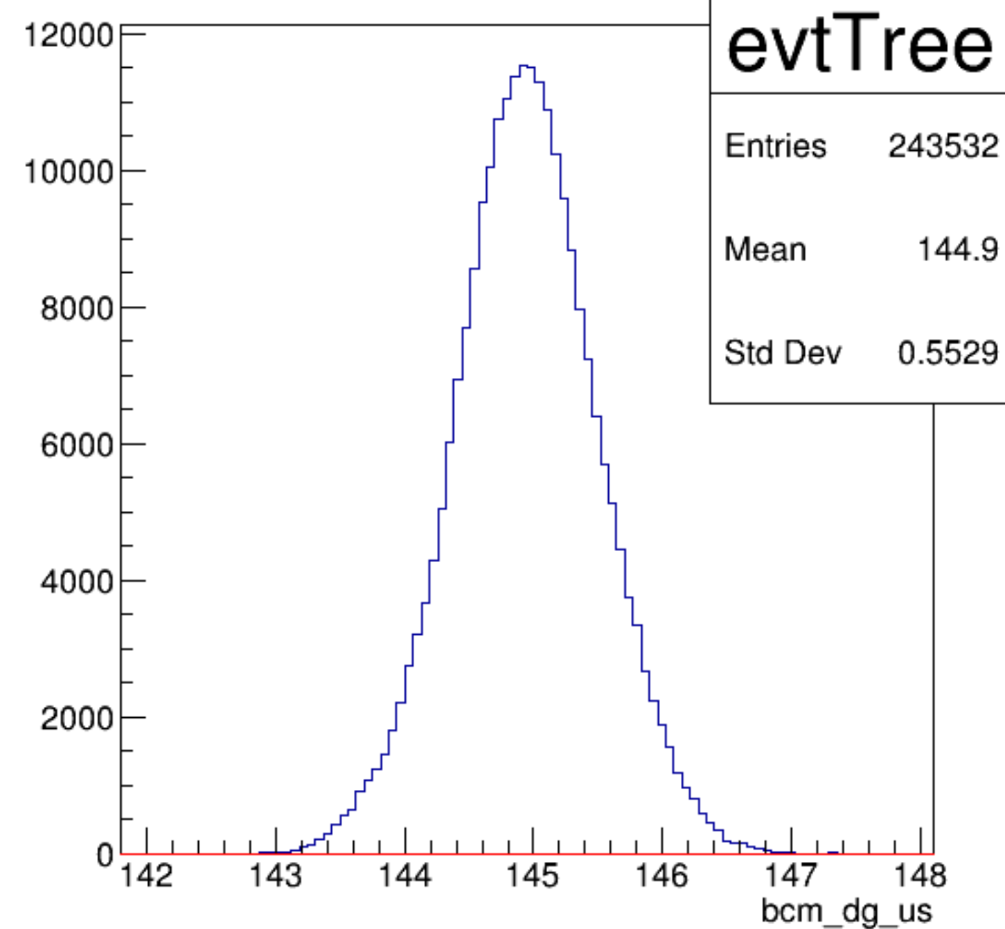
bcm_dg_us {ErrorFlag==0}
