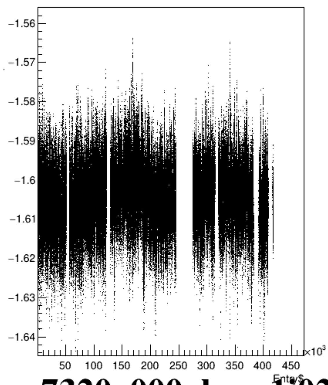
bpm1i02Y/mm:Entry$ {ErrorFlag==0}
