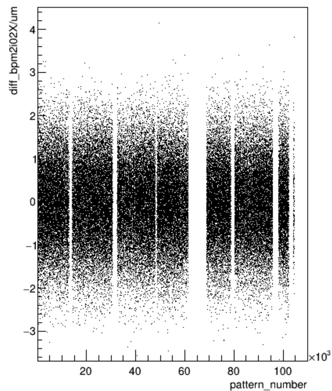
diff_bpm2i02X/um:pattern_number (ErrorFlag==0)
