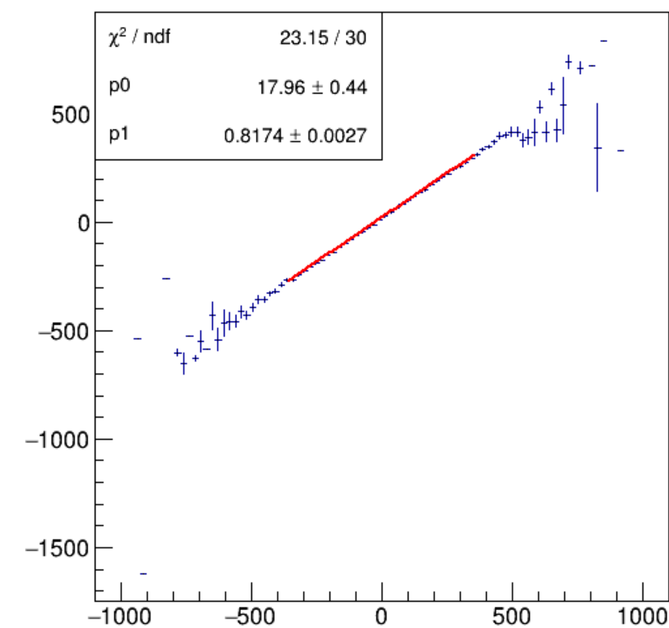
asym_bpm0i01aWS/ppm:Aq/ppm {ErrorFlag==0}
