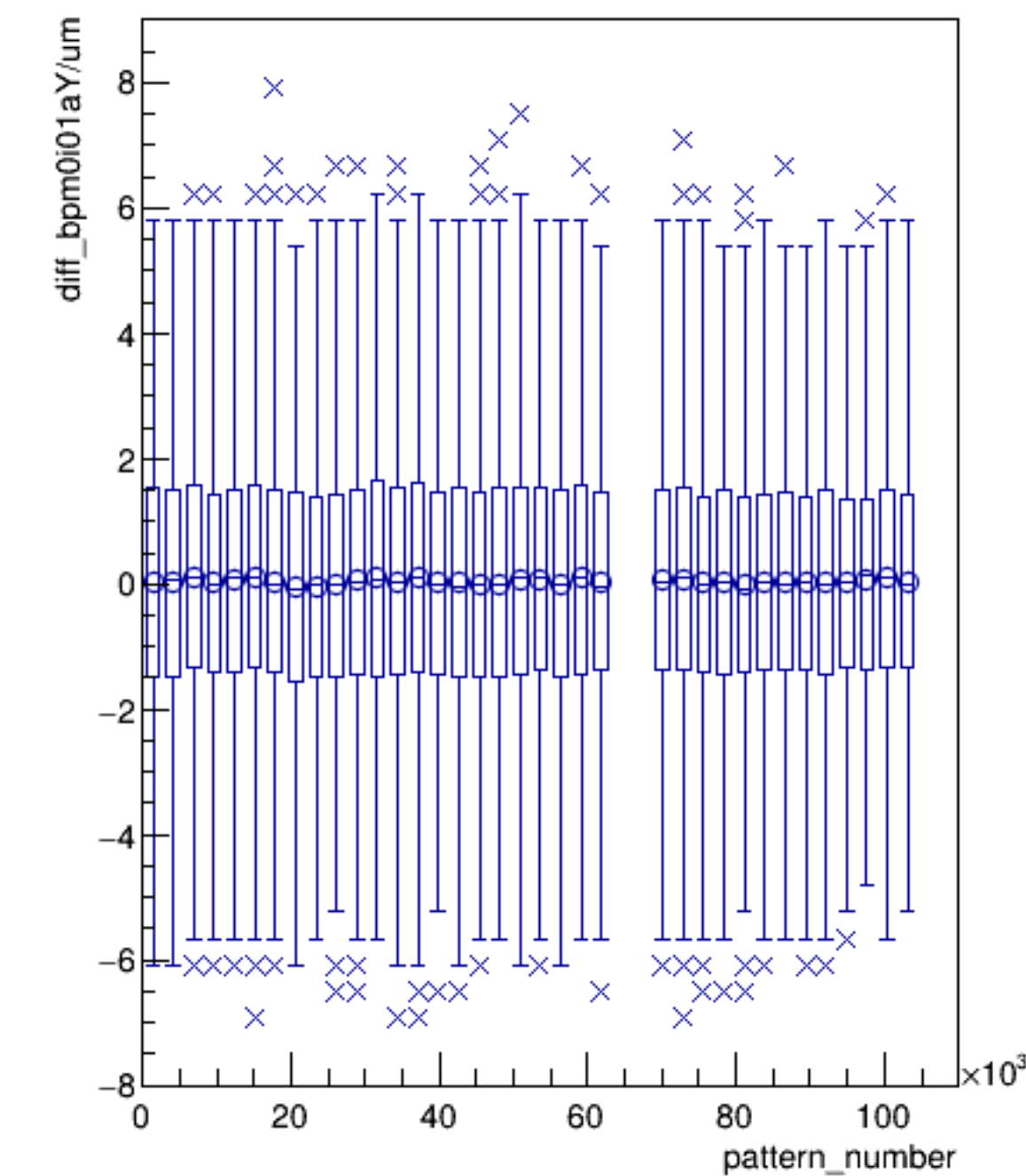
diff_bpm0i01aY/um:pattern_number (ErrorFlag==0)
