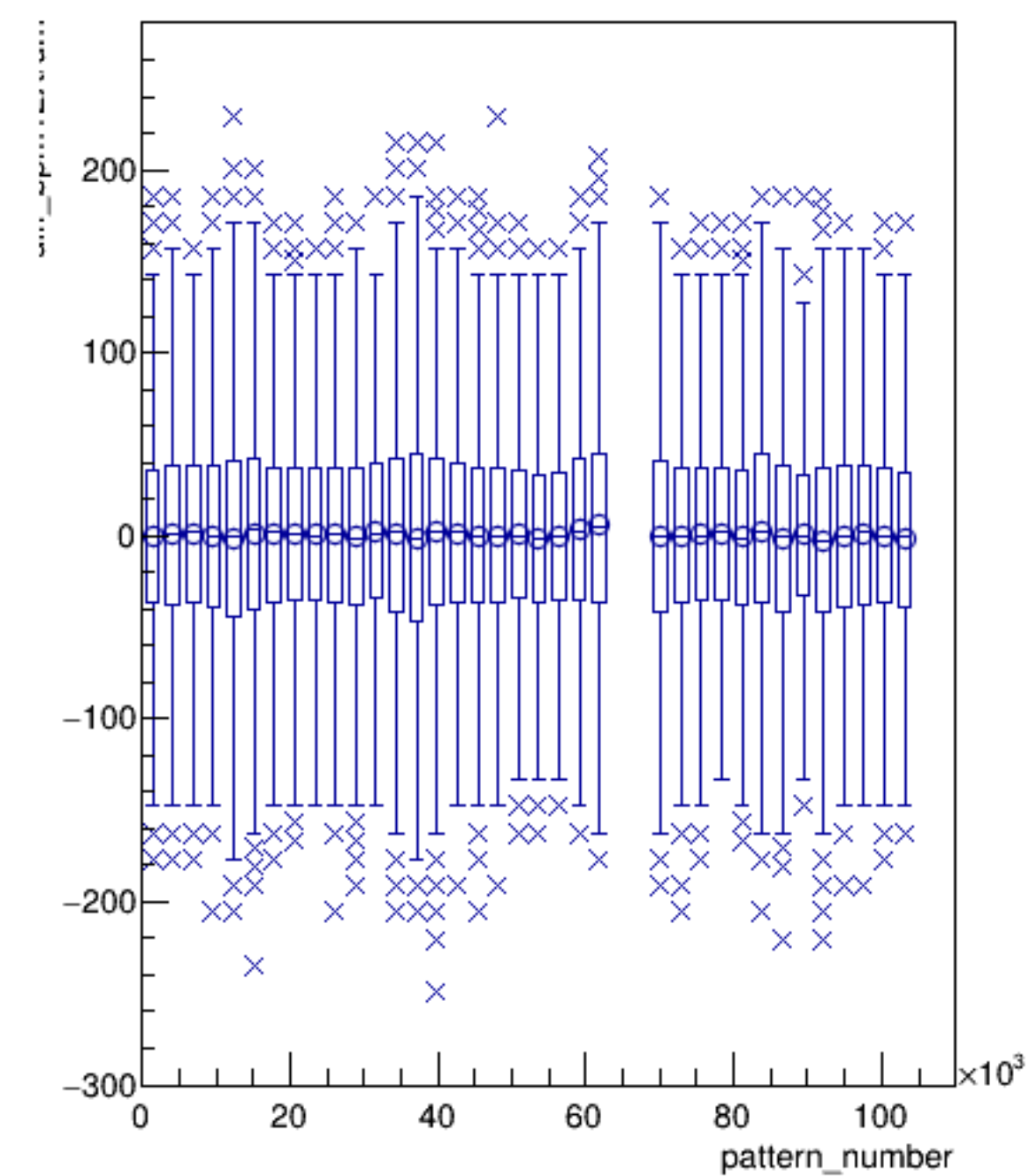
diff_bpm12X/um:pattern_number {ErrorFlag==0}
