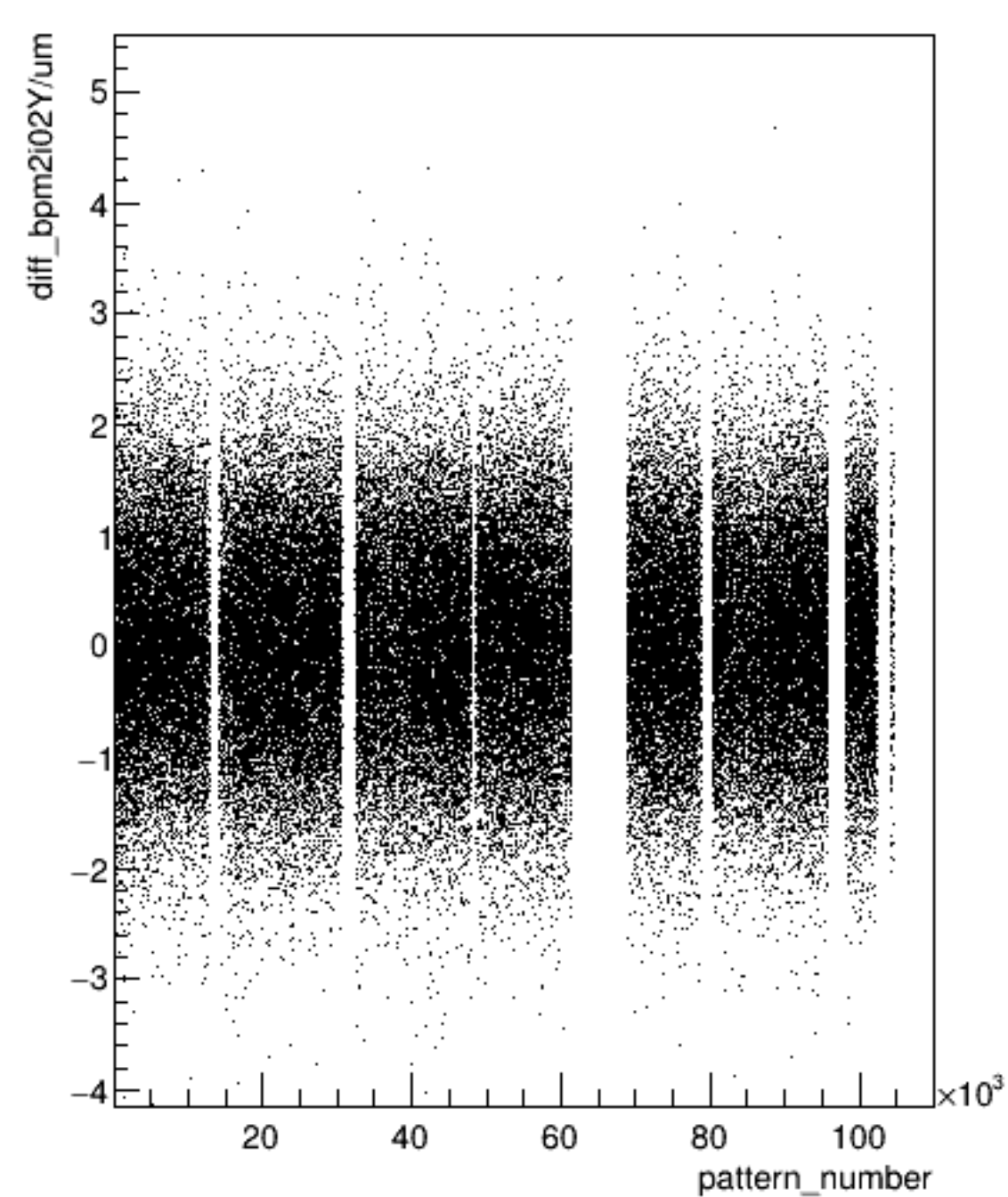
diff_bpm2i02Y/um:pattern_number (ErrorFlag==0)
