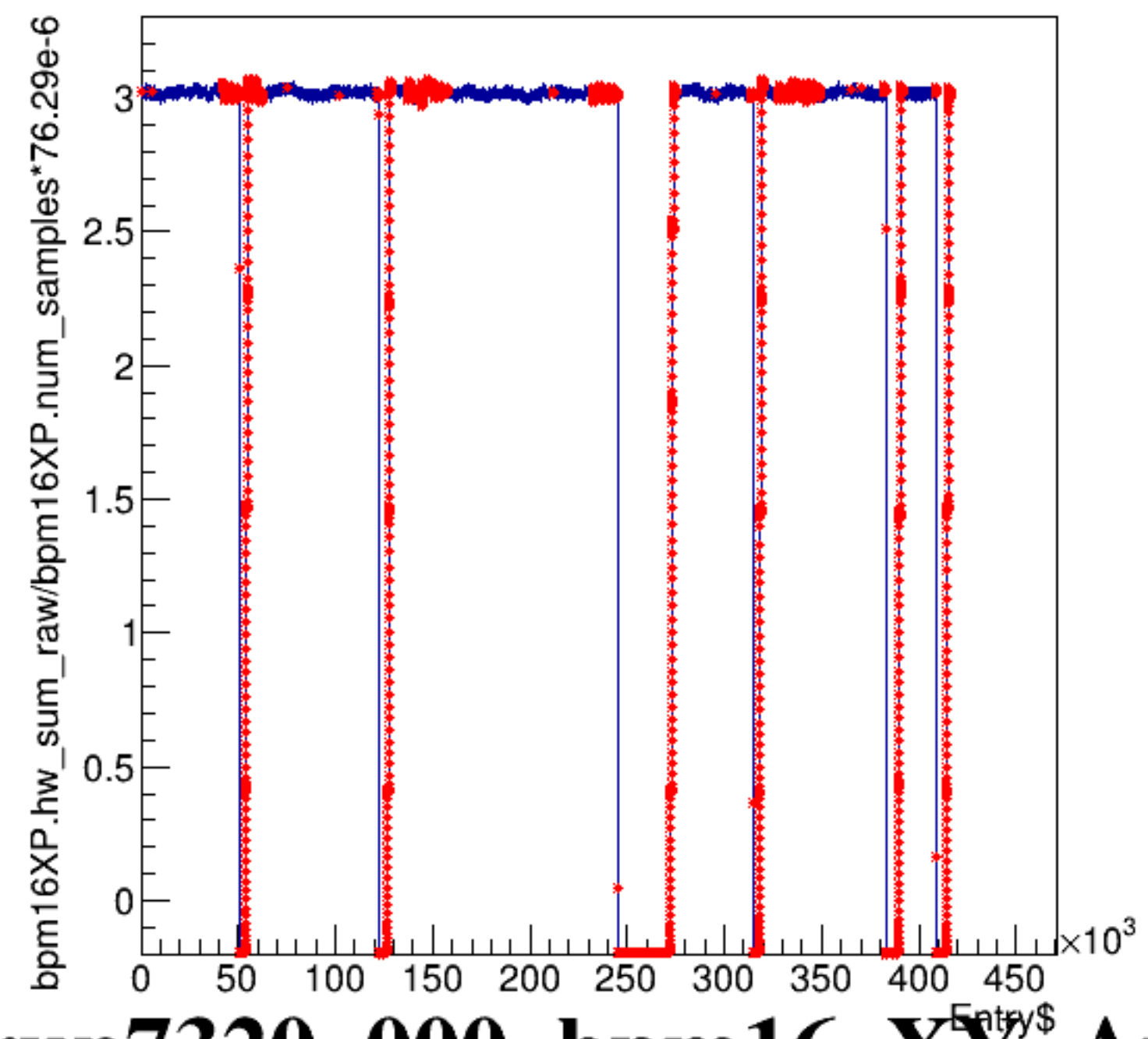
bpm16XP.hw_sum_raw/bpm16XP.num_samples*76.29e-6:Entry$
