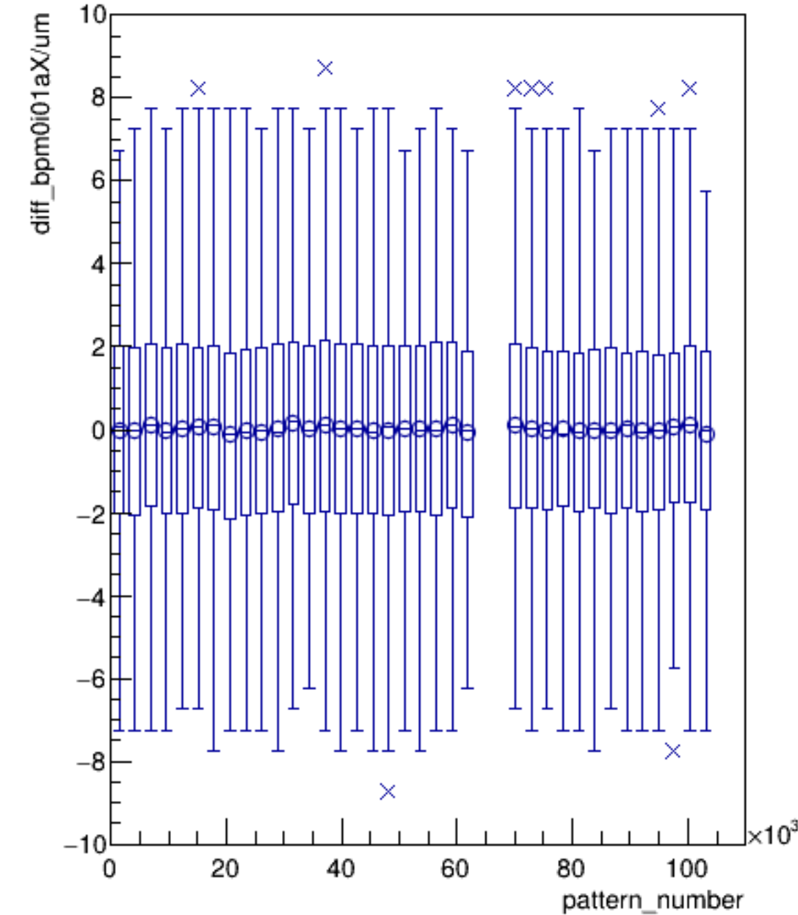
diff_bpm0i01aX/um:pattern_number (ErrorFlag==0)
