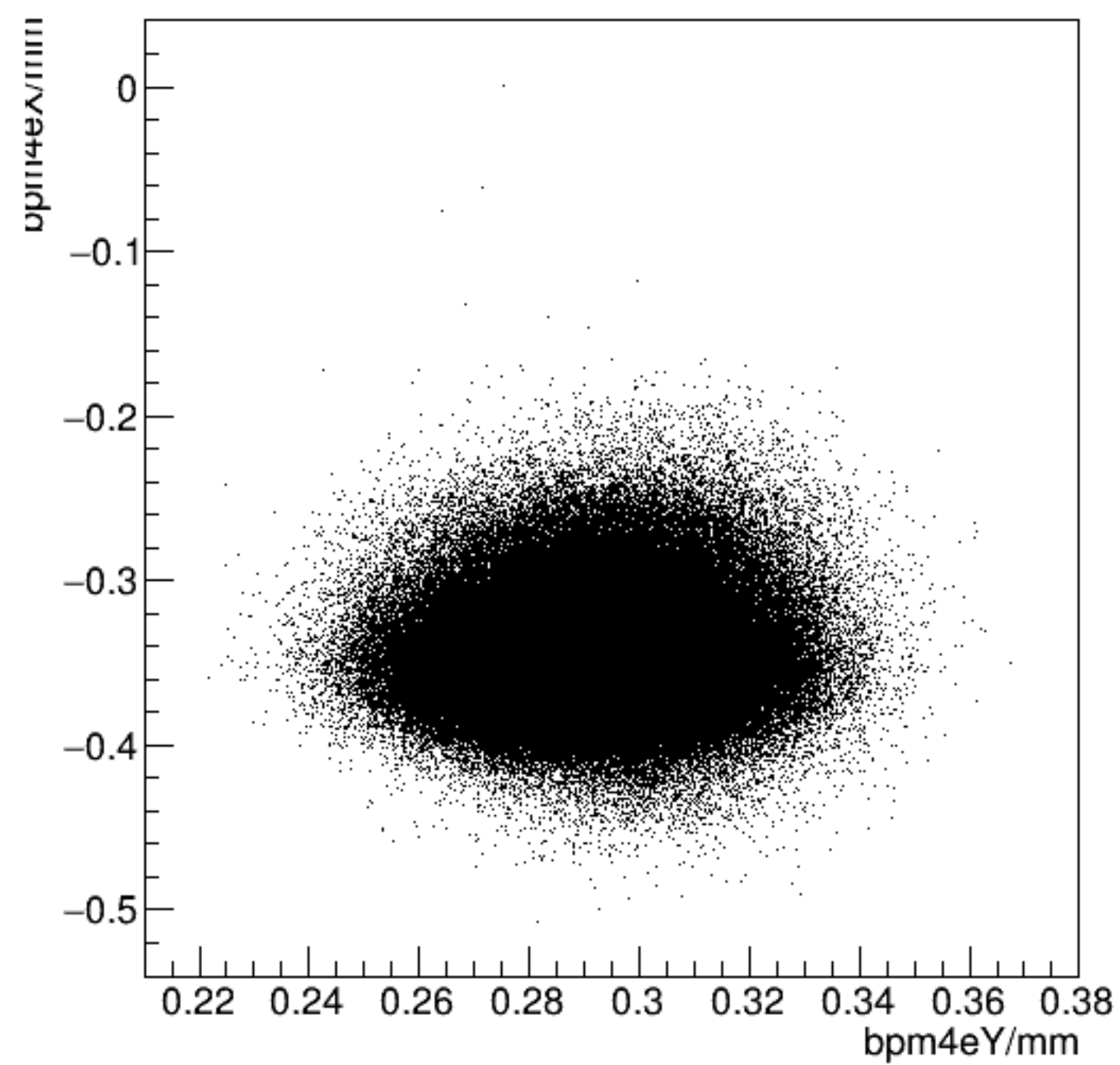
bpm4eX/mm:bpm4eY/mm {ErrorFlag==0}
