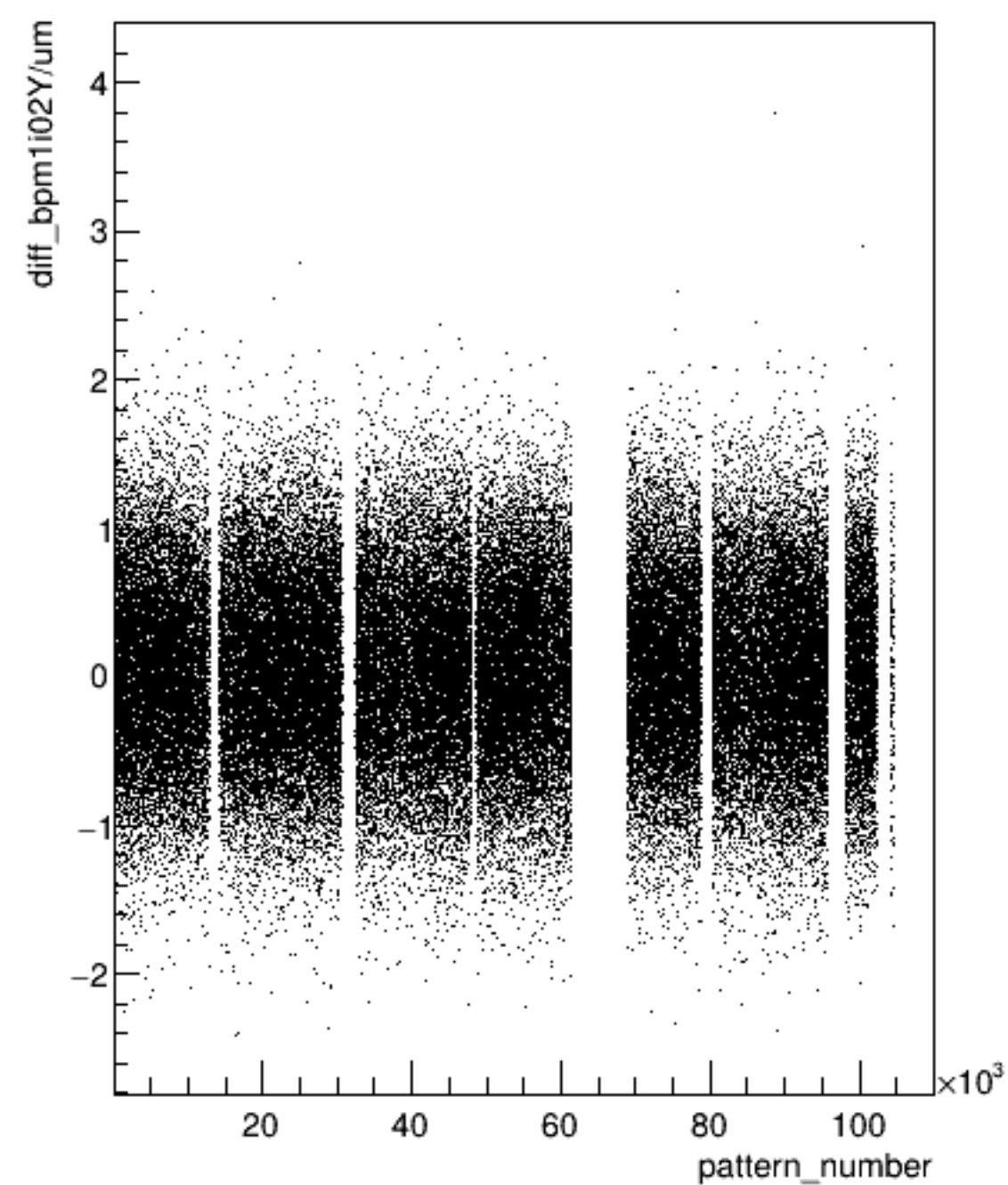
diff_bpm1i02Y/um:pattern_number (ErrorFlag==0)
