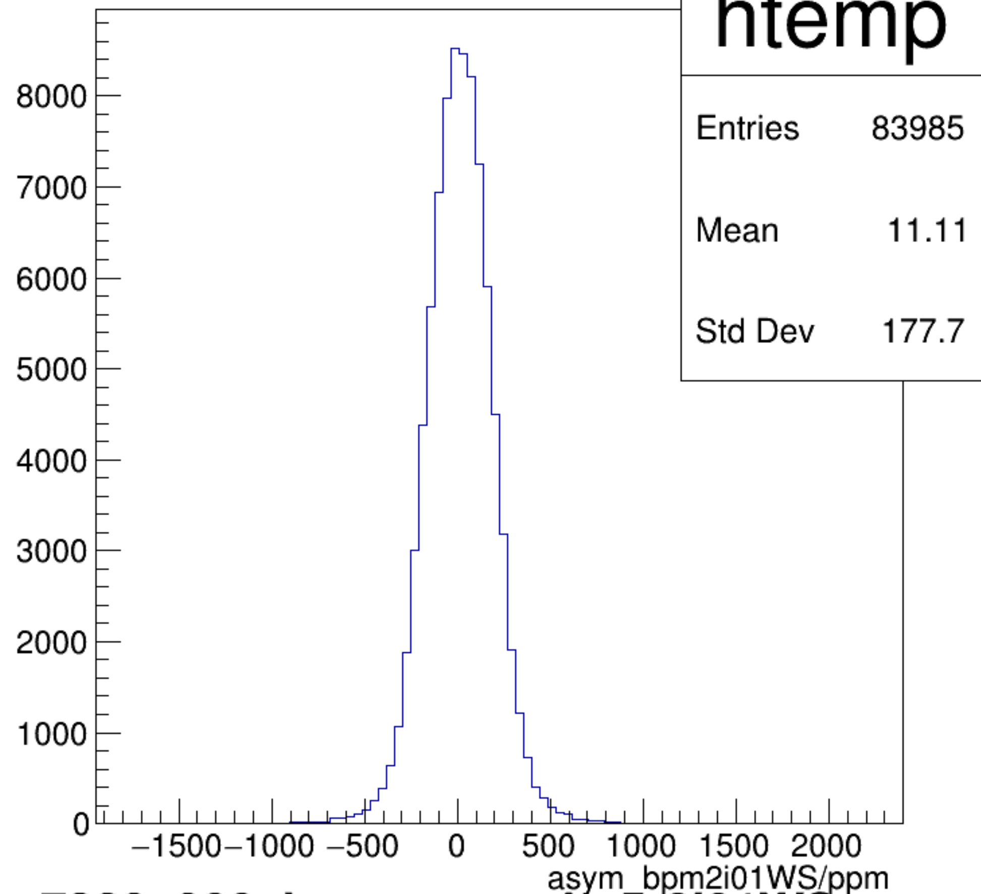
run7320_000_bpm_asym_bpm2i01WS.png
