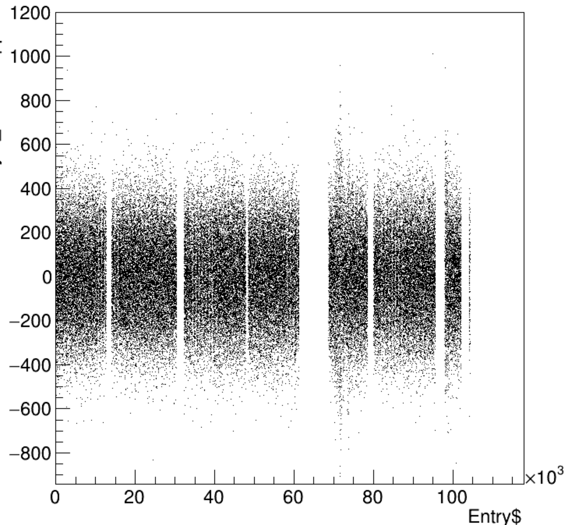
asym_bcm0l02/ppm:Entry$ {ErrorFlag==0}
