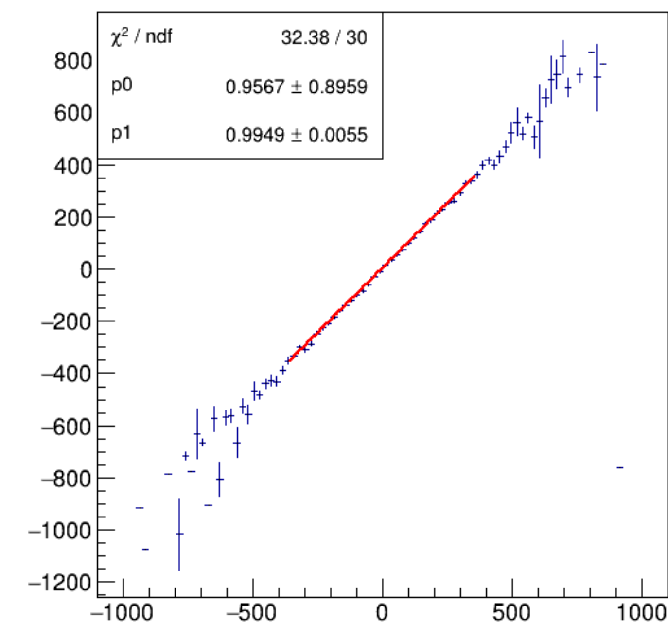
asym_bpm4ecWS/ppm:Aq/ppm {ErrorFlag==0}
