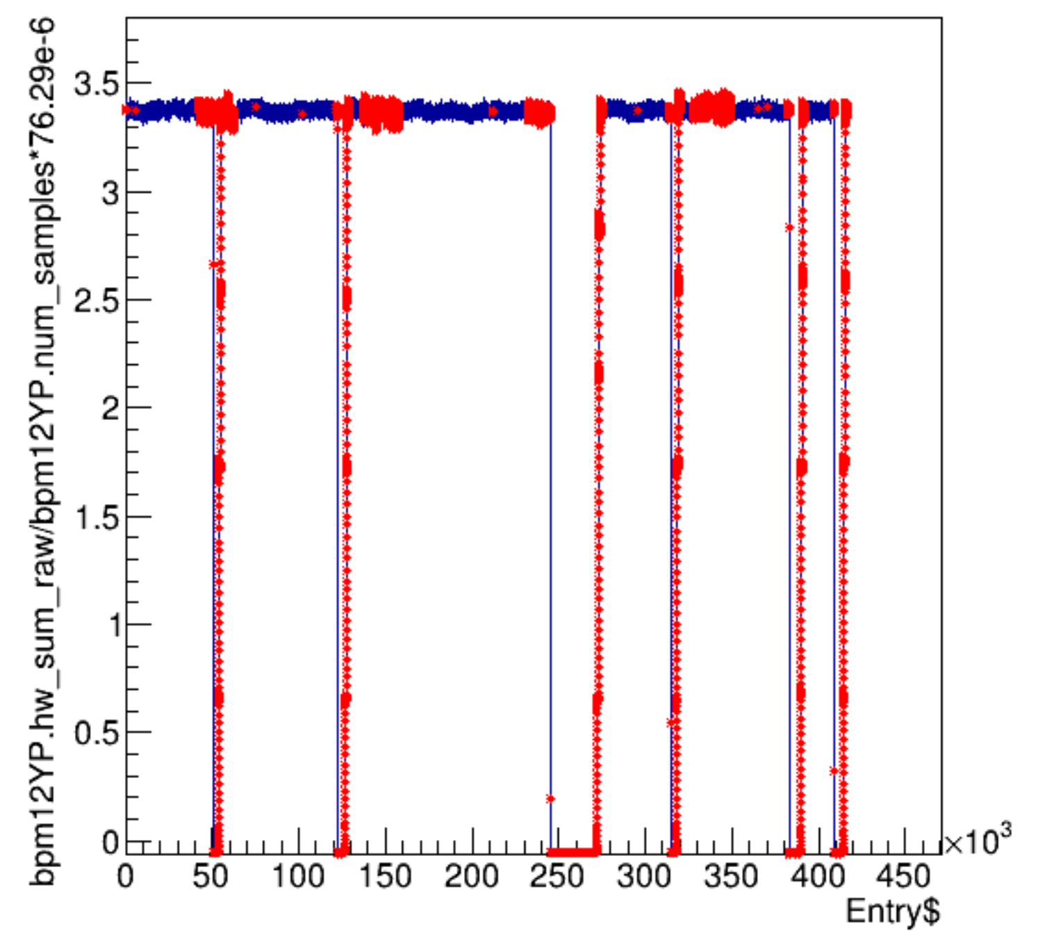
bpm12YP.hw_sum_raw/bpm12YP.num_samples*76.29e-6:Entry$
