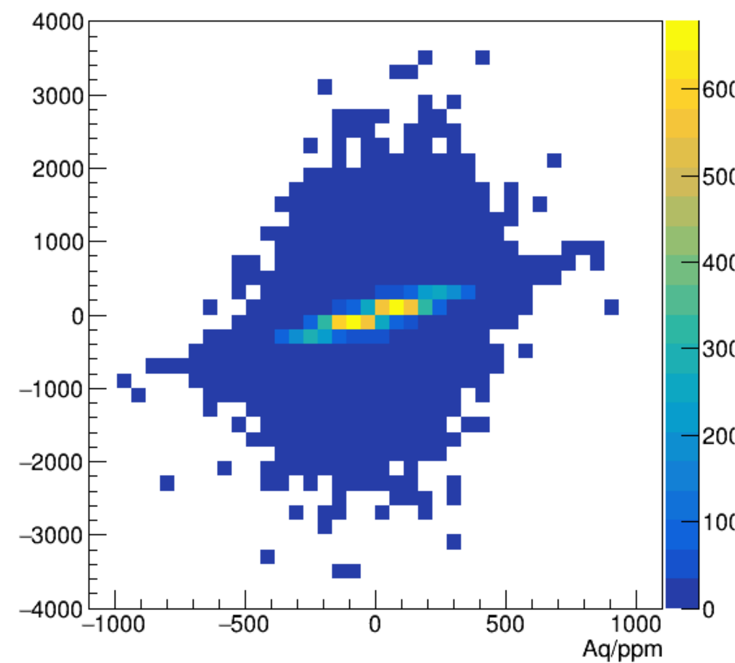
asym_bpm4acWS/ppm:Aq/ppm {ErrorFlag==0}
