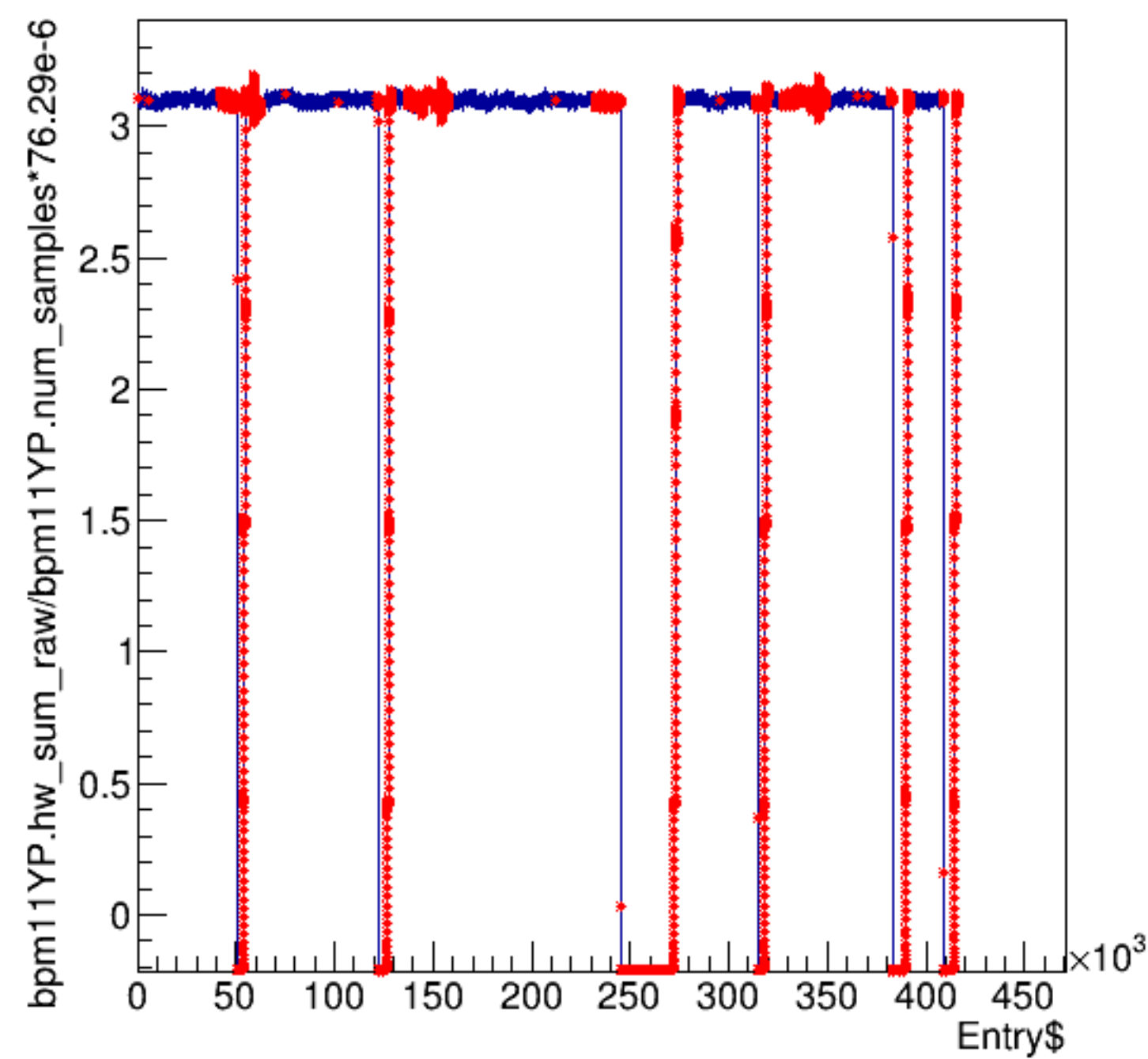
bpm11YP.hw_sum_raw/bpm11YP.num_samples*76.29e-6:Entry$
