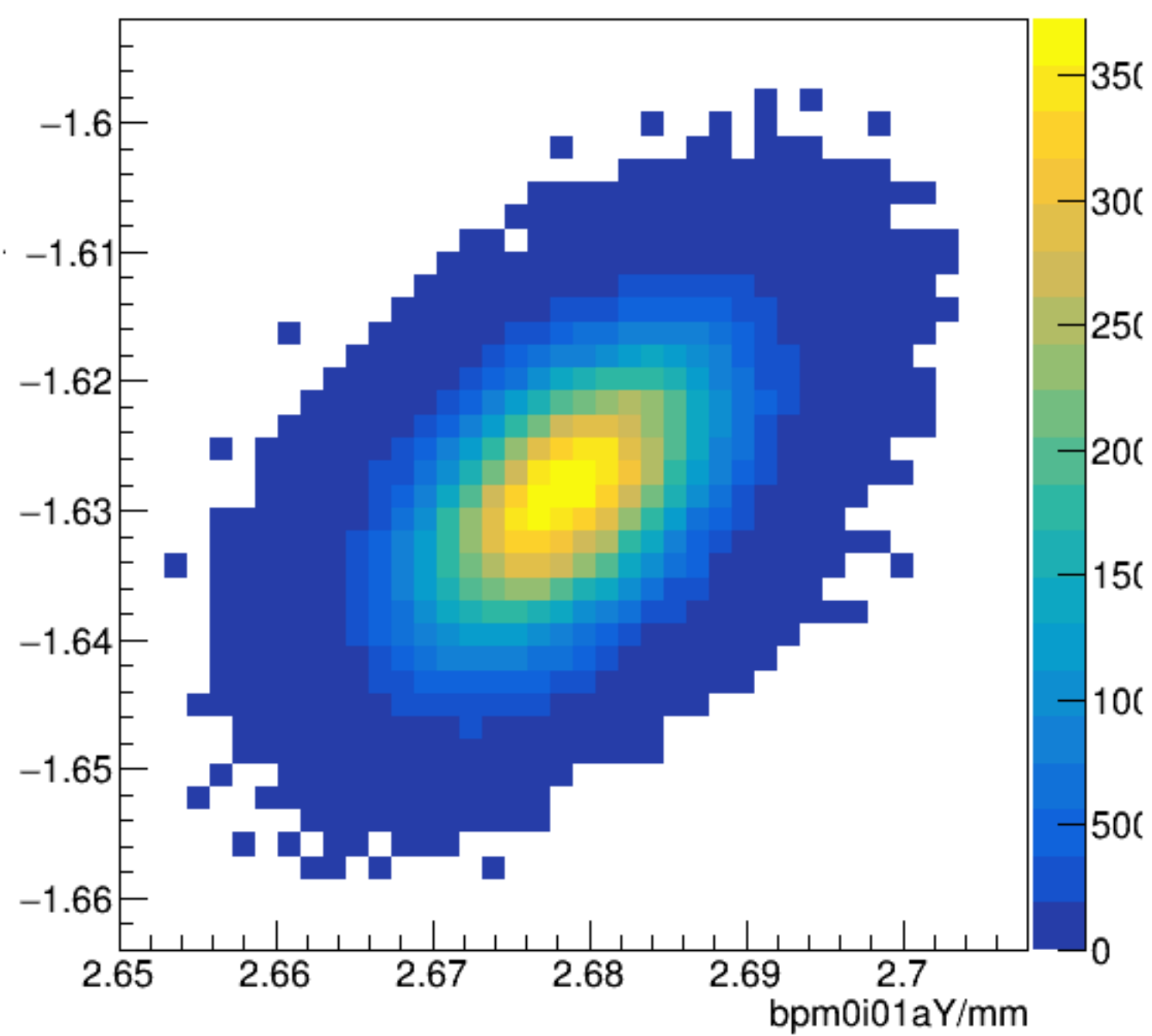
bpm0i01aX/mm:bpm0i01aY/mm {ErrorFlag==0}
