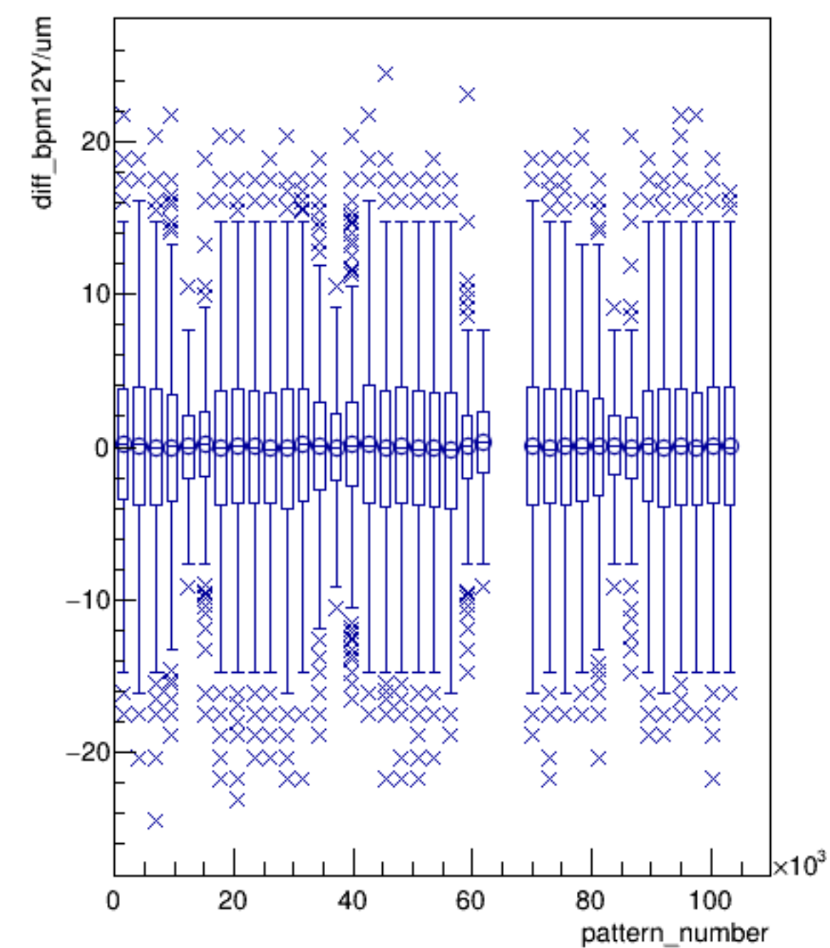
diff_bpm12Y/um:pattern_number {ErrorFlag==0}
