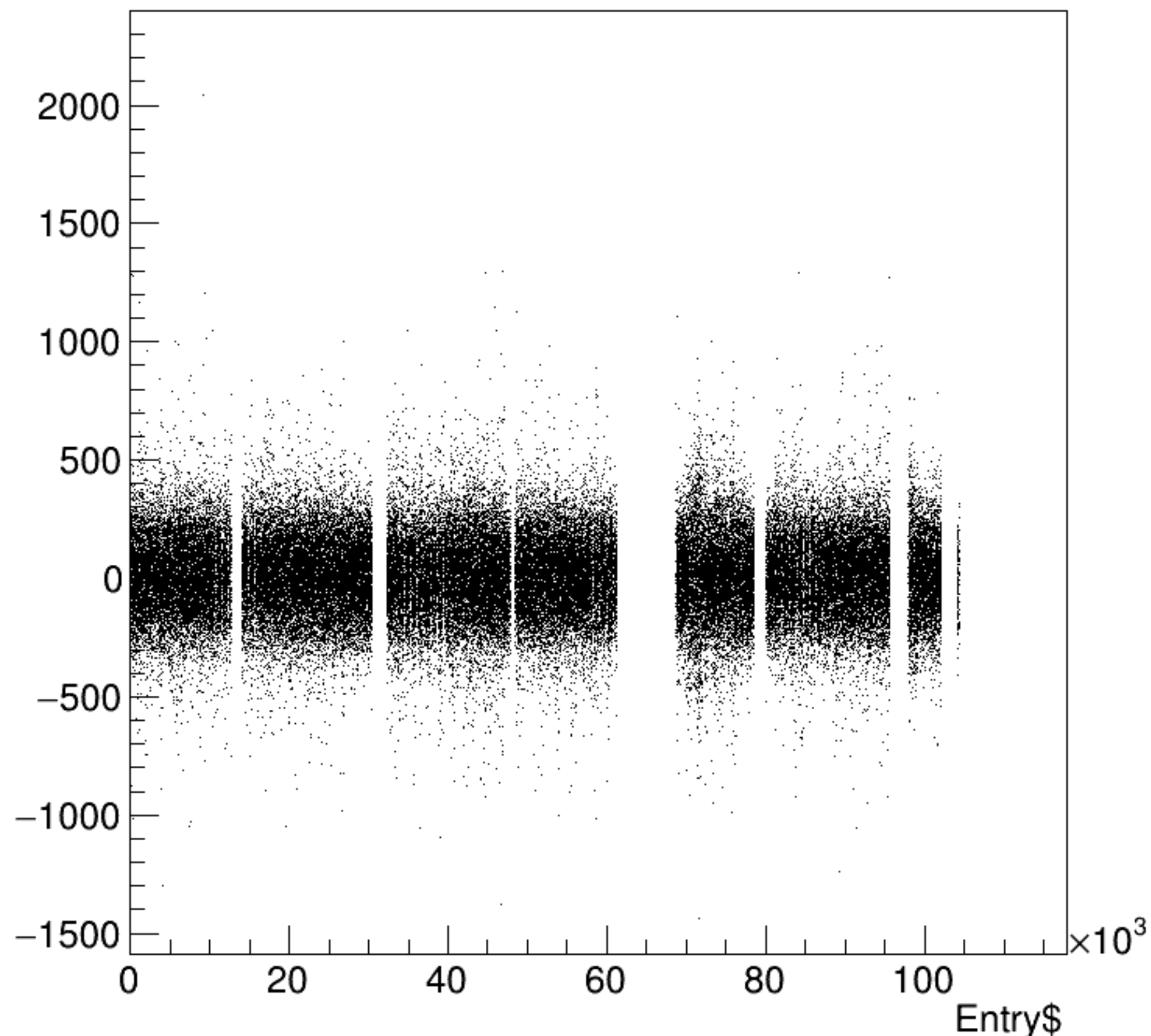
asym_bpm2i01WS/ppm:Entry$ {ErrorFlag==0}
