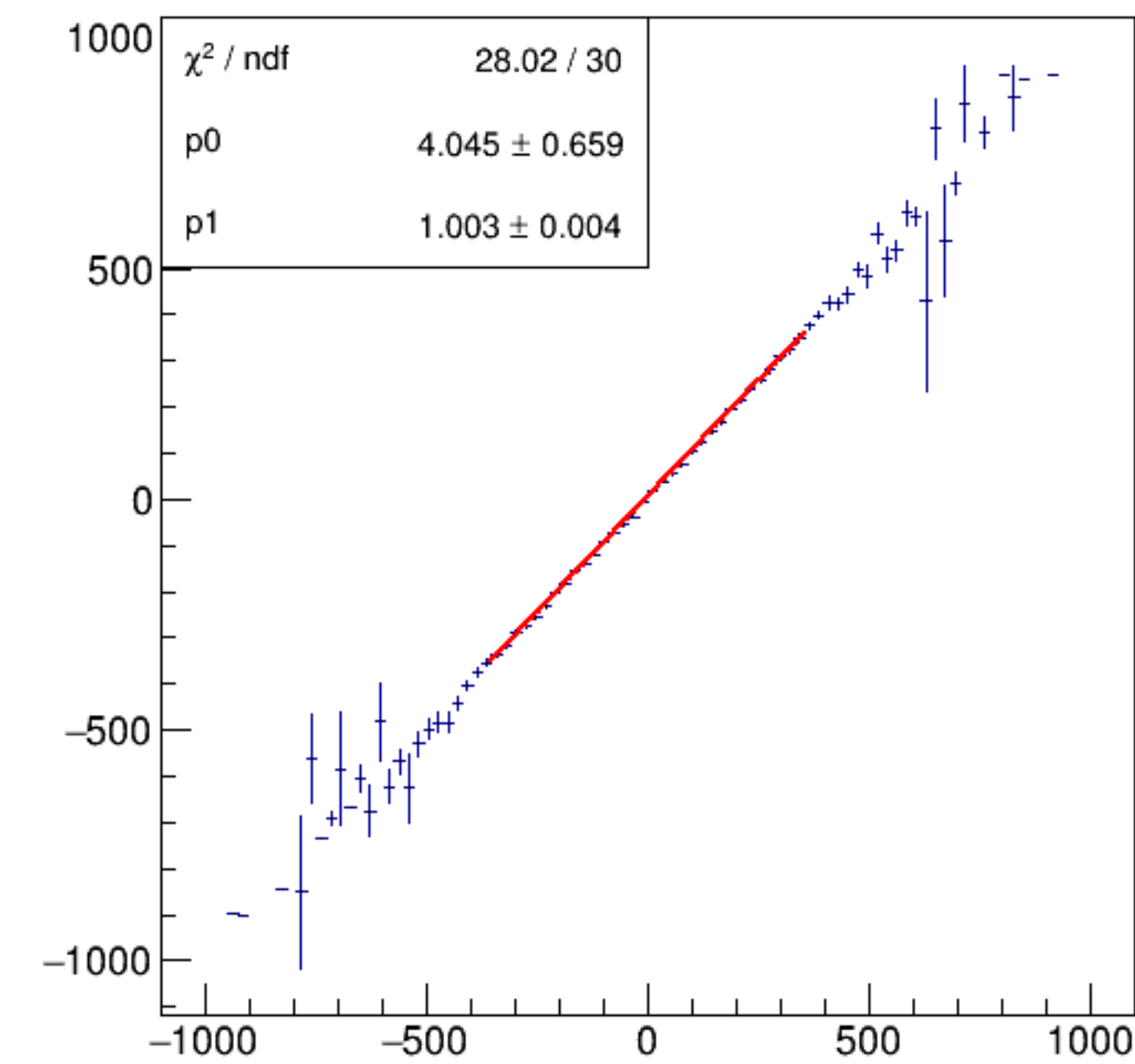
asym_bpm0l01WS/ppm:Aq/ppm {ErrorFlag==0}
