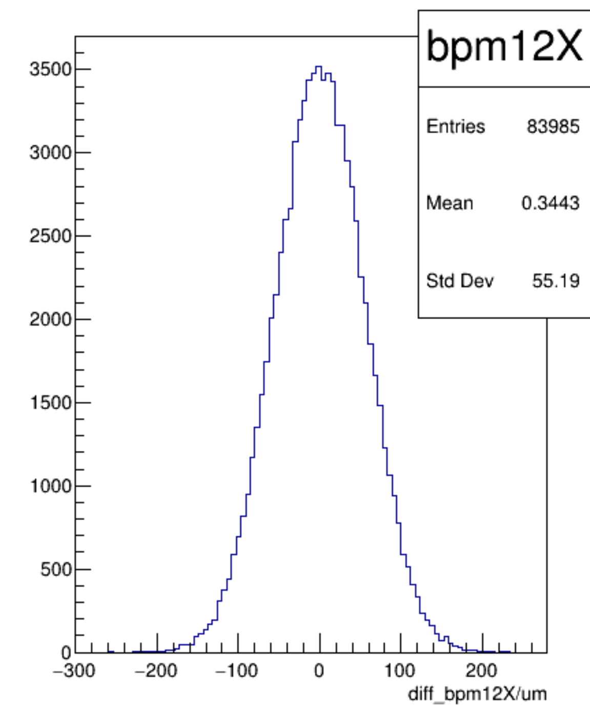
diff_bpm12X/um {ErrorFlag==0}
