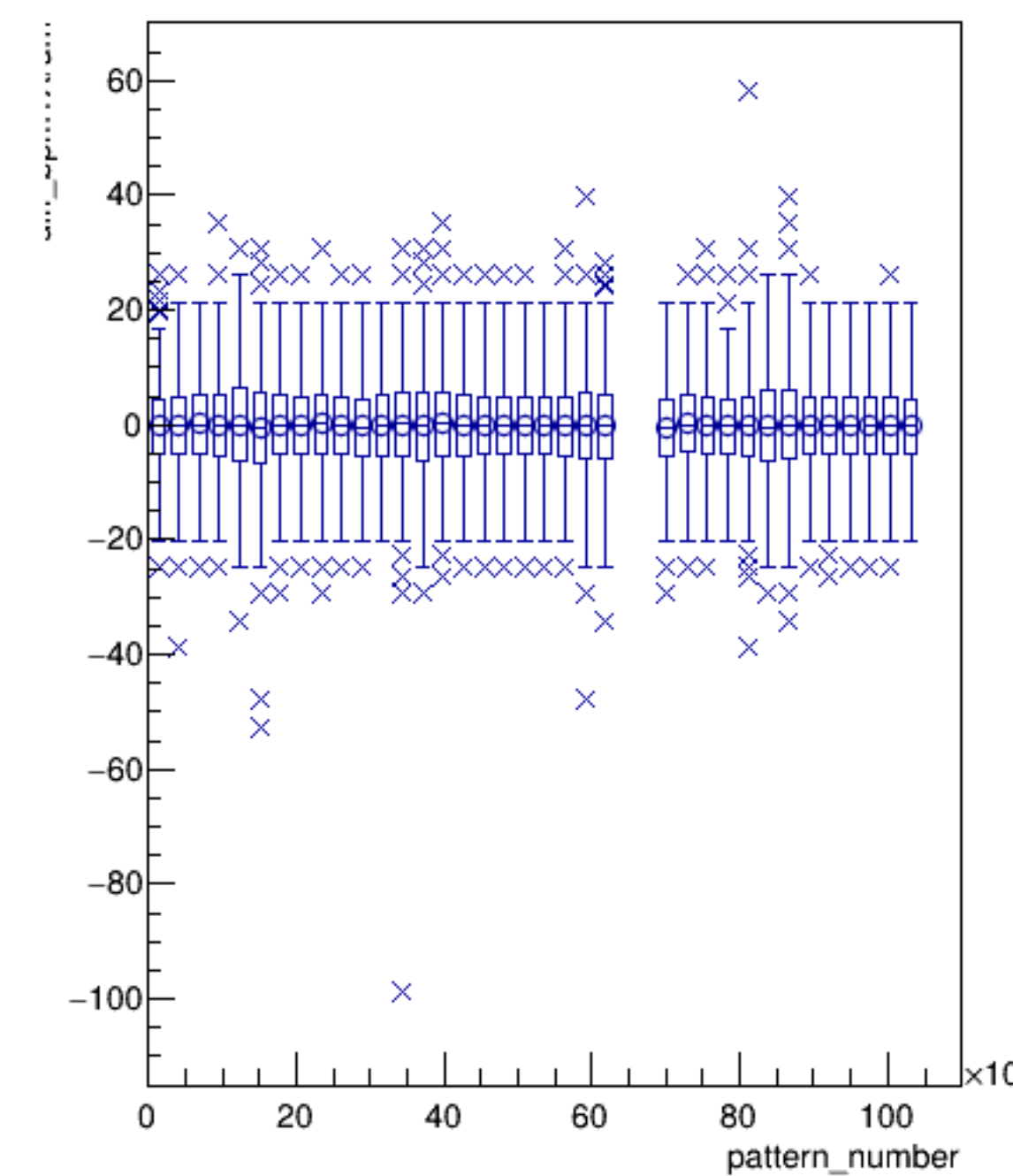
diff_bpm1X/um:pattern_number {ErrorFlag==0}
