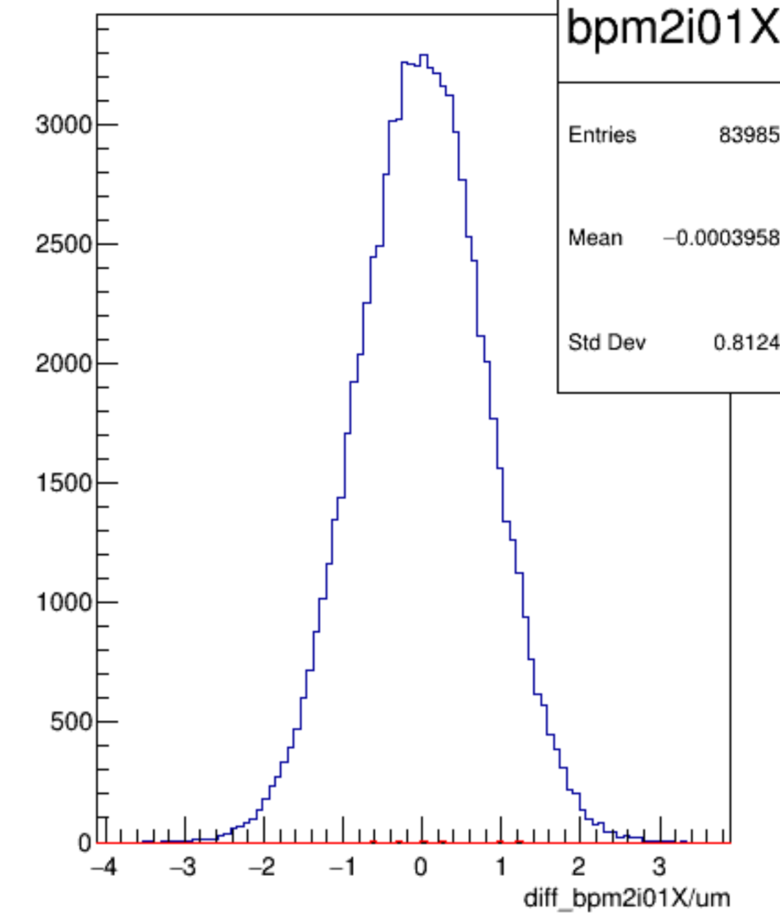
diff_bpm2i01X/um {ErrorFlag==0}
