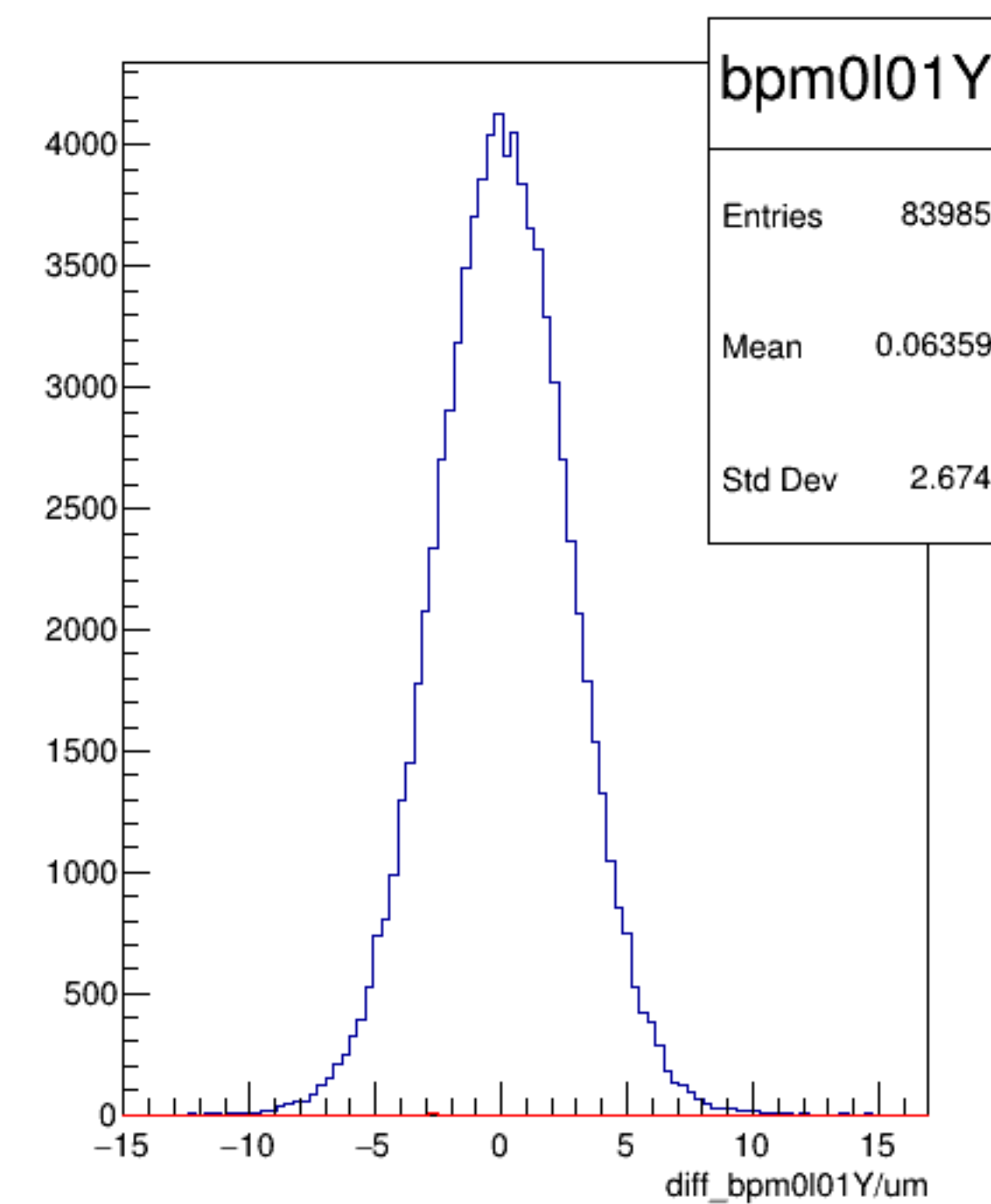
diff_bpm0l01Y/um {ErrorFlag==0}
