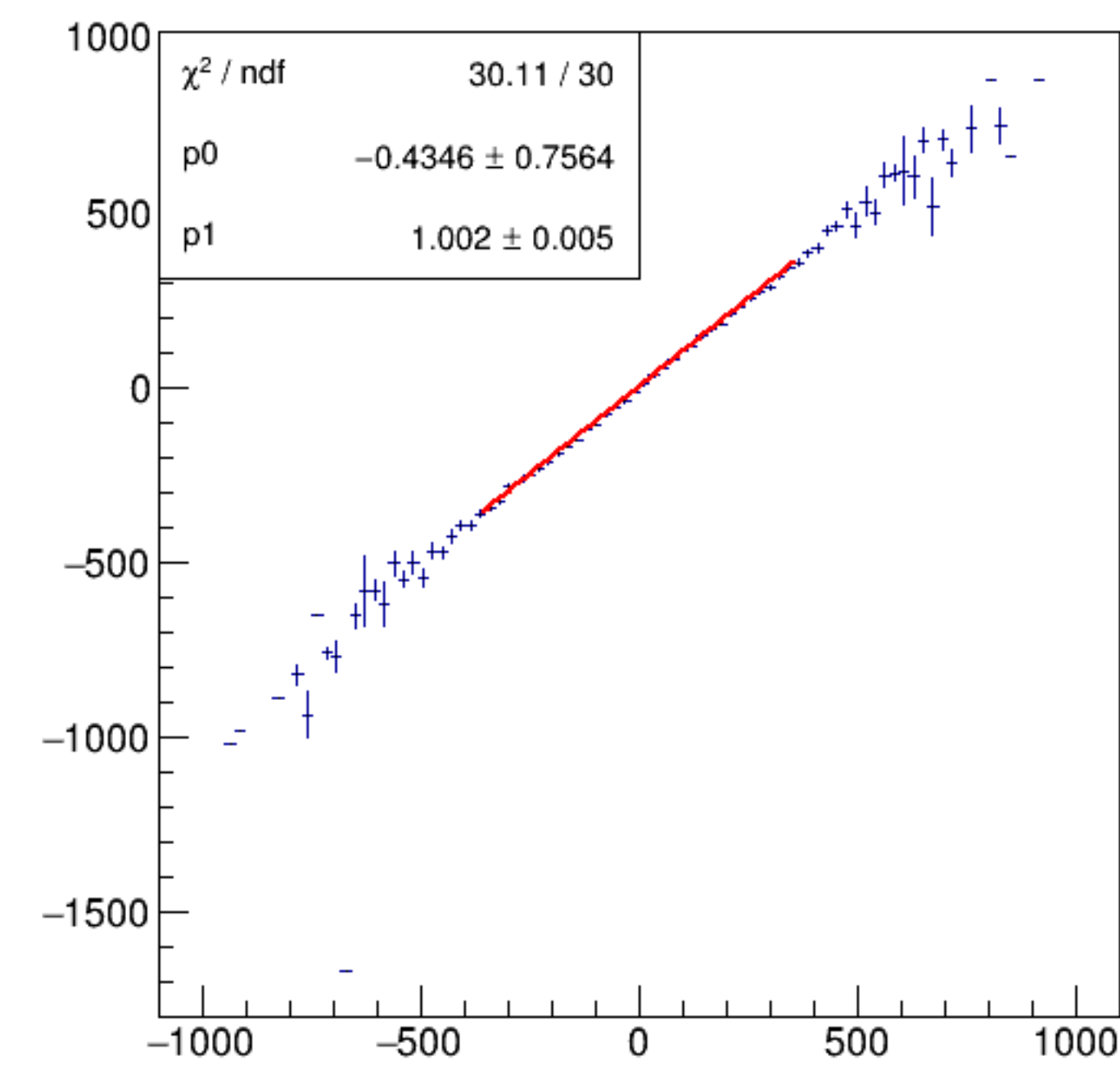
asym_bpm1WS/ppm:Aq/ppm {ErrorFlag==0}
