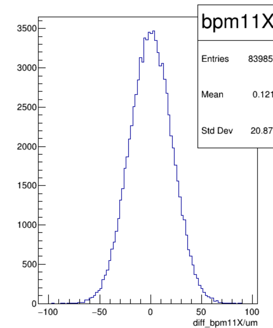
diff_bpm11X/um {ErrorFlag==0}
