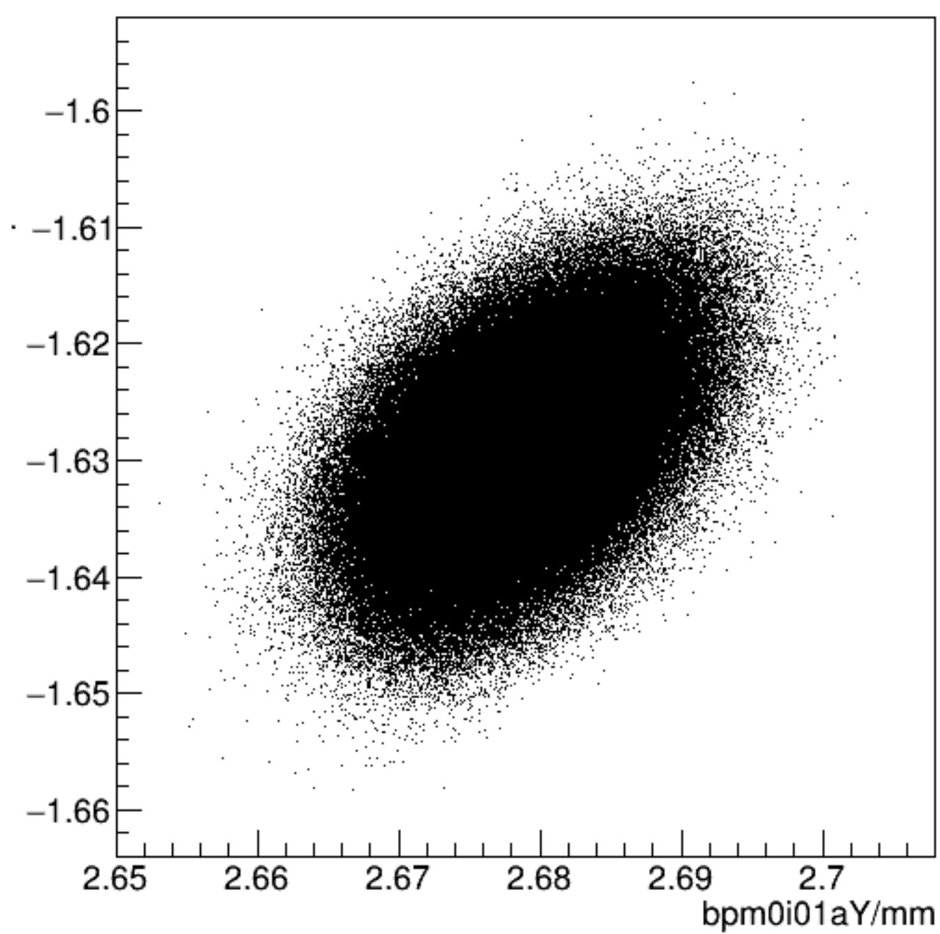
bpm0i01aX/mm:bpm0i01aY/mm {ErrorFlag==0}
