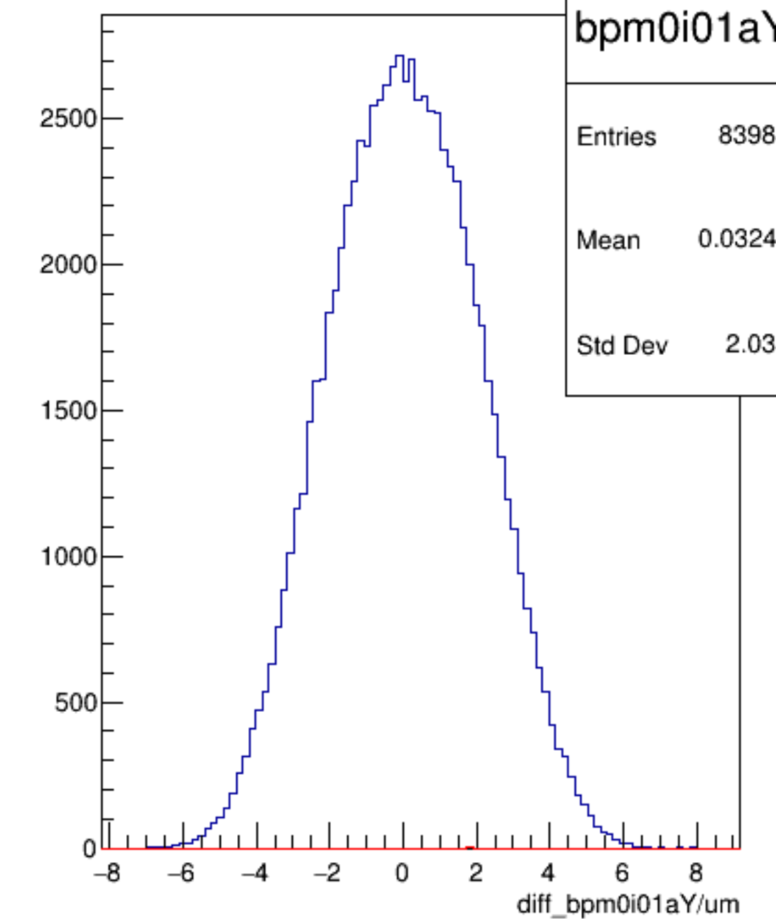
diff_bpm0i01aY/um {ErrorFlag==0}
