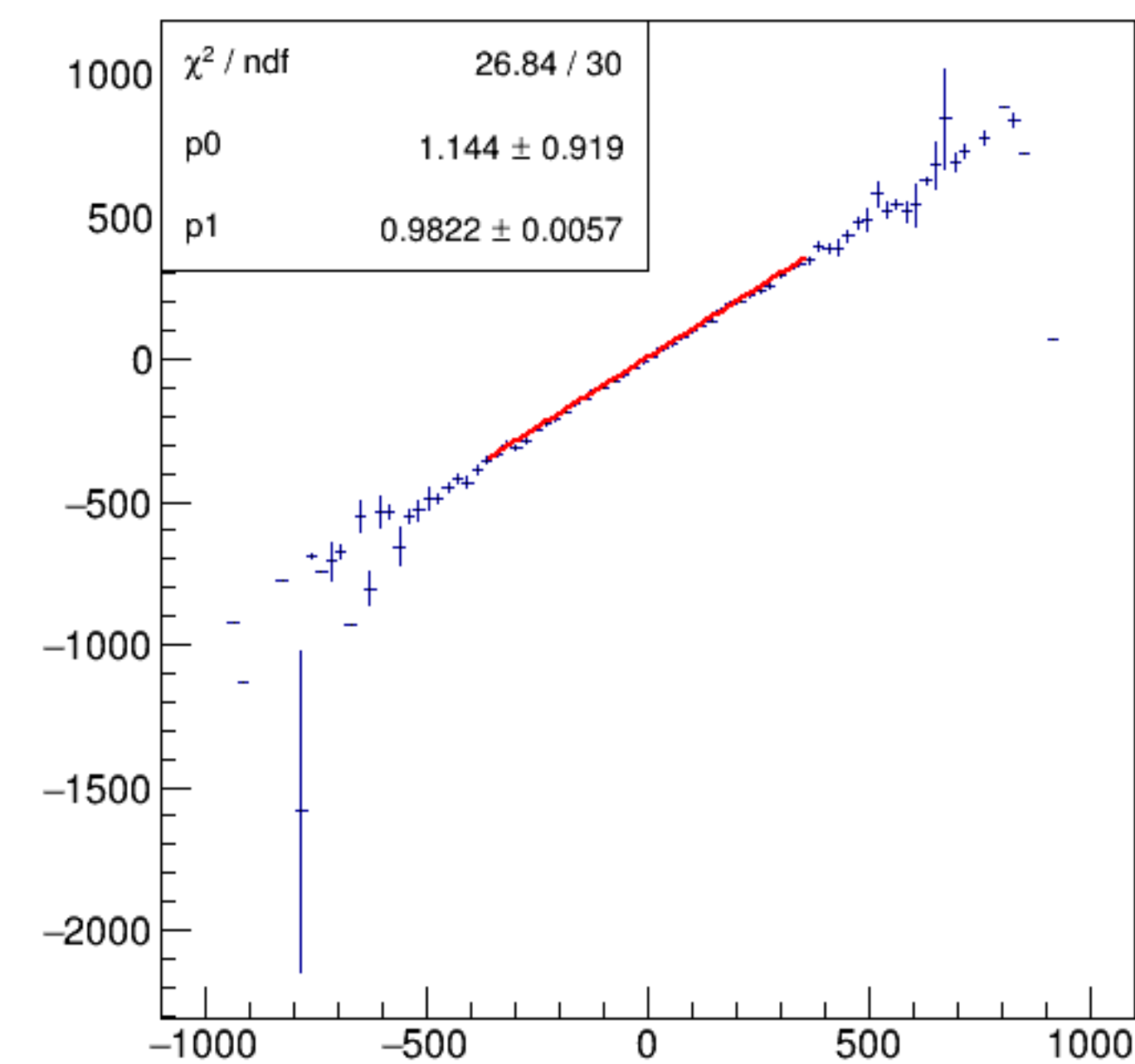
asym_bpm4acWS/ppm:Aq/ppm {ErrorFlag==0}
