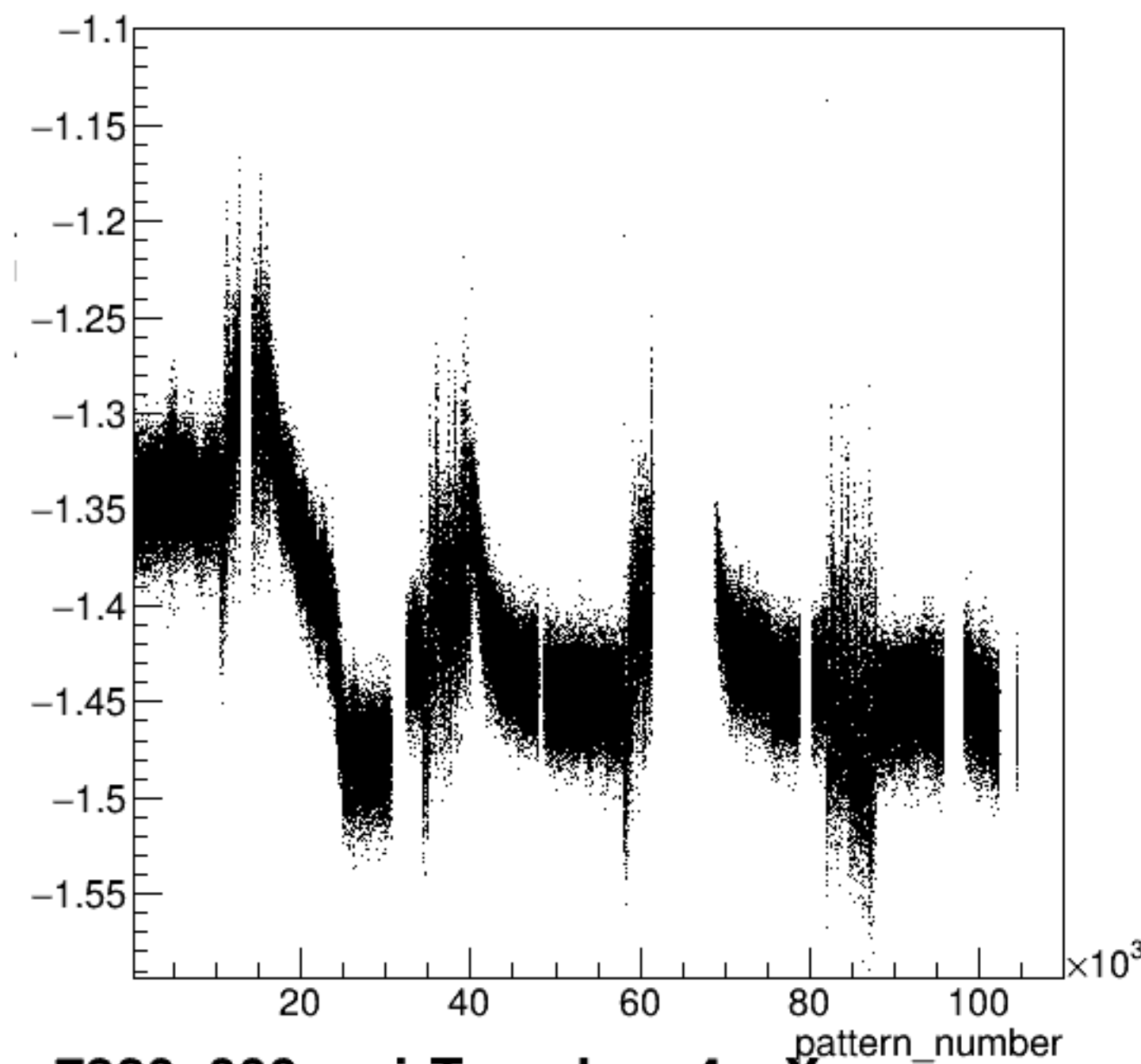
yield_bpm4acX/mm:pattern_number {ErrorFlag==0}
