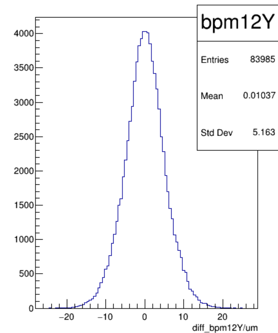
diff_bpm12Y/um {ErrorFlag==0}
