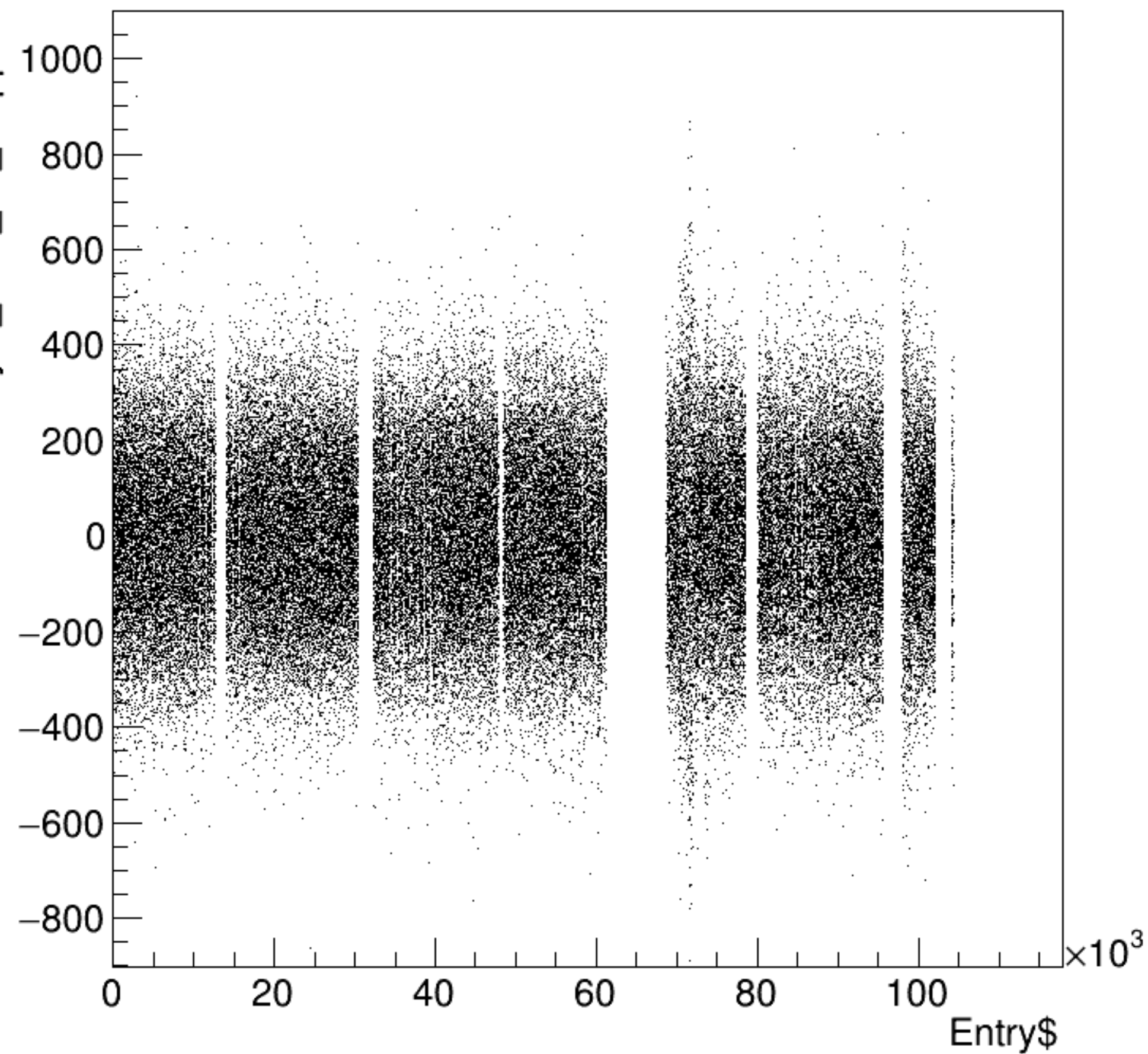
asym_bcm_an_us/ppm:Entry$ {ErrorFlag==0}
