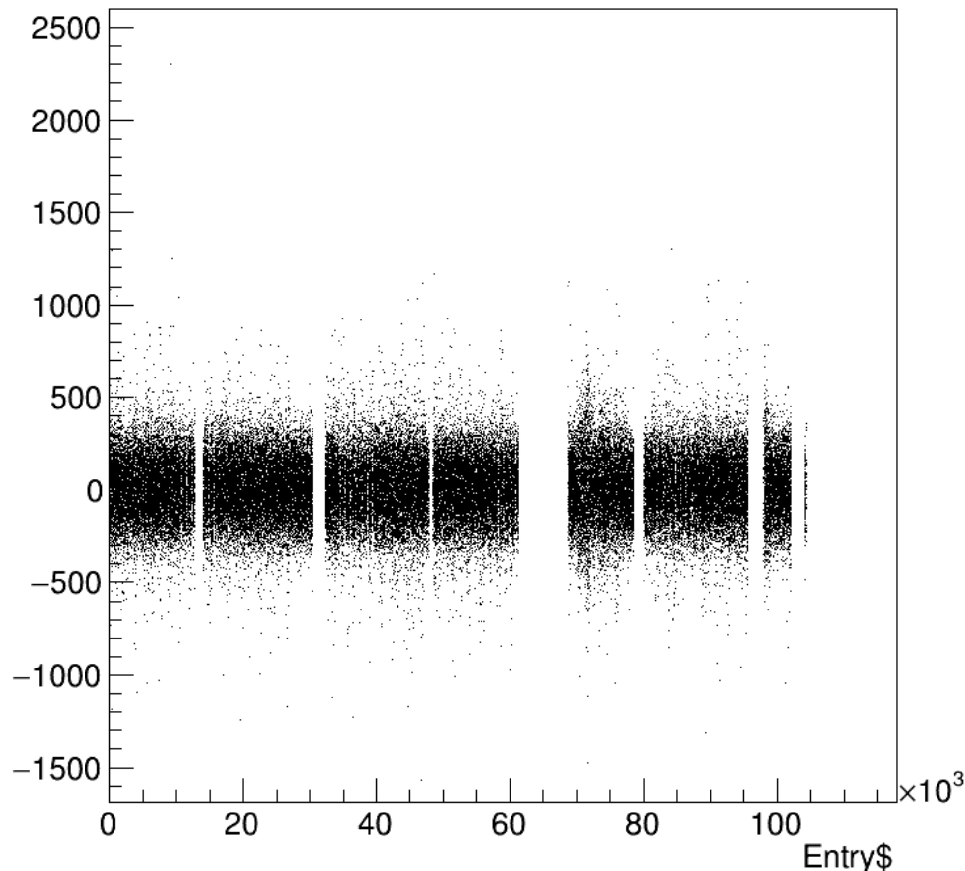
asym_bpm2i02WS/ppm:Entry$ {ErrorFlag==0}
