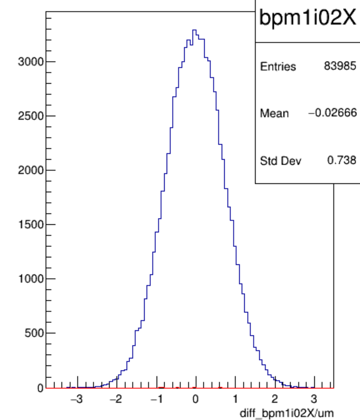
diff_bpm1i02X/um {ErrorFlag==0}
