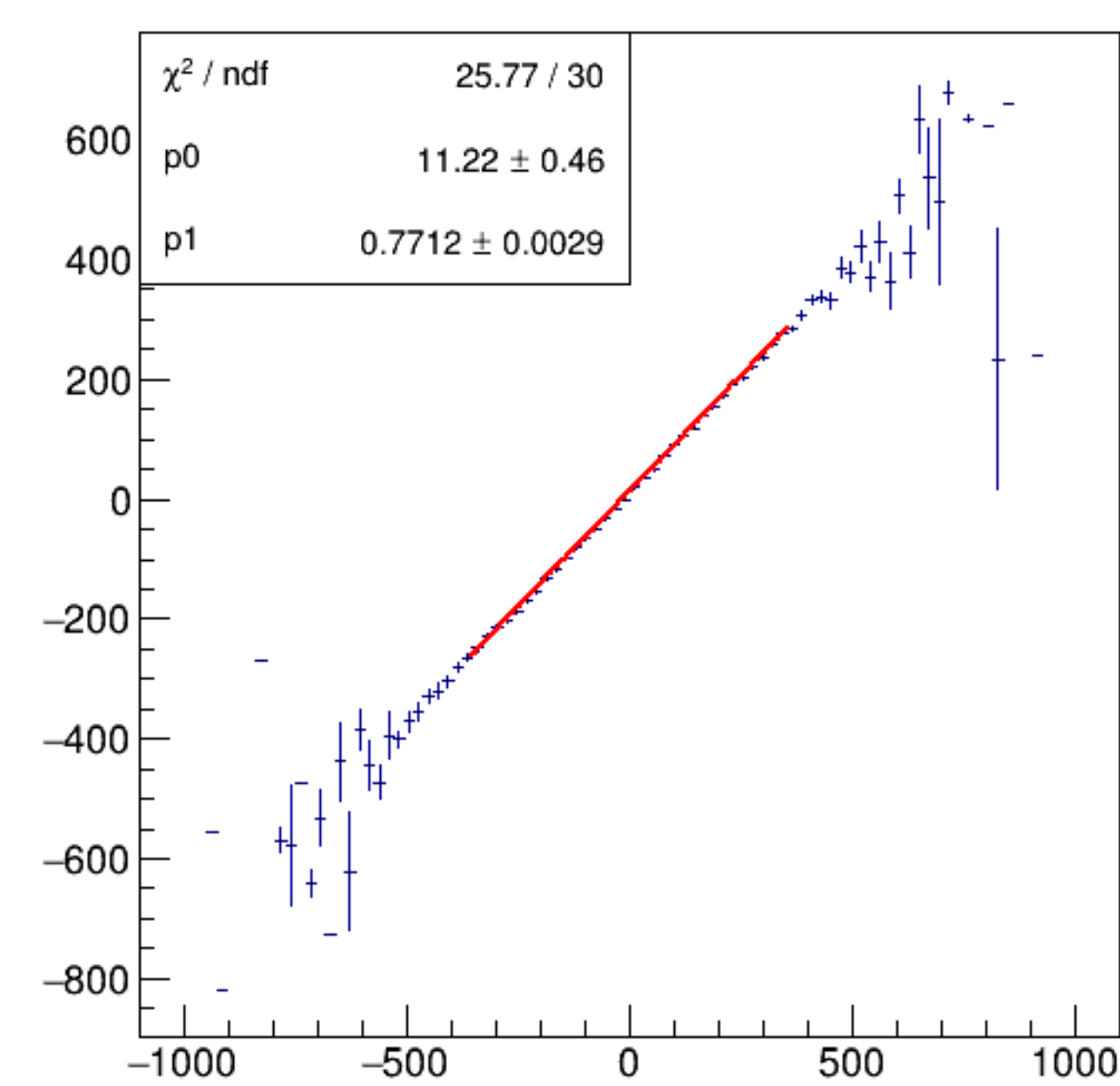
asym_bpm1i02WS/ppm:Aq/ppm {ErrorFlag==0}
