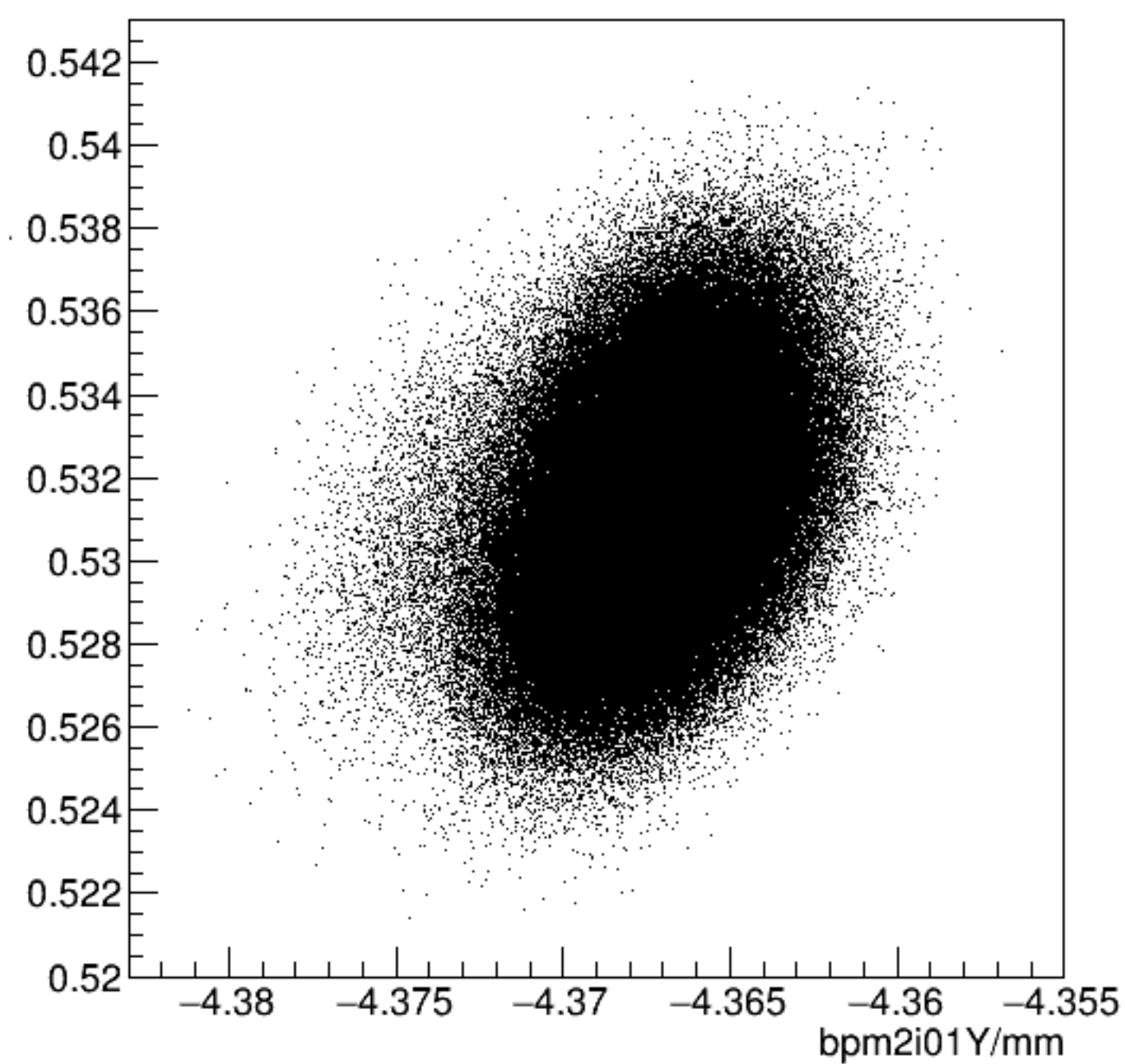
bpm2i01X/mm:bpm2i01Y/mm {ErrorFlag==0}
