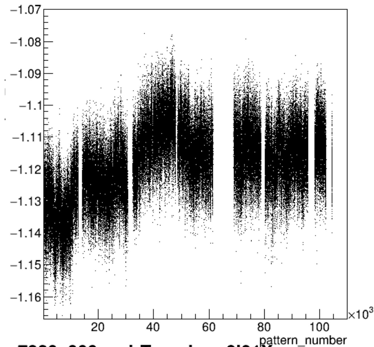
yield_bpm0l01X/mm:pattern_number {ErrorFlag==0}
