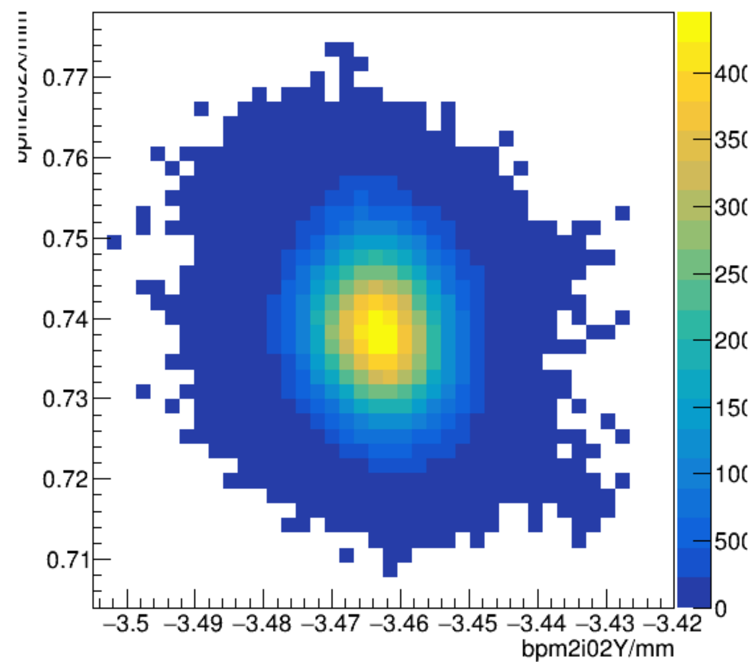
bpm2i02X/mm:bpm2i02Y/mm {ErrorFlag==0}
