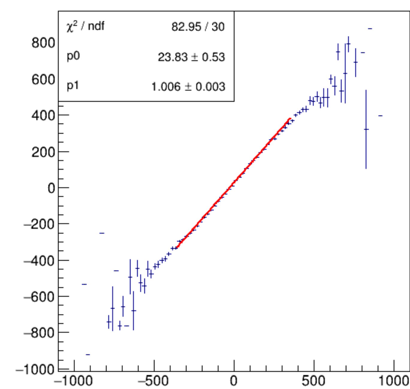
asym_bpm0i02WS/ppm:Aq/ppm {ErrorFlag==0}
