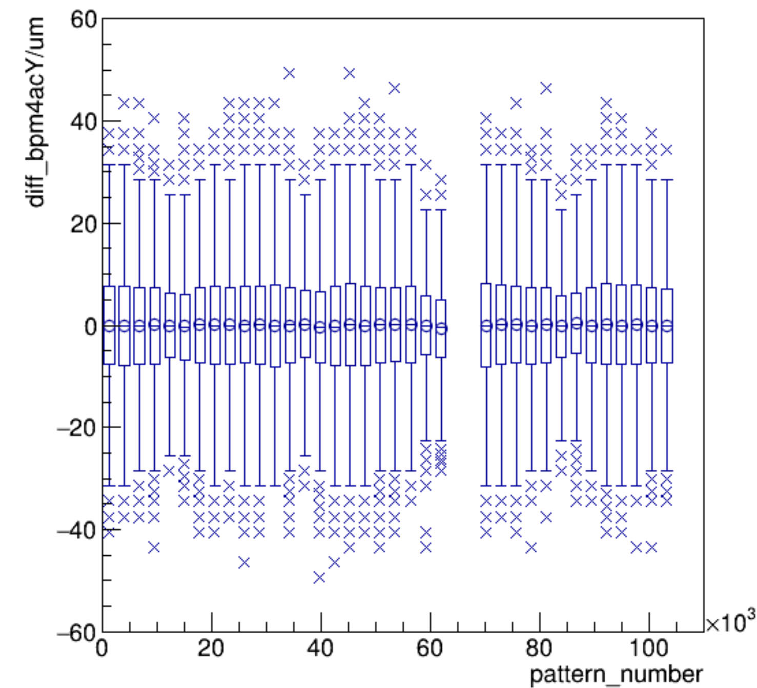
diff_bpm4acY/um:pattern_number {ErrorFlag==0}
