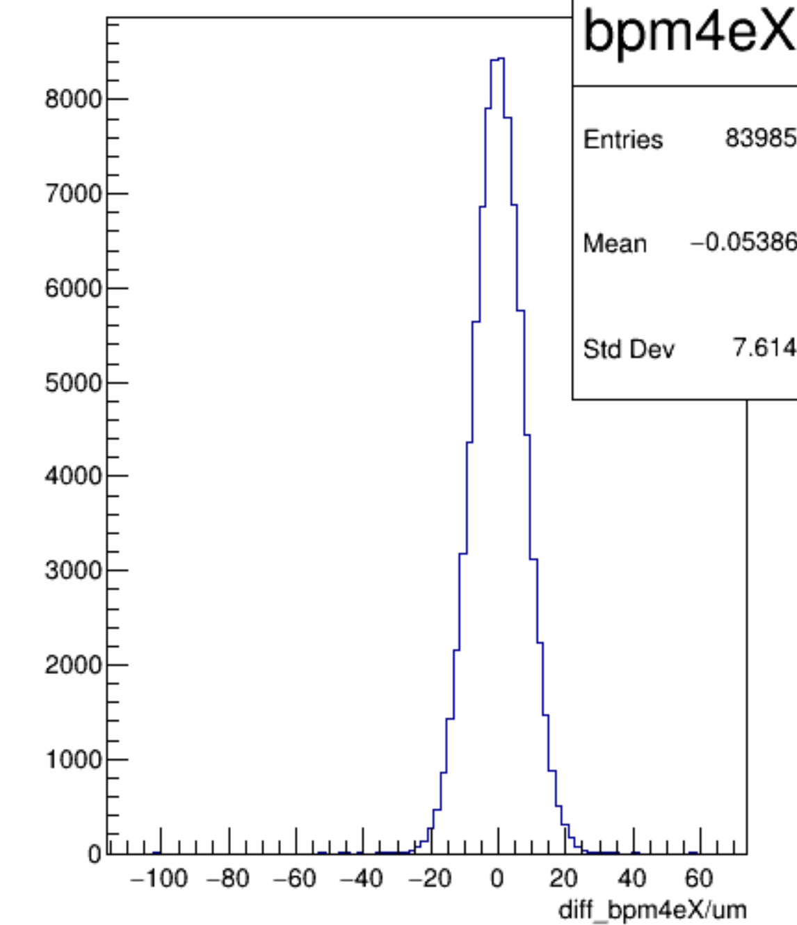
diff_bpm4eX/um {ErrorFlag==0}
