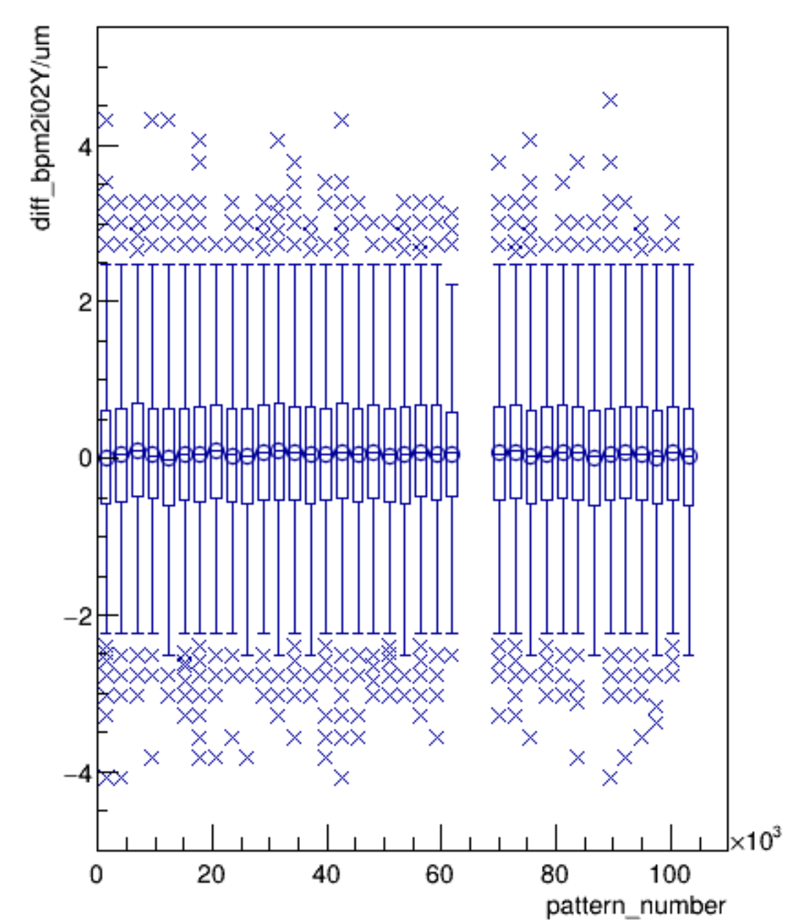
diff_bpm2i02Y/um:pattern_number (ErrorFlag==0)
