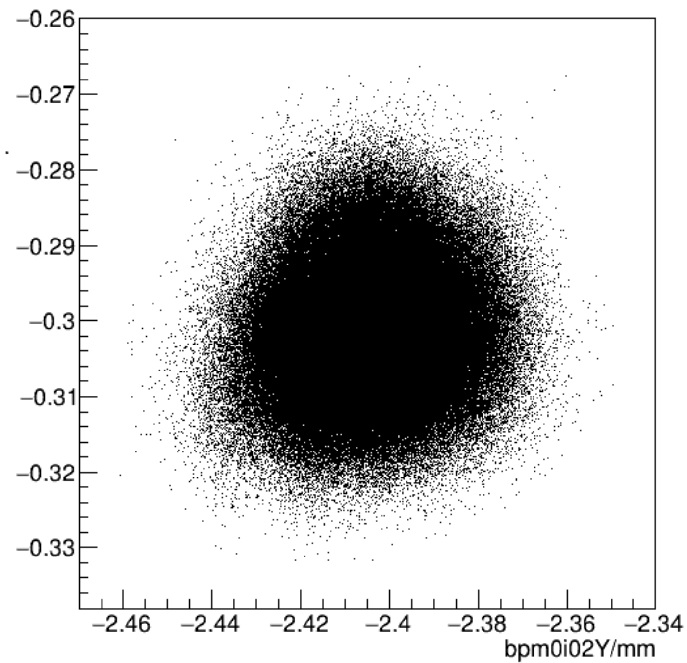
bpm0i02X/mm:bpm0i02Y/mm {ErrorFlag==0}
