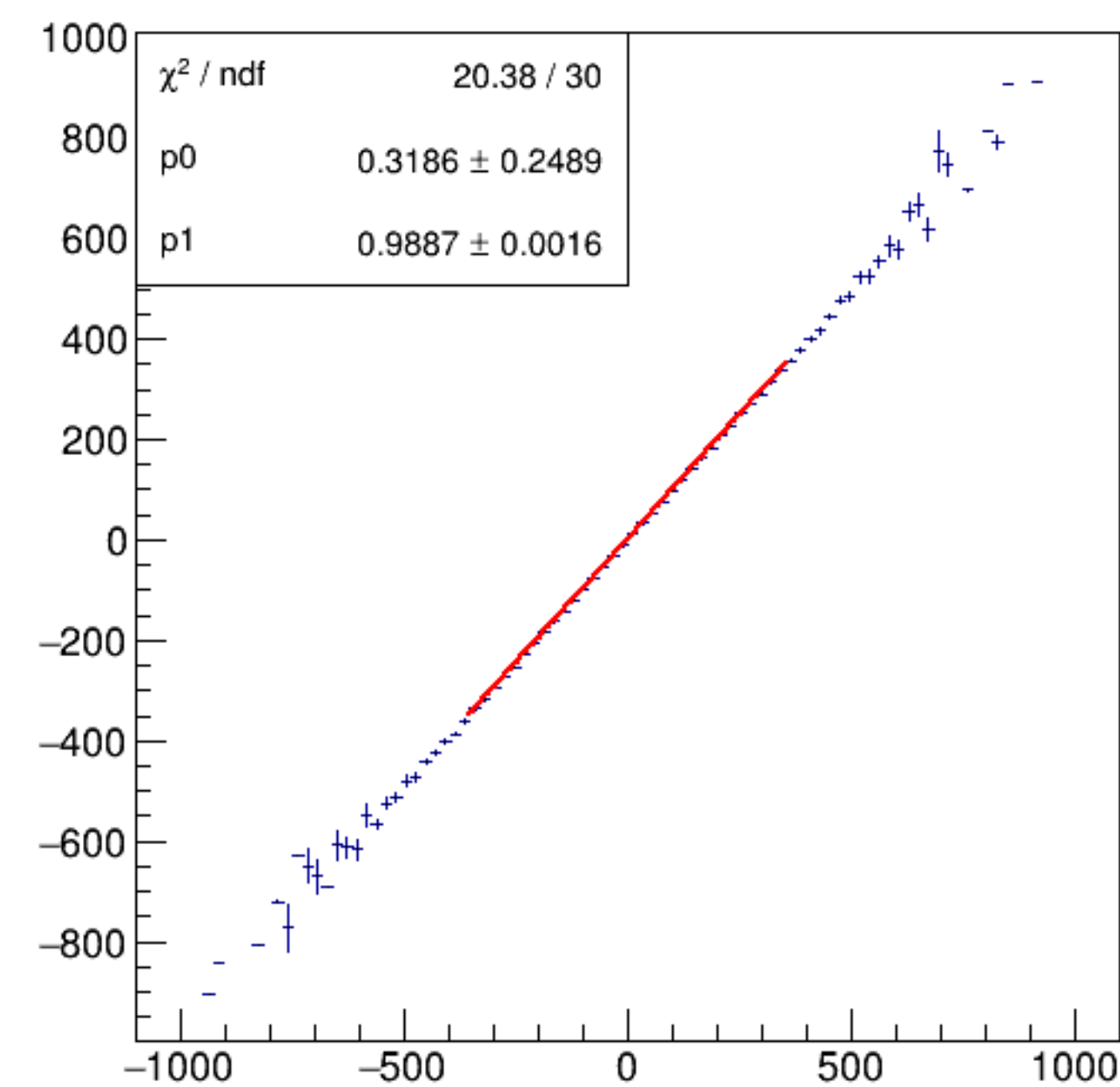
asym_bpm11WS/ppm:Aq/ppm {ErrorFlag==0}
