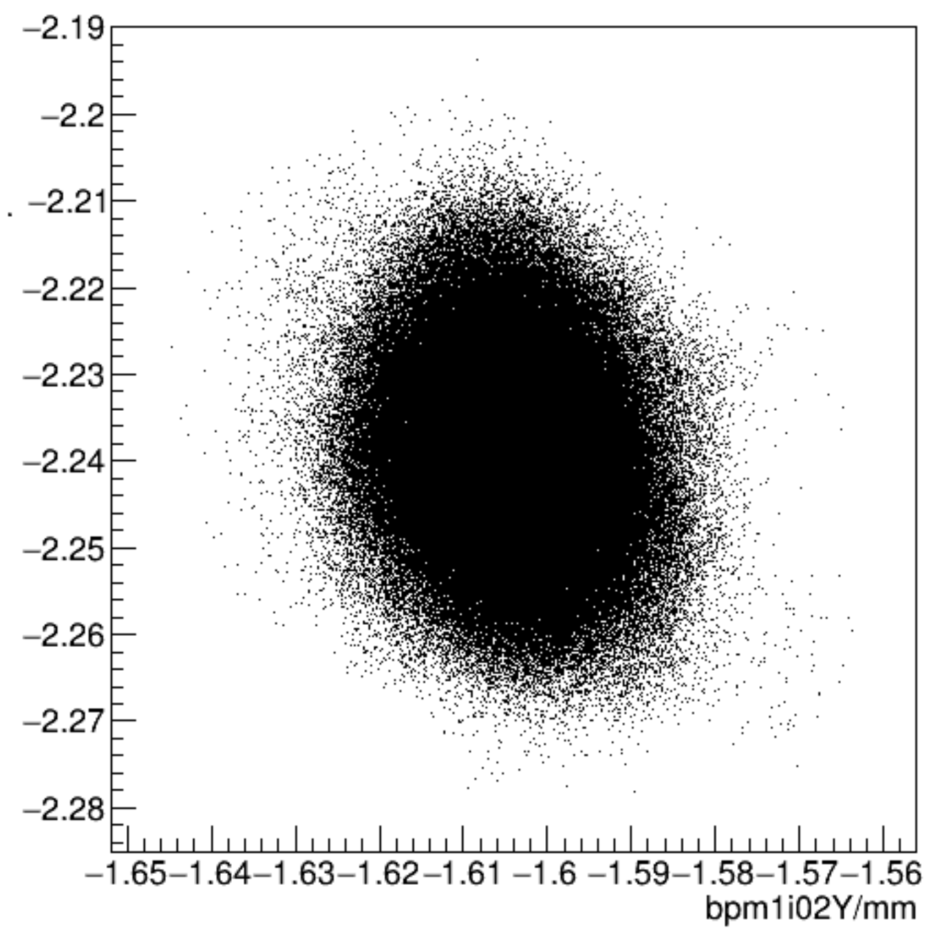
bpm1i02X/mm:bpm1i02Y/mm {ErrorFlag==0}
