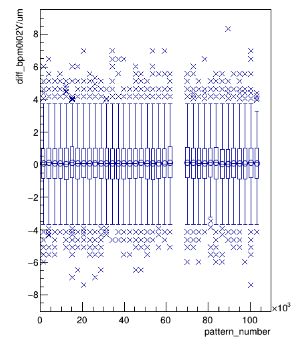
diff_bpm0i02Y/um:pattern_number (ErrorFlag==0)
