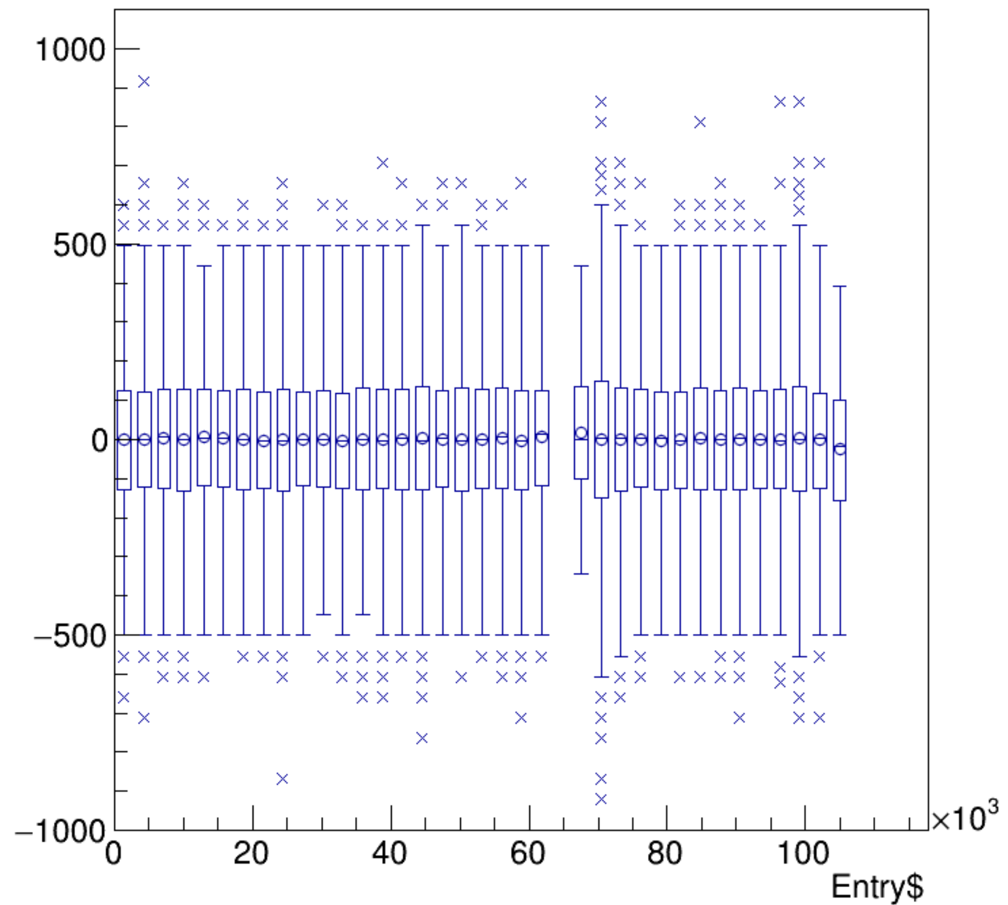
asym_bcm_an_us/ppm:Entry$ {ErrorFlag==0}
