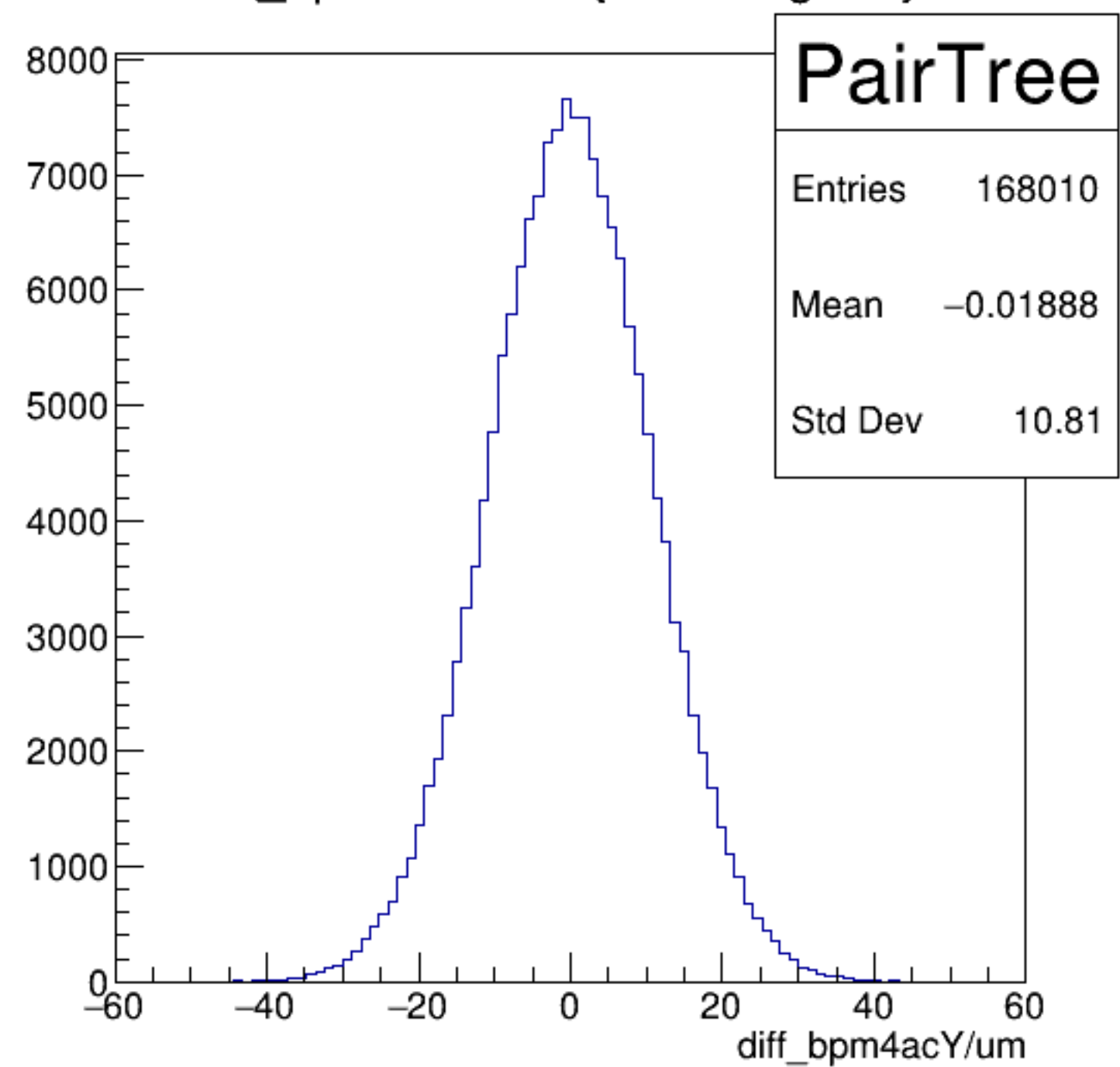
diff_bpm4acY/um {ErrorFlag==0}
