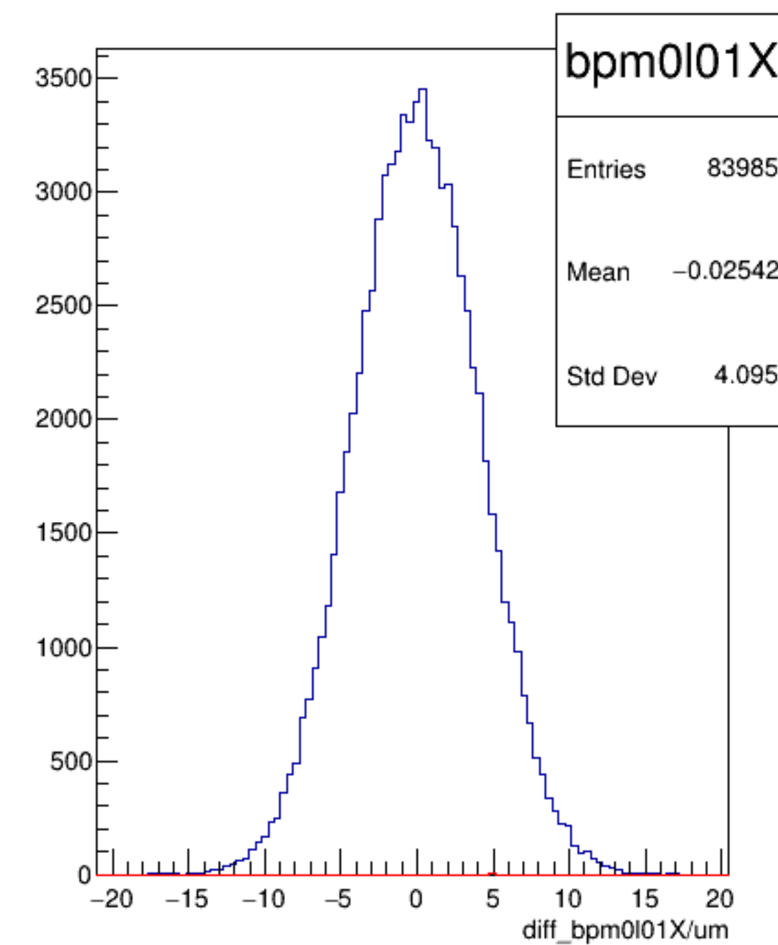
diff_bpm0l01X/um {ErrorFlag==0}
