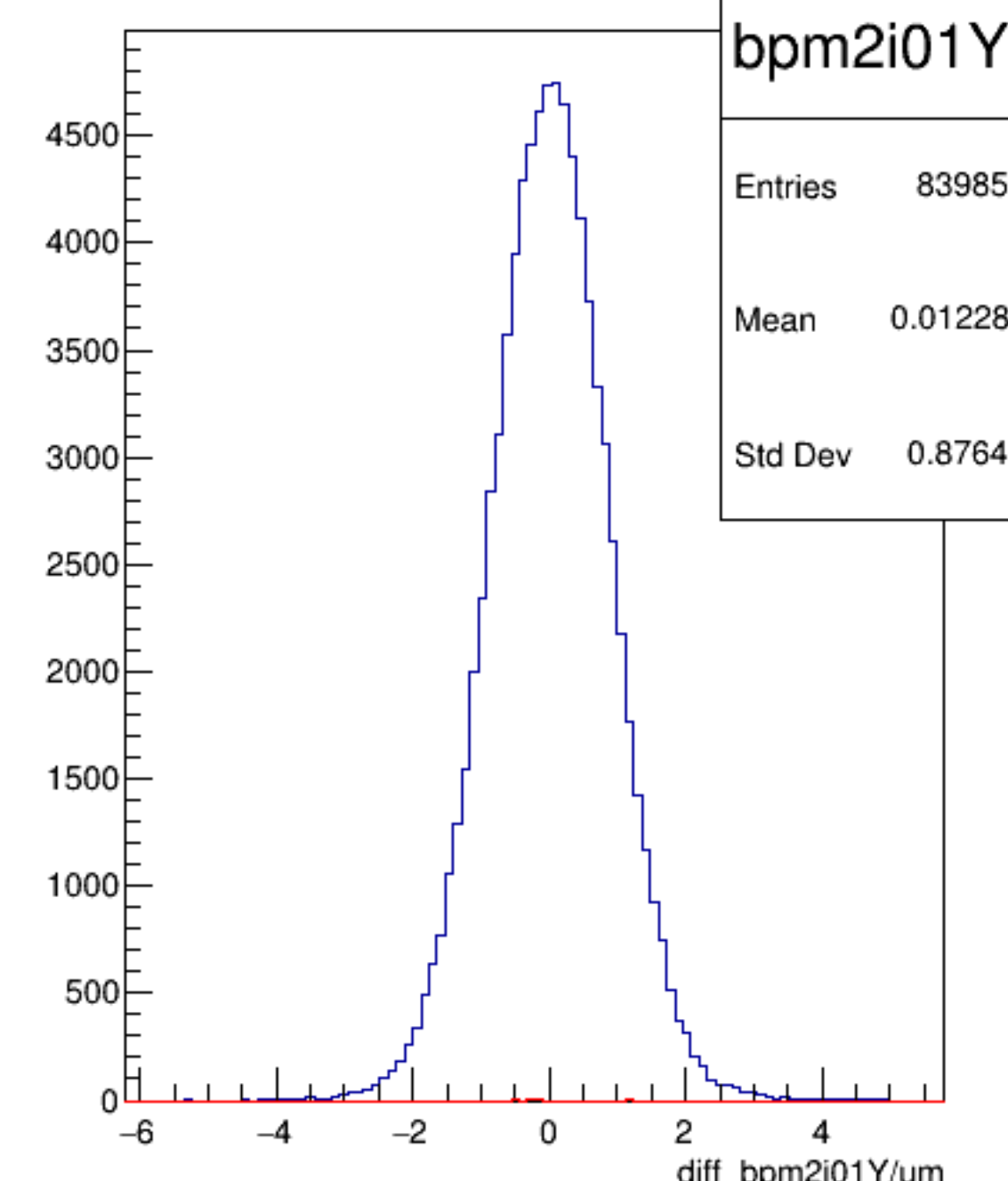
diff_bpm2i01Y/um {ErrorFlag==0}
