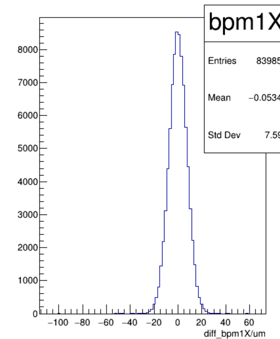
diff_bpm1X/um {ErrorFlag==0}
