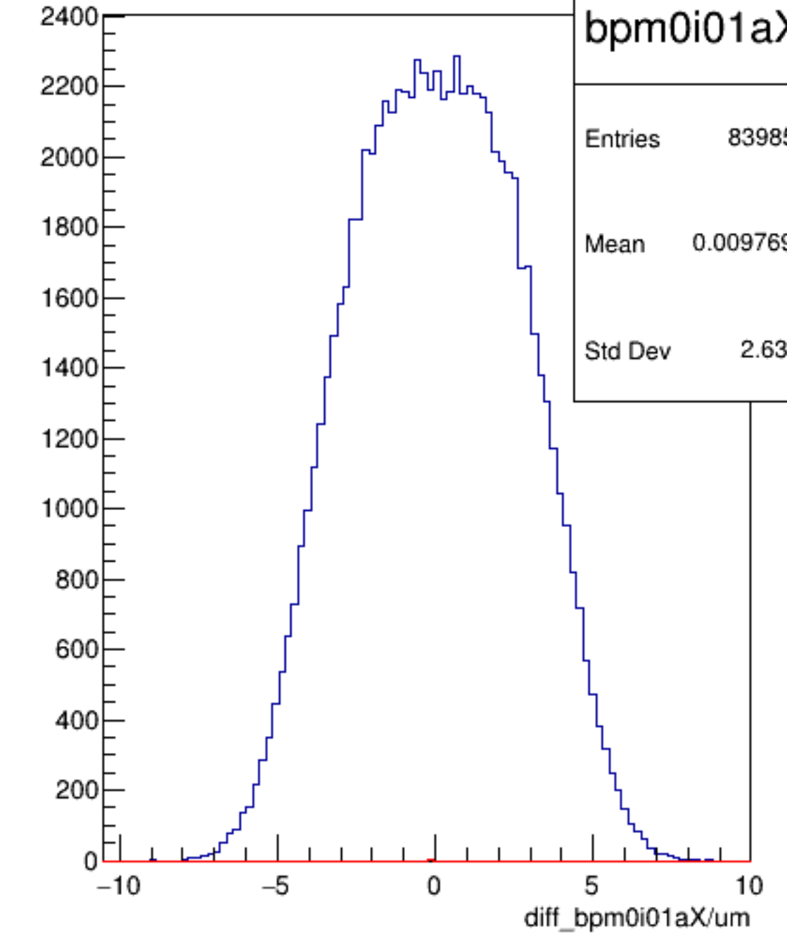
diff_bpm0i01aX/um {ErrorFlag==0}
