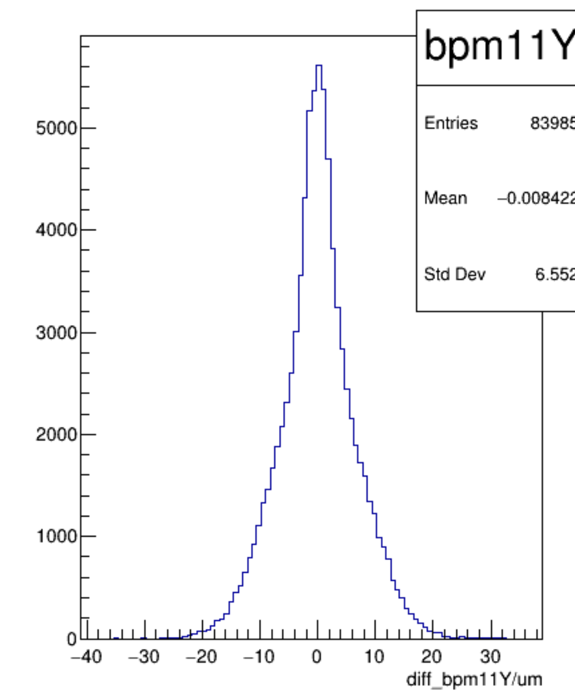
diff_bpm11Y/um {ErrorFlag==0}
