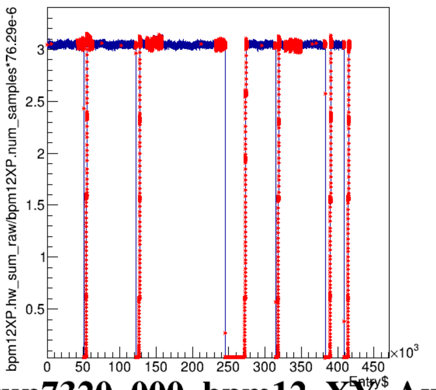
bpm12XP.hw_sum_raw/bpm12XP.num_samples*76.29e-6:Entry$
