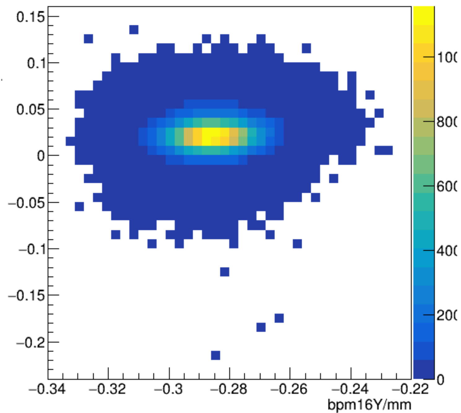
bpm16X/mm:bpm16Y/mm {ErrorFlag==0}
