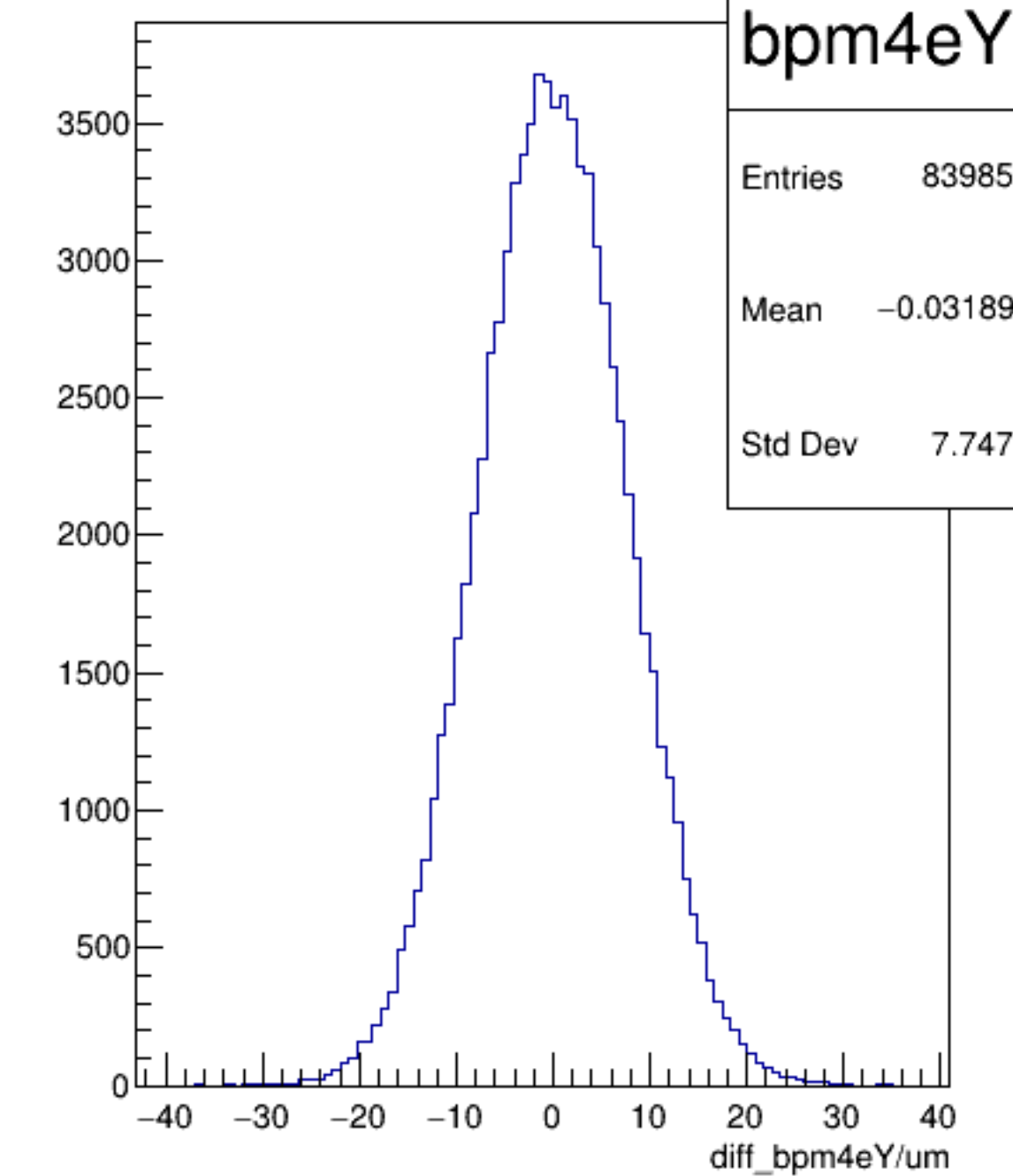
diff_bpm4eY/um {ErrorFlag==0}
