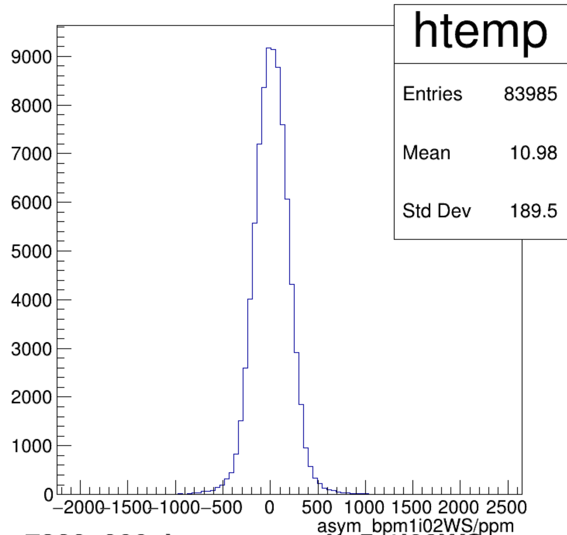
run7320_000_bpm_asym_bpm1i02WS.png
