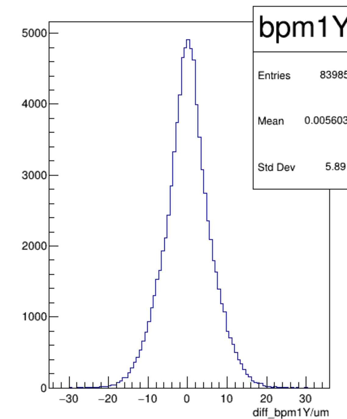
diff_bpm1Y/um {ErrorFlag==0}
