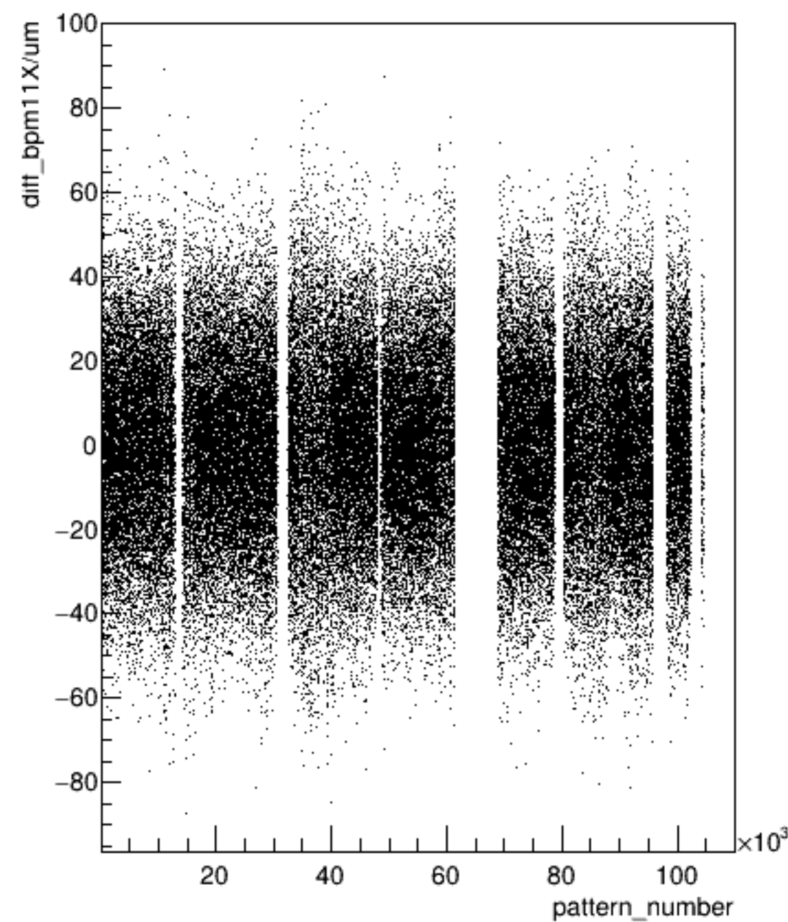
diff_bpm11X/um:pattern_number {ErrorFlag==0}
