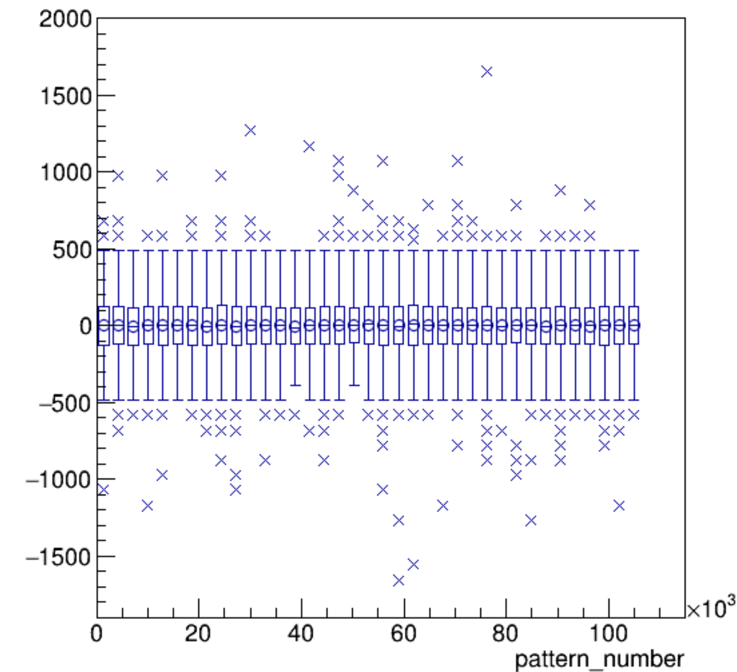
asym_bcm_dg_us/ppm:pattern_number {ErrorFlag==0}
