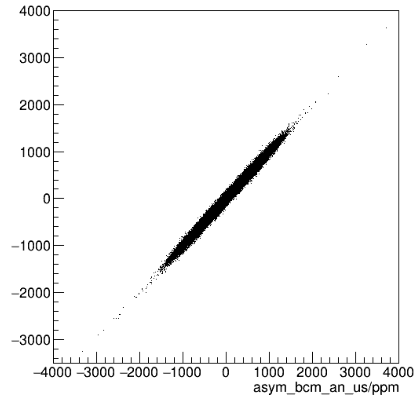
run7338_000_asym_bcm_dg_ds_vs_asym_bcm_an_us_pr.png
