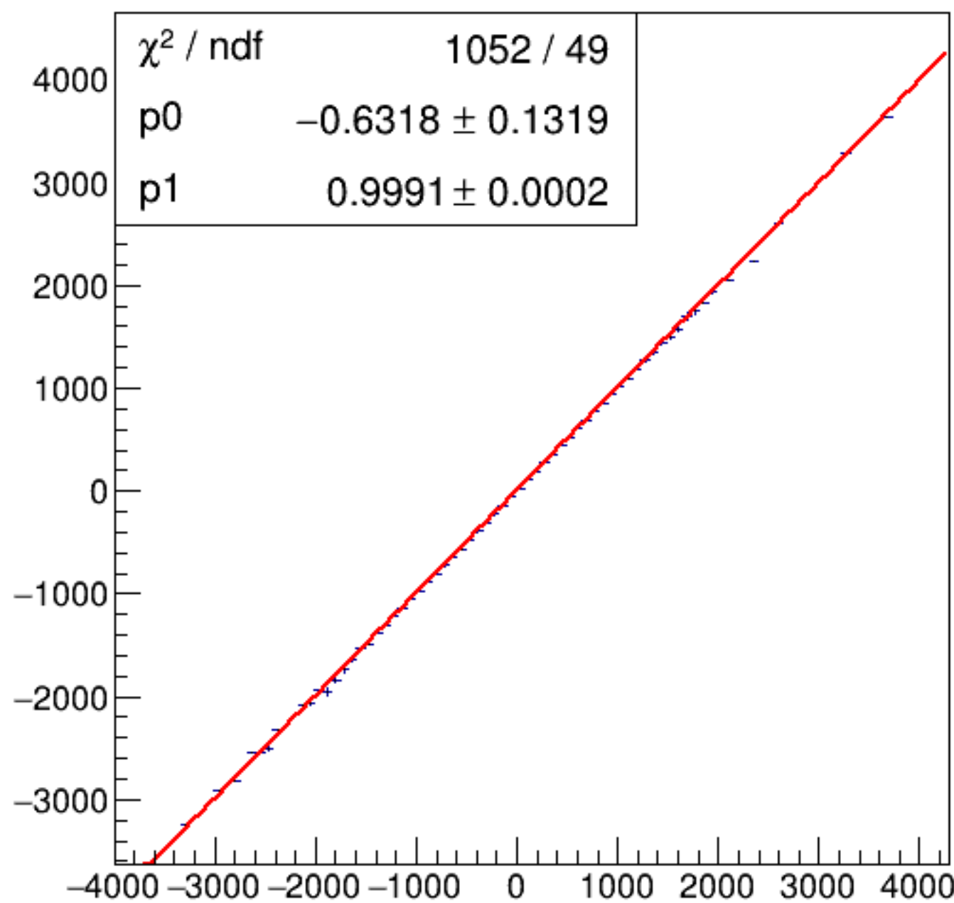
run7338_000_asym_bcm_dg_ds_vs_asym_bcm_an_us_pr.png
