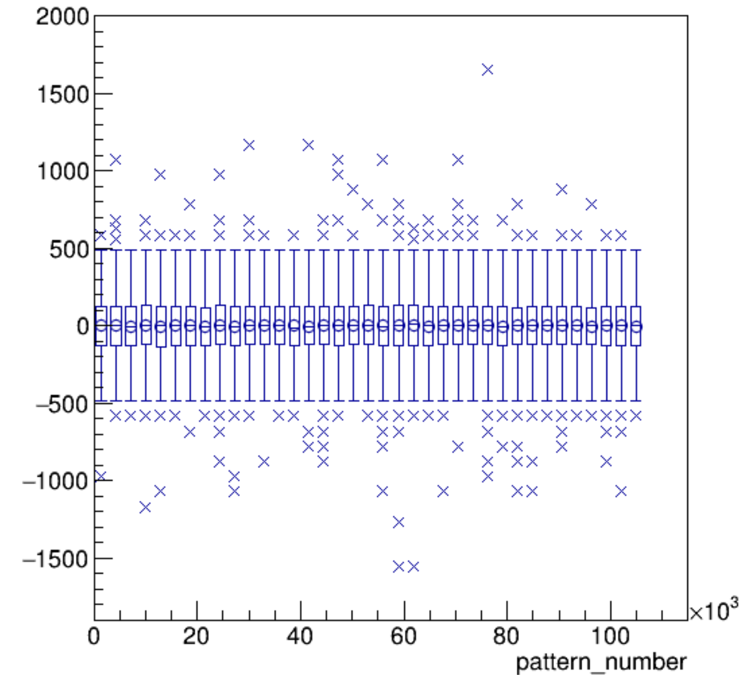
asym_bcm_dg_ds/ppm:pattern_number {ErrorFlag==0}
