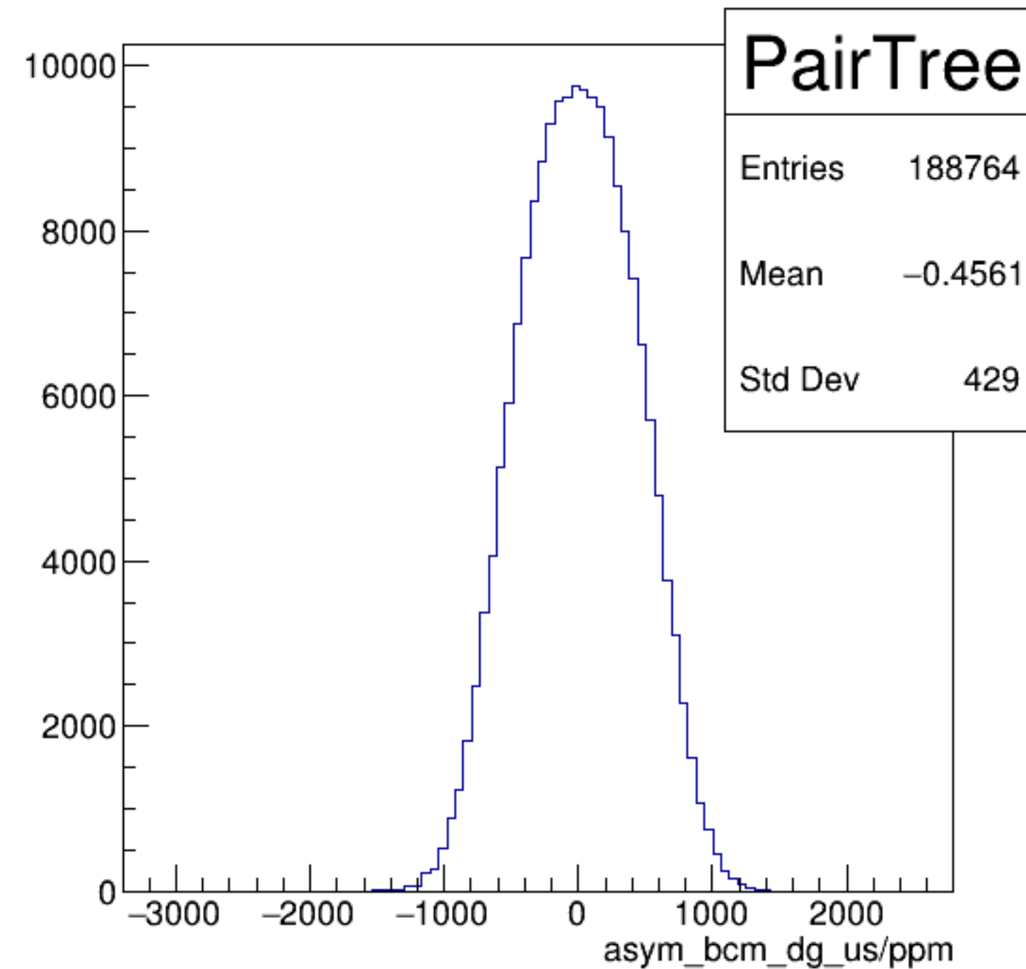
asym_bcm_dg_us/ppm {ErrorFlag==0}
