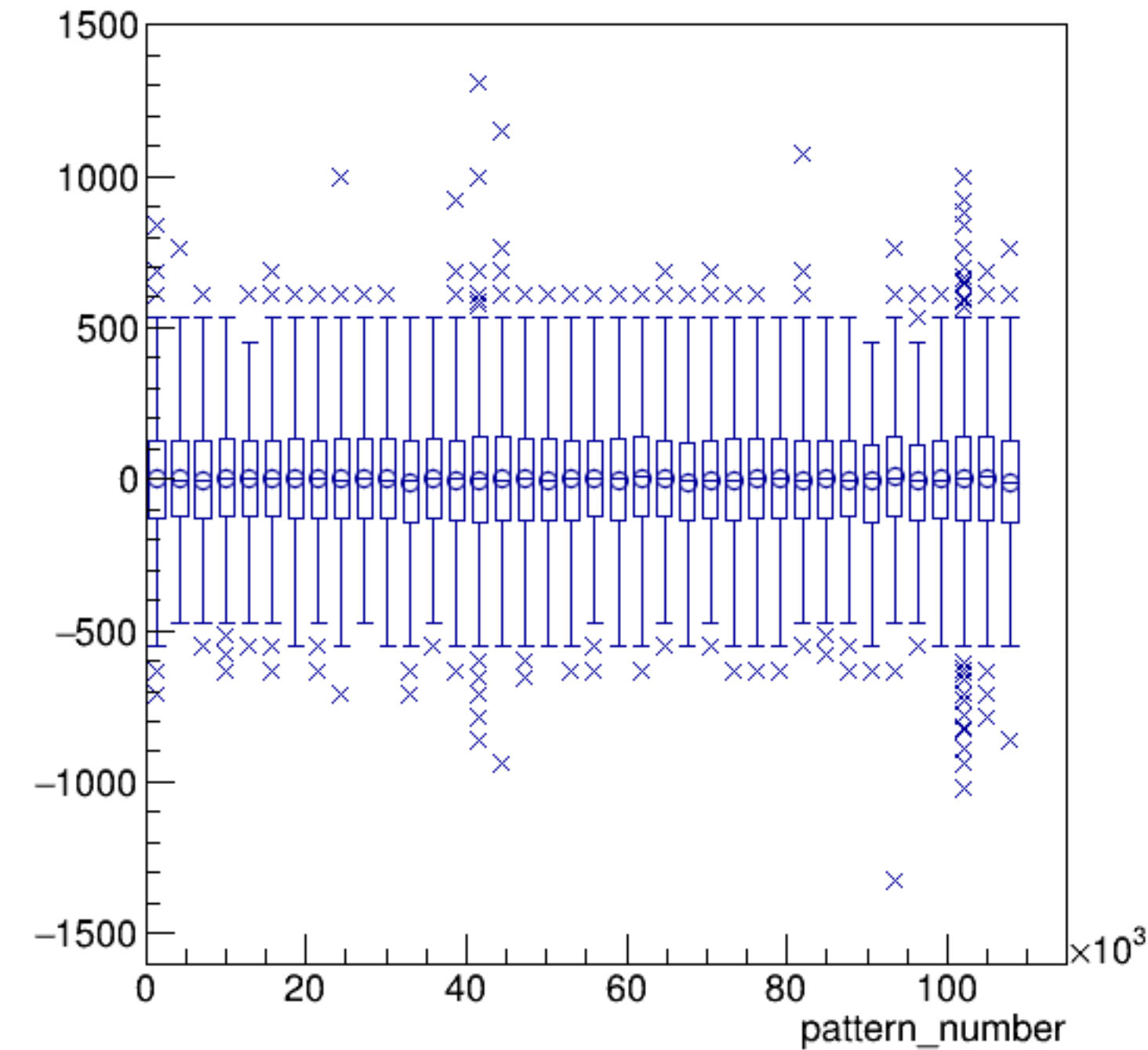
asym_bcm0l02/ppm:pattern_number {ErrorFlag==0}
