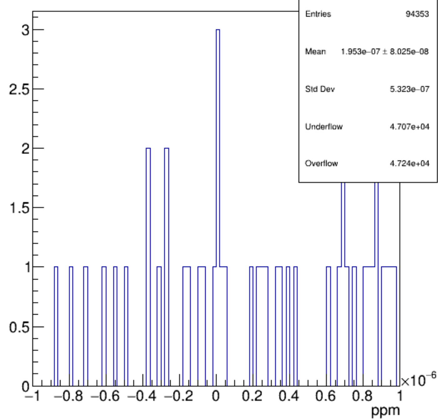
asym_bcm_an_diff
