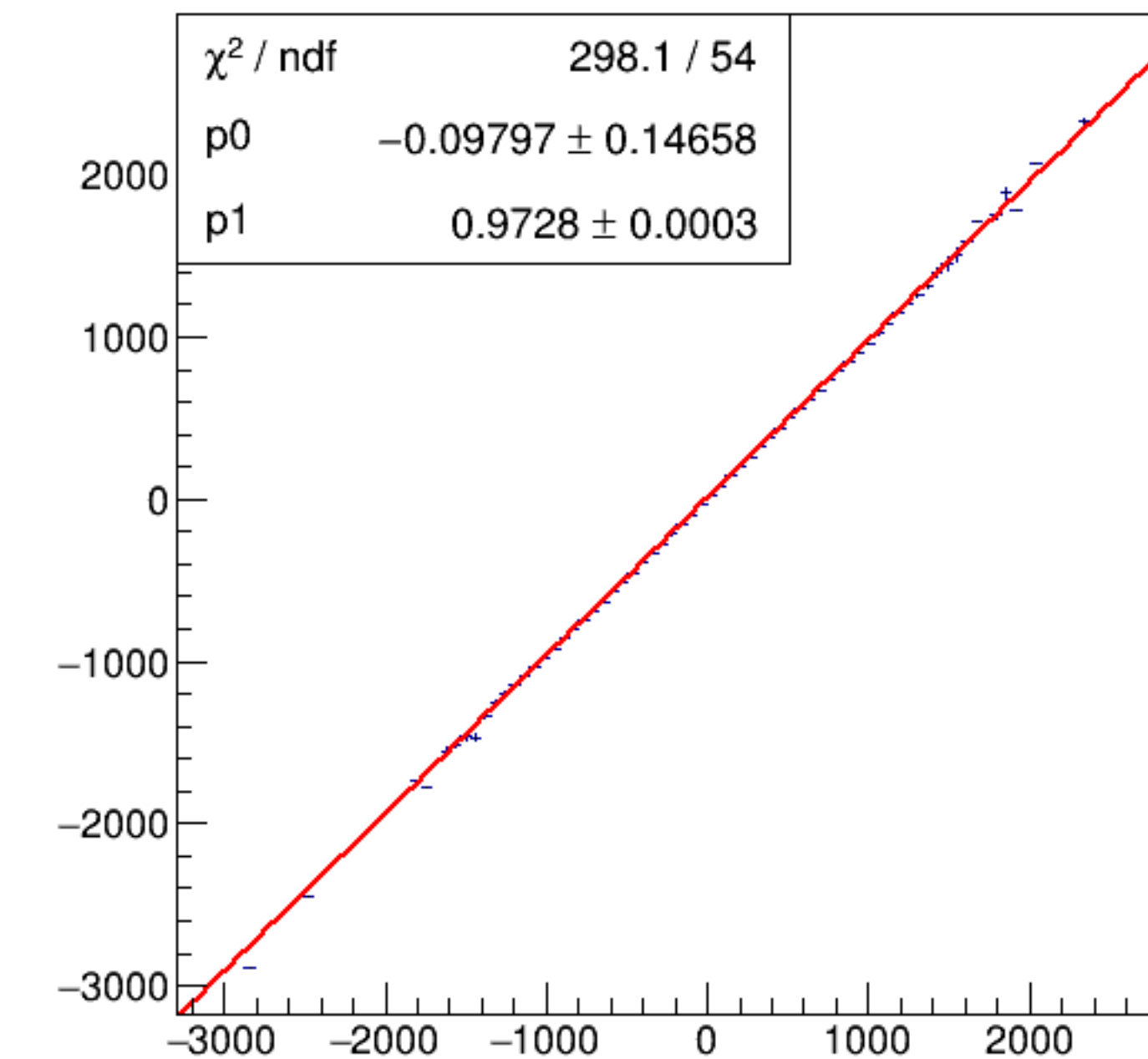
run7340_000_asym_bcm_dg_us_vs_asym_bcm_an_ds3_pr.png
