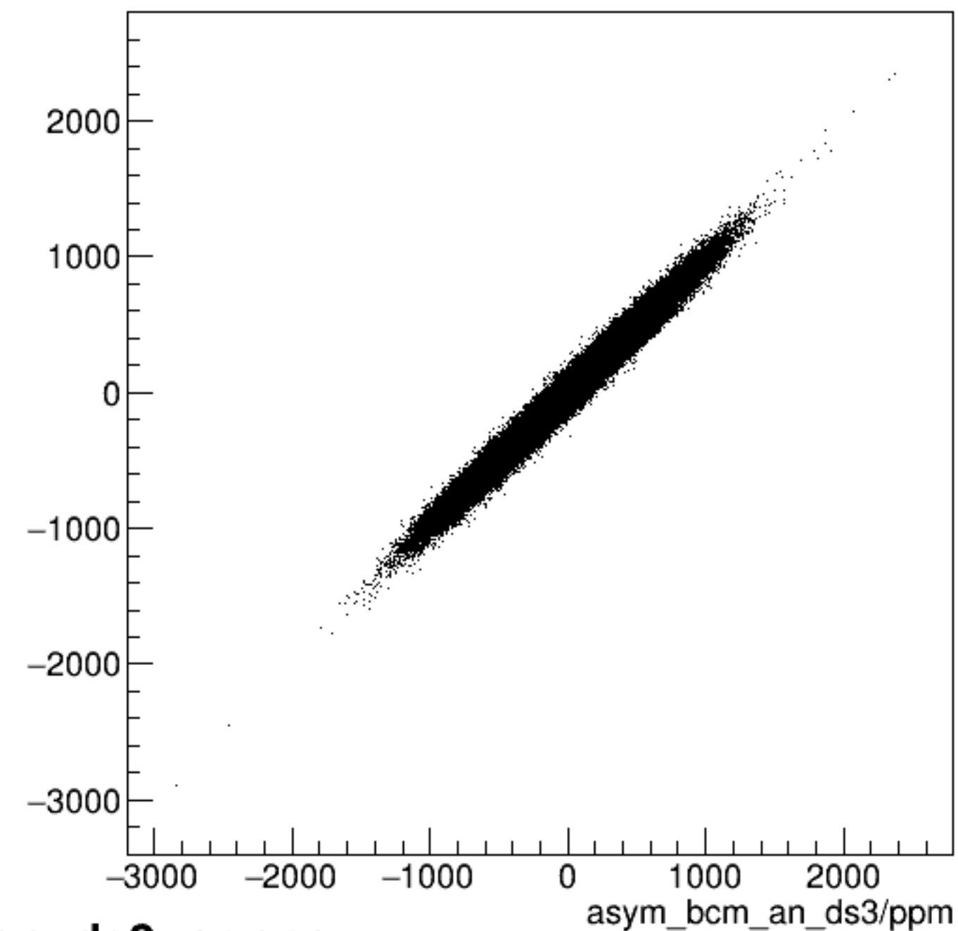
run7340_000_asym_bcm_dg_us_vs_asym_bcm_an_ds3_pr.png
