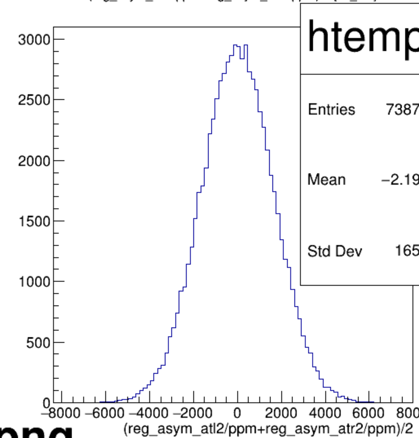
(reg_asym_atl2/ppm+reg_asym_atr2/ppm)/2 {ok_cut}
