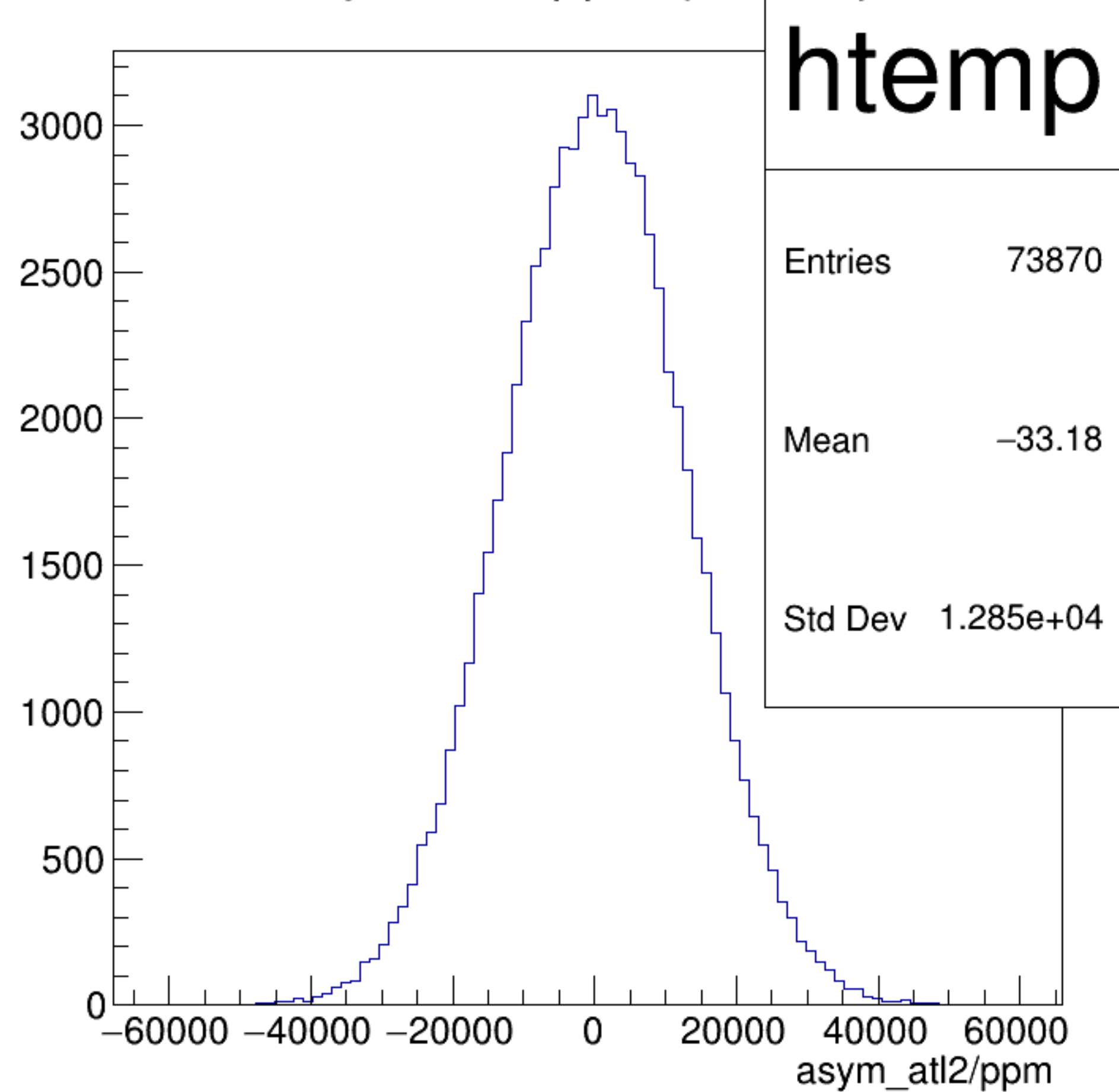
asym_atl2/ppm {ok_cut}
