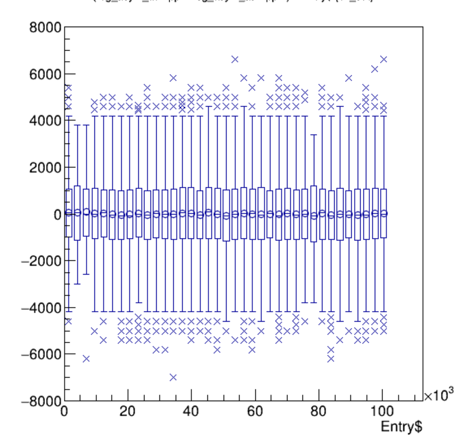
(reg_asym_atl2/ppm-reg_asym_atr2/ppm)/2:Entry$ {ok_cut}
