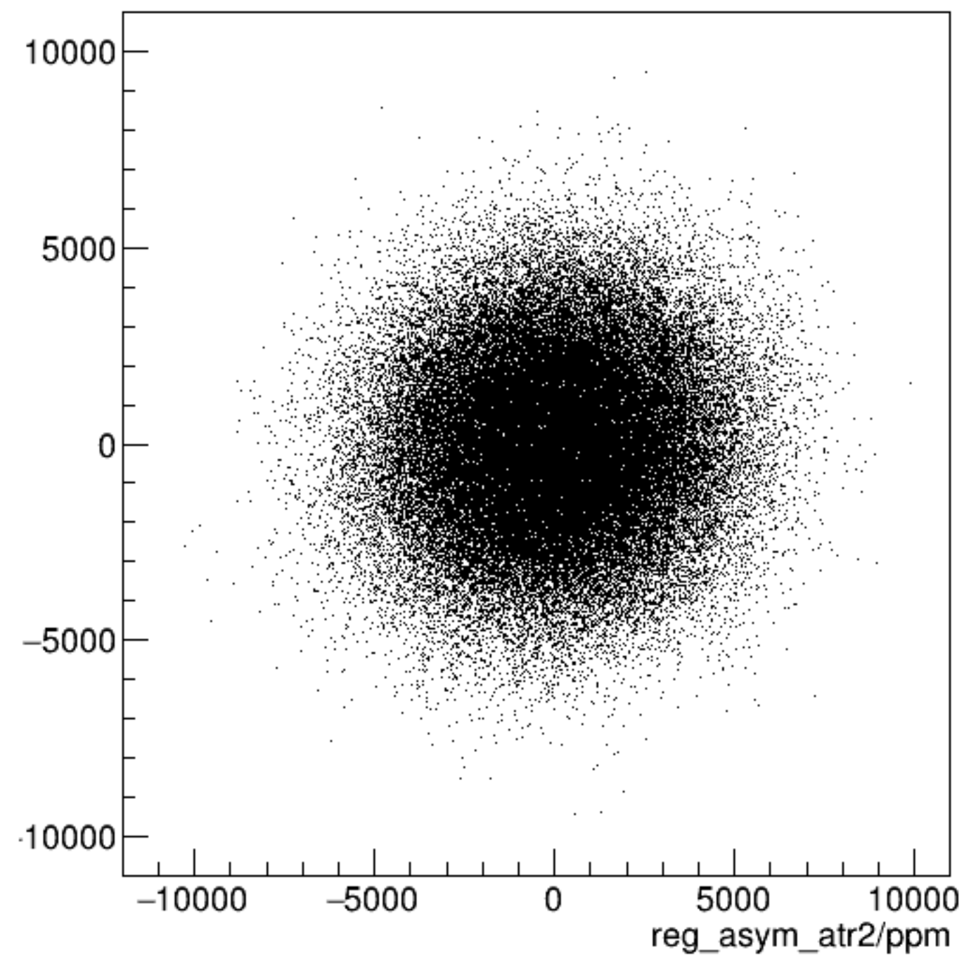
reg_asym_atl2/ppm:reg_asym_atr2/ppm {ok_cut}
