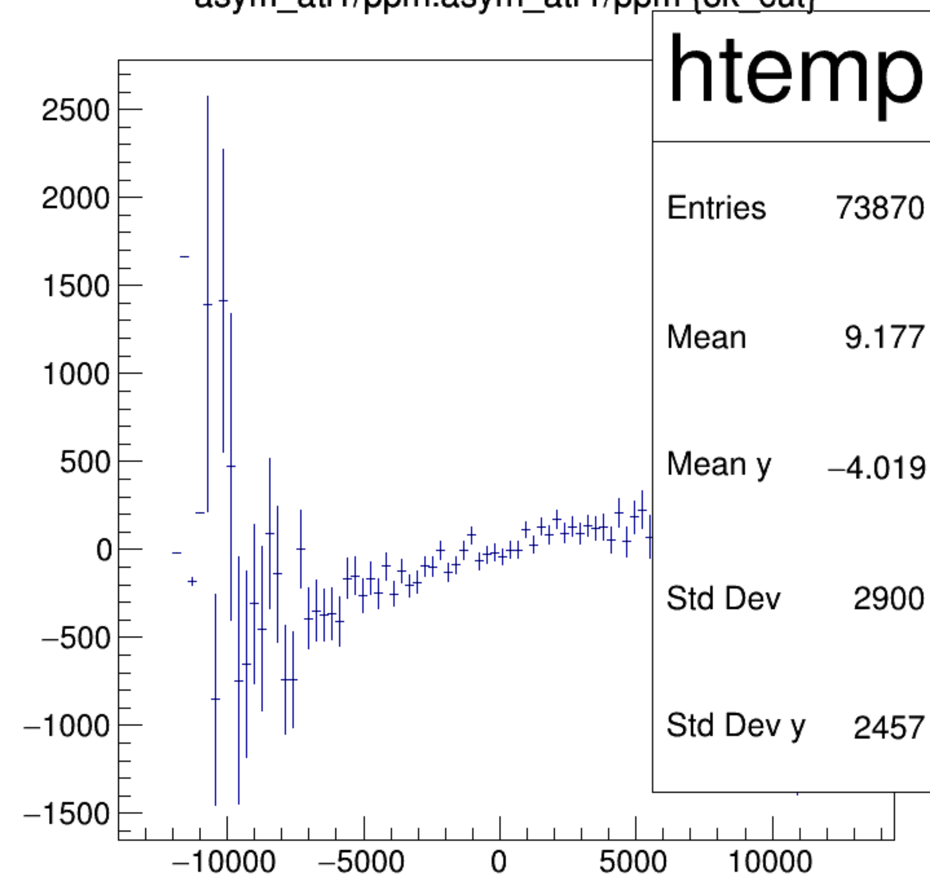
asym_atl1/ppm:asym_atr1/ppm {ok_cut}
