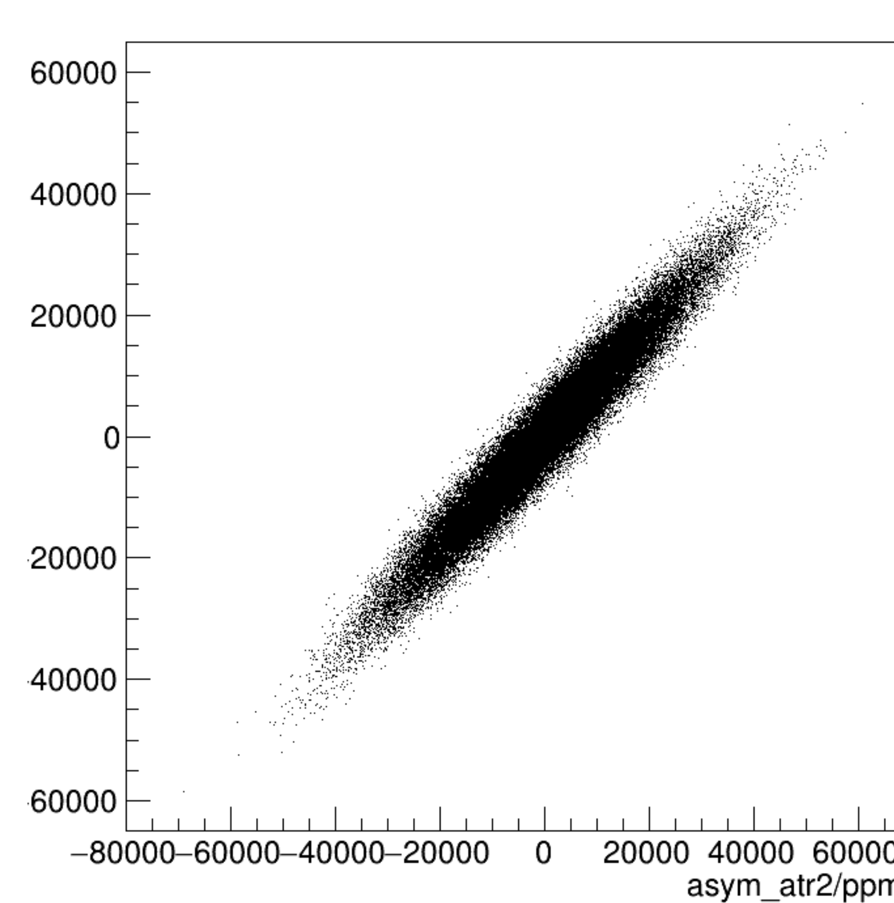
asym_atl2/ppm:asym_atr2/ppm {ok_cut}
