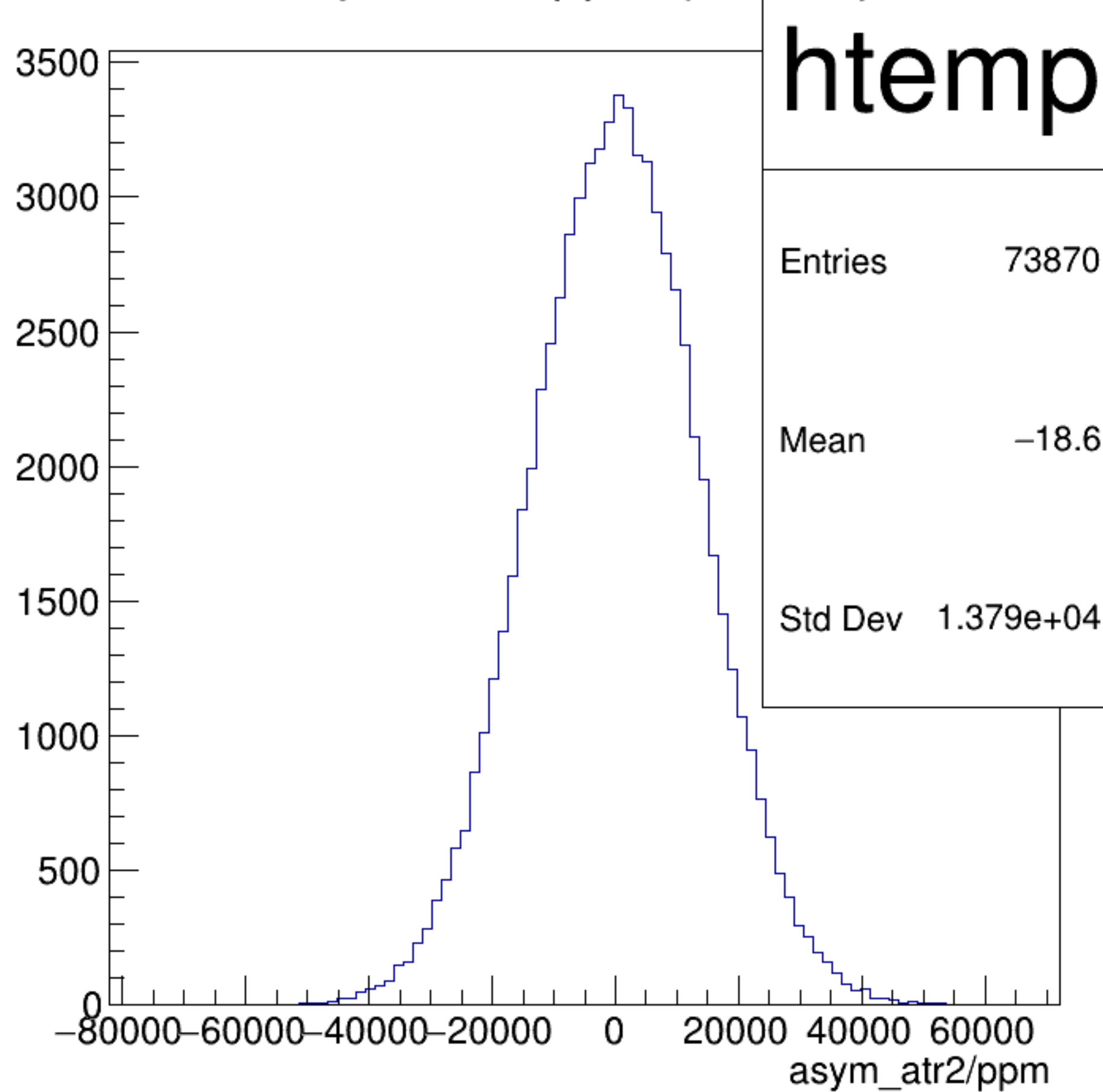
asym_atr2/ppm {ok_cut}
