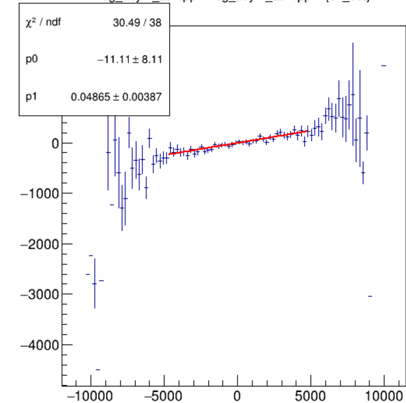
reg_asym_atl2/ppm:reg_asym_atr2/ppm {ok_cut}
