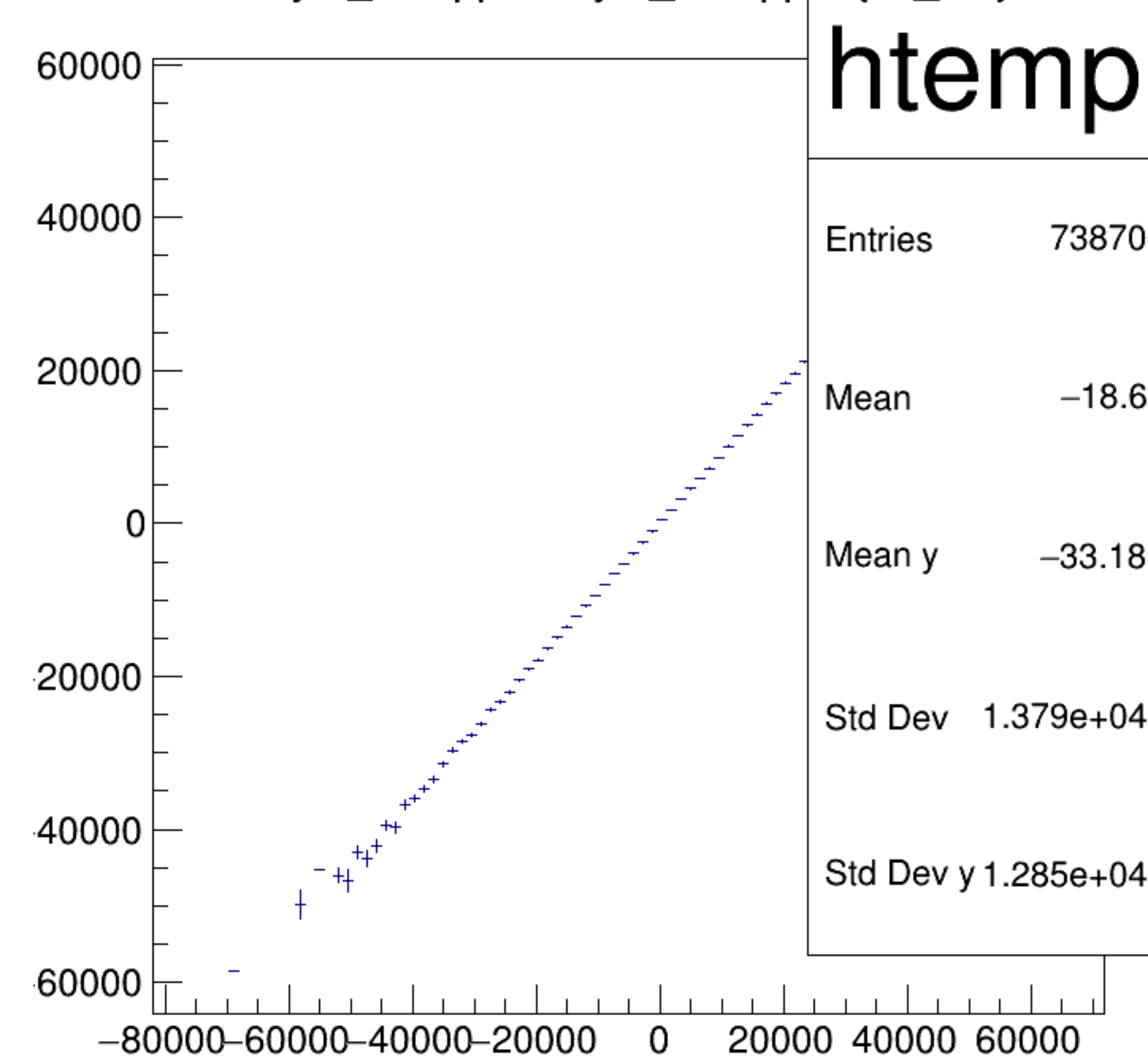
asym_atl2/ppm:asym_atr2/ppm {ok_cut}
