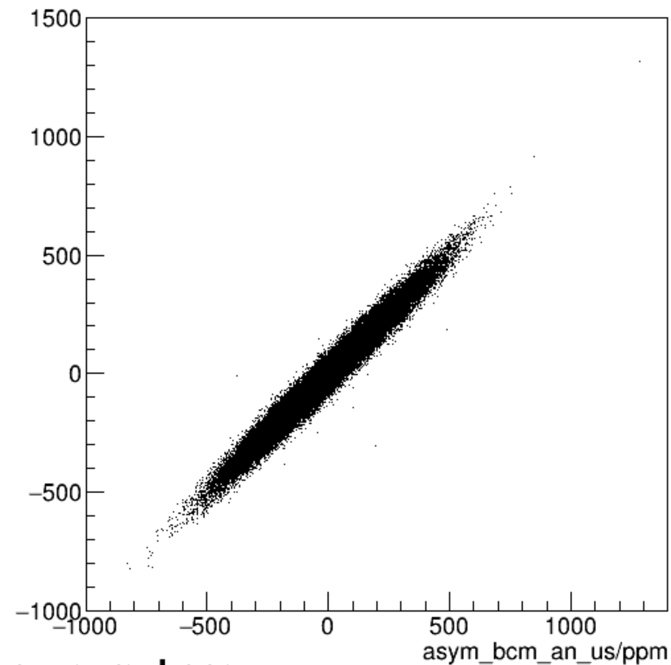
run7354_000_asym_bcm_dg_ds_vs_asym_bcm_an_us_mul.png
