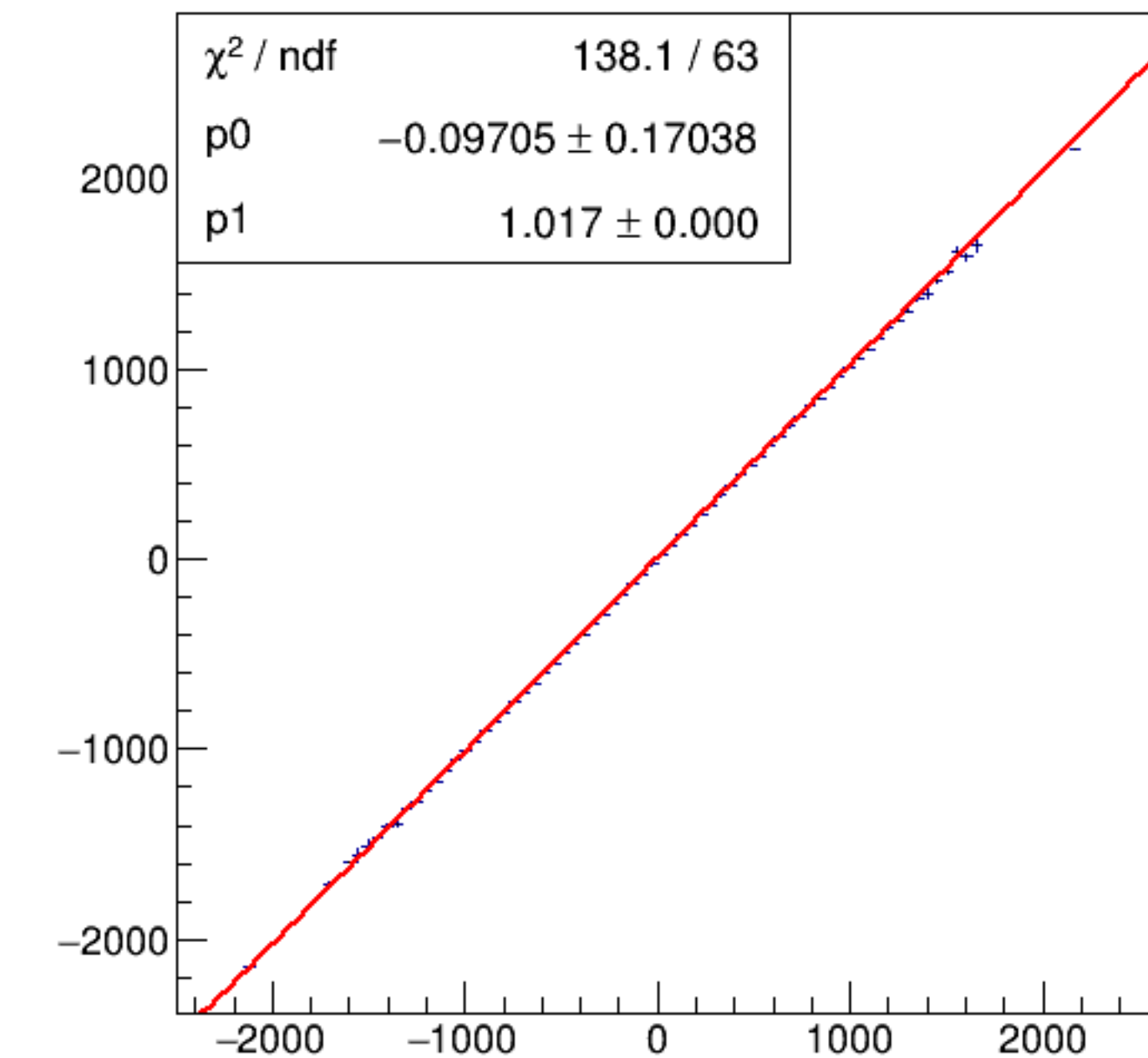
run7354_000_asym_bcm_dg_us_vs_asym_bcm_an_ds3_pr.png
