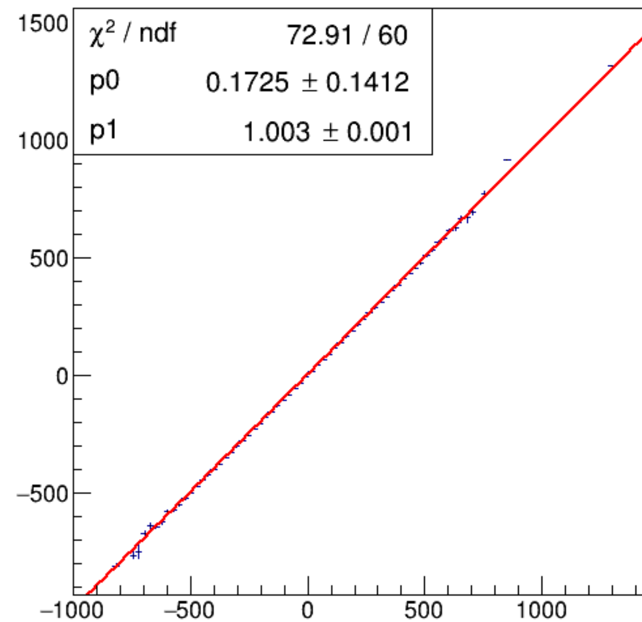
run7354_000_asym_bcm_dg_ds_vs_asym_bcm_an_us_mul.png
