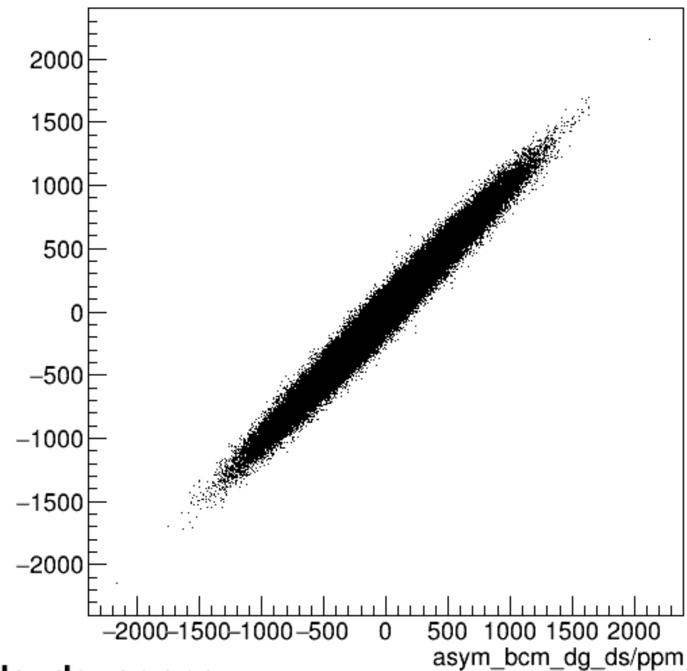
run7354_000_asym_bcm_dg_us_vs_asym_bcm_dg_ds_pr.png
