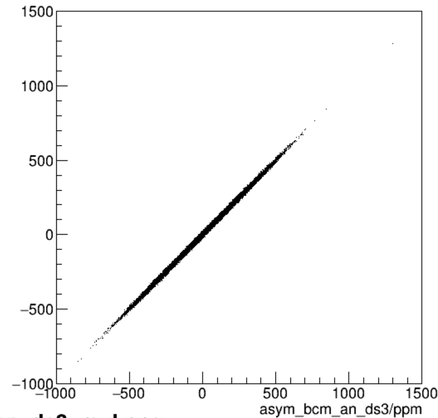
run7354_000_asym_bcm_an_ds_vs_asym_bcm_an_ds3_mul.png
