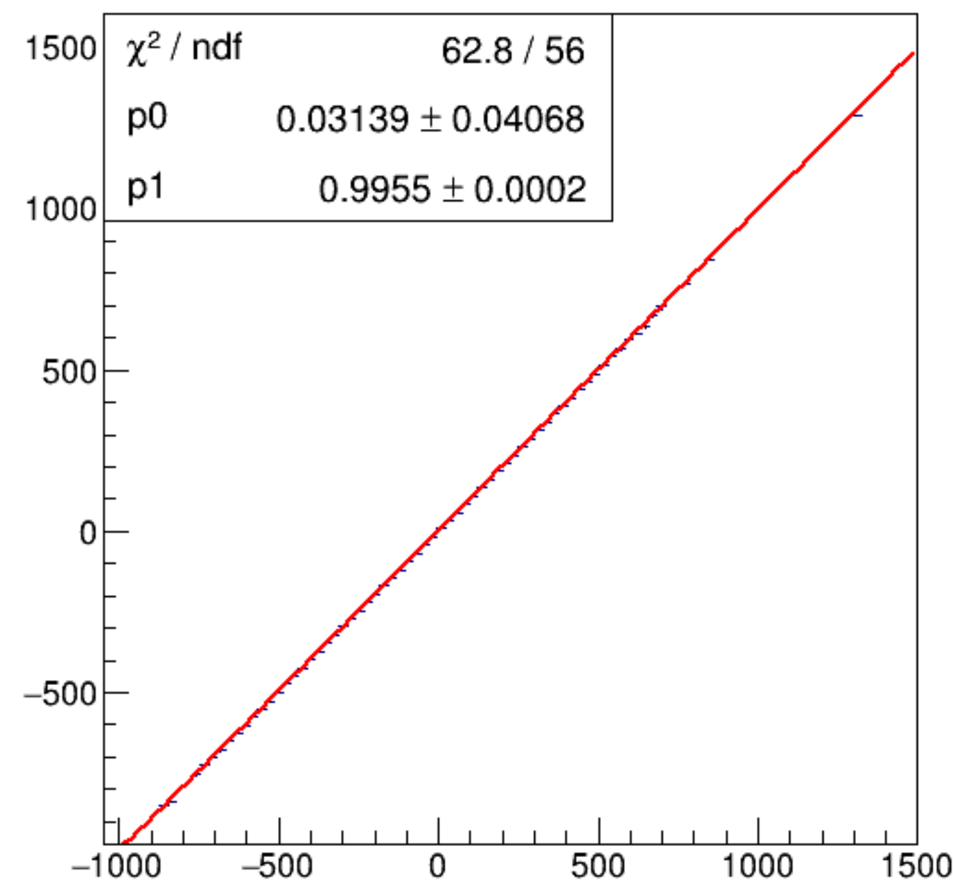
run7354_000_asym_bcm_an_ds_vs_asym_bcm_an_ds3_mul.png
