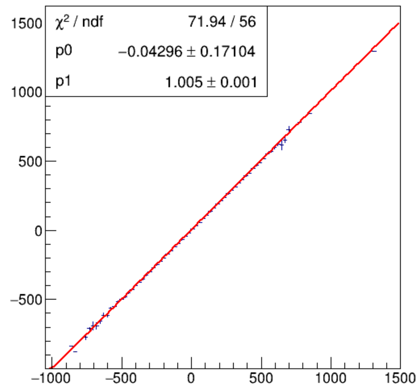
run7354_000_asym_bcm_dg_us_vs_asym_bcm_an_ds3_mul.png
