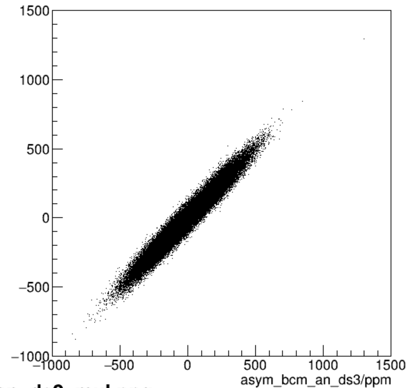
run7354_000_asym_bcm_dg_us_vs_asym_bcm_an_ds3_mul.png
