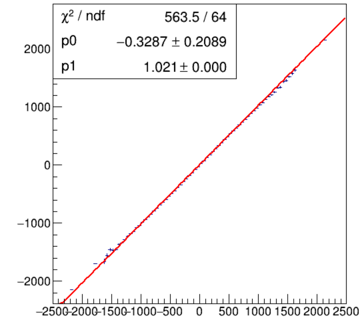
run7354_000_asym_bcm_dg_us_vs_asym_bcm_dg_ds_pr.png
