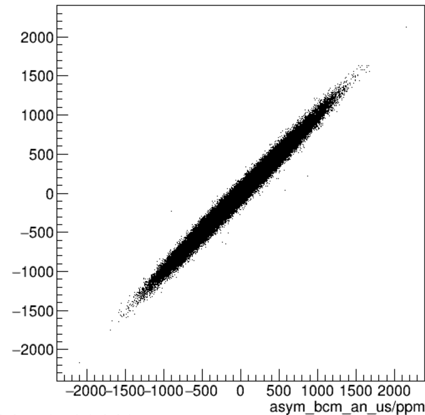
run7354_000_asym_bcm_dg_ds_vs_asym_bcm_an_us_pr.png
