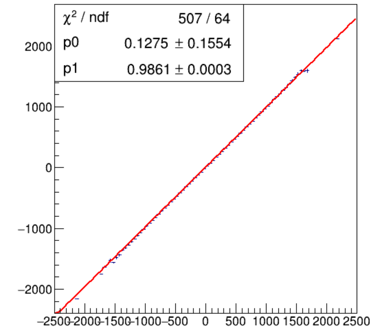
run7354_000_asym_bcm_dg_ds_vs_asym_bcm_an_us_pr.png
