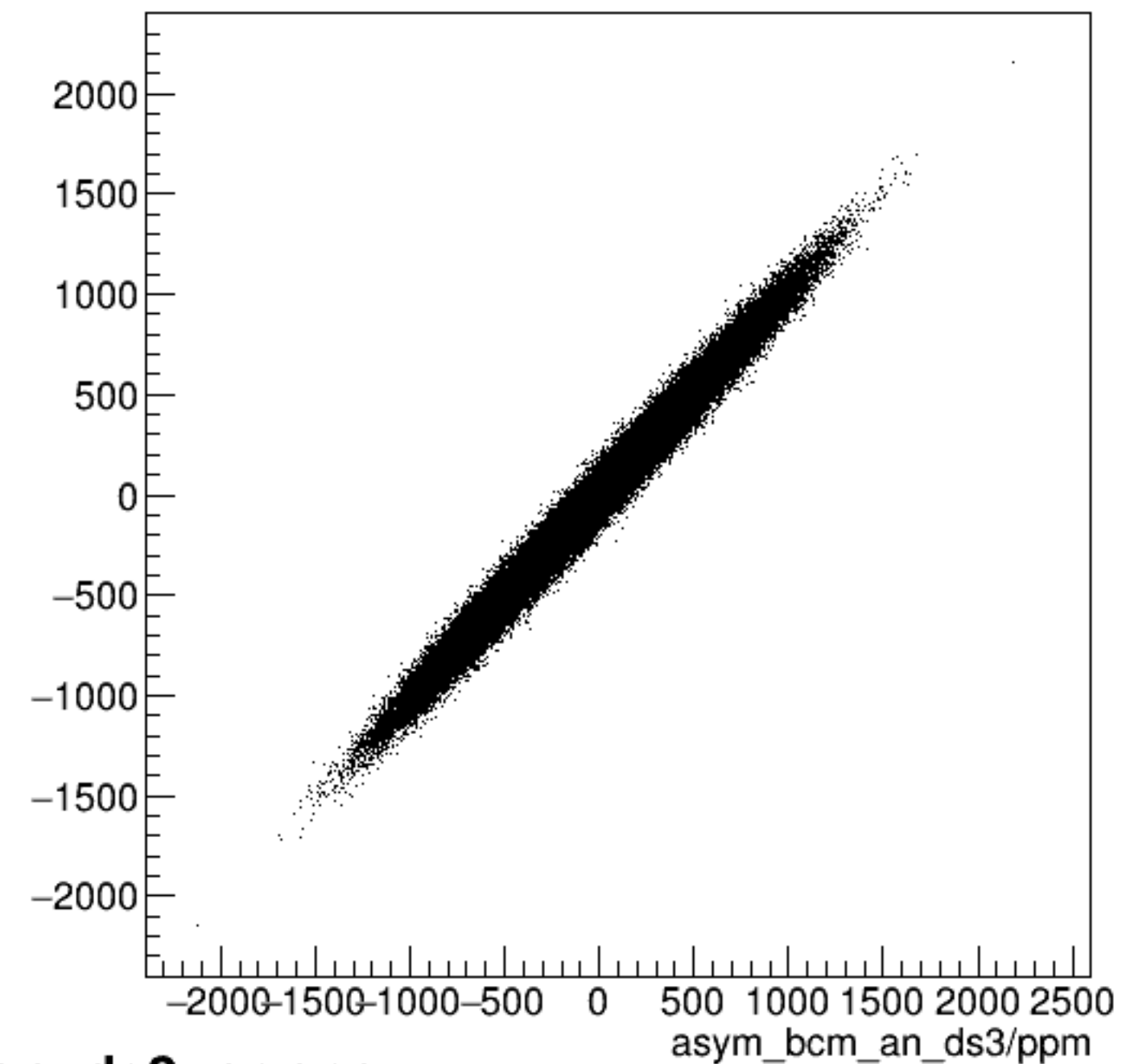
run7354_000_asym_bcm_dg_us_vs_asym_bcm_an_ds3_pr.png
