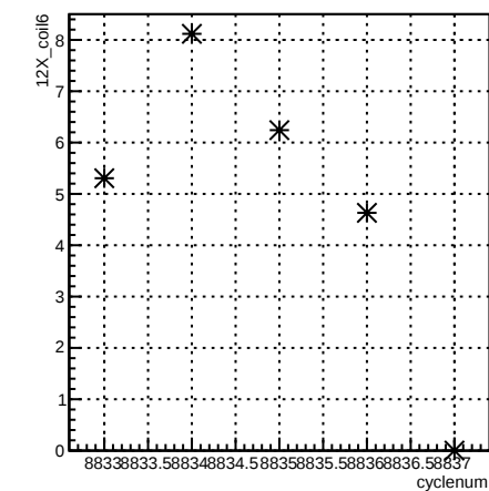
12X_coil6:cyclenum {run == 7355}
