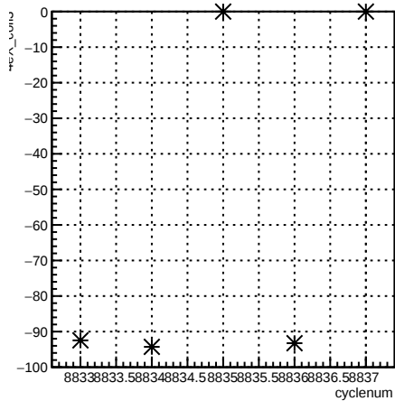
4eX_coil3:cyclenum {run == 7355}
