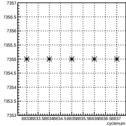
run:cyclenum {run == 7355}
