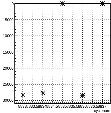
usr_coil1:cyclenum {run == 7355}
