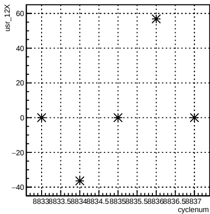
usr_12X:cyclenum {run == 7355}
