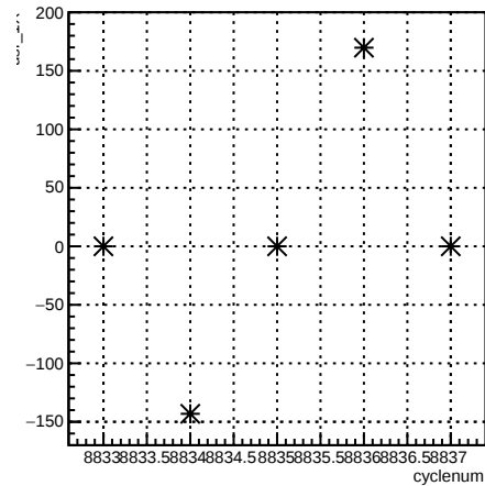
usr_1X:cyclenum {run == 7355}
