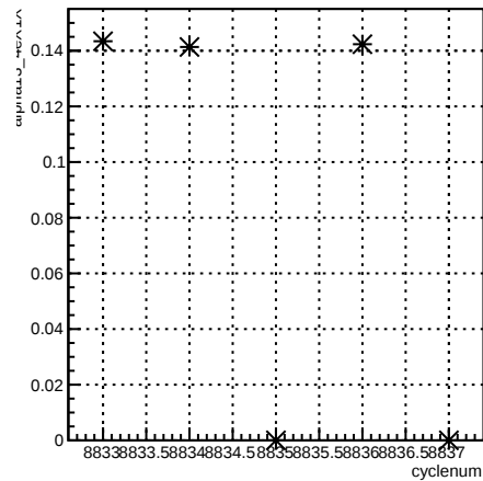
delta46_12X4eY:cyclenum {run == 7355}
