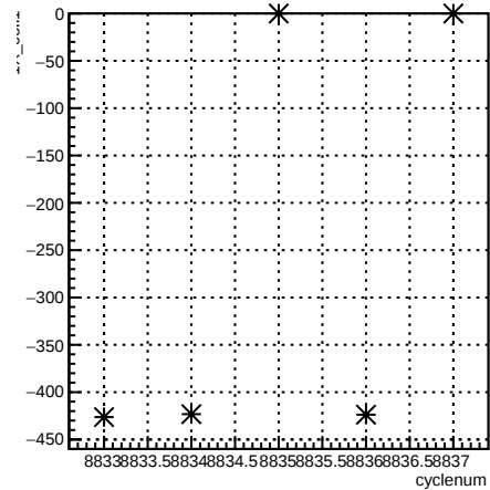
1X_coil1:cyclenum {run == 7355}
