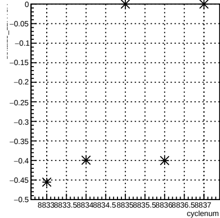
segment:cyclenum {run == 7355}
