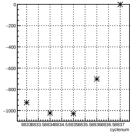
usr_coil6:cyclenum {run == 7355}
