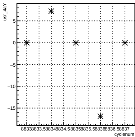
usr_4aY:cyclenum {run == 7355}
