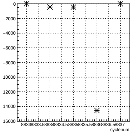
12X_coil7:cyclenum {run == 7355}
