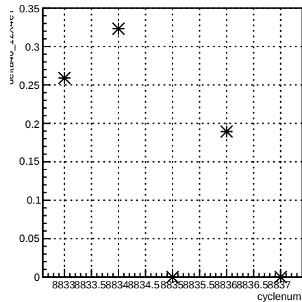
delta46_12X4eY:cyclenum {run == 7355}
