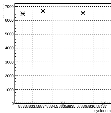
usl_coil3:cyclenum {run == 7355}
