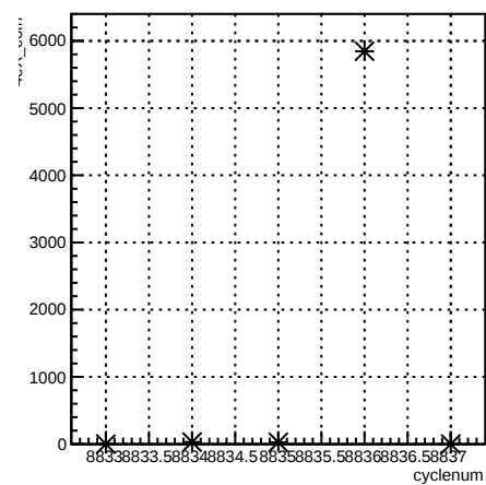
4eX_coil7:cyclenum {run == 7355}
