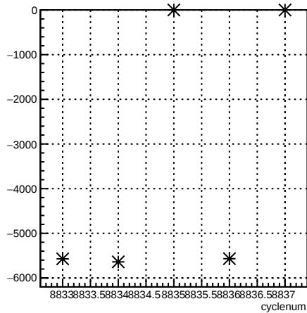
usr_coil3:cyclenum {run == 7355}
