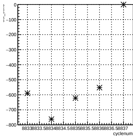
usl_coil6:cyclenum {run == 7355}
