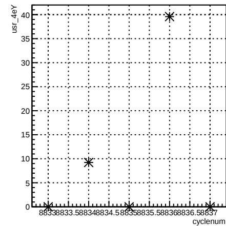
usr_4eY:cyclenum {run == 7355}
