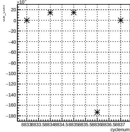
usl_coil7:cyclenum {run == 7355}
