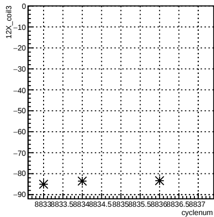
12X_coil3:cyclenum {run == 7355}
