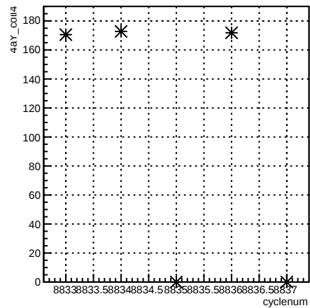
4aY_coil4:cyclenum {run == 7355}
