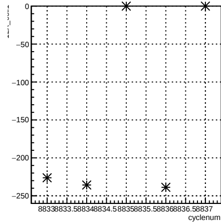
12X_coil1:cyclenum {run == 7355}
