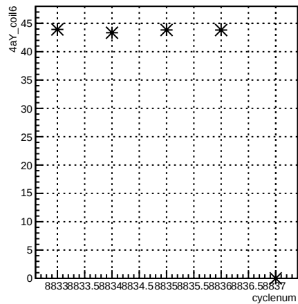
4aY_coil6:cyclenum {run == 7355}
