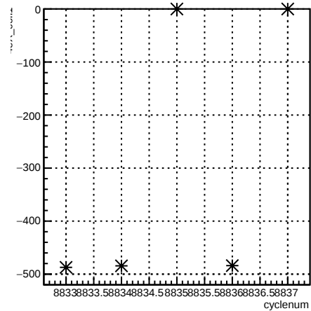
4eX_coil1:cyclenum {run == 7355}
