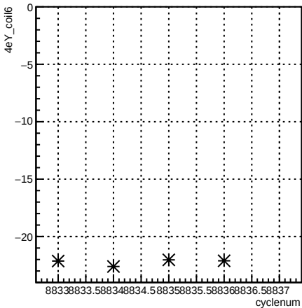
4eY_coil6:cyclenum {run == 7355}
