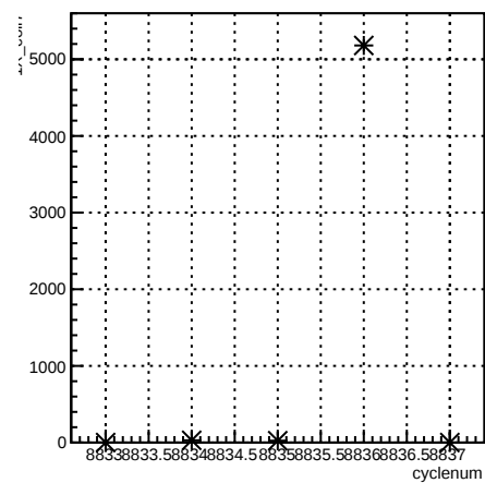
1X_coil7:cyclenum {run == 7355}
