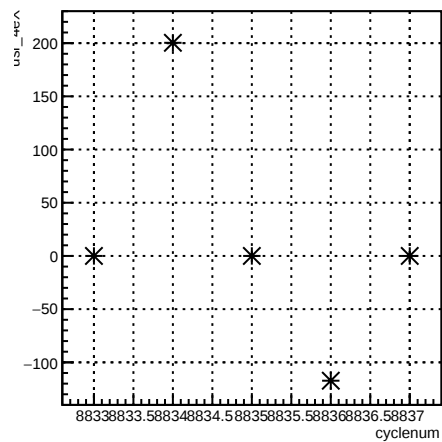
usr_4eX:cyclenum {run == 7355}
