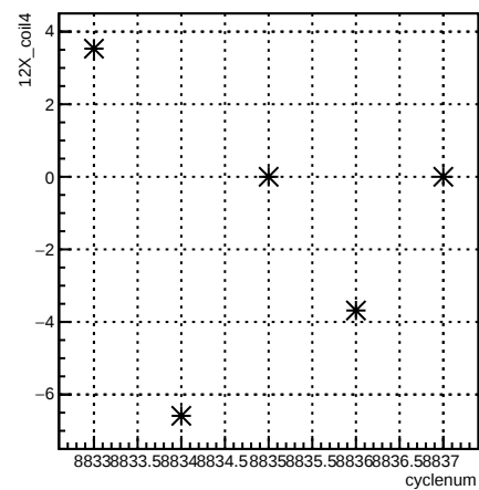
12X_coil4:cyclenum {run == 7355}
