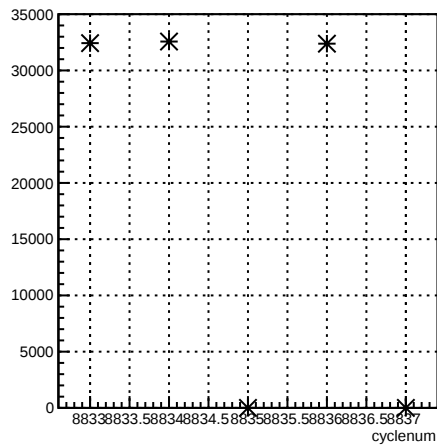
usl_coil1:cyclenum {run == 7355}
