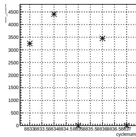
usr_coil4:cyclenum {run == 7355}
