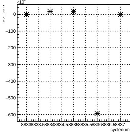
usr_coil7:cyclenum {run == 7355}
