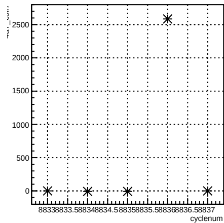
4aY_coil7:cyclenum {run == 7355}
