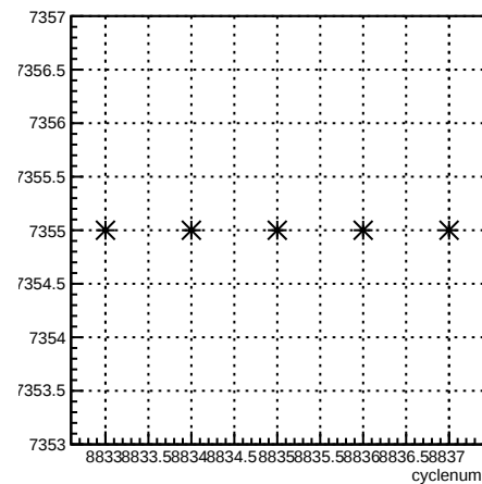
run:cyclenum {run == 7355}
