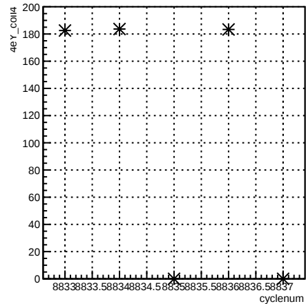
4eY_coil4:cyclenum {run == 7355}
