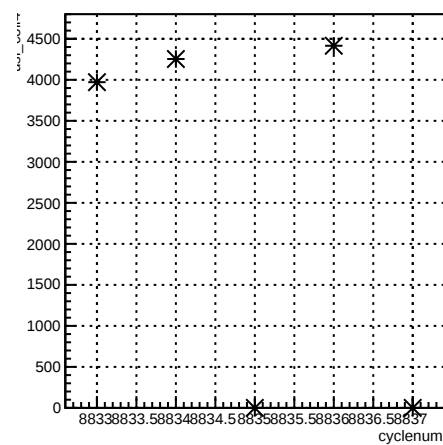
usl_coil4:cyclenum {run == 7355}
