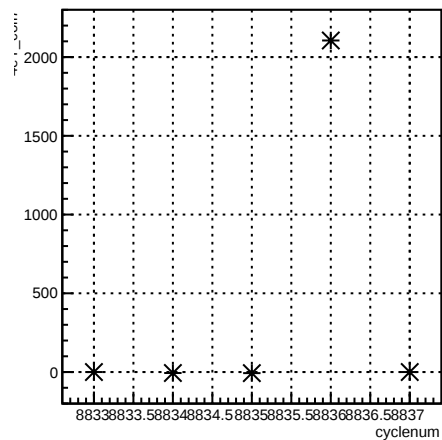
4eY_coil7:cyclenum {run == 7355}
