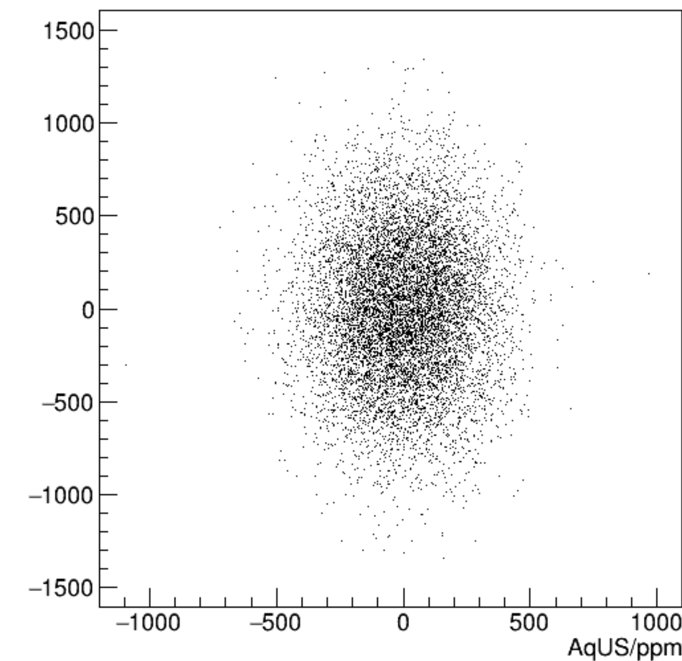
reg_asym_dsr/ppm:AqUS/ppm {ok_cut}
