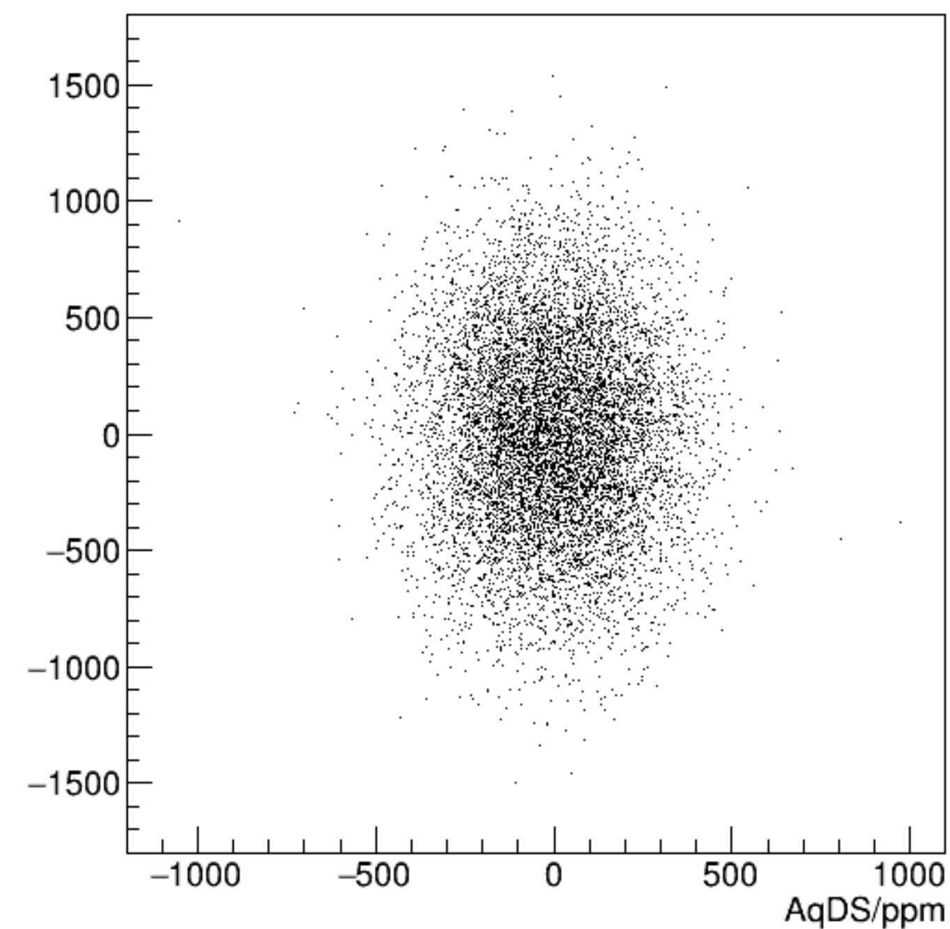
reg_asym_dsl/ppm:AqDS/ppm {ok_cut}
