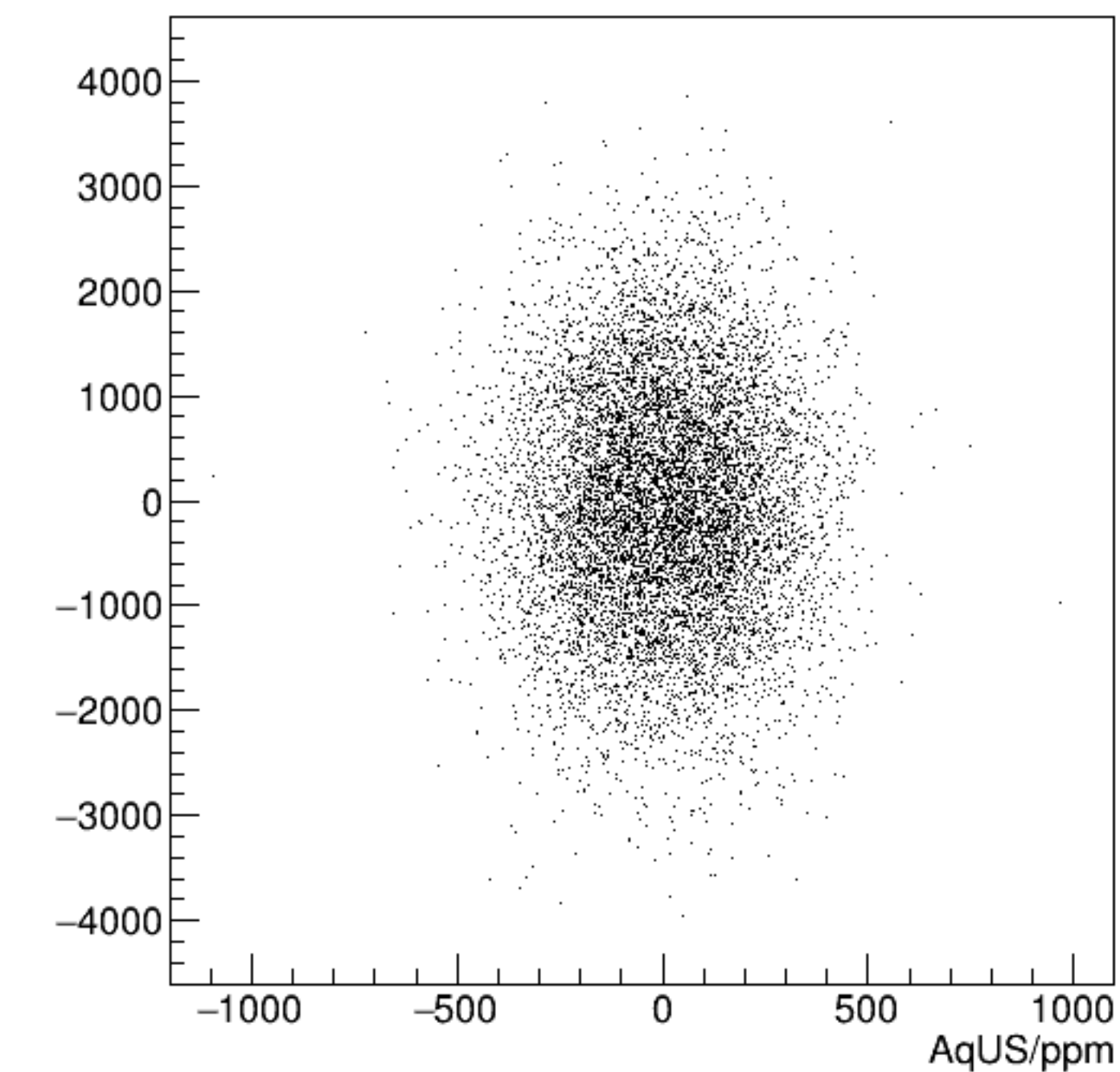
reg_asym_usl/ppm:AqUS/ppm {ok_cut}
