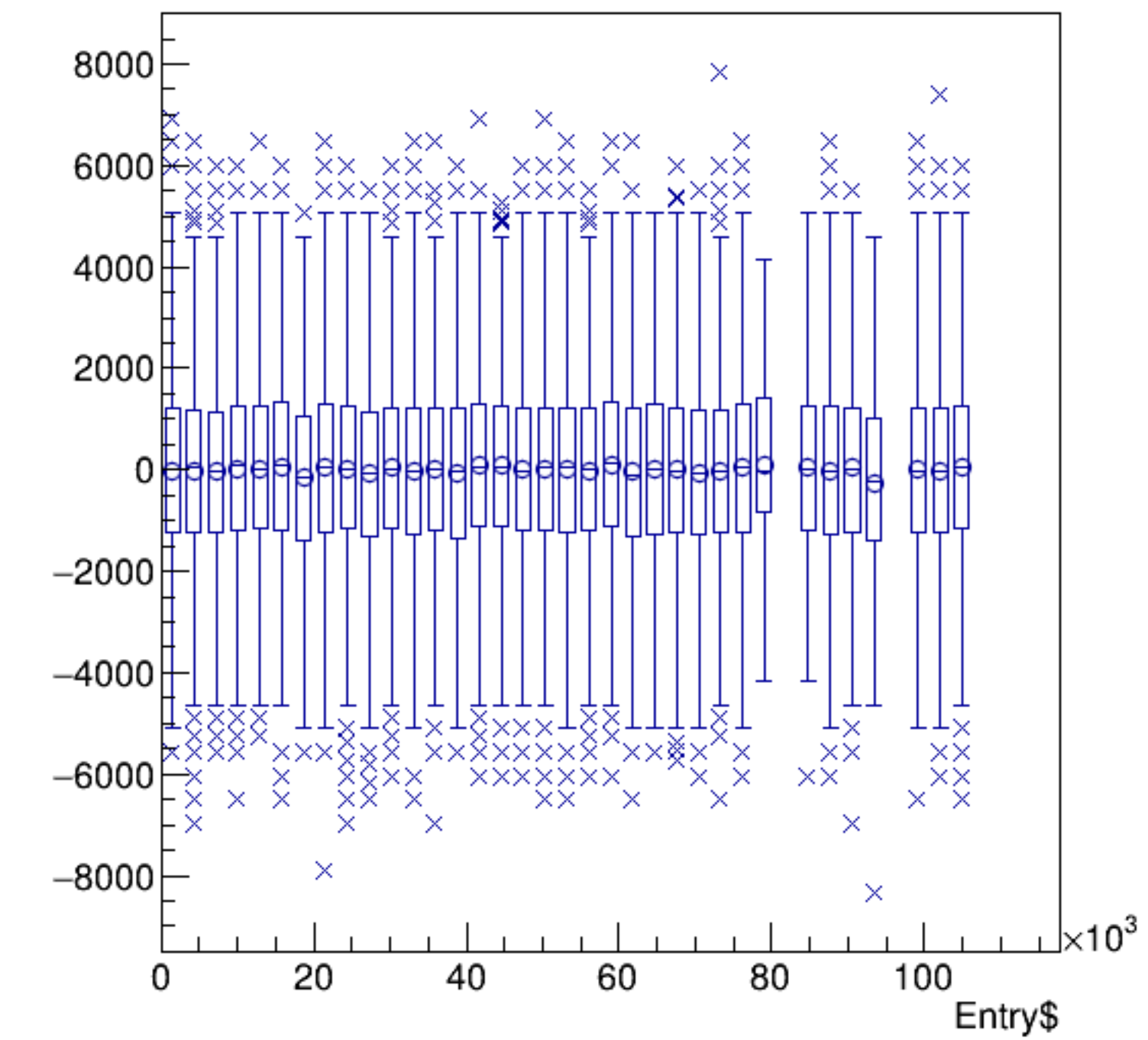
(reg_asym_atl1/ppm+reg_asym_atr1/ppm)/2:Entry$ {ok_cut}
