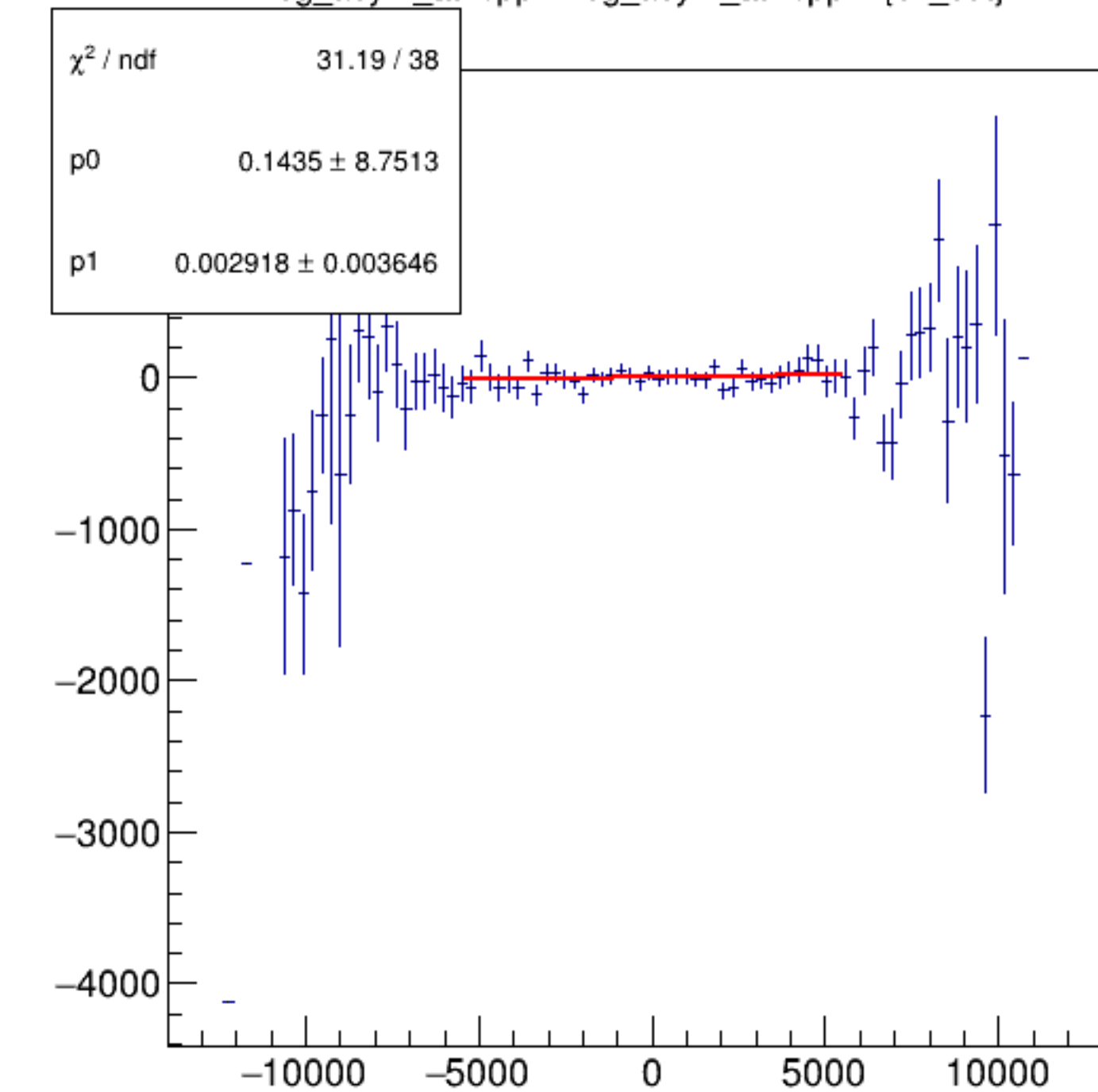
reg_asym_atl1/ppm:reg_asym_atr1/ppm {ok_cut}
