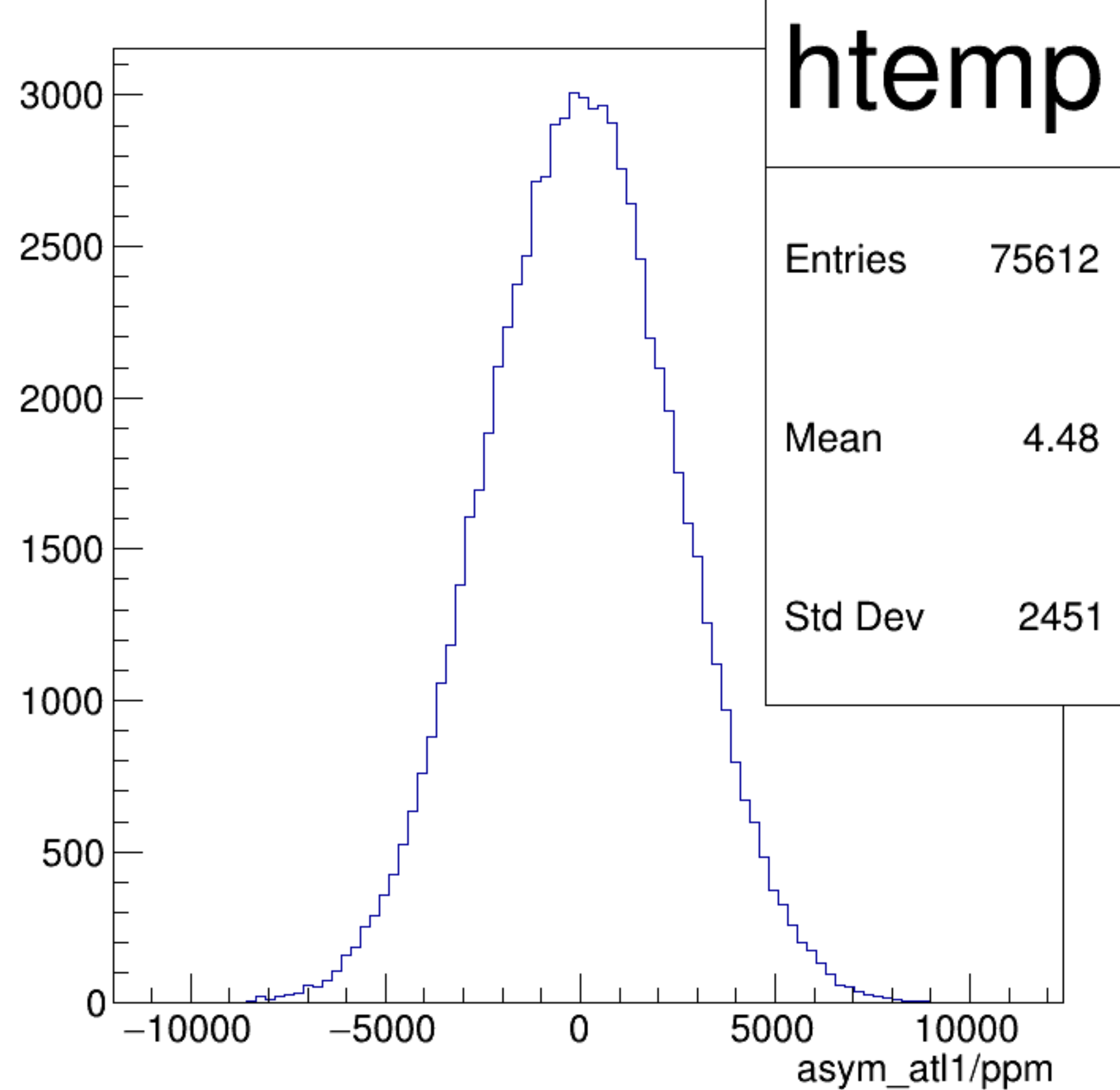
asym_atl1/ppm {ok_cut}
