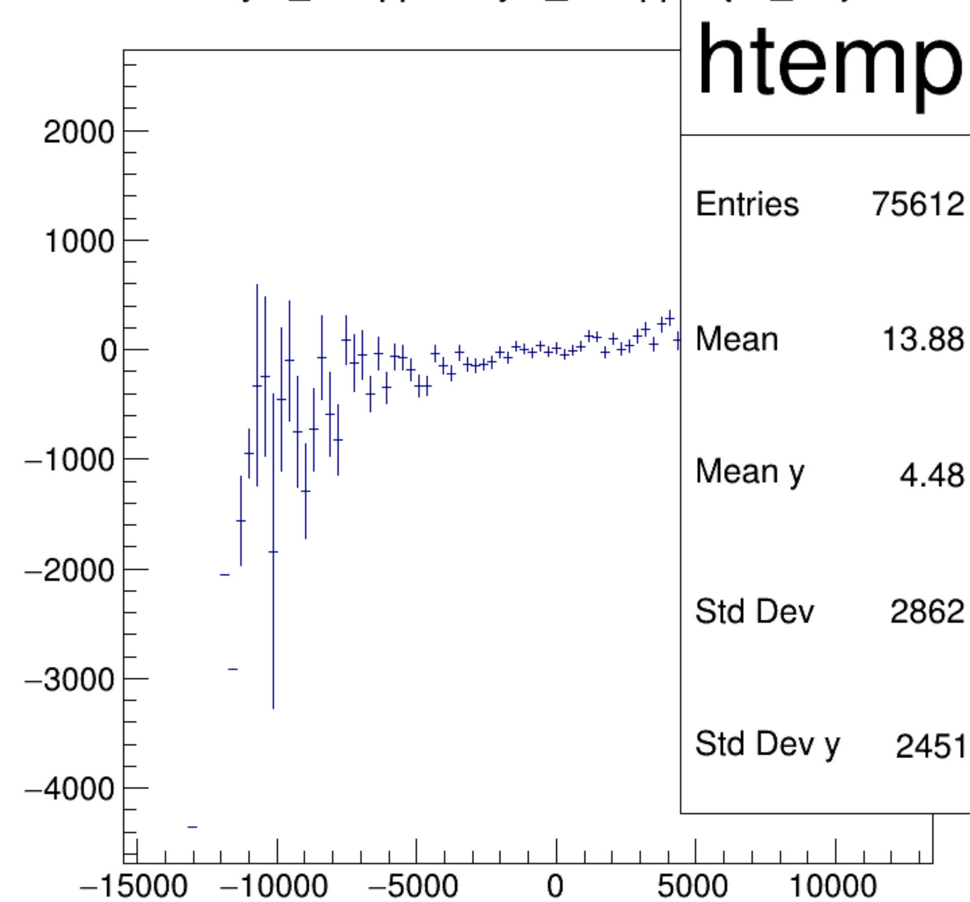
asym_atl1/ppm:asym_atr1/ppm {ok_cut}
