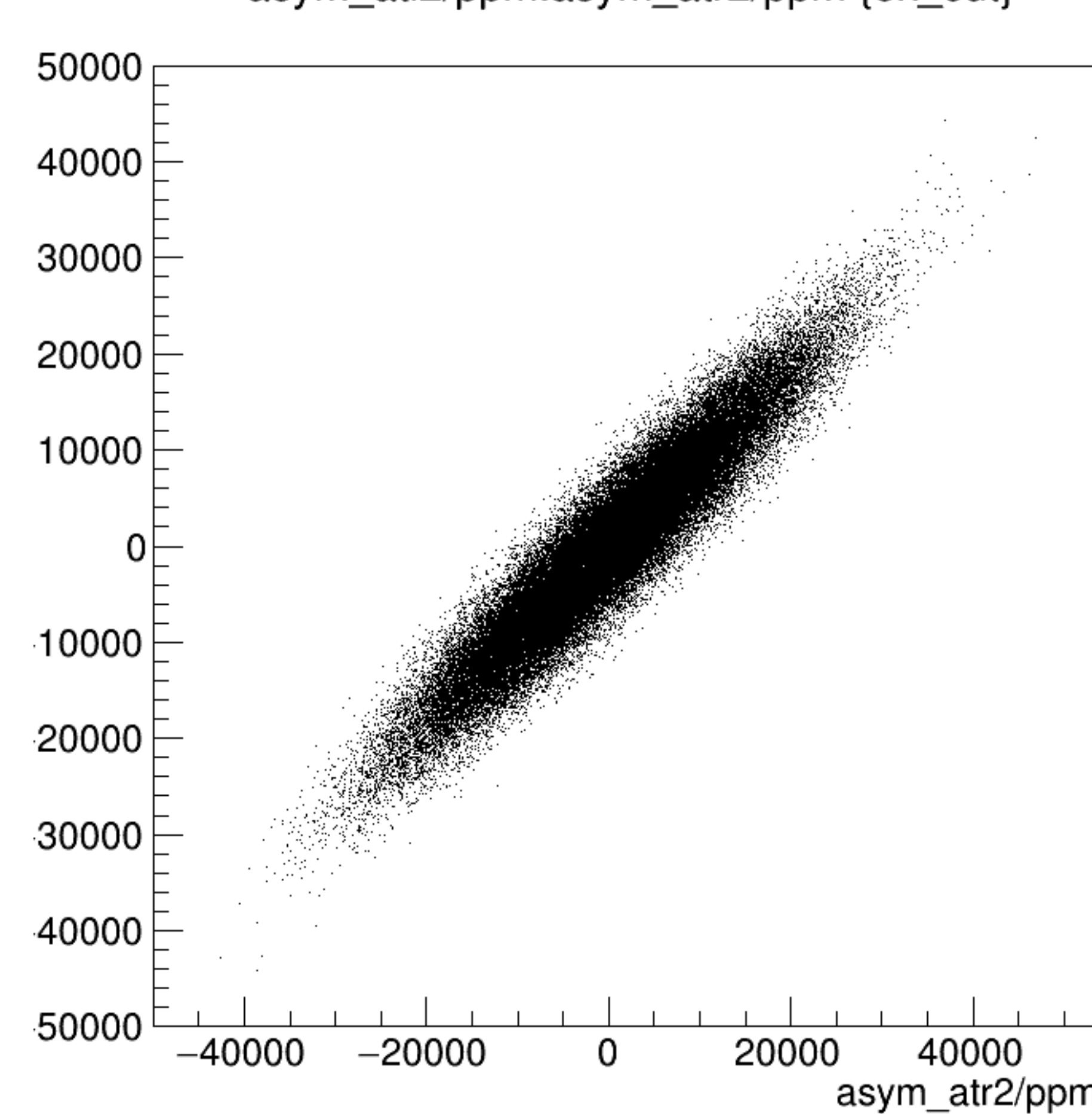
asym_atl2/ppm:asym_atr2/ppm {ok_cut}
