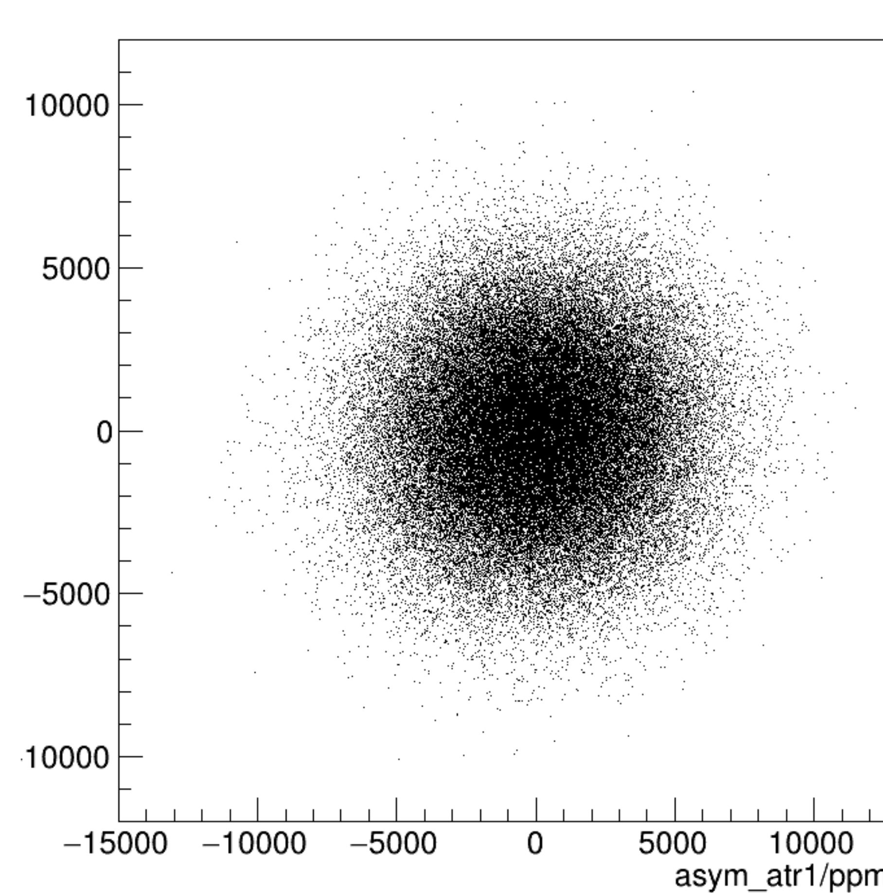
asym_atl1/ppm:asym_atr1/ppm {ok_cut}
