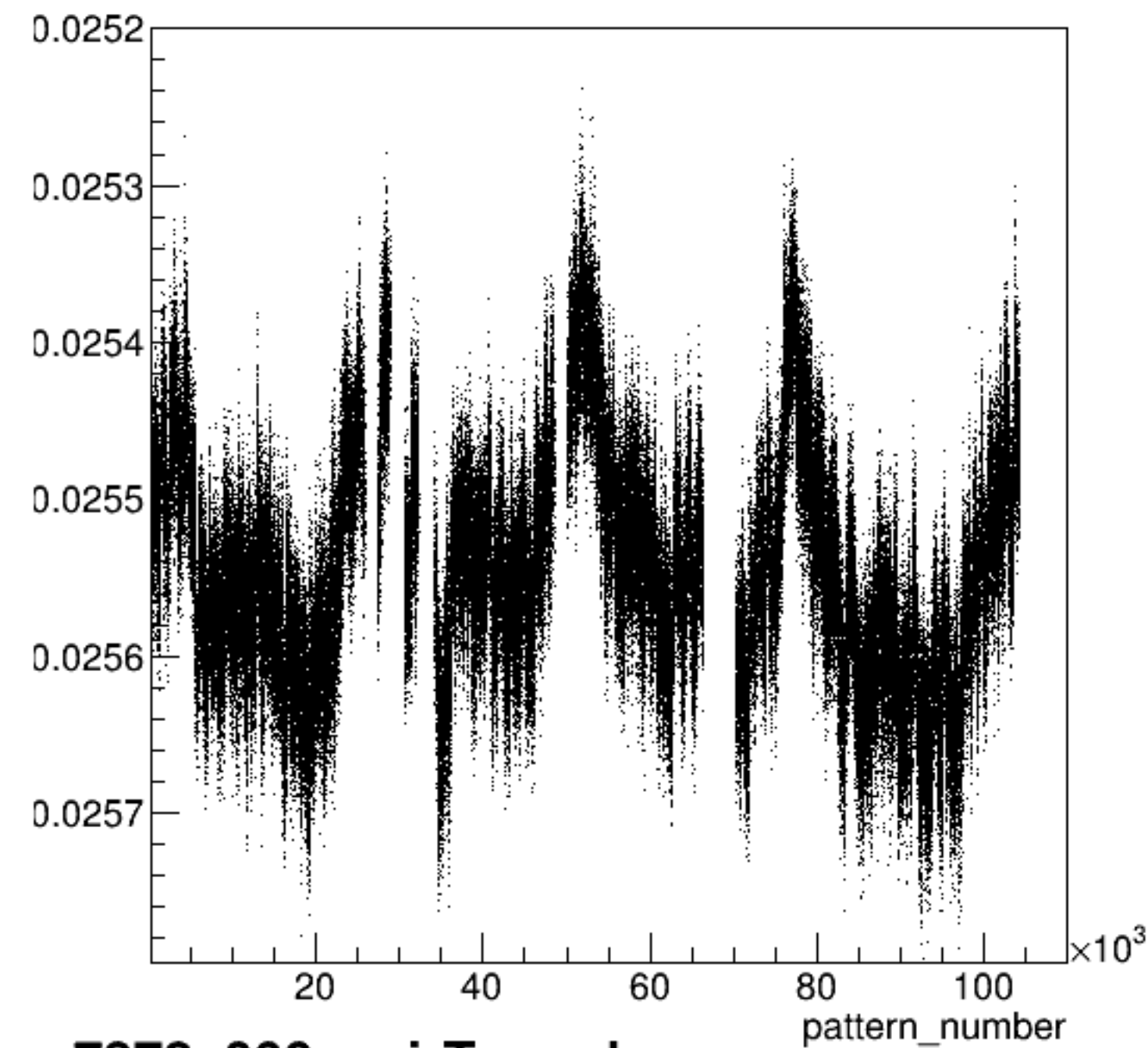
yield_dsr:pattern_number {ErrorFlag==0}
