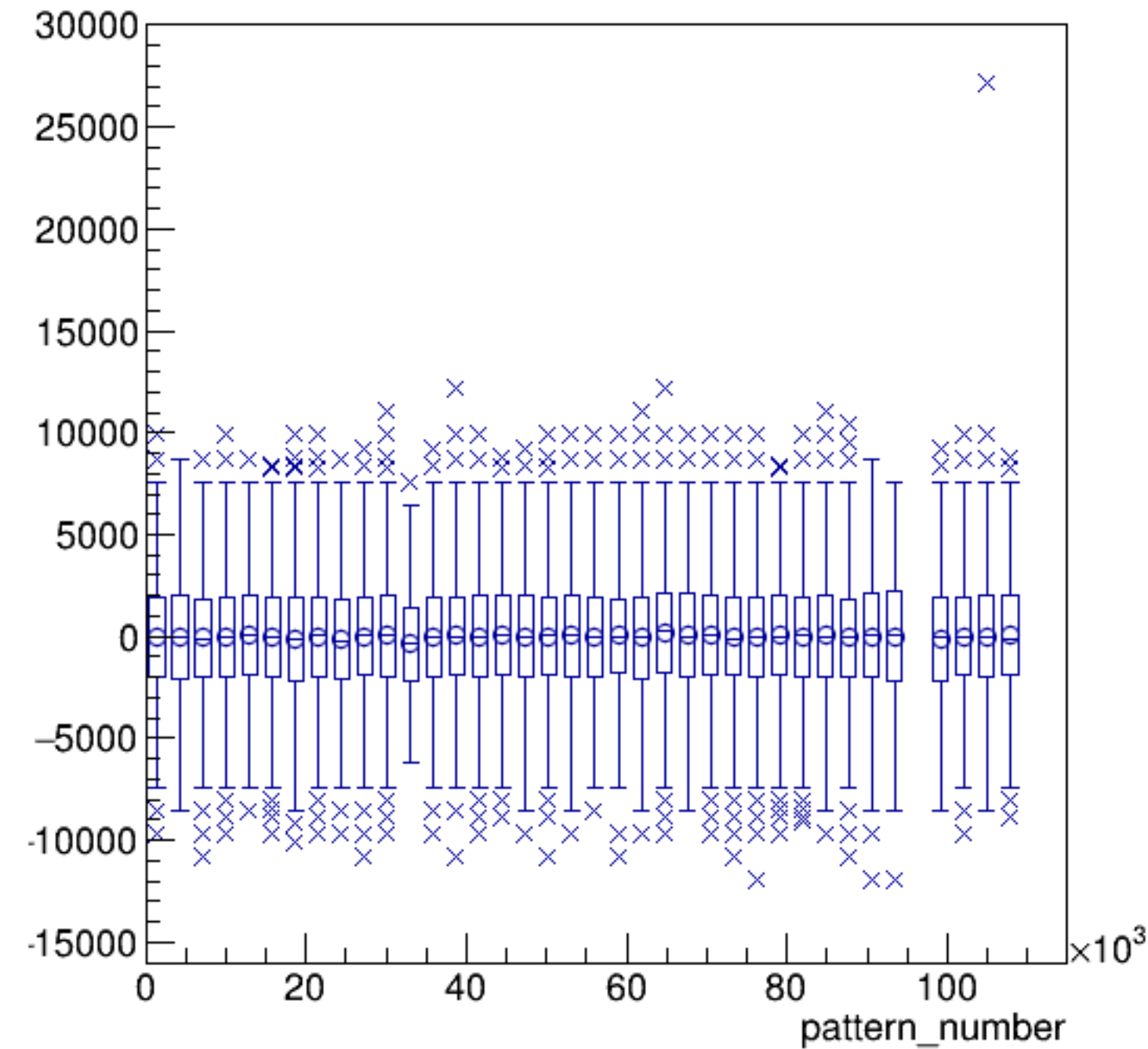
asym_atr1/ppm:pattern_number {ErrorFlag==0}
