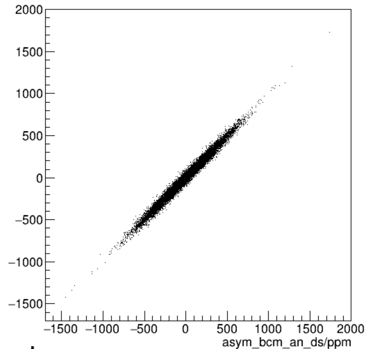
run7407_000_asym_bcm_an_us_vs_asym_bcm_an_ds_pr.png
