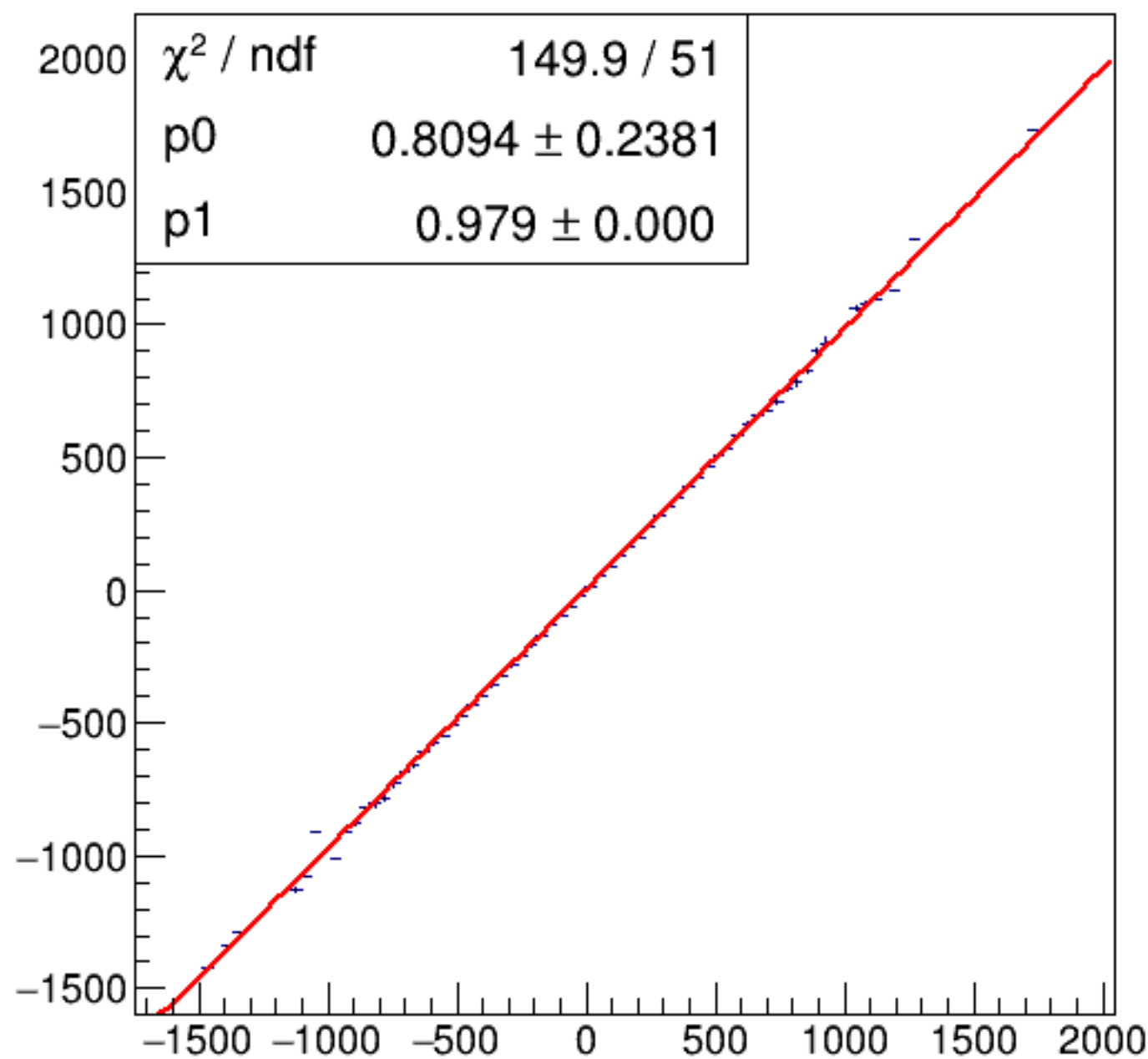
run7407_000_asym_bcm_an_us_vs_asym_bcm_an_ds_pr.png
