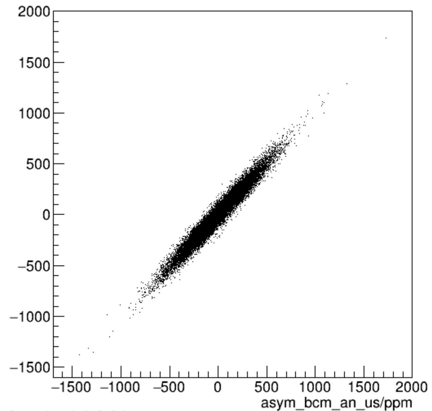
run7407_000_asym_bcm_dg_ds_vs_asym_bcm_an_us_pr.png
