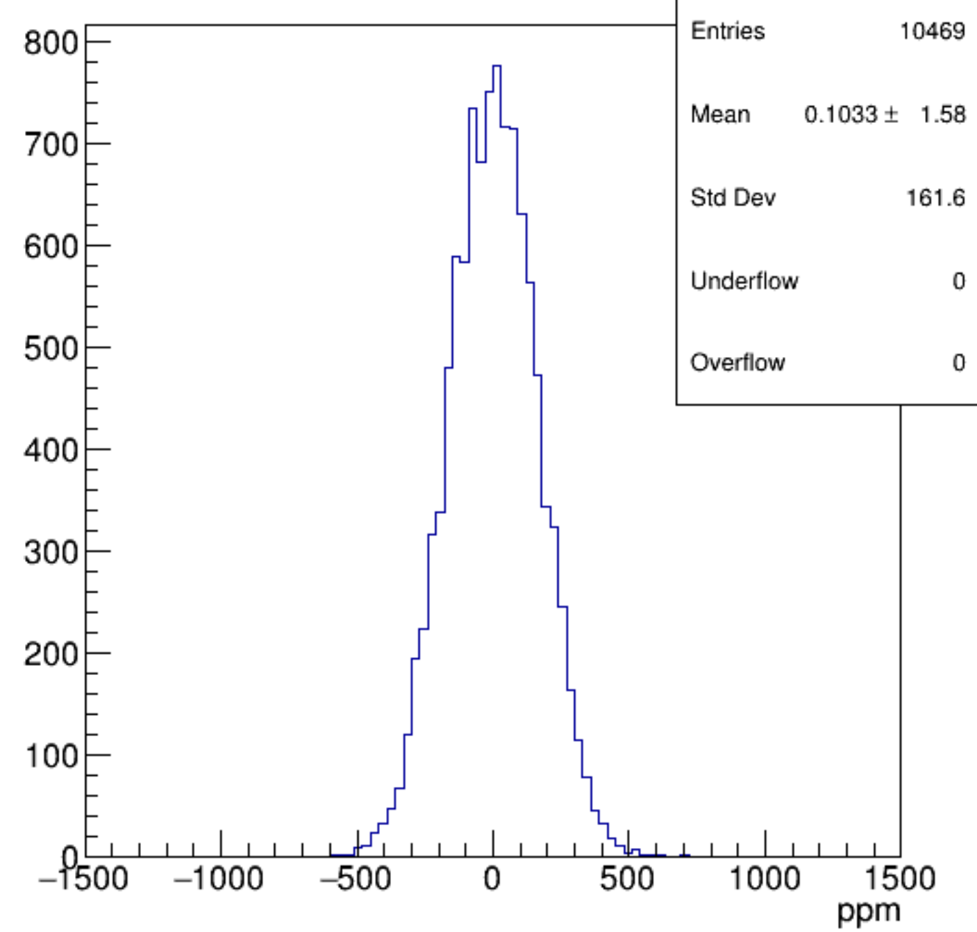
asym_bcm_dg_ds
