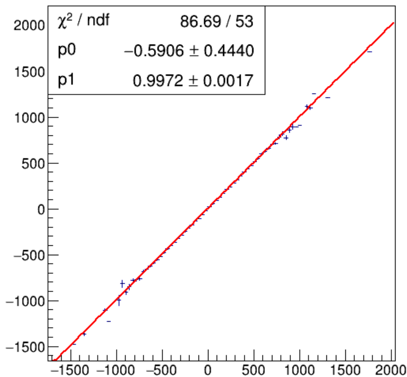
run7407_000_asym_bcm_dg_us_vs_asym_bcm_an_ds3_pr.png
