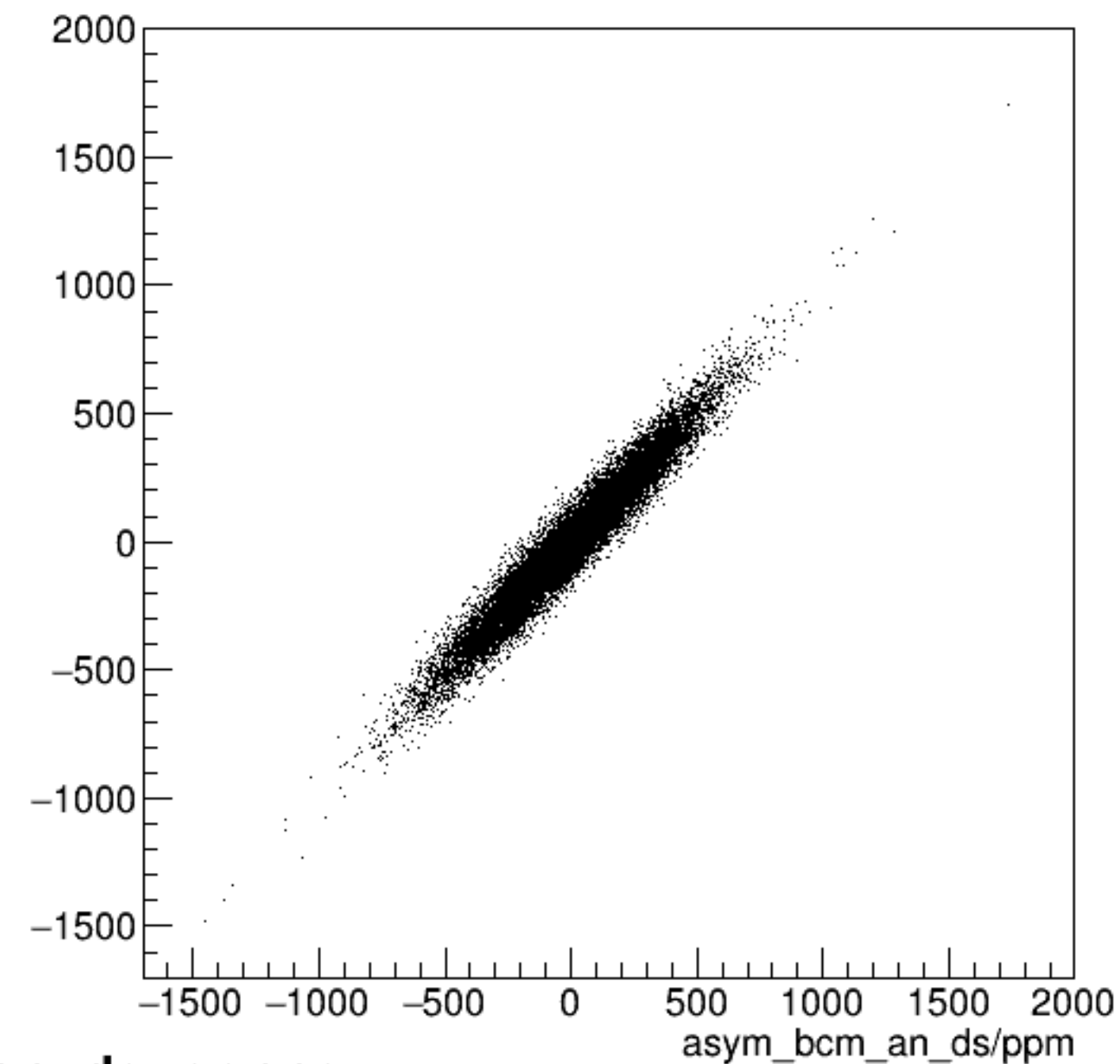
run7407_000_asym_bcm_dg_us_vs_asym_bcm_an_ds_pr.png
