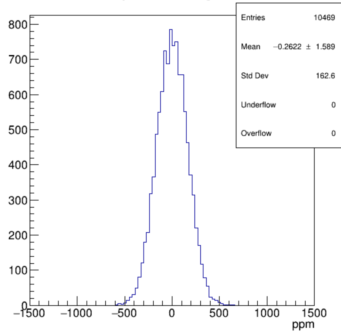
asym_bcm_dg_us
