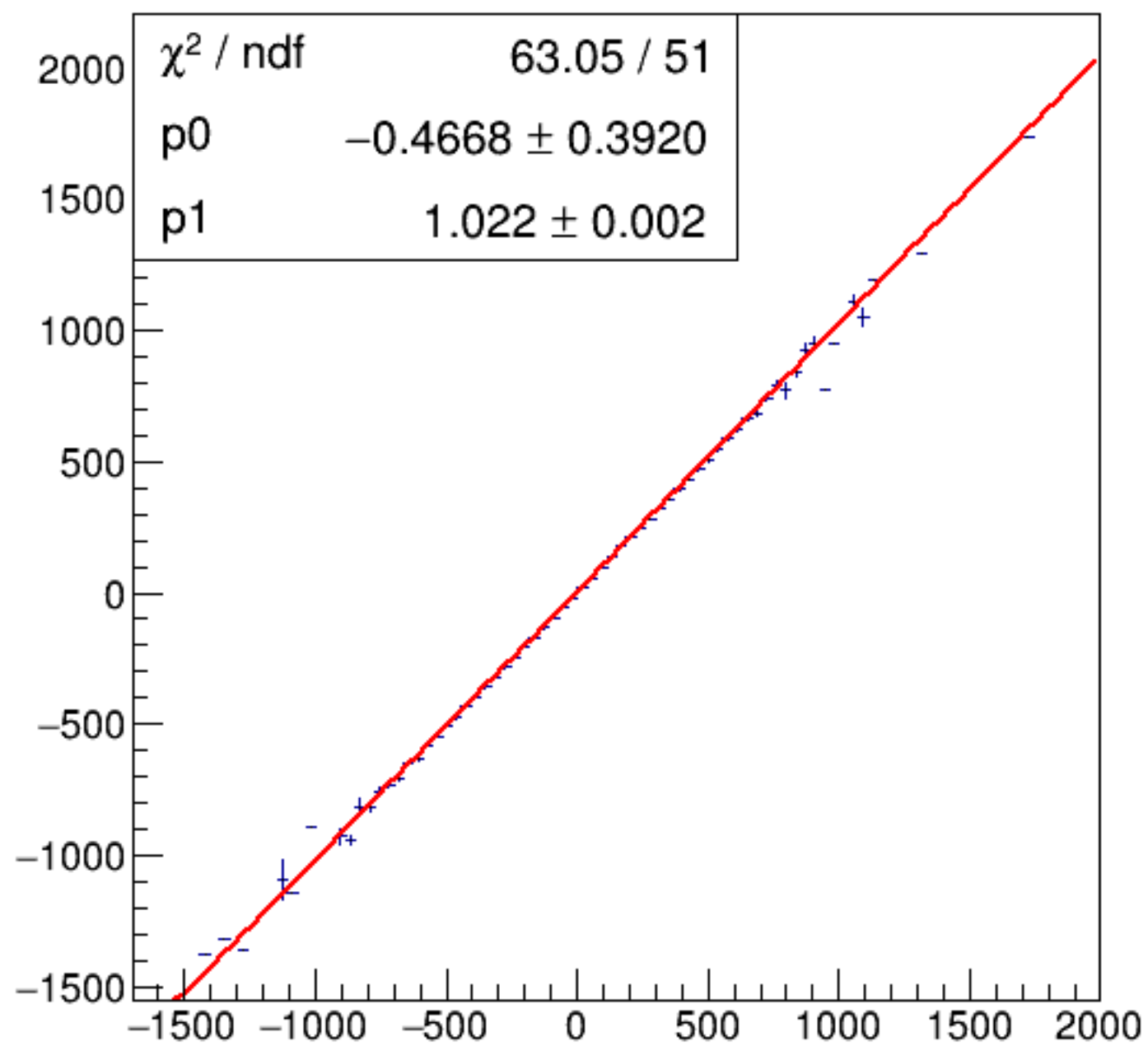
run7407_000_asym_bcm_dg_ds_vs_asym_bcm_an_us_pr.png
