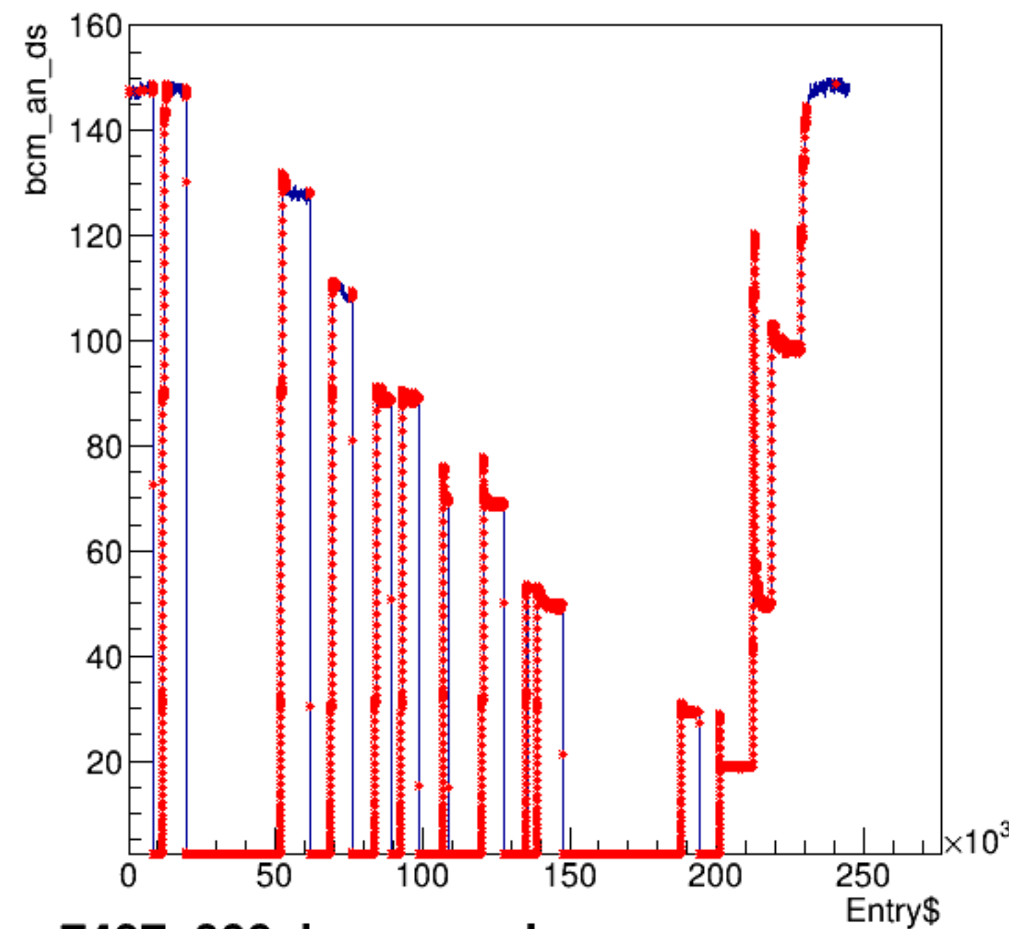
bcm_an_ds:Entry$
