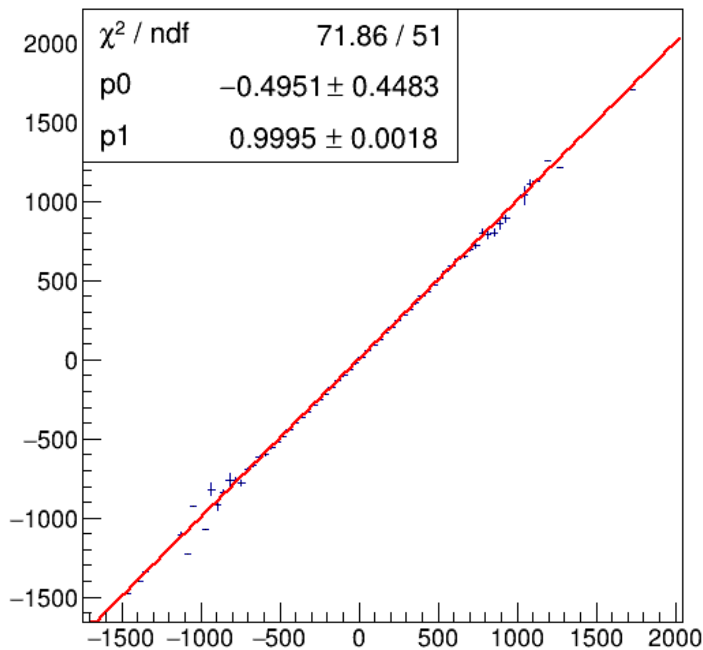
run7407_000_asym_bcm_dg_us_vs_asym_bcm_an_ds_pr.png
