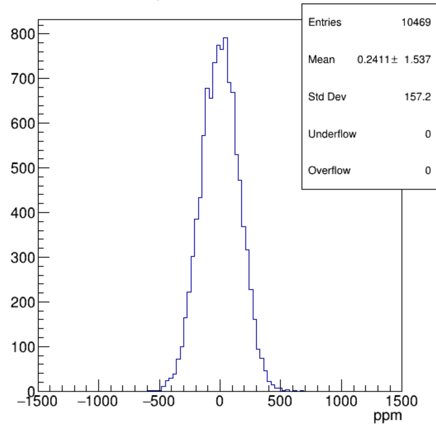
asym_bcm_an_ds
