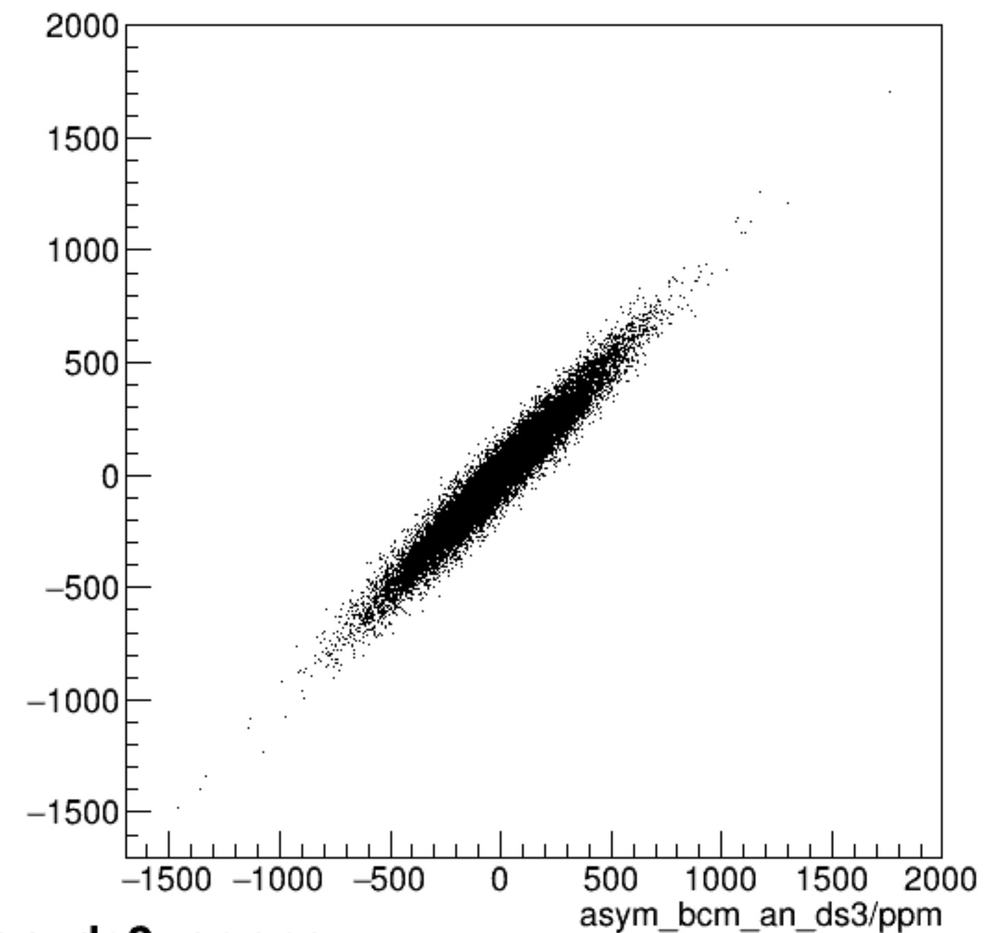
run7407_000_asym_bcm_dg_us_vs_asym_bcm_an_ds3_pr.png
