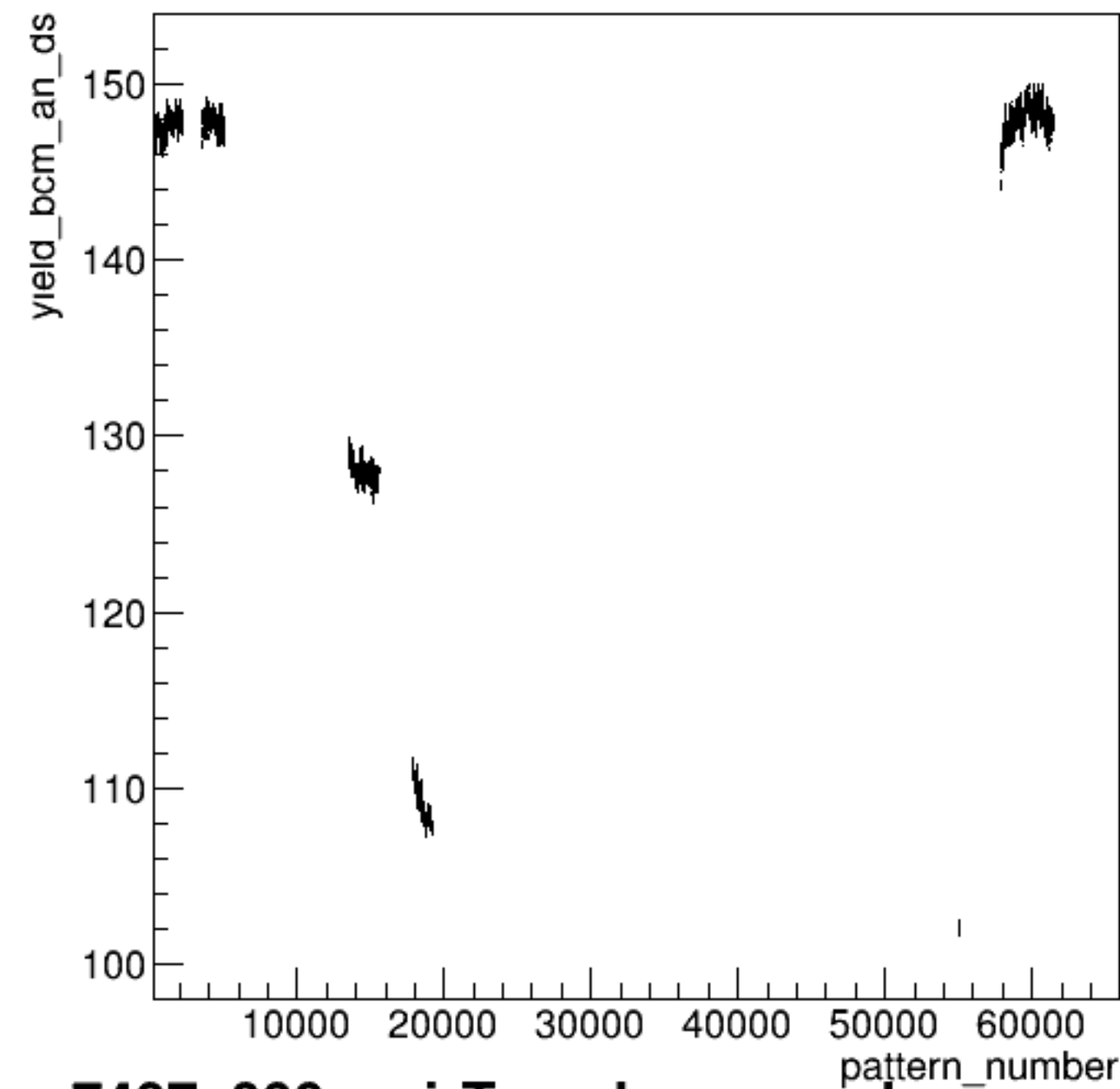
yield_bcm_an_ds:pattern_number {ErrorFlag==0}
