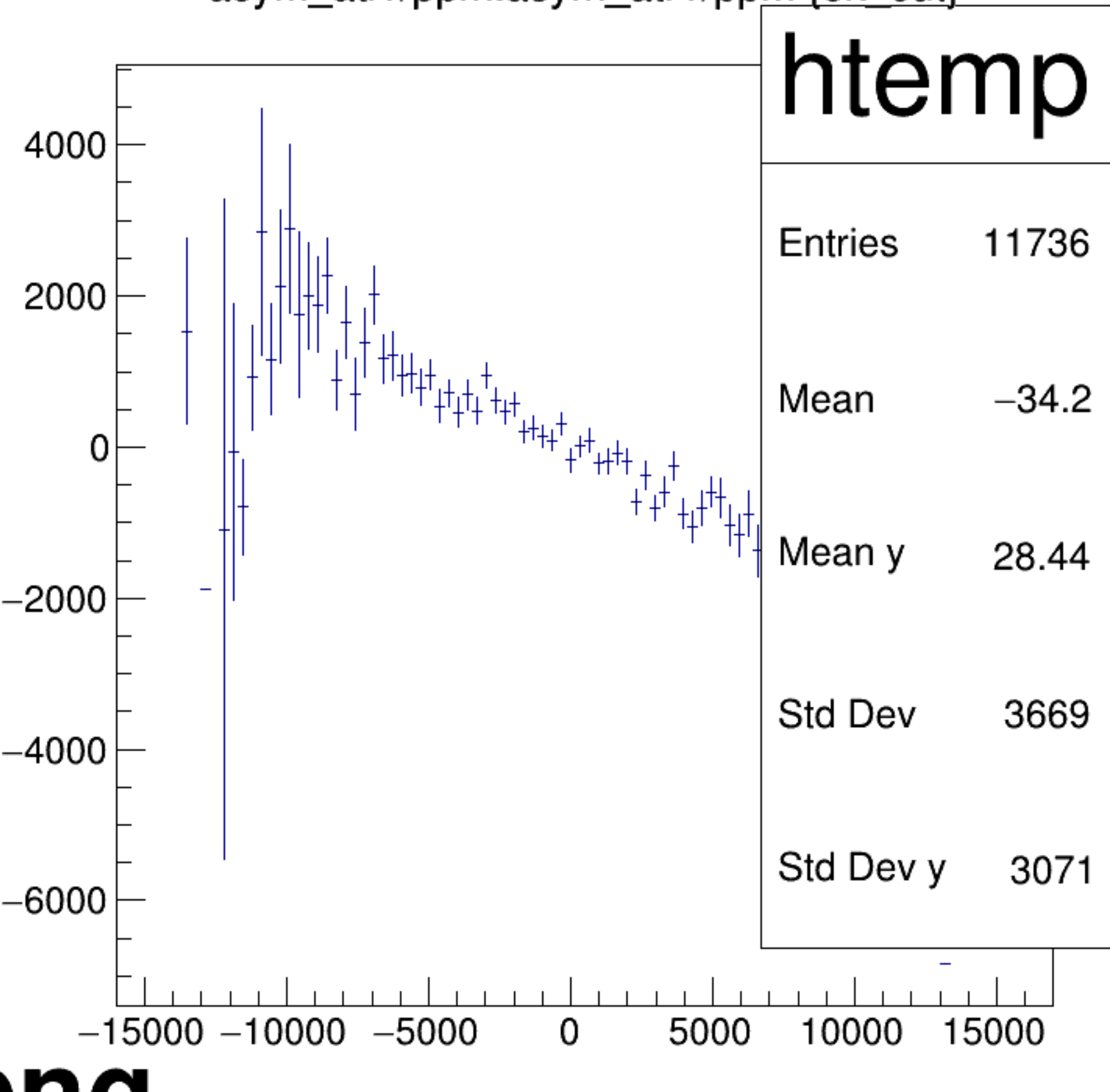
asym_atl1/ppm:asym_atr1/ppm {ok_cut}
