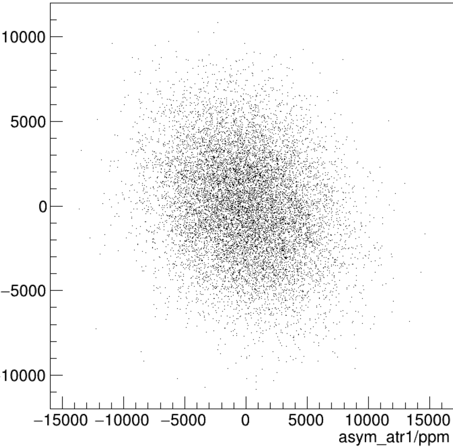
asym_atl1/ppm:asym_atr1/ppm {ok_cut}
