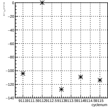
1X_coil1:cyclenum {run == 7630}
