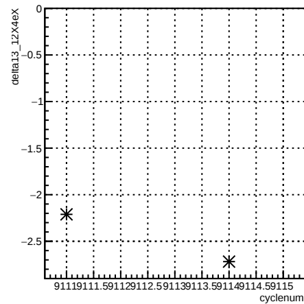
delta13_12X4eX:cyclenum {run == 7630}
