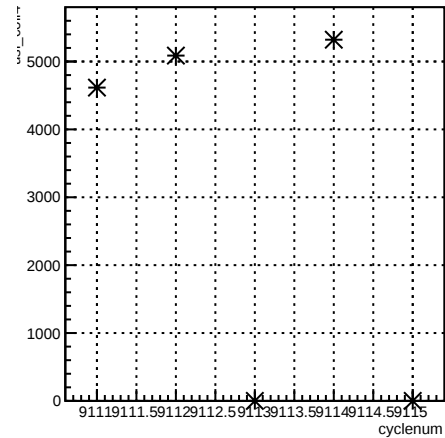
run:cyclenum {run == 7630}
