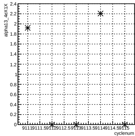
alpha13_4eX1X:cyclenum {run == 7630}
