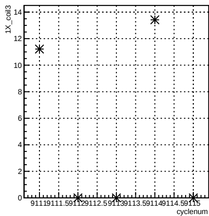
1X_coil3:cyclenum {run == 7630}
