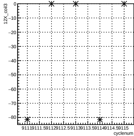
12X_coil3:cyclenum {run == 7630}
