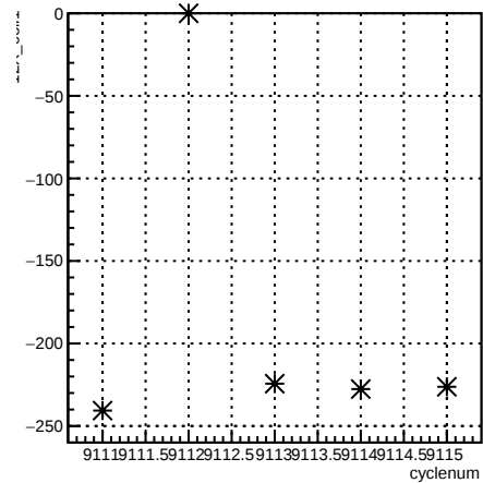
12X_coil1:cyclenum {run == 7630}
