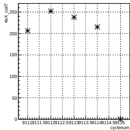
4eX_coil7:cyclenum {run == 7630}
