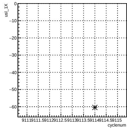
usl_1X:cyclenum {run == 7630}
