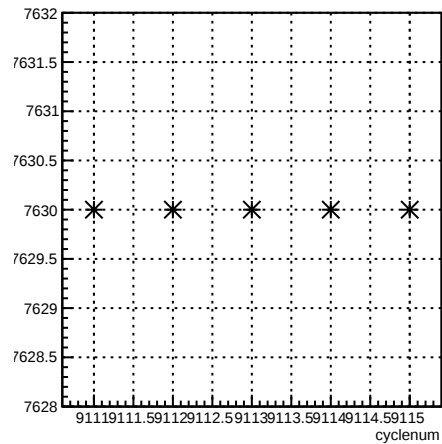
run:cyclenum {run == 7630}
