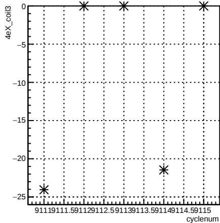
4eX_coil3:cyclenum {run == 7630}
