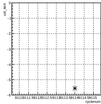
usl_4eX:cyclenum {run == 7630}
