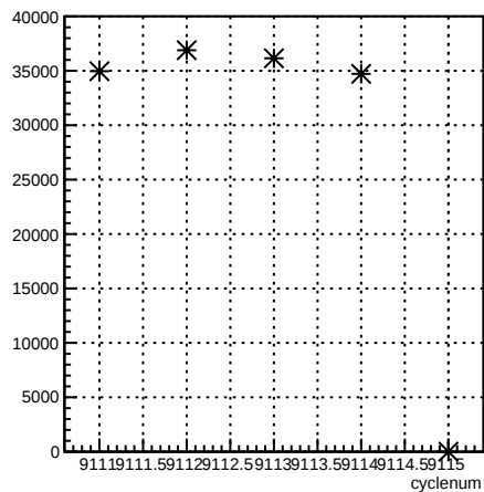
usr_coil7:cyclenum {run == 7630}
