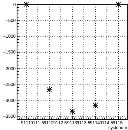
usr_coil6:cyclenum {run == 7630}
