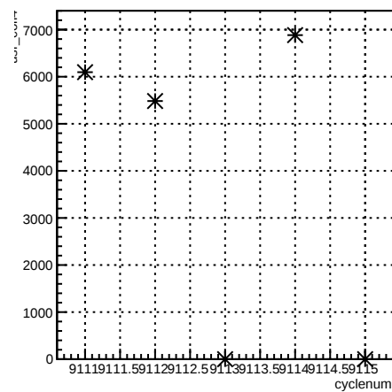
usr_coil4:cyclenum {run == 7630}
