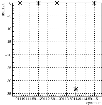
usl_12X:cyclenum {run == 7630}
