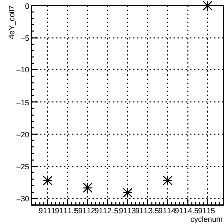
4eY_coil7:cyclenum {run == 7630}
