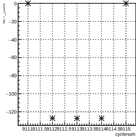
4eY_coil6:cyclenum {run == 7630}
