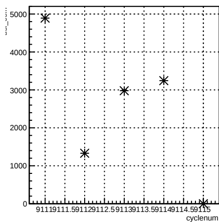
usl_coil7:cyclenum {run == 7630}
