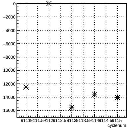
usr_coil1:cyclenum {run == 7630}
