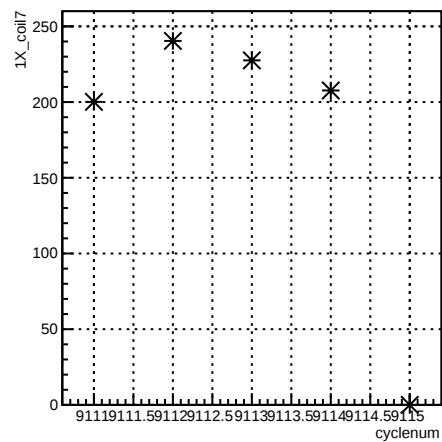
1X_coil7:cyclenum {run == 7630}
