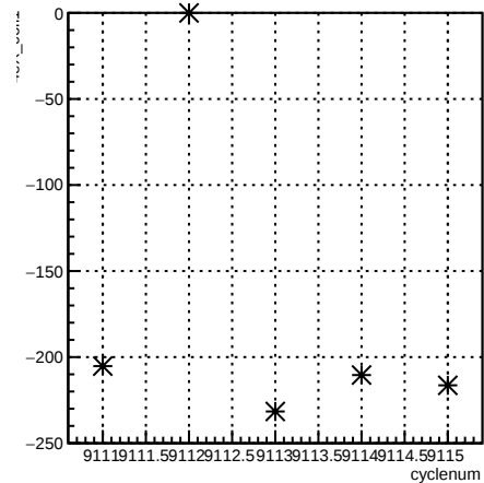
4eX_coil1:cyclenum {run == 7630}
