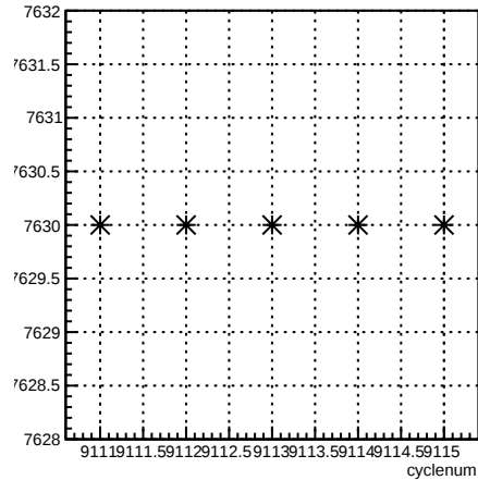
run:cyclenum {run == 7630}
