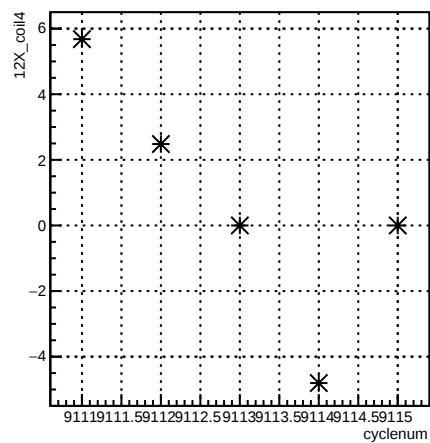
12X_coil4:cyclenum {run == 7630}
