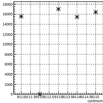
usl_coil6:cyclenum {run == 7630}
