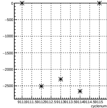
usl_coil6:cyclenum {run == 7630}
