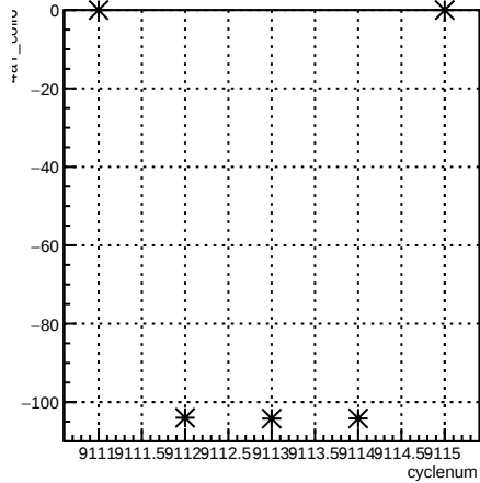
4eY_coil6:cyclenum {run == 7630}
