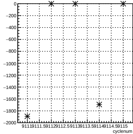
usr_coil3:cyclenum {run == 7630}
