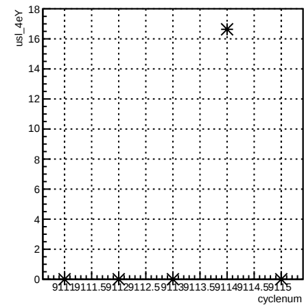
usl_4eY:cyclenum {run == 7630}
