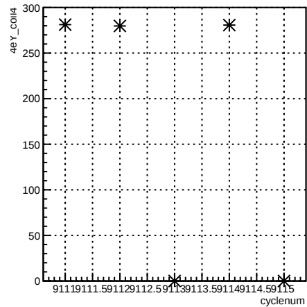
4eY_coil4:cyclenum {run == 7630}
