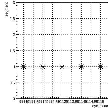
segment:cyclenum {run == 7630}
