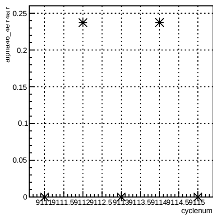
alpha46_4eY4aY:cyclenum {run == 7630}
