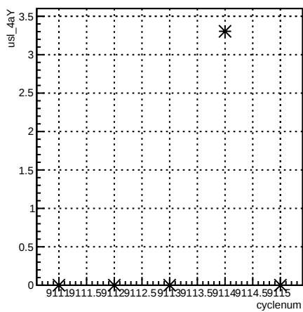
usl_4aY:cyclenum {run == 7630}
