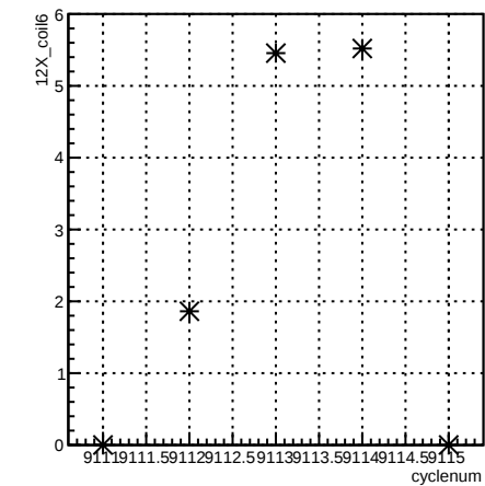
12X_coil6:cyclenum {run == 7630}
