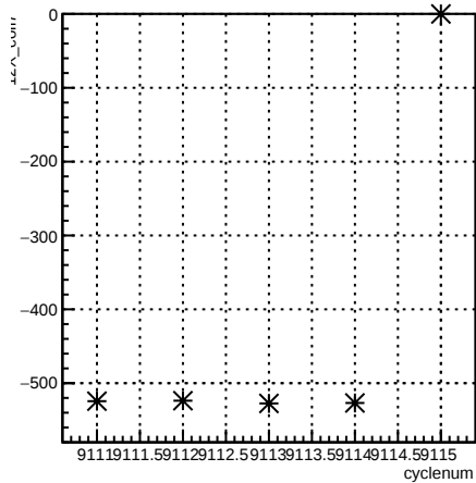
12X_coil7:cyclenum {run == 7630}
