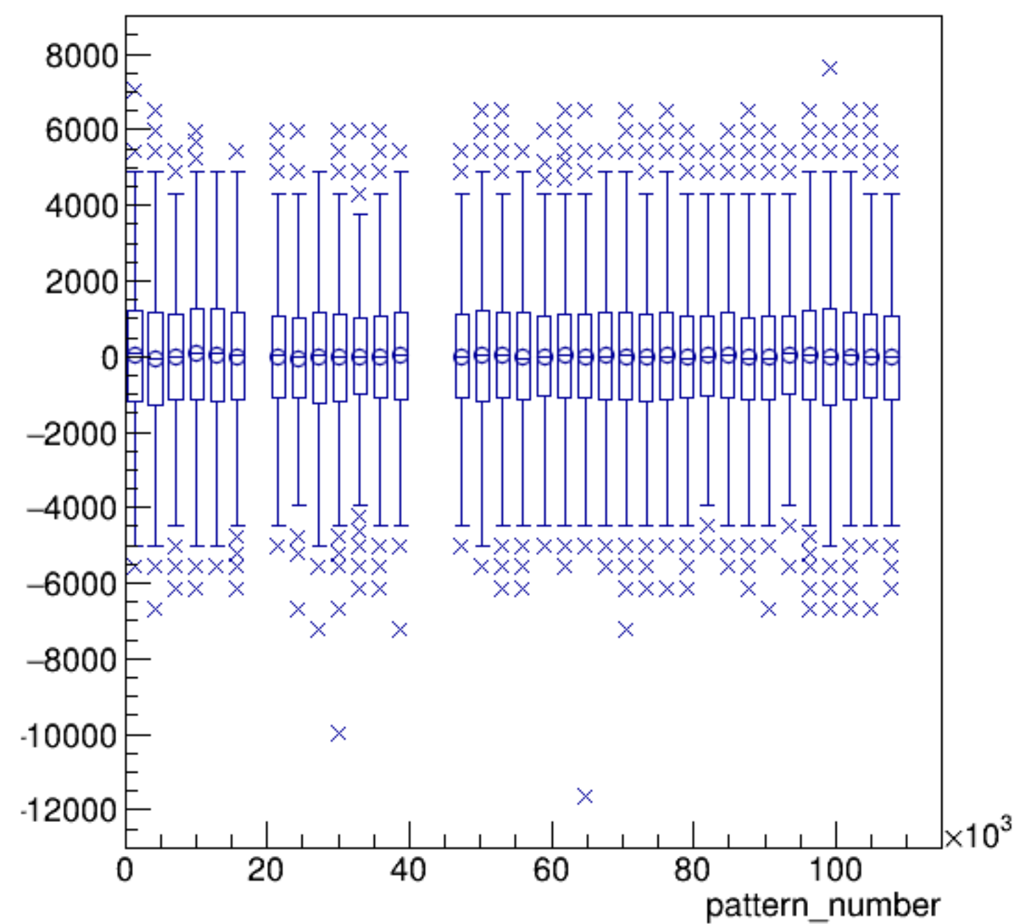
asym_sam7/ppm:pattern_number {ErrorFlag==0}
