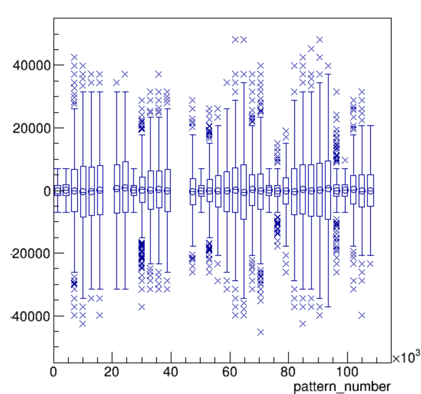
asym_sam6/ppm:pattern_number {ErrorFlag==0}
