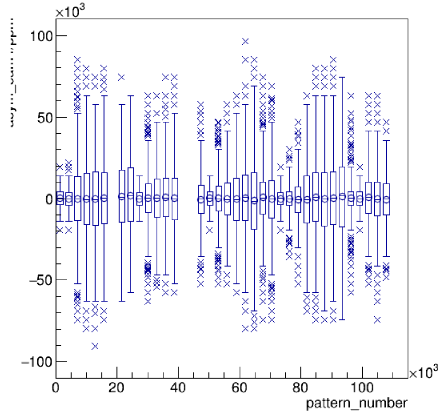
asym_sam4/ppm:pattern_number {ErrorFlag==0}
