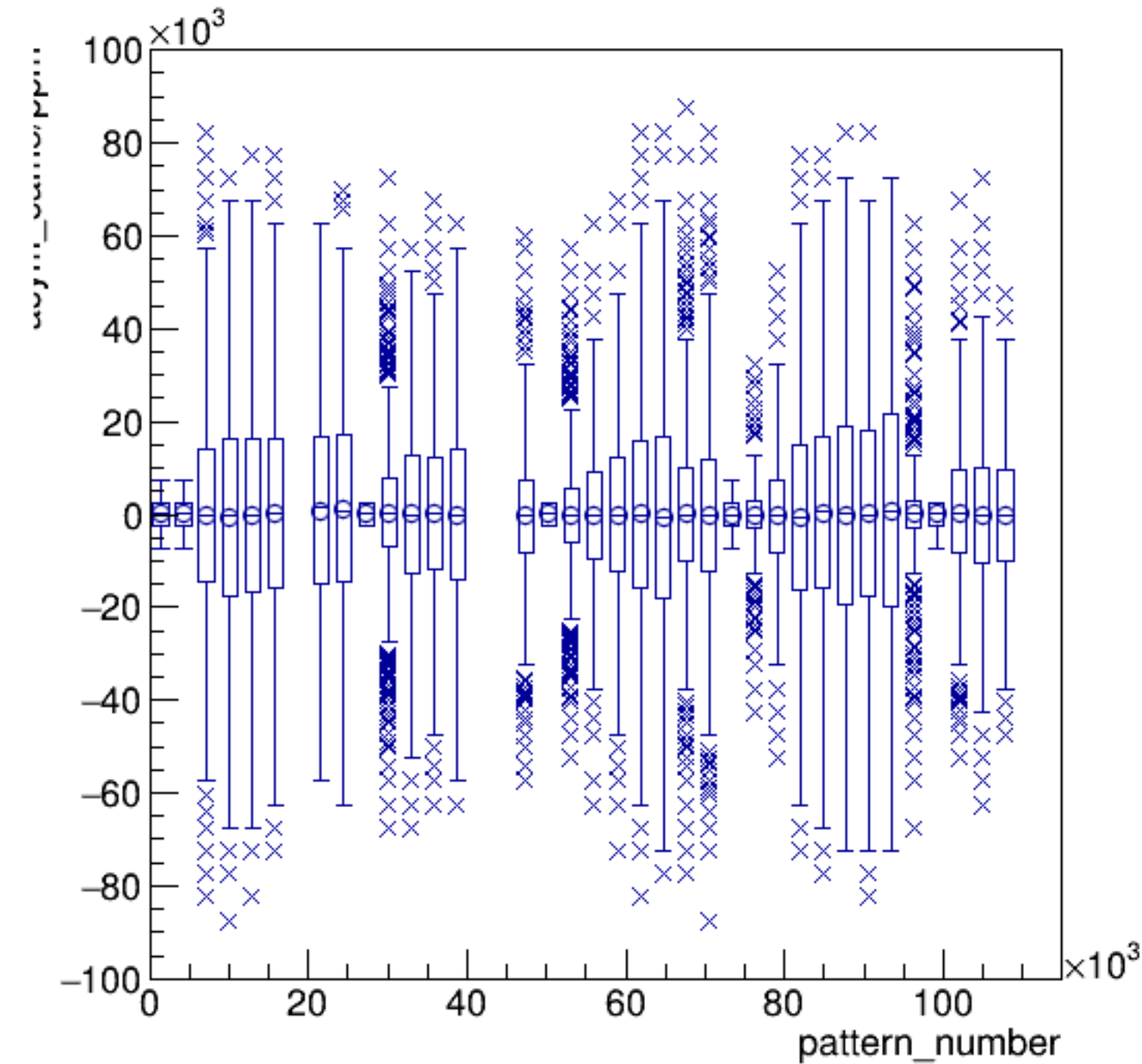
asym_sam5/ppm:pattern_number {ErrorFlag==0}
