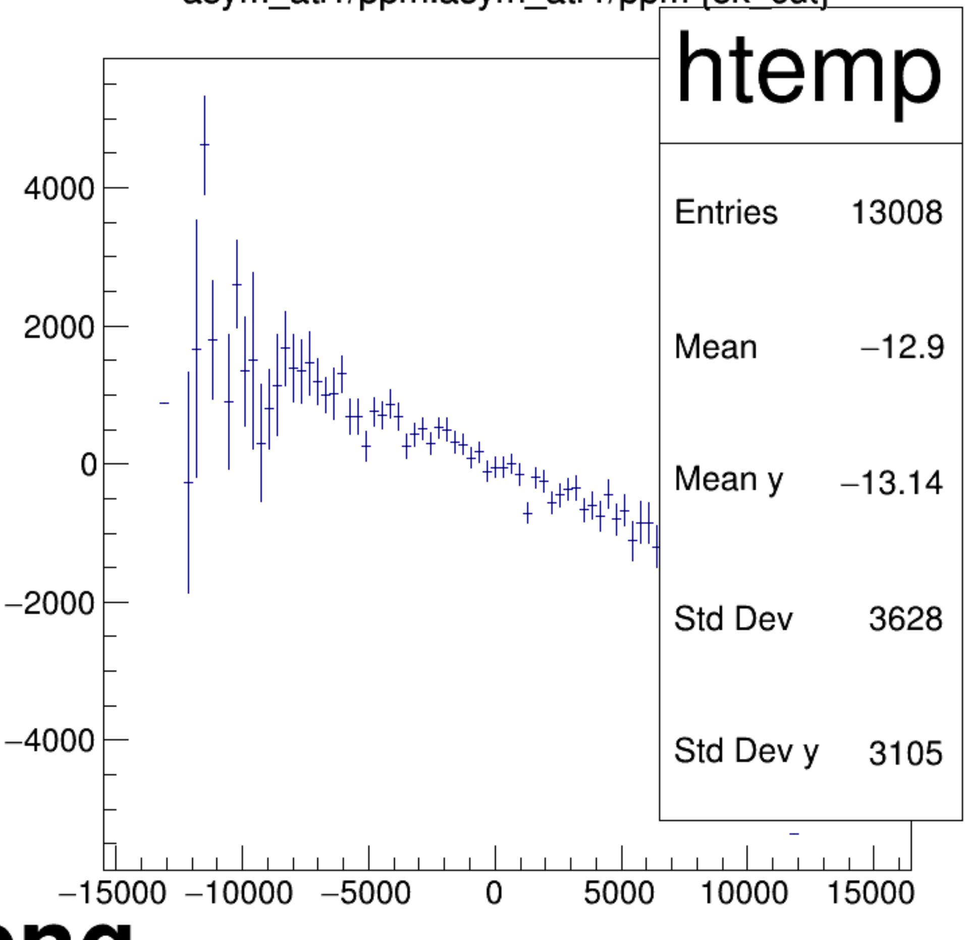
asym_atl1/ppm:asym_atr1/ppm {ok_cut}
