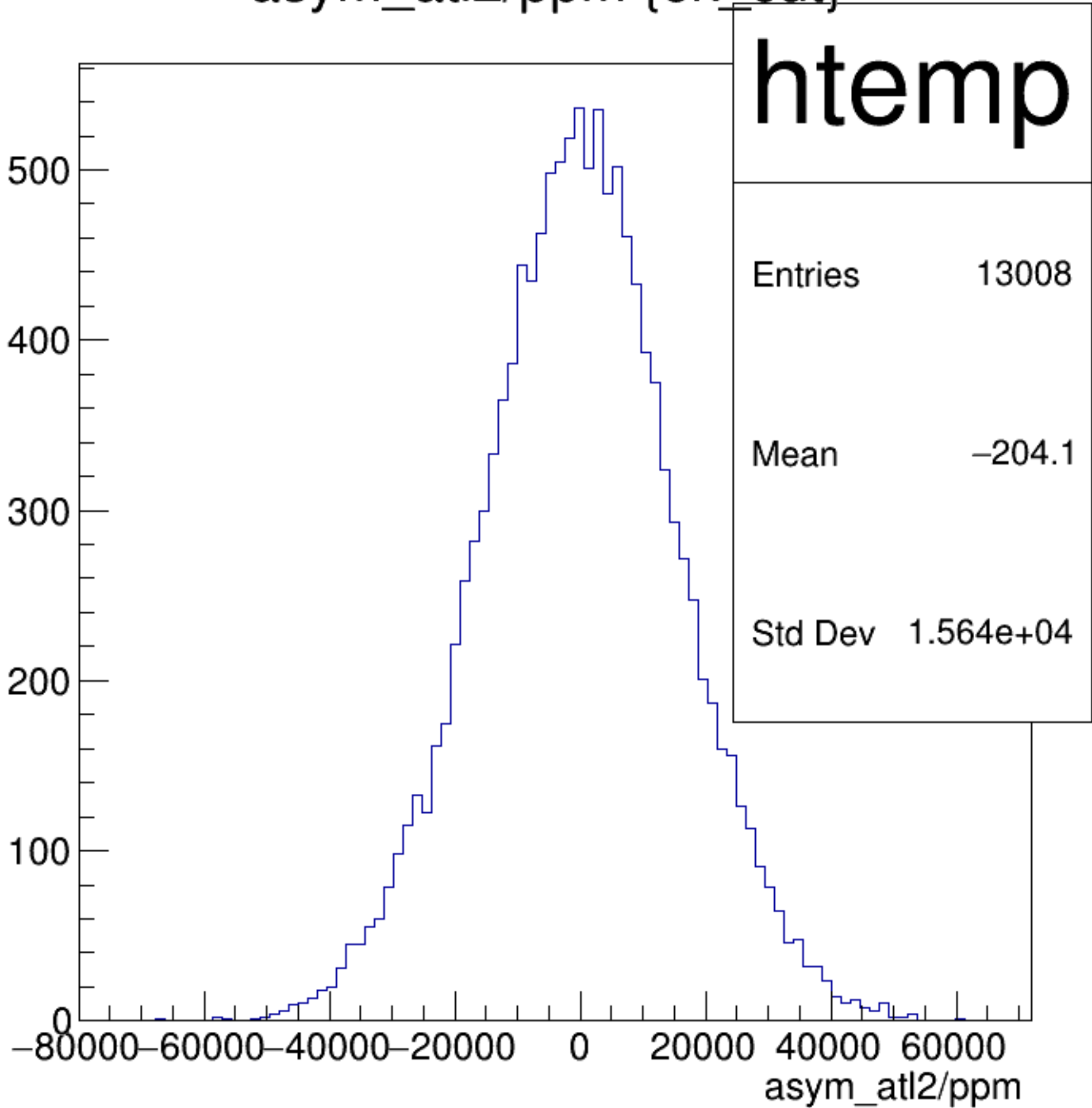
asym_atl2/ppm {ok_cut}
