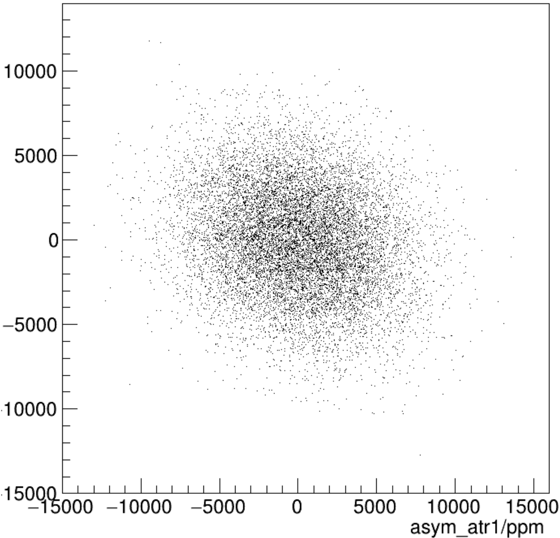
asym_atl1/ppm:asym_atr1/ppm {ok_cut}
