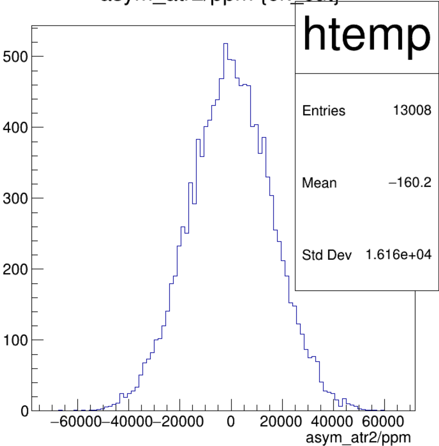
asym_atr2/ppm {ok_cut}
