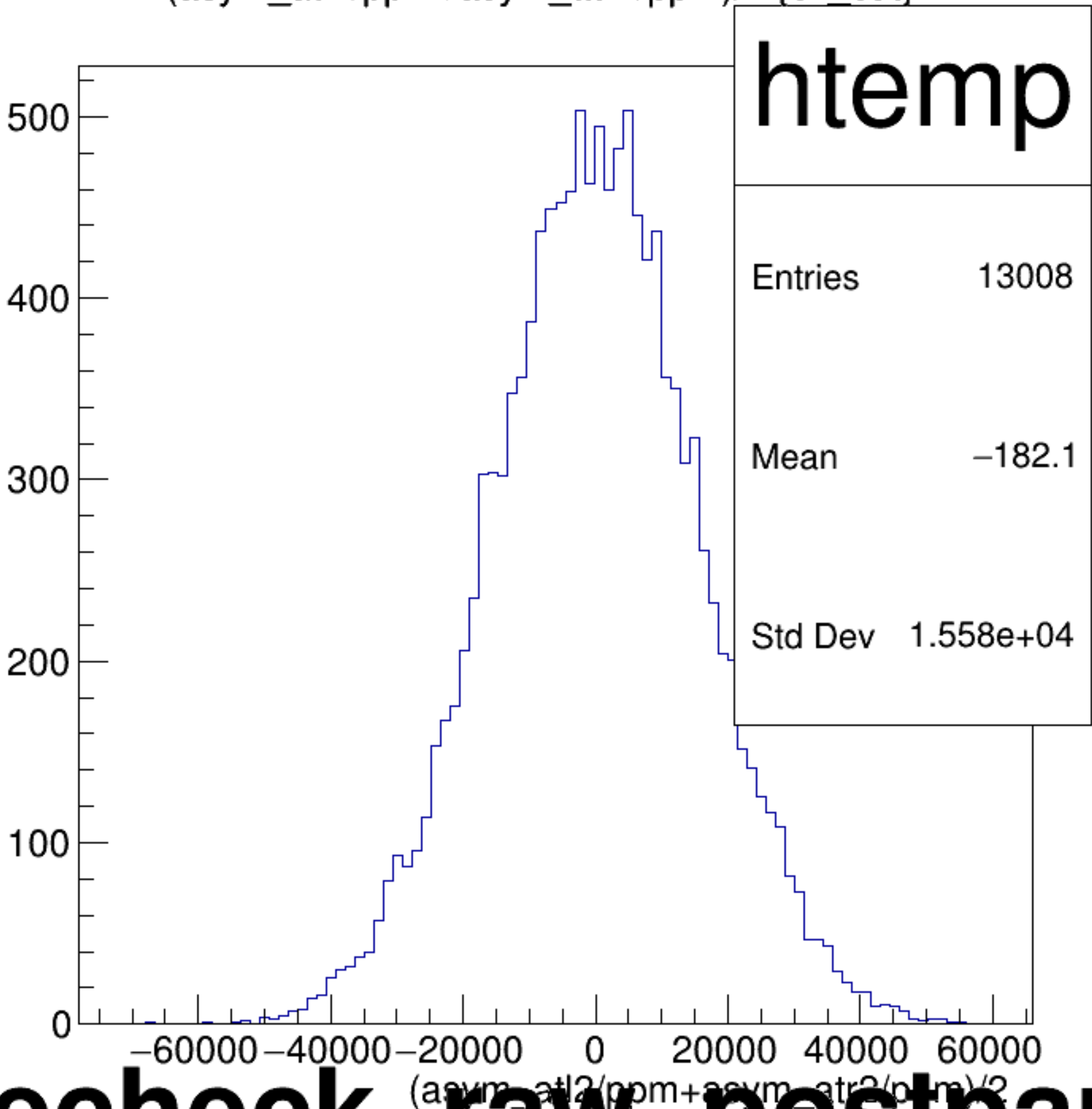
(asym_atl2/ppm+asym_atr2/ppm)/2 {ok_cut}
