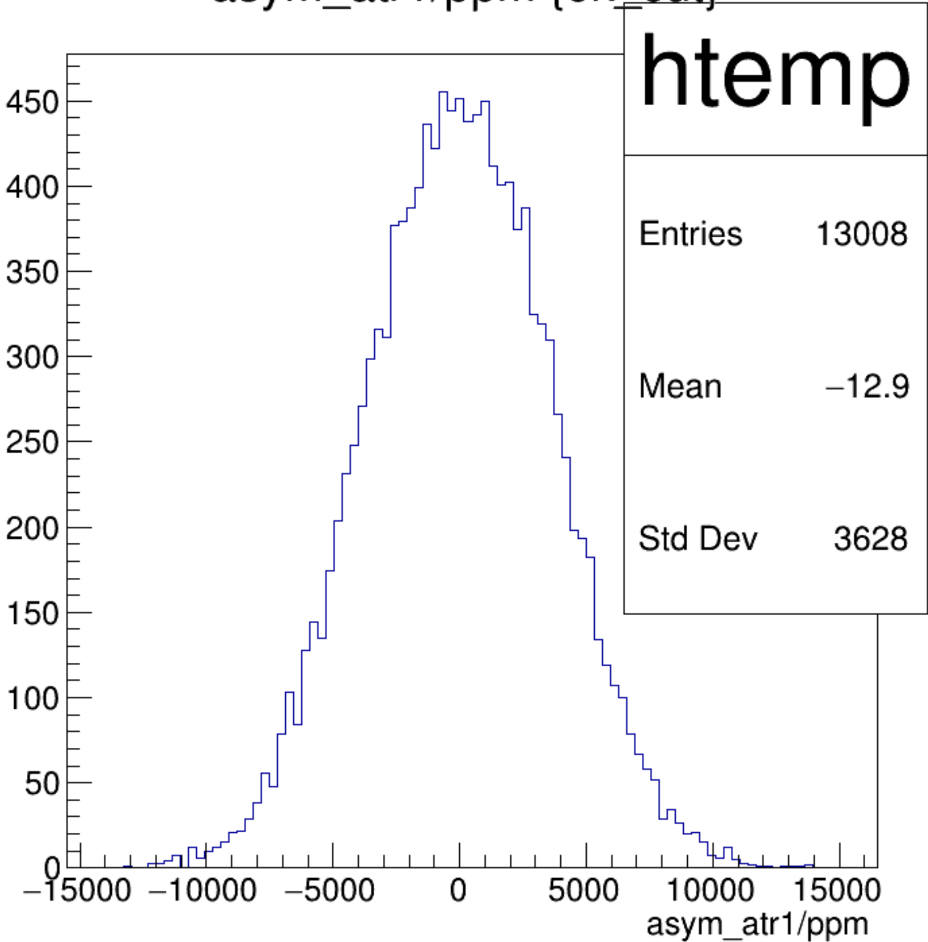
asym_atr1/ppm {ok_cut}
