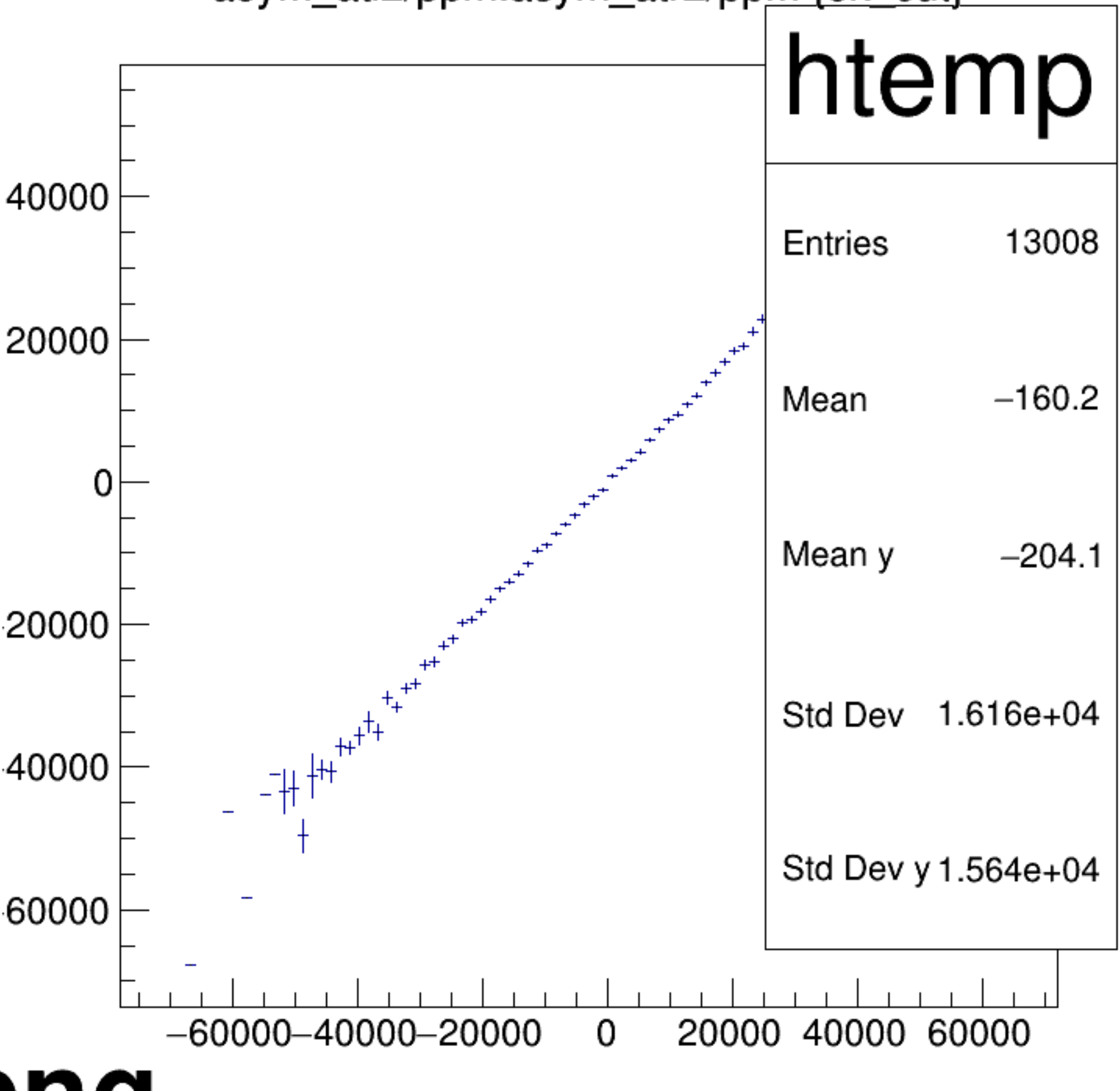
asym_atl2/ppm:asym_atr2/ppm {ok_cut}
