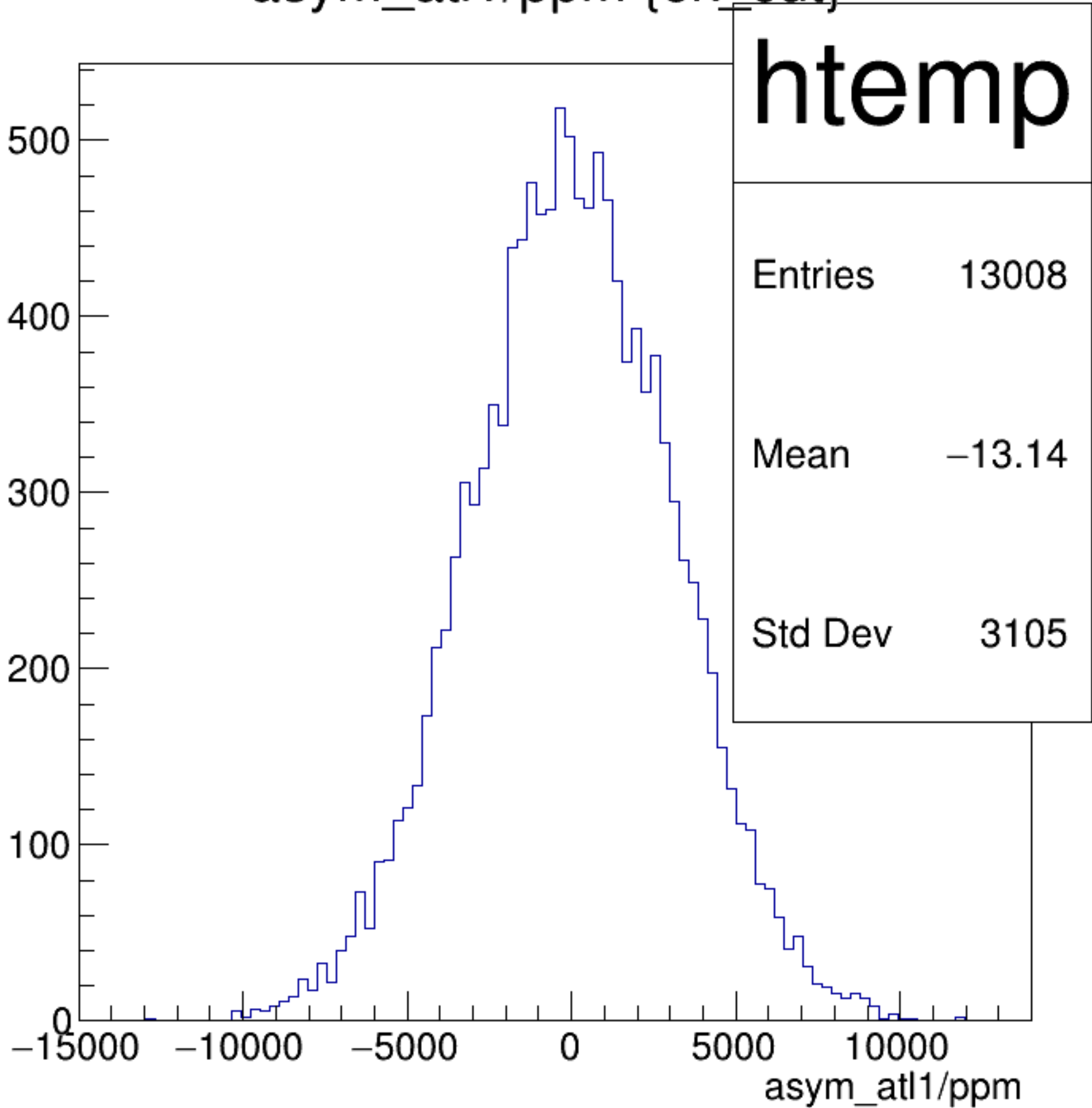
asym_atl1/ppm {ok_cut}
