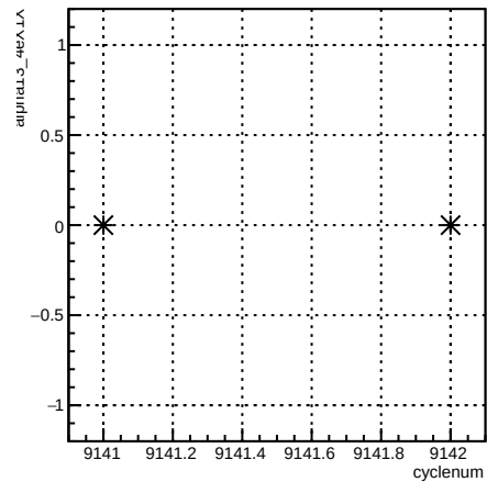
delta46_12X4eY:cyclenum {run == 7658}
