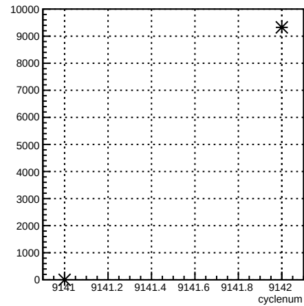
usr_coil4:cyclenum {run == 7658}
