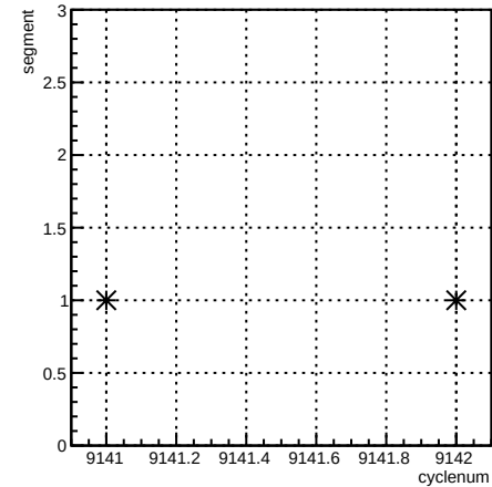
segment:cyclenum {run == 7658}
