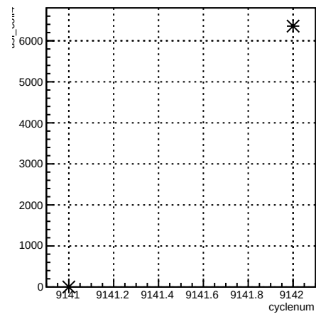
usl_coil4:cyclenum {run == 7658}
