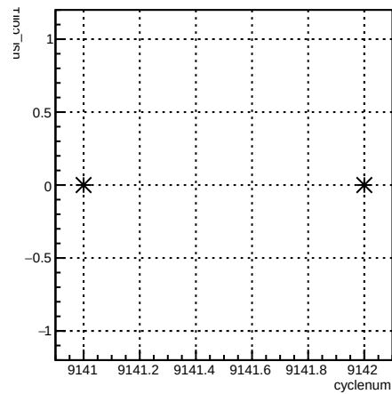
usl_coil1:cyclenum {run == 7658}
