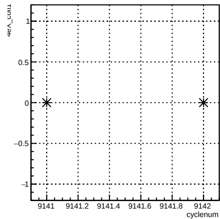
4eX_coil1:cyclenum {run == 7658}
