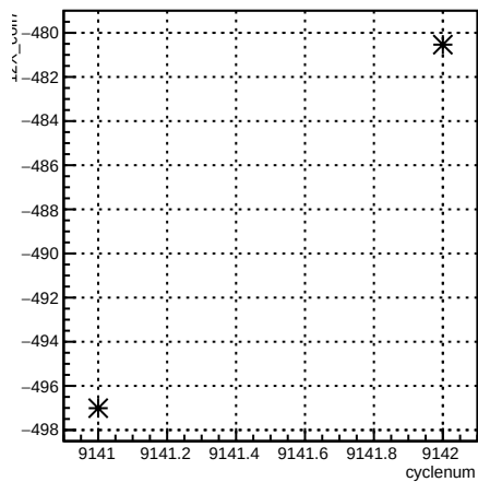
12X_coil7:cyclenum {run == 7658}
