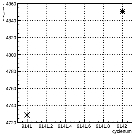
usl_coil7:cyclenum {run == 7658}
