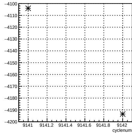
usr_coil6:cyclenum {run == 7658}
