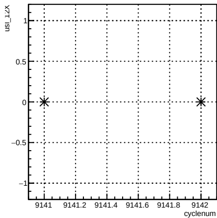
usl_12X:cyclenum {run == 7658}
