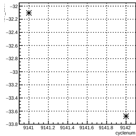
4eY_coil7:cyclenum {run == 7658}
