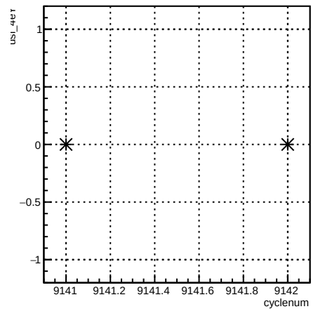
usl_4eY:cyclenum {run == 7658}
