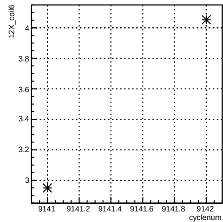
12X_coil6:cyclenum {run == 7658}
