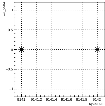
4eX_coil3:cyclenum {run == 7658}
