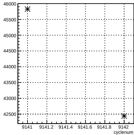
usr_coil7:cyclenum {run == 7658}
