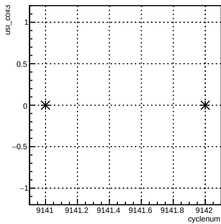
usl_coil3:cyclenum {run == 7658}
