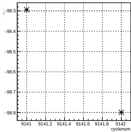
4eY_coil6:cyclenum {run == 7658}
