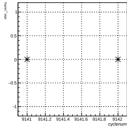
usr_coil6:cyclenum {run == 7658}
