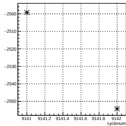
usl_coil6:cyclenum {run == 7658}
