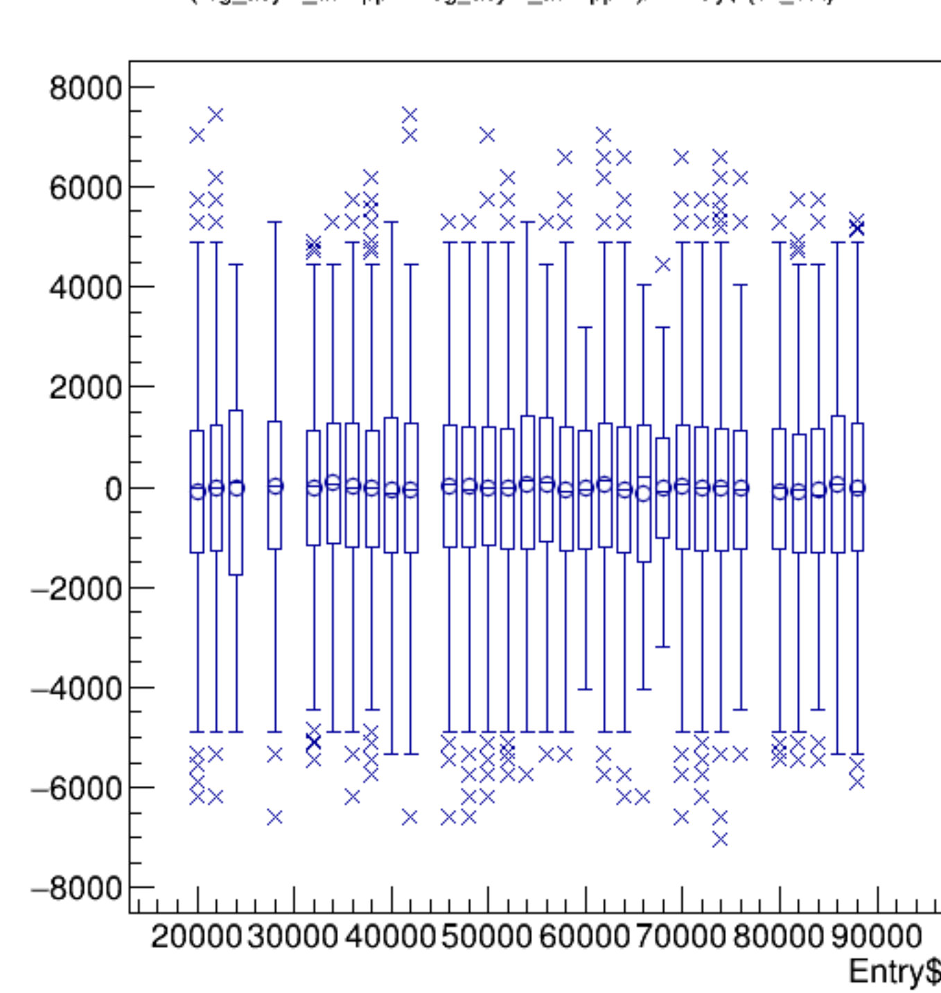
(reg_asym_atl1/ppm+reg_asym_atr1/ppm)/2:Entry$ {ok_cut}
