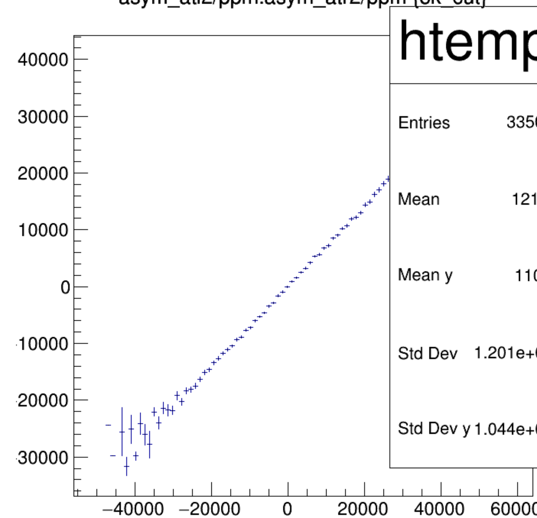
asym_atl2/ppm:asym_atr2/ppm {ok_cut}
