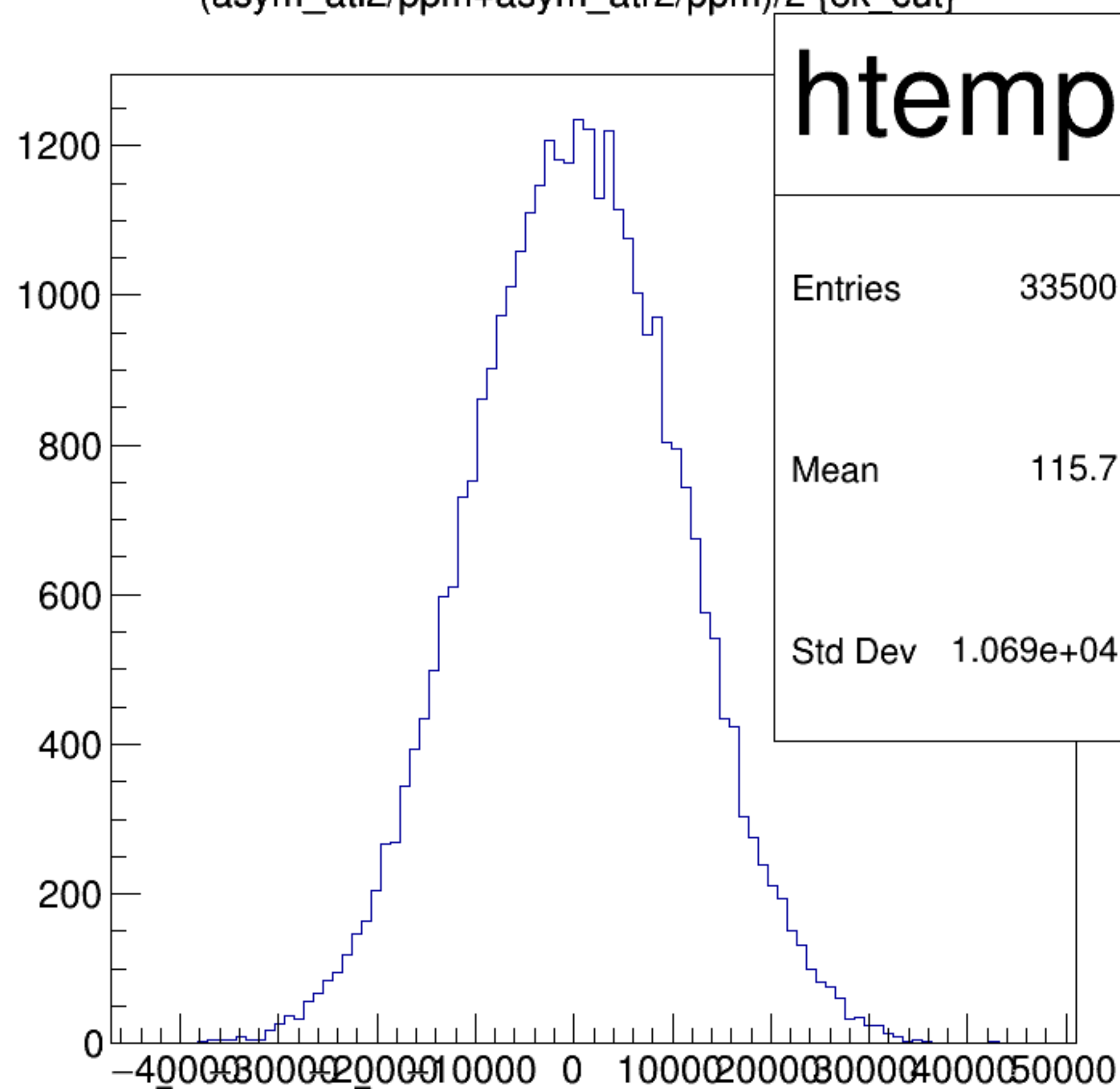
(asym_atl2/ppm+asym_atr2/ppm)/2 {ok_cut}
