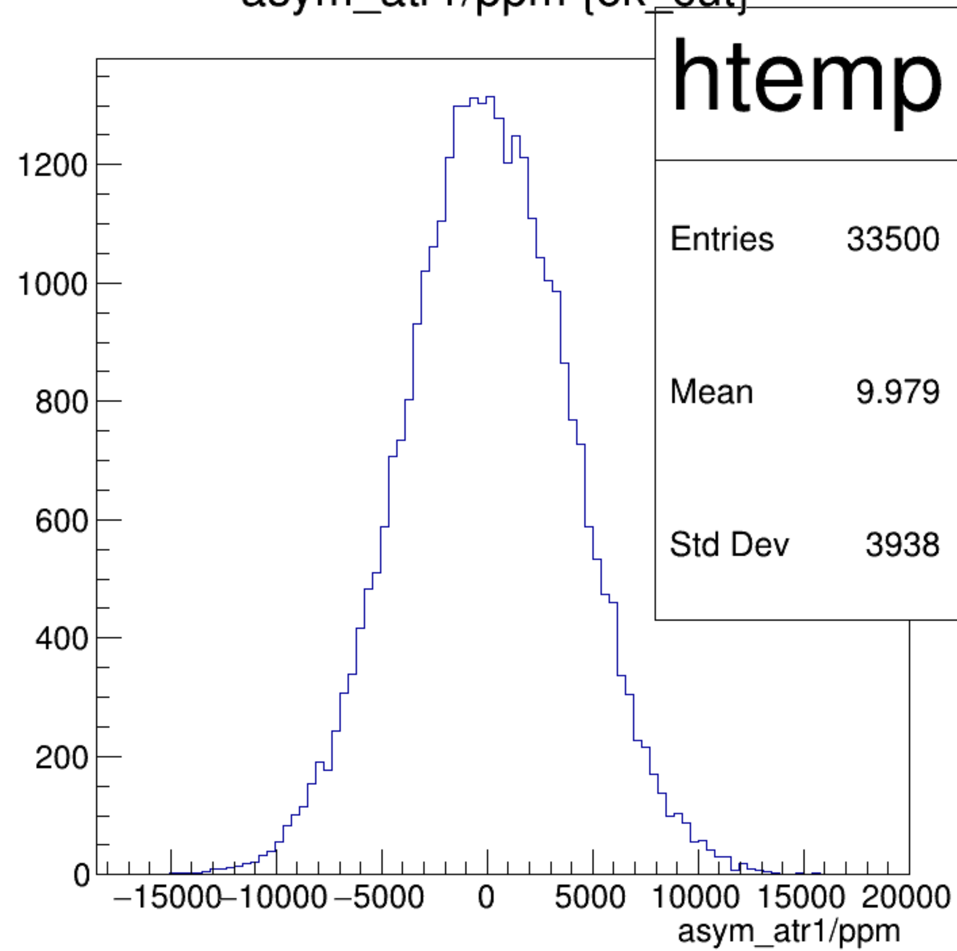
asym_atr1/ppm {ok_cut}
