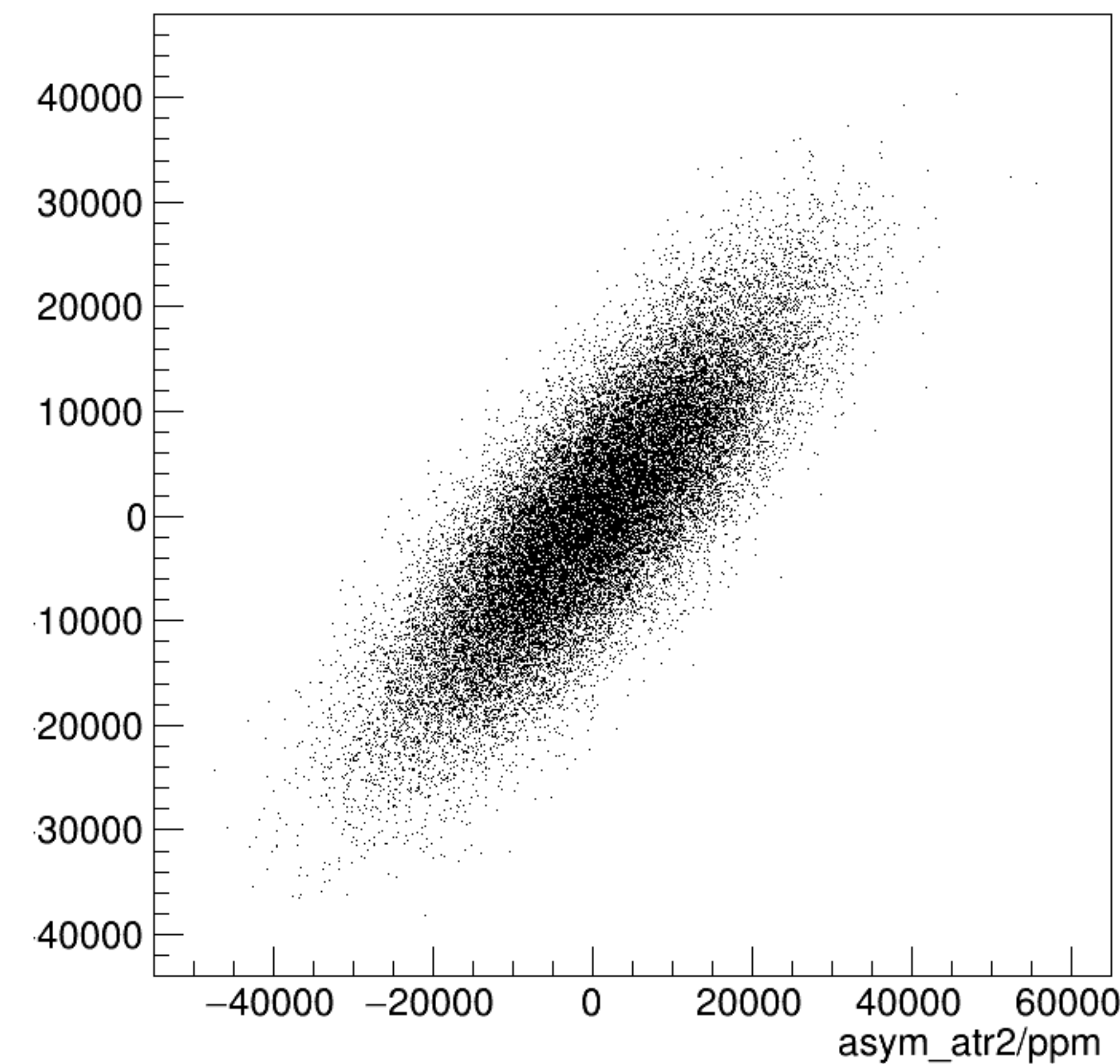
asym_atl2/ppm:asym_atr2/ppm {ok_cut}
