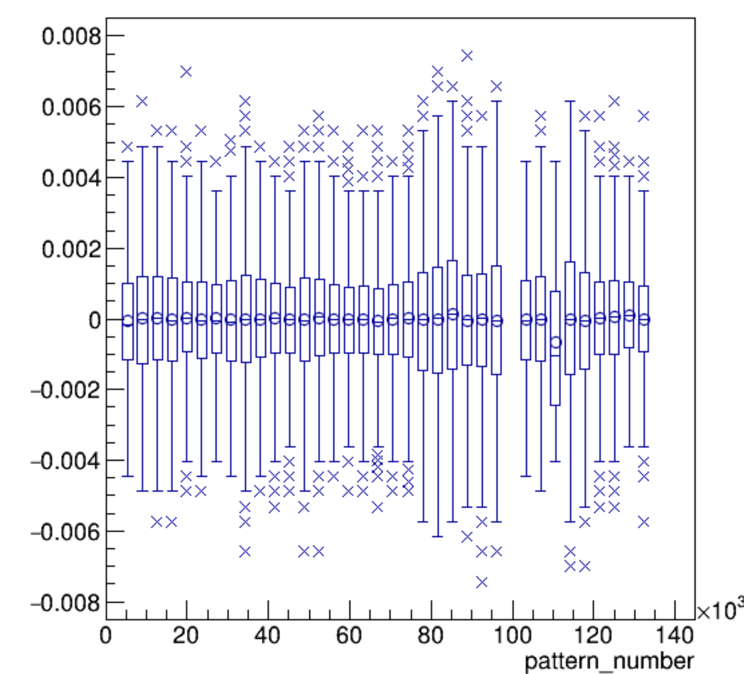
asym_bcm_an_diff*yield_bcm_an_diff:pattern_number {ErrorFlag==0}
