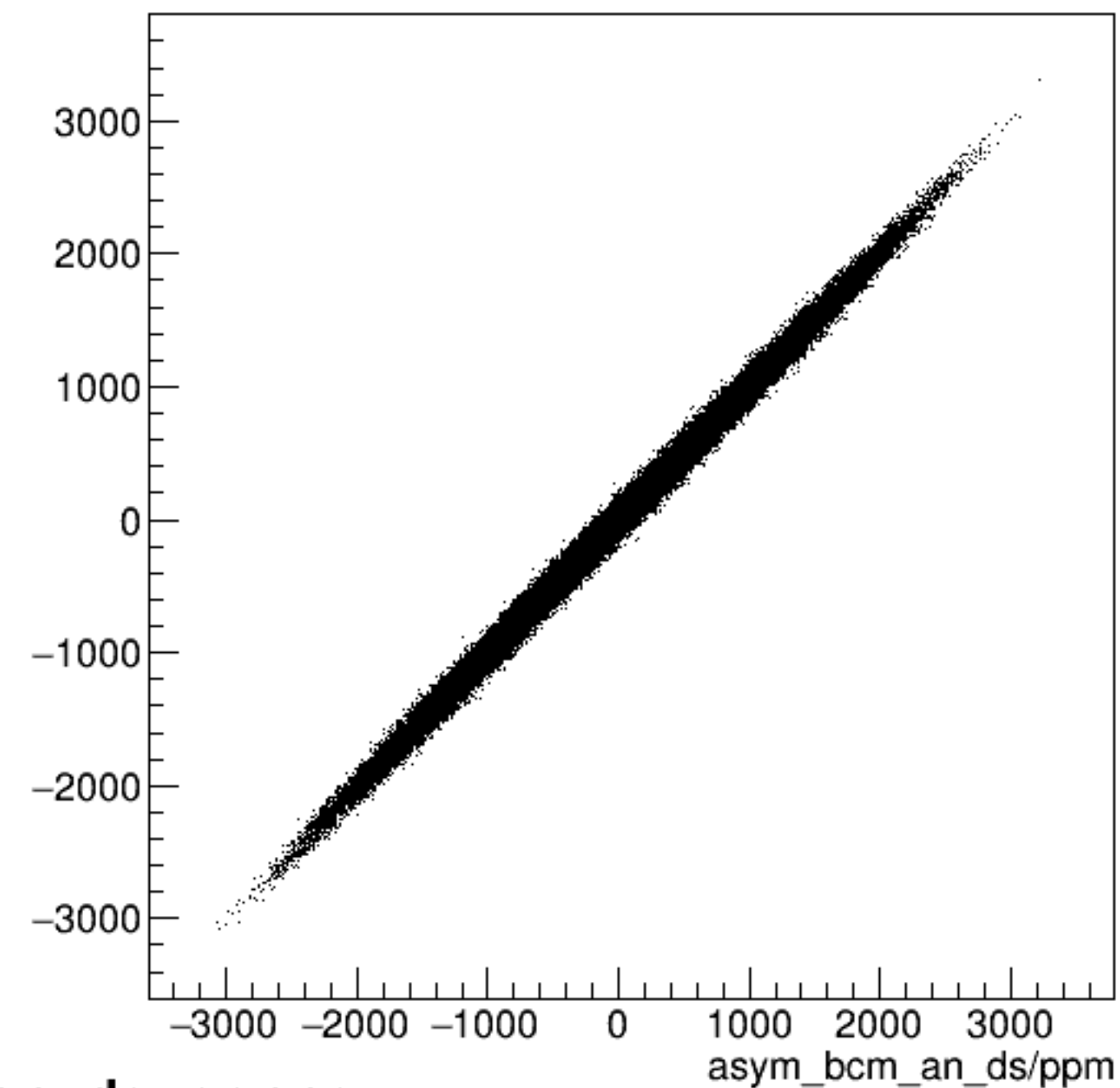
run7660_000_asym_bcm_dg_us_vs_asym_bcm_an_ds_pr.png
