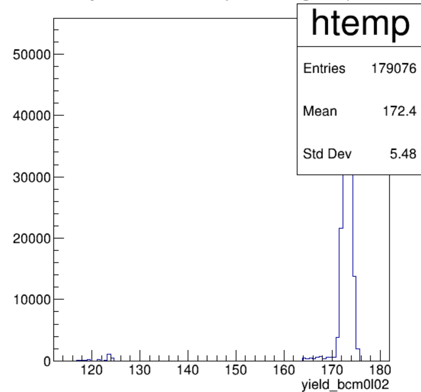
yield_bcm0l02 {ErrorFlag==0}
