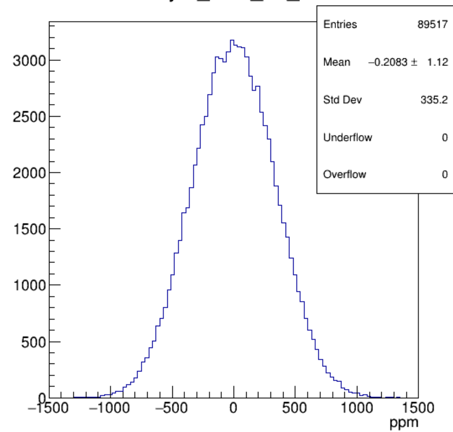
asym_bcm_an_ds
