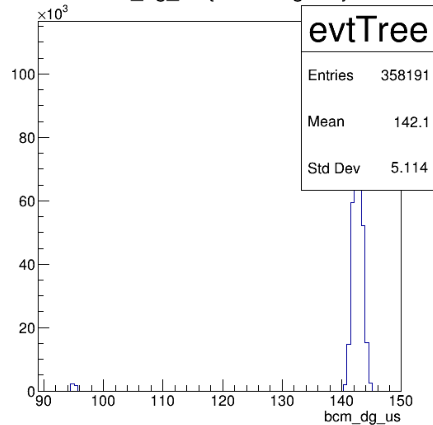
bcm_dg_us {ErrorFlag==0}
