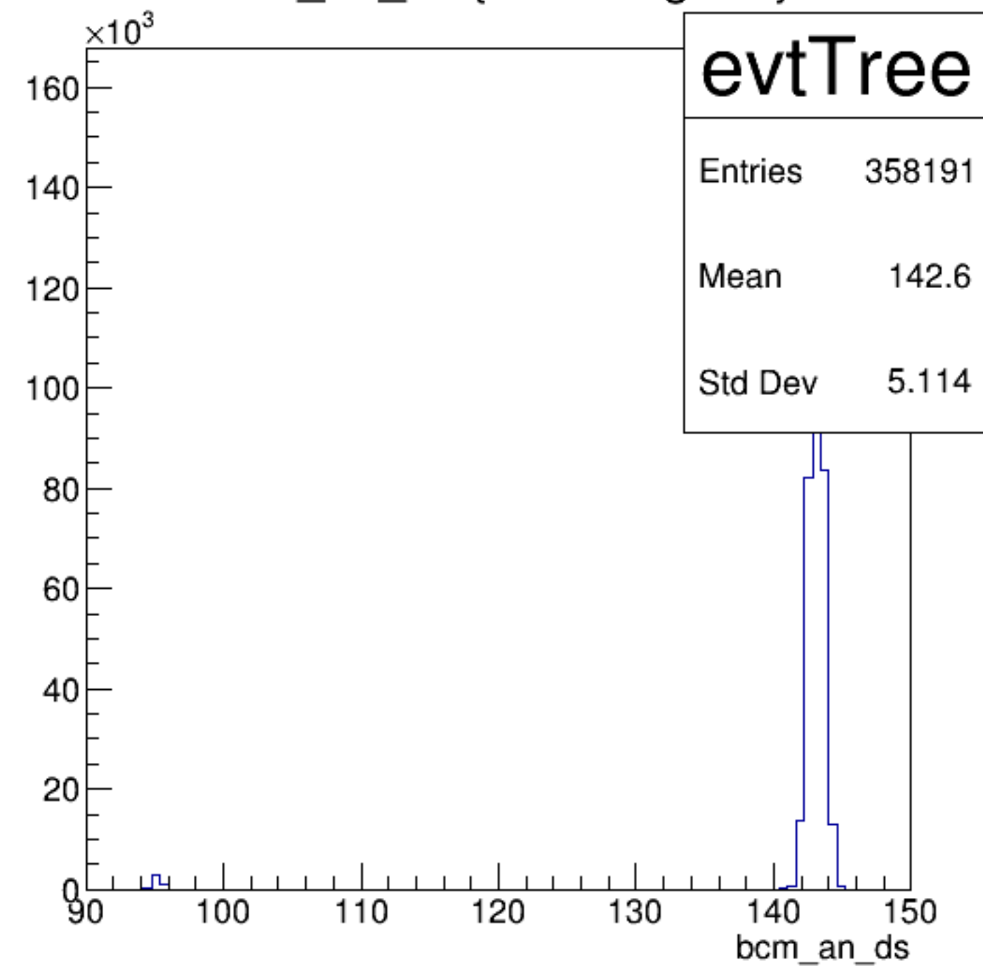
bcm_an_ds {ErrorFlag==0}
