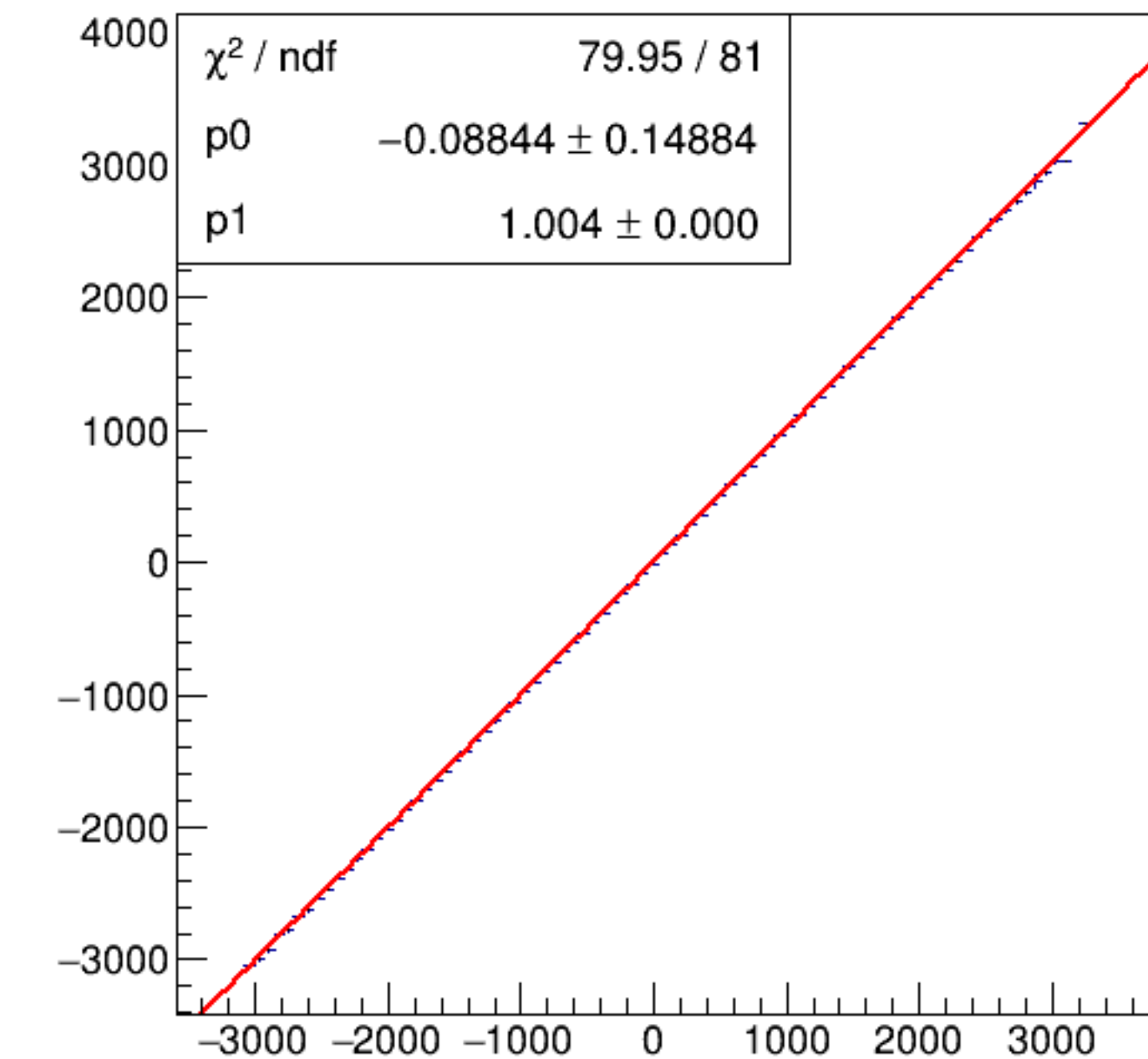
run7660_000_asym_bcm_dg_us_vs_asym_bcm_an_ds_pr.png
