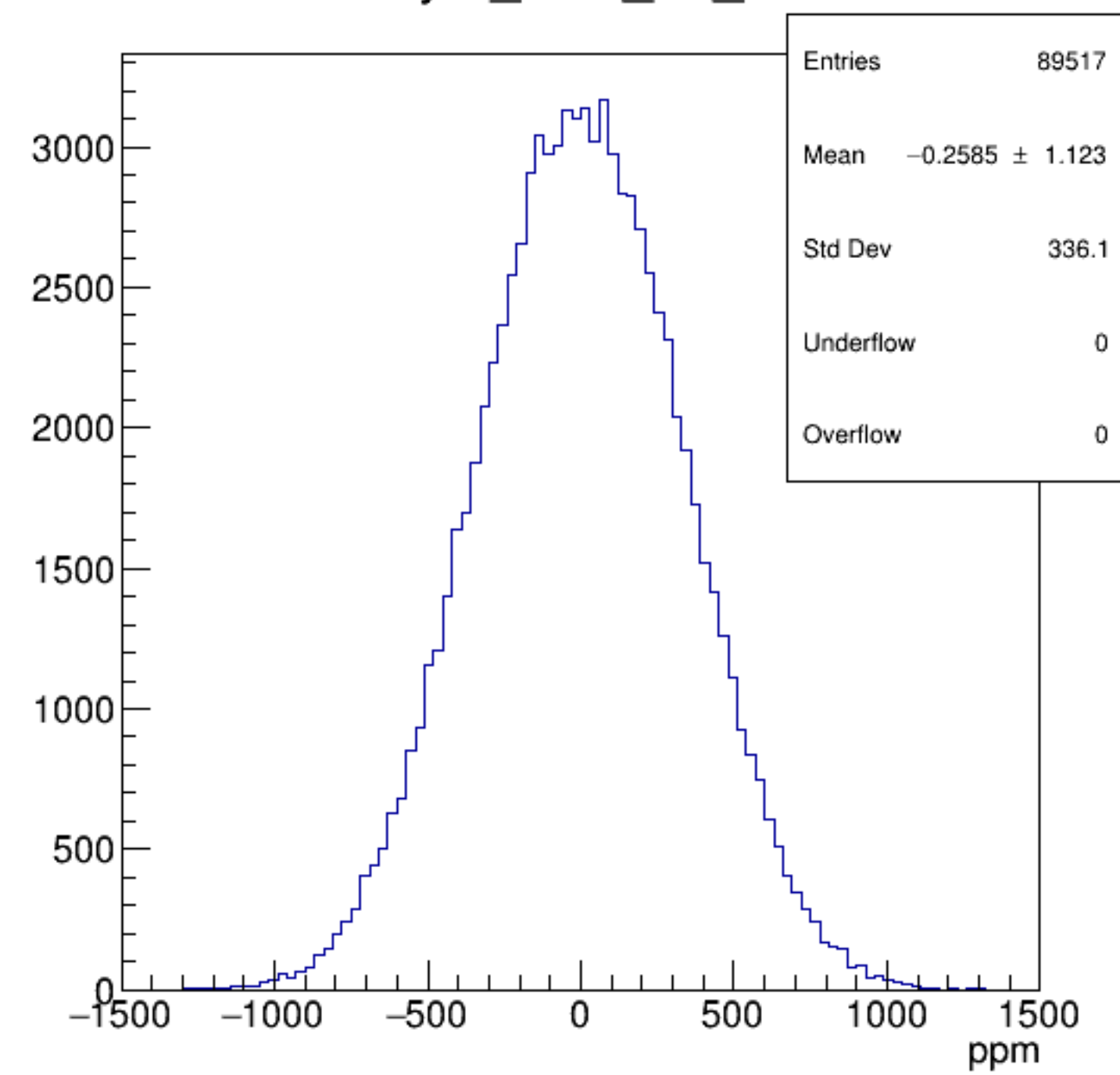
asym_bcm_an_us
