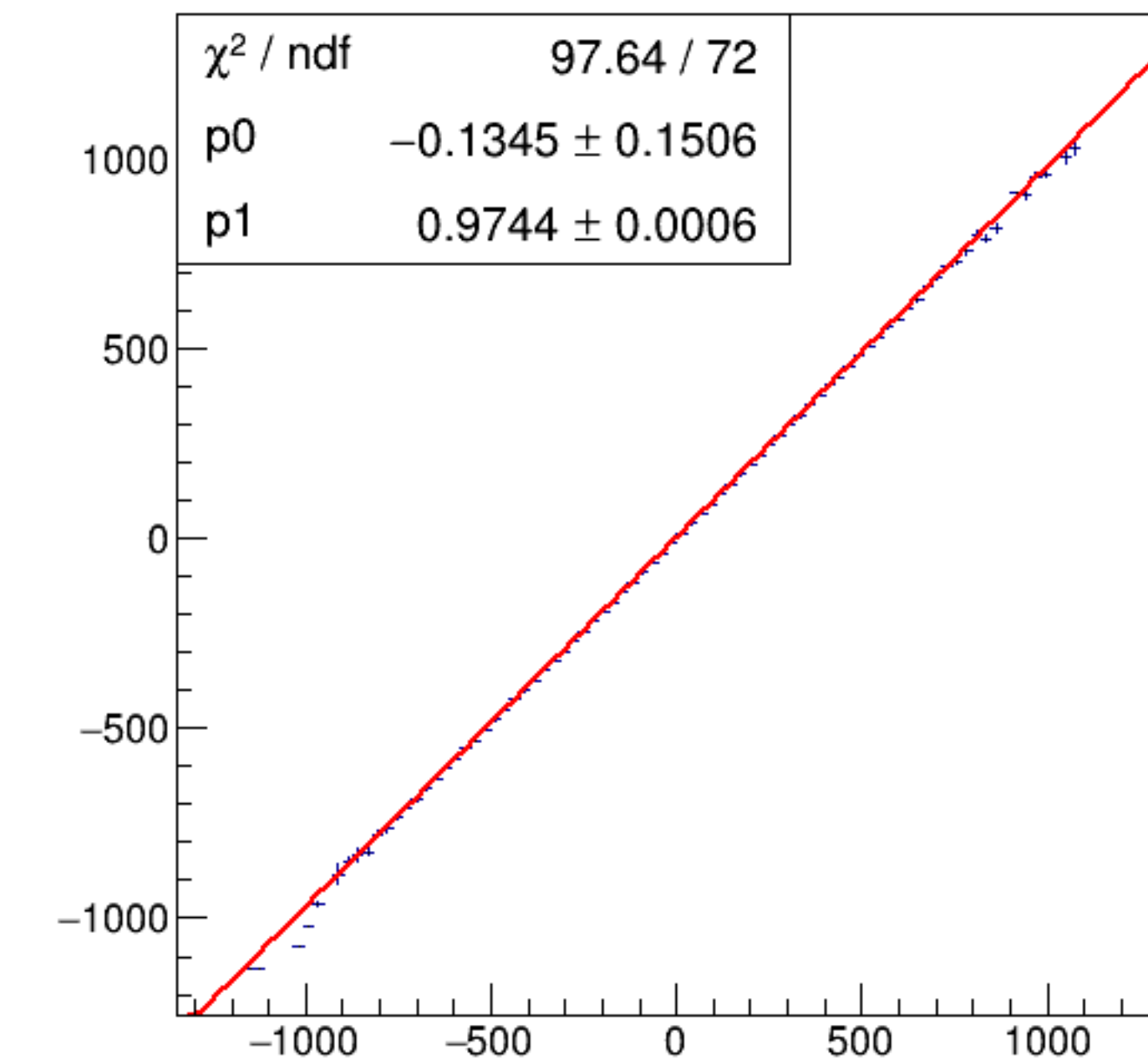
run7687_000_asym_bcm_an_us_vs_asym_bcm_an_ds3_mul.png
