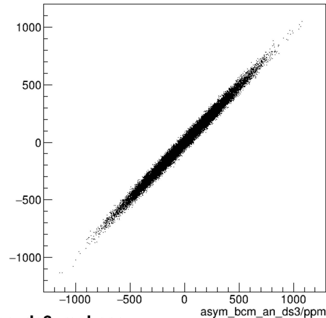
run7687_000_asym_bcm_an_us_vs_asym_bcm_an_ds3_mul.png
