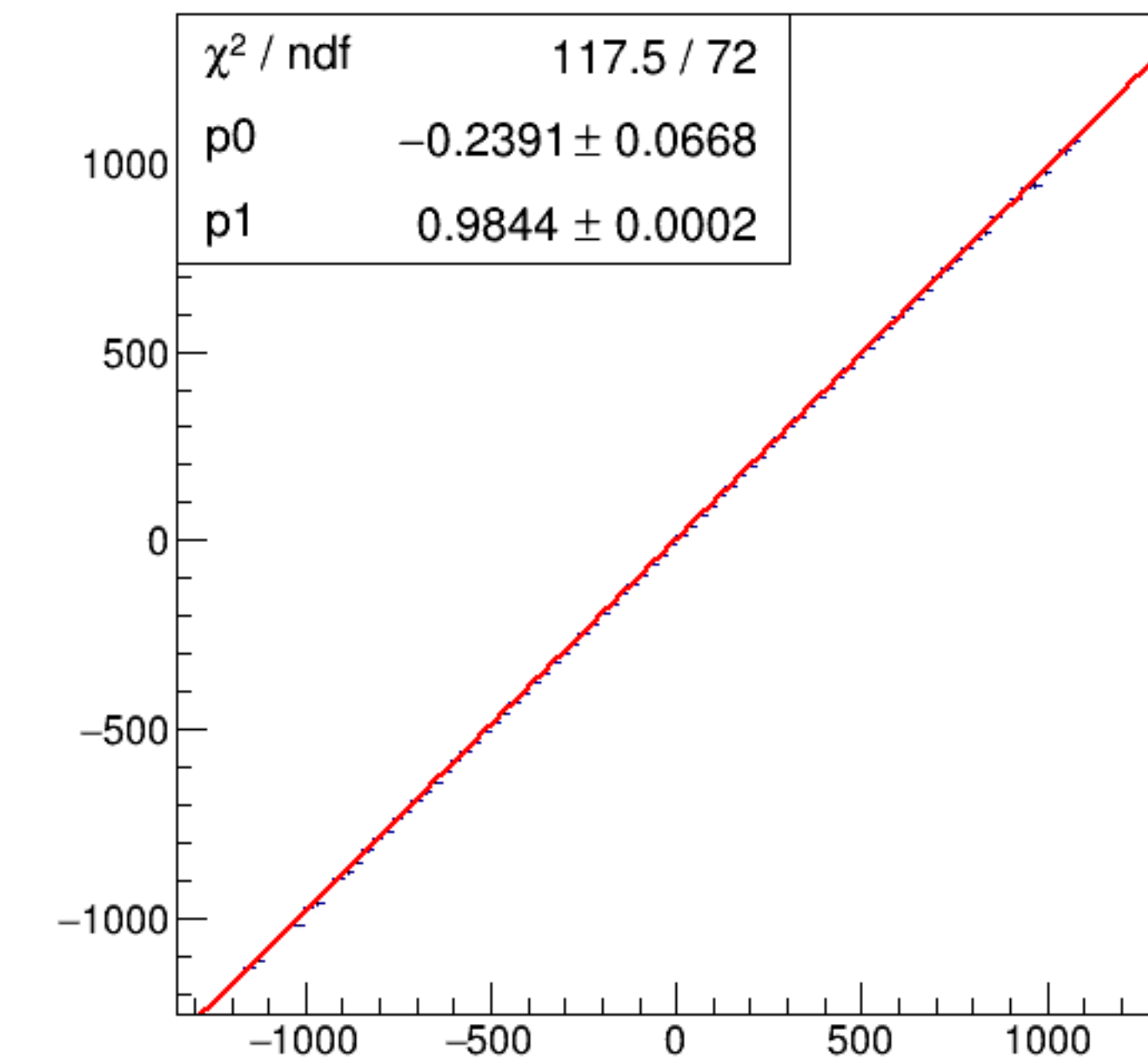
run7687_000_asym_bcm_an_ds_vs_asym_bcm_an_ds3_mul.png
