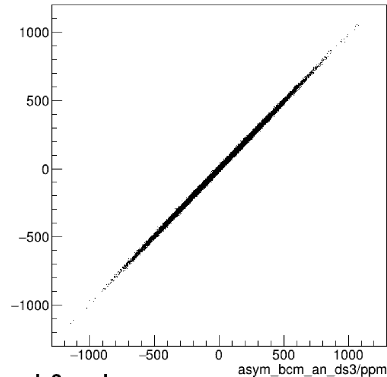
run7687_000_asym_bcm_an_ds_vs_asym_bcm_an_ds3_mul.png
