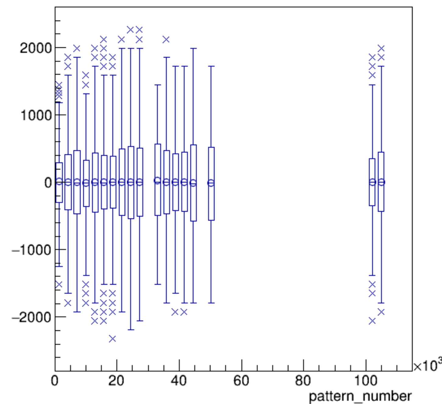
asym_bcm_an_ds3/ppm:pattern_number {ErrorFlag==0}
