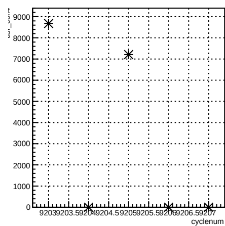
usr_coil4:cyclenum {run == 7697}
