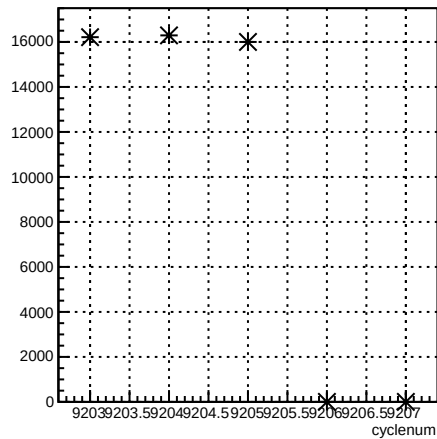
usl_coil6:cyclenum {run == 7697}
