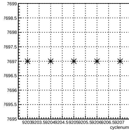
run:cyclenum {run == 7697}
