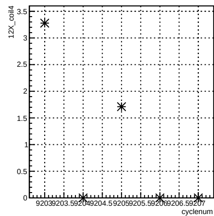
12X_coil4:cyclenum {run == 7697}
