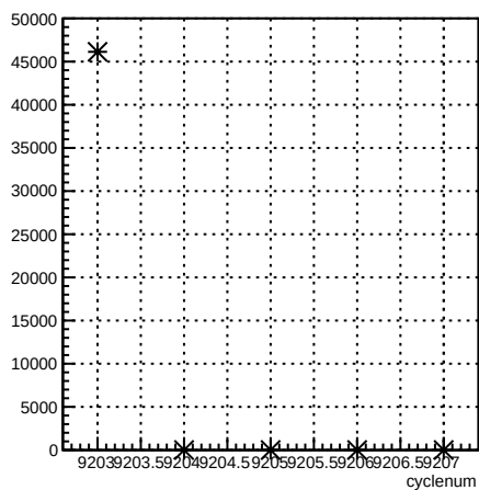
usr_coil7:cyclenum {run == 7697}
