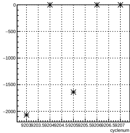
usr_coil3:cyclenum {run == 7697}
