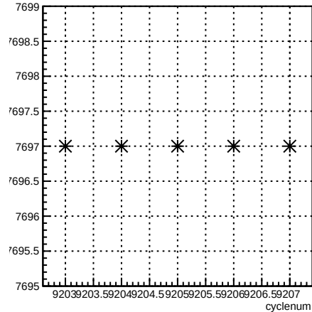
run:cyclenum {run == 7697}
