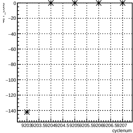
4eY_coil6:cyclenum {run == 7697}
