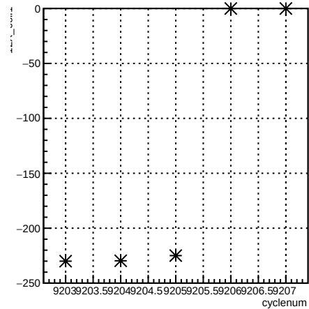
12X_coil1:cyclenum {run == 7697}
