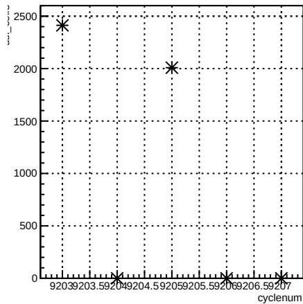
usl_coil7:cyclenum {run == 7697}
