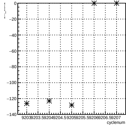
1X_coil1:cyclenum {run == 7697}
