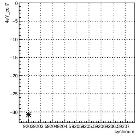
4eY_coil7:cyclenum {run == 7697}
