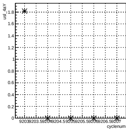
usl_4aY:cyclenum {run == 7697}
