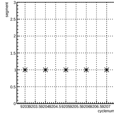
segment:cyclenum {run == 7697}
