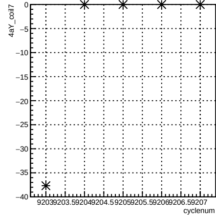
4aY_coil7:cyclenum {run == 7697}
