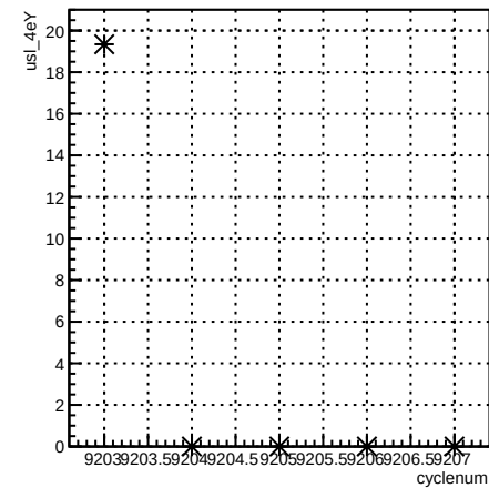
usl_4eY:cyclenum {run == 7697}
