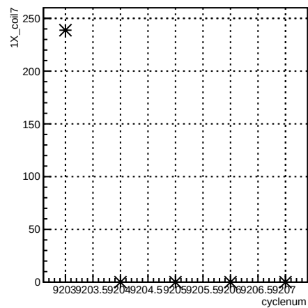
1X_coil7:cyclenum {run == 7697}
