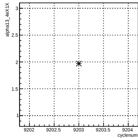
alpha13_4eX1X:cyclenum {run == 7697}
