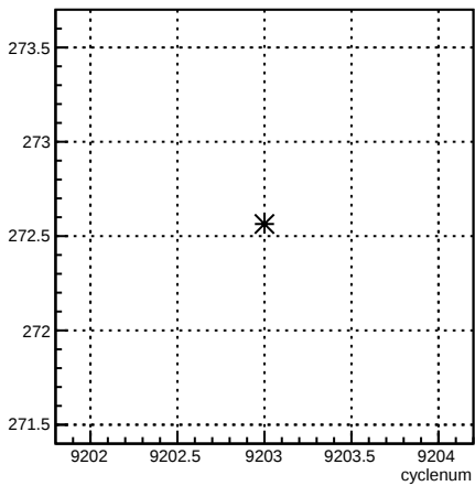
4eY_coil4:cyclenum {run == 7697}
