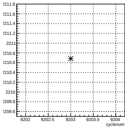
usl_coil3:cyclenum {run == 7697}
