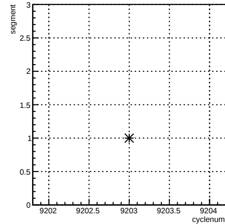
segment:cyclenum {run == 7697}
