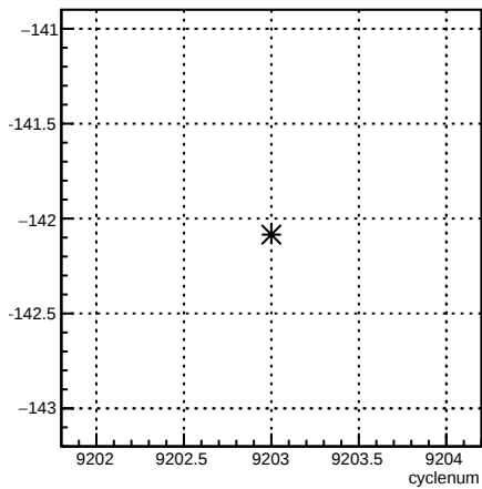
4eY_coil6:cyclenum {run == 7697}
