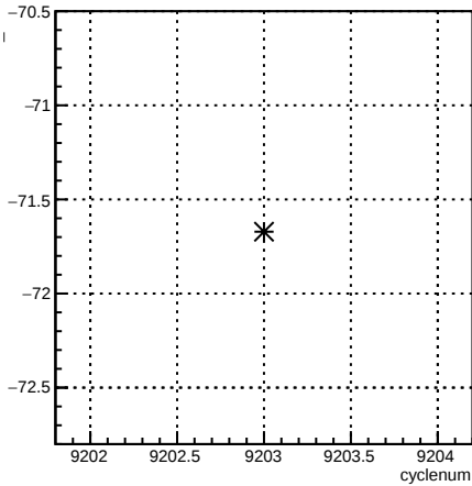
usl_1X:cyclenum {run == 7697}
