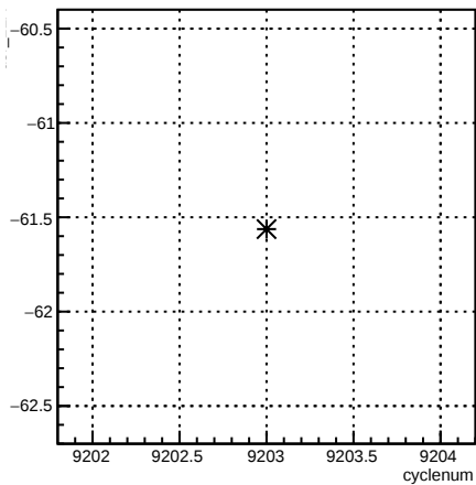
usr_12X:cyclenum {run == 7697}
