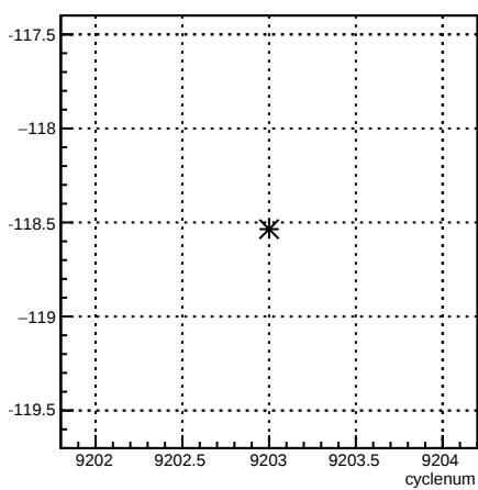
4aY_coil6:cyclenum {run == 7697}
