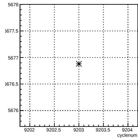
usl_coil4:cyclenum {run == 7697}
