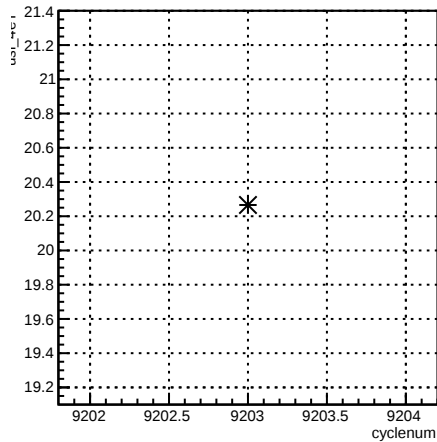
usl_4eY:cyclenum {run == 7697}
