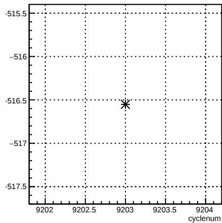
12X_coil7:cyclenum {run == 7697}
