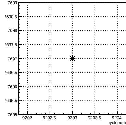
run:cyclenum {run == 7697}
