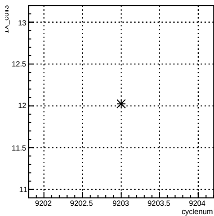
1X_coil3:cyclenum {run == 7697}
