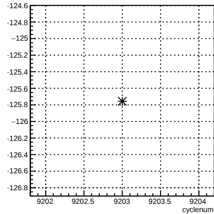
1X_coil1:cyclenum {run == 7697}
