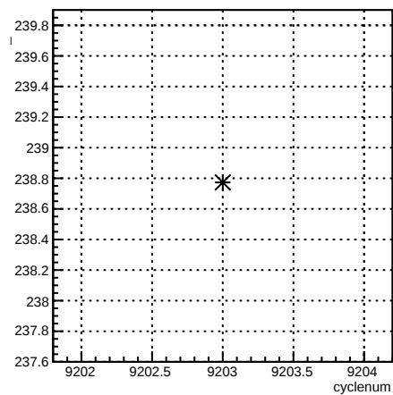
1X_coil7:cyclenum {run == 7697}
