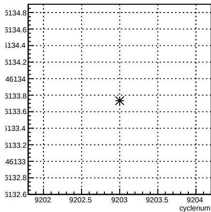
usr_coil7:cyclenum {run == 7697}
