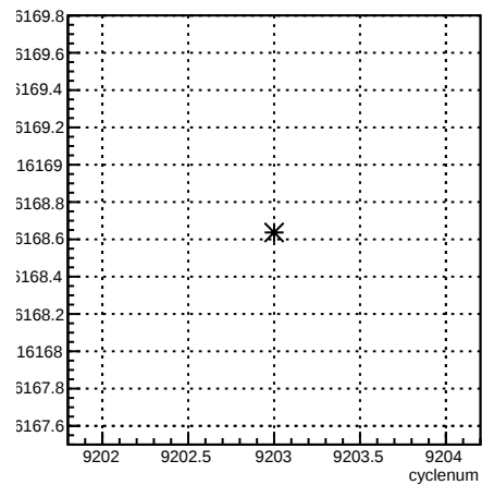
usl_coil1:cyclenum {run == 7697}
