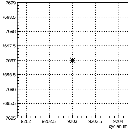
run:cyclenum {run == 7697}
