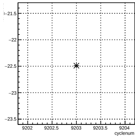
4eX_coil3:cyclenum {run == 7697}
