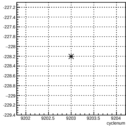
12X_coil6:cyclenum {run == 7697}
