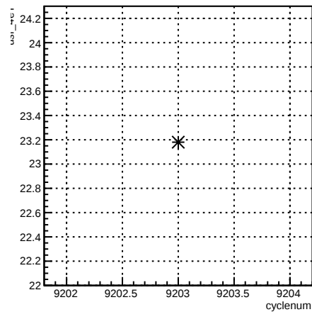
usr_4eY:cyclenum {run == 7697}
