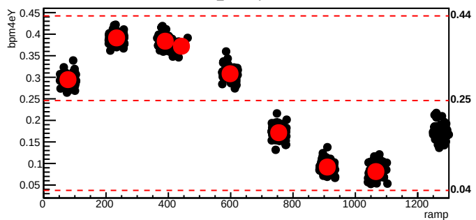
bmod_trim4,cyc=9203
