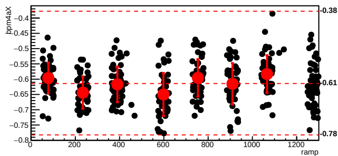
bmod_trim3,cyc=9203
