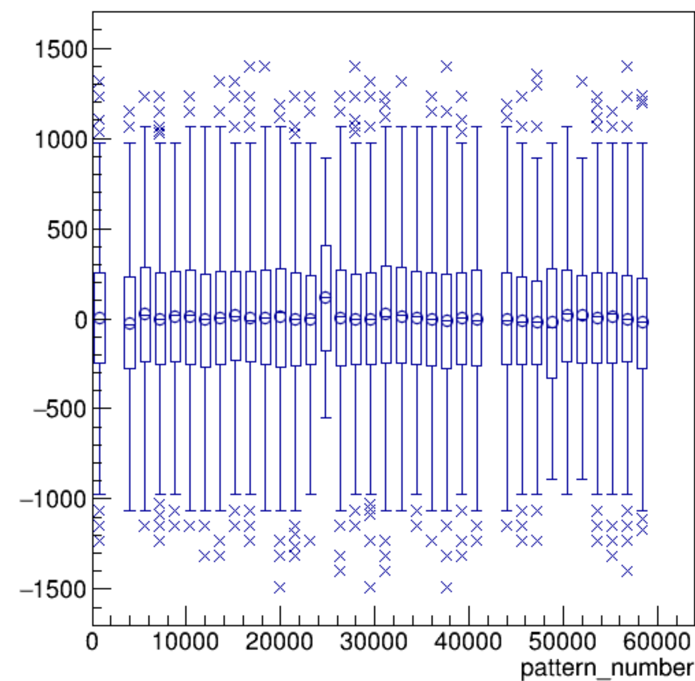
asym_dsr/ppm:pattern_number {ErrorFlag==0}
