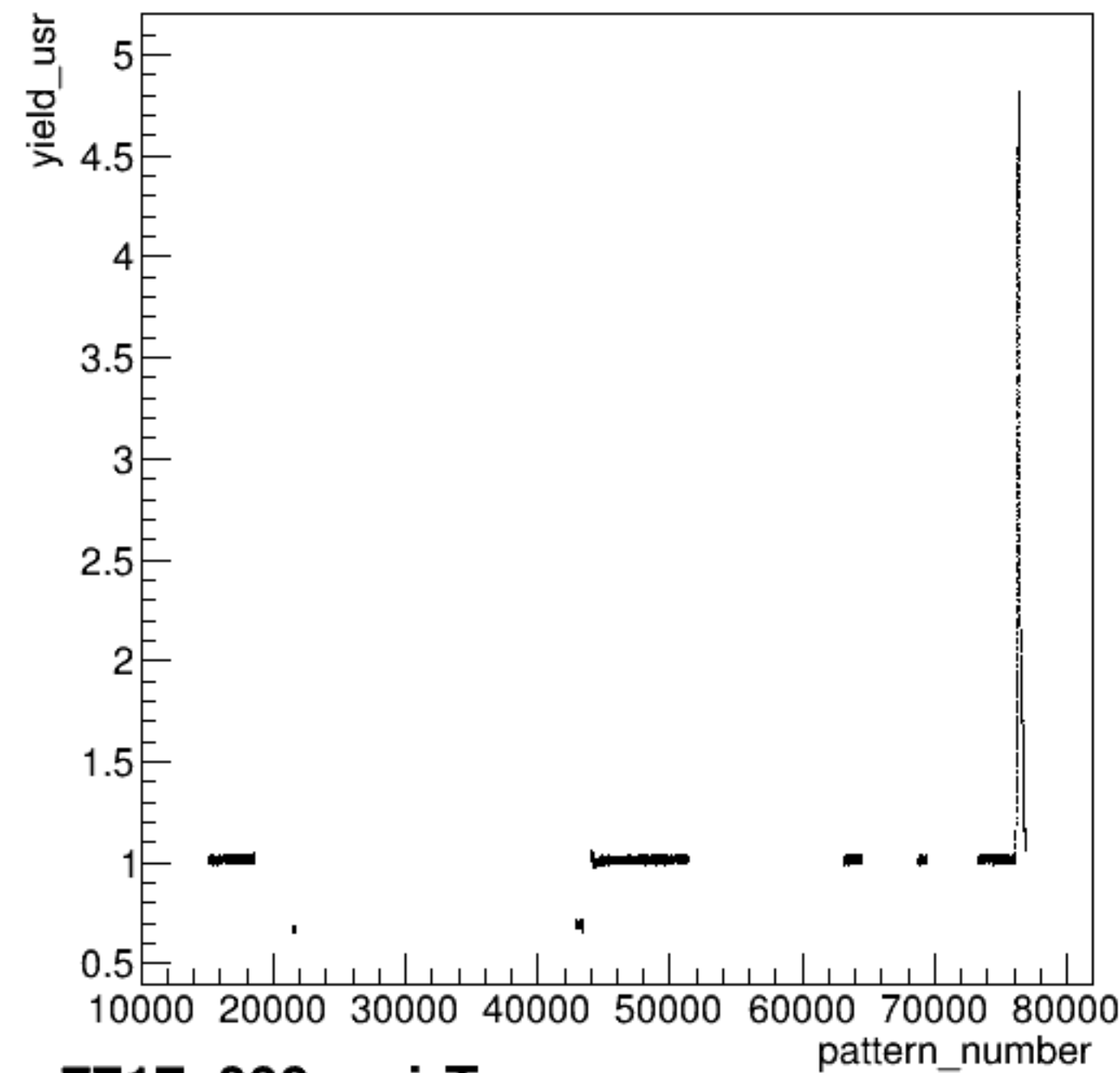
yield_usr:pattern_number {ErrorFlag==0}
