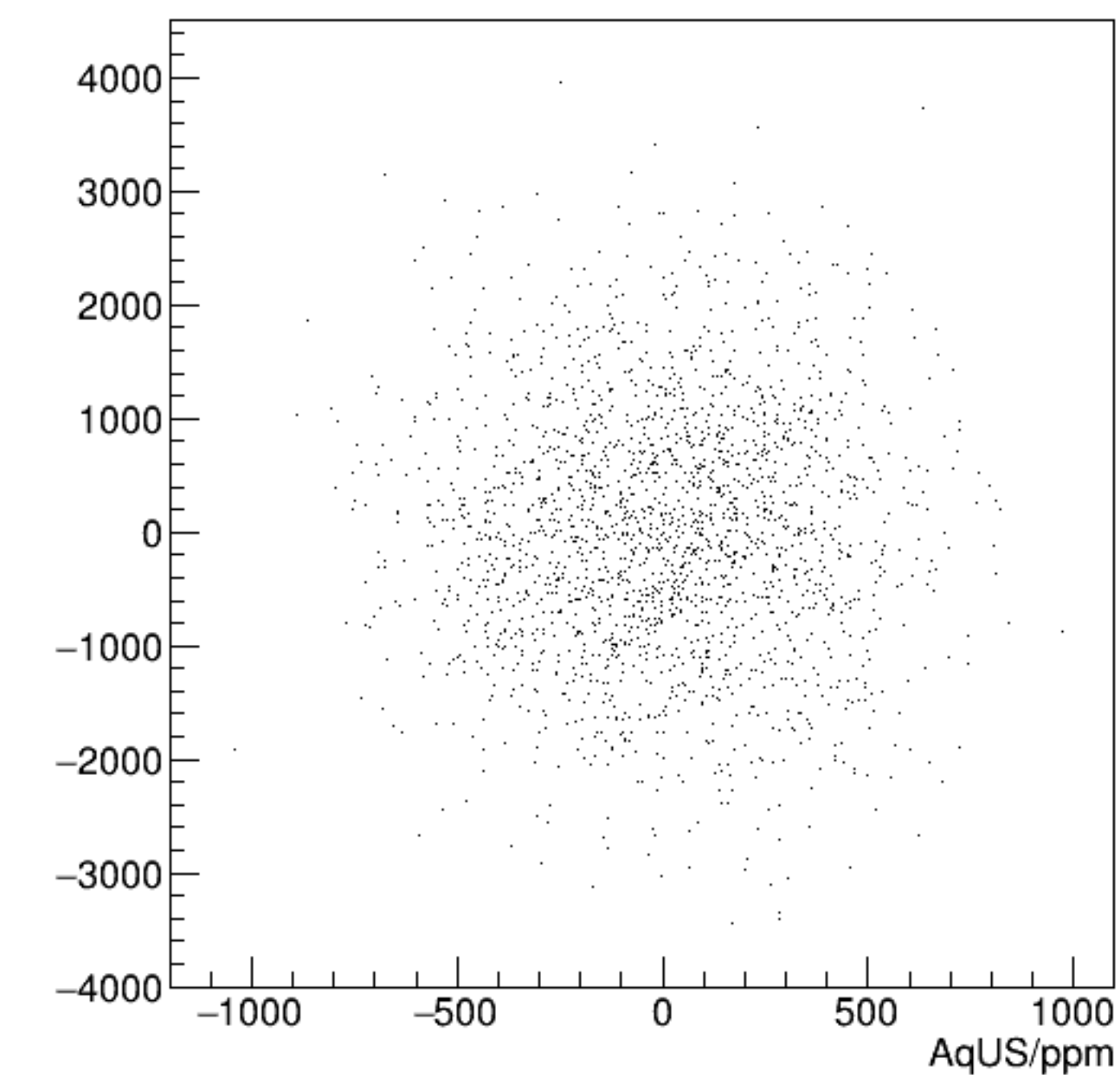
reg_asym_usl/ppm:AqUS/ppm {ok_cut}
