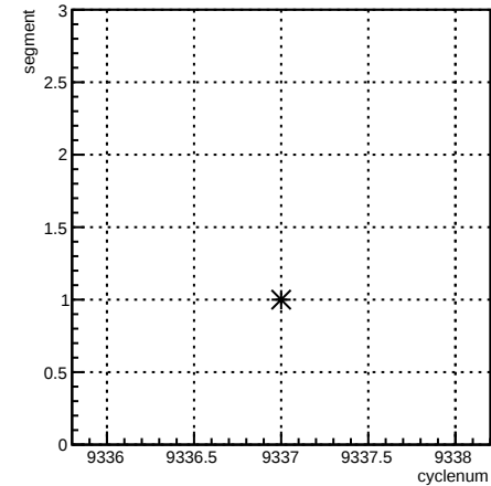
segment:cyclenum {run == 7765}
