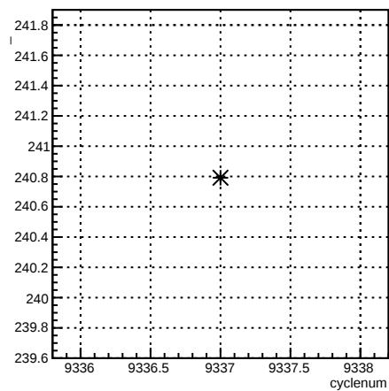
1X_coil7:cyclenum {run == 7765}
