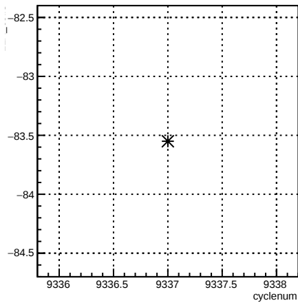
12X_coil7:cyclenum {run == 7765}
