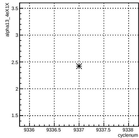
alpha13_4eX1X:cyclenum {run == 7765}
