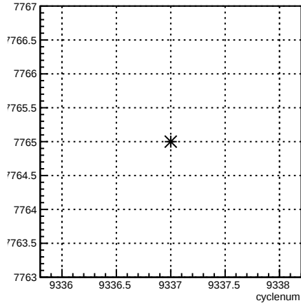
run:cyclenum {run == 7765}
