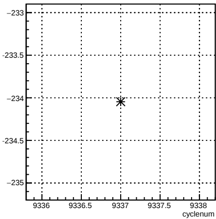
12X_coil6:cyclenum {run == 7765}
