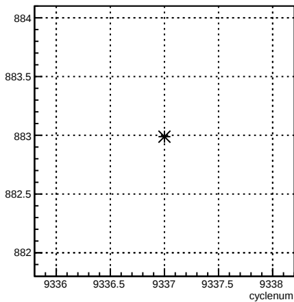
usr_coil6:cyclenum {run == 7765}
