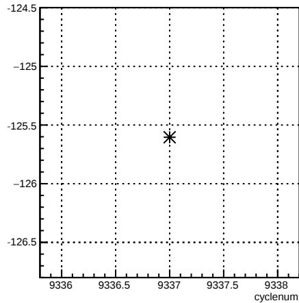
1X_coil1:cyclenum {run == 7765}
