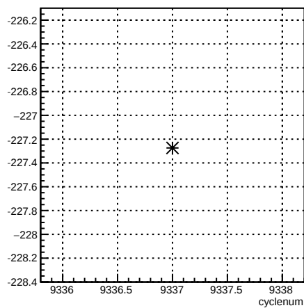
4eX_coil1:cyclenum {run == 7765}
