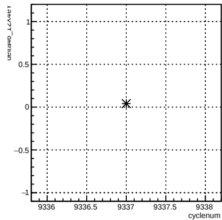
delta46_12X4eY:cyclenum {run == 7765}
