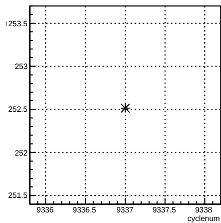
4eX_coil7:cyclenum {run == 7765}
