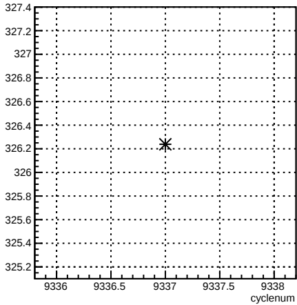
4aY_coil4:cyclenum {run == 7765}
