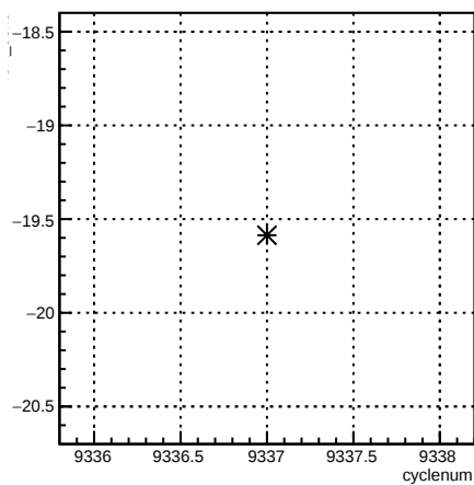
4eX_coil3:cyclenum {run == 7765}
