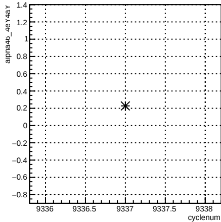
alpha46_4eY4aY:cyclenum {run == 7765}
