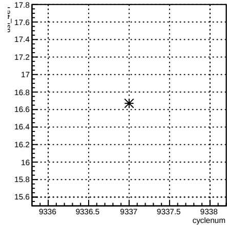
usl_4eY:cyclenum {run == 7765}
