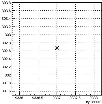
4eY_coil4:cyclenum {run == 7765}
