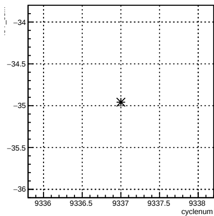
4eY_coil7:cyclenum {run == 7765}
