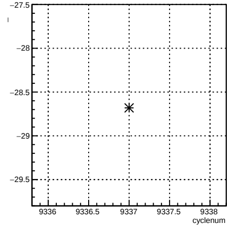
usr_4eY:cyclenum {run == 7765}
