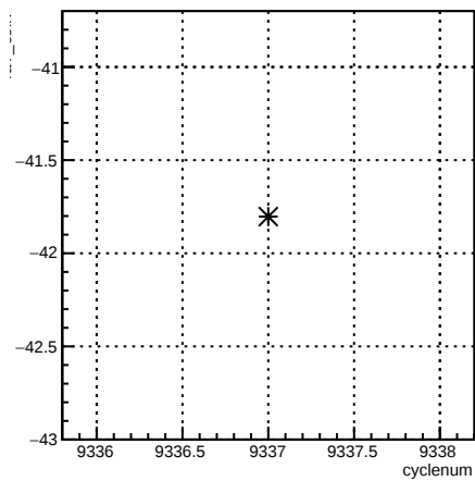
4aY_coil7:cyclenum {run == 7765}
