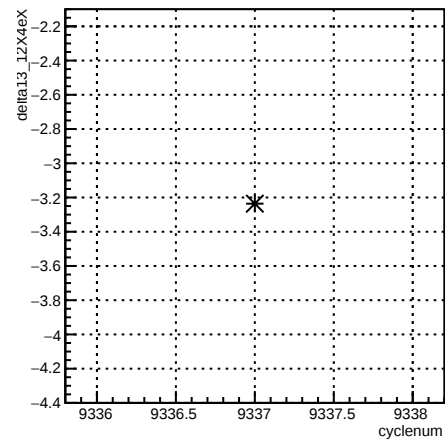
delta13_12X4eX:cyclenum {run == 7765}
