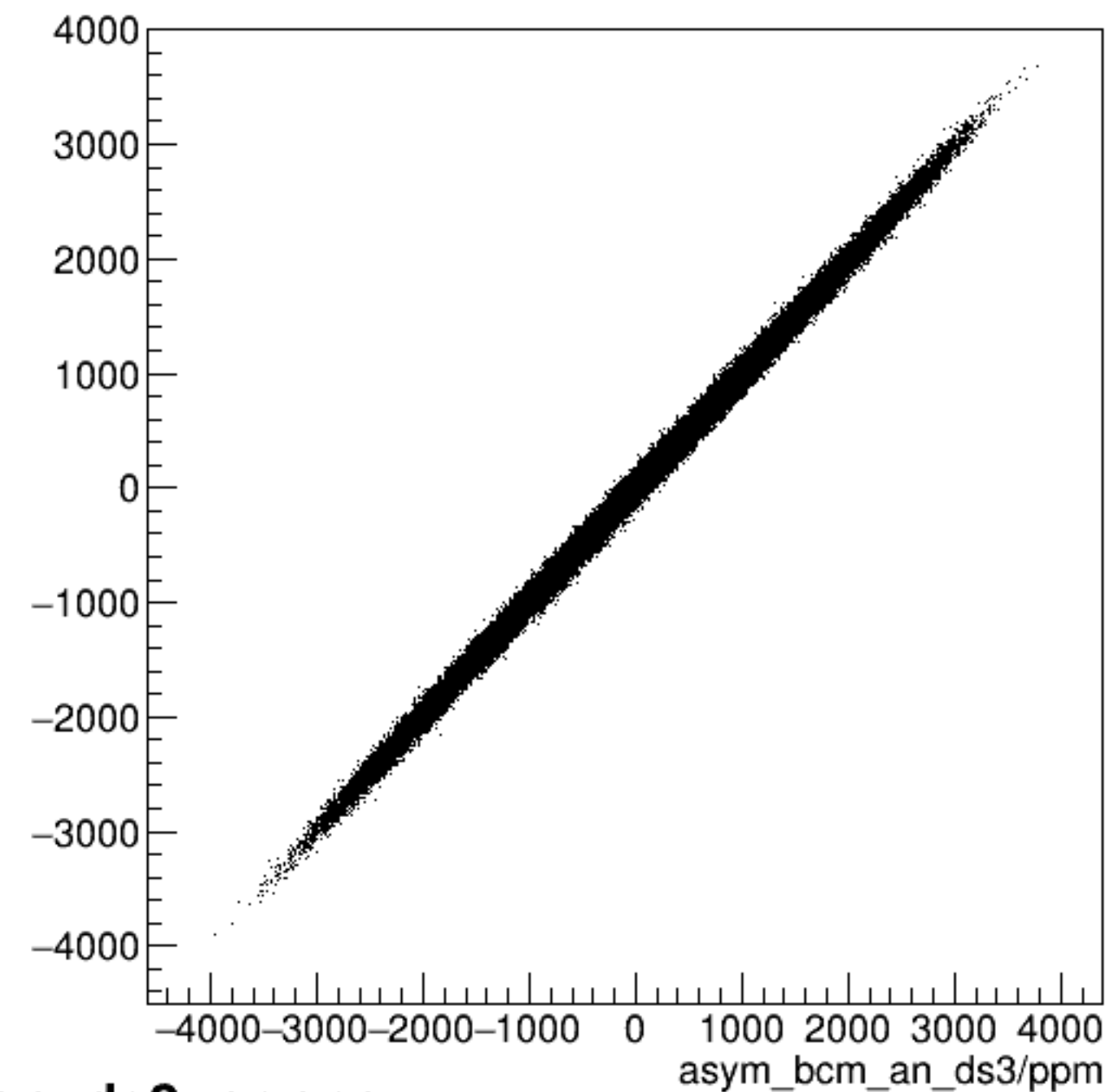
run7783_000_asym_bcm_dg_us_vs_asym_bcm_an_ds3_pr.png
