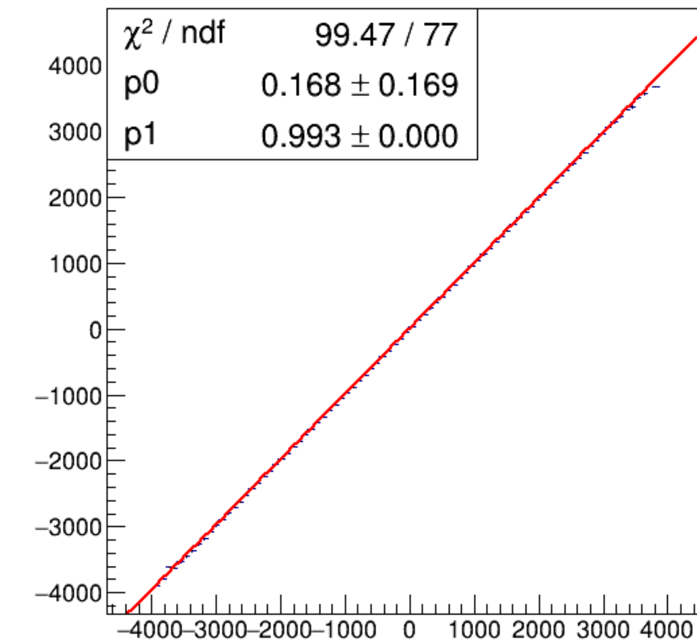
run7783_000_asym_bcm_dg_us_vs_asym_bcm_an_ds3_pr.png
