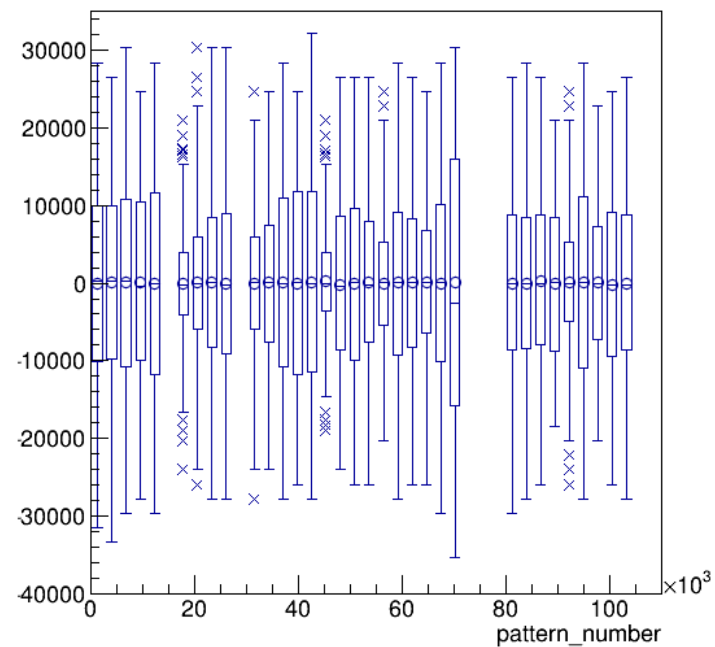
asym_sam3/ppm:pattern_number {ErrorFlag==0}
