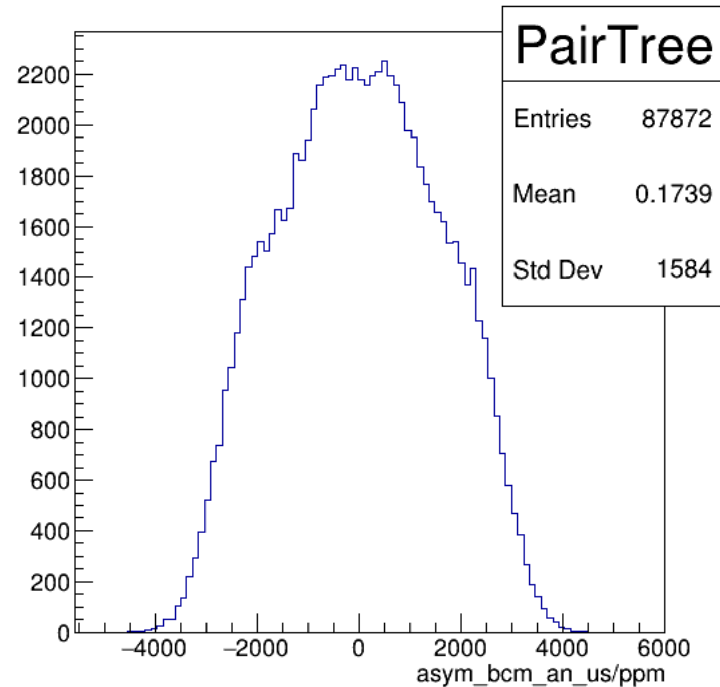
asym_bcm_an_us/ppm {ErrorFlag==0}
