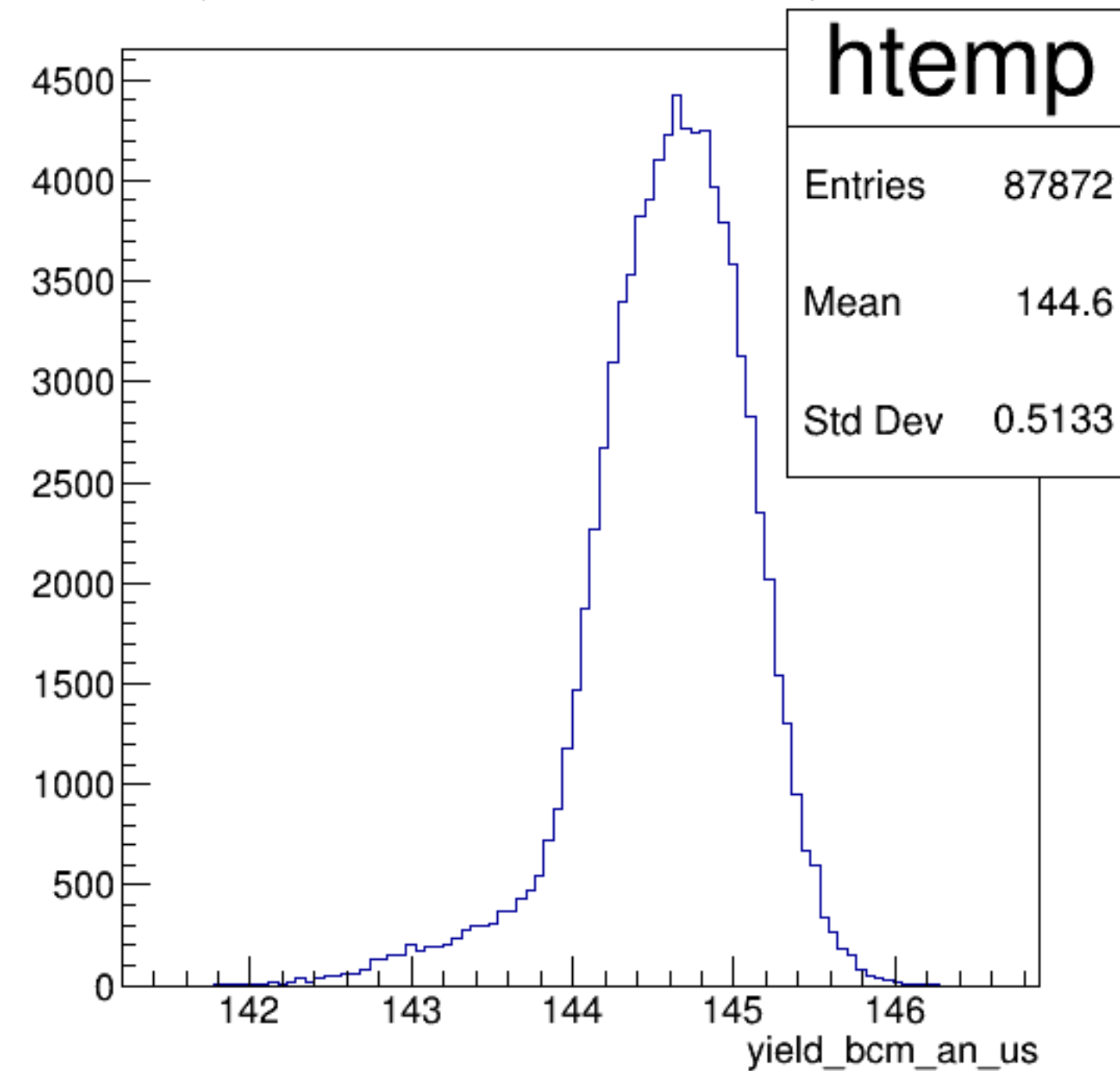
yield_bcm_an_us {ErrorFlag==0}
