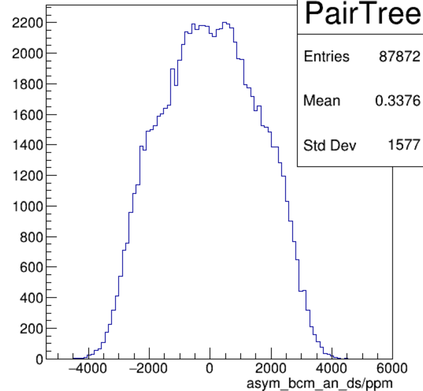
asym_bcm_an_ds/ppm {ErrorFlag==0}
