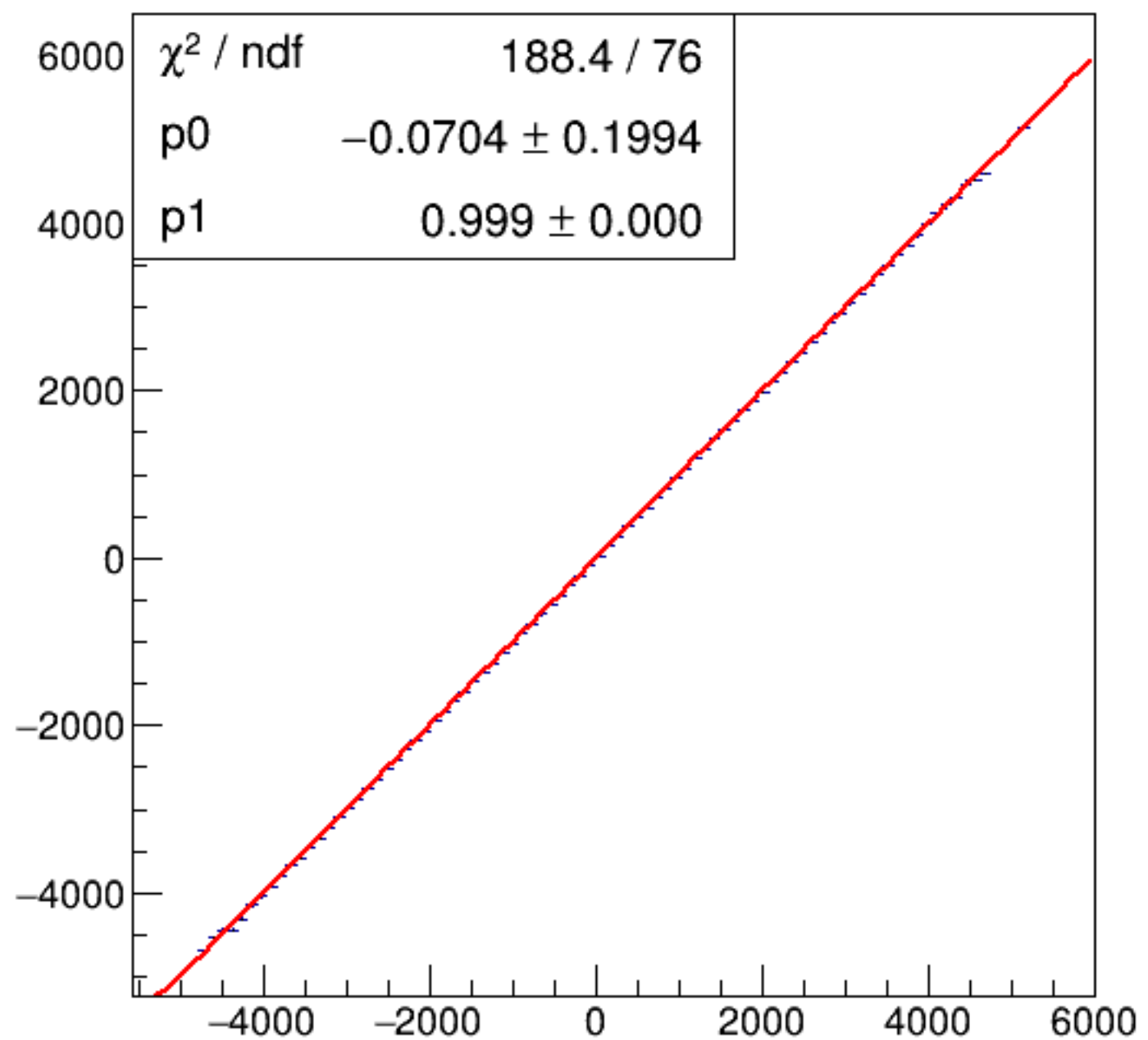
run7790_000_asym_bcm_dg_ds_vs_asym_bcm_an_us_pr.png
