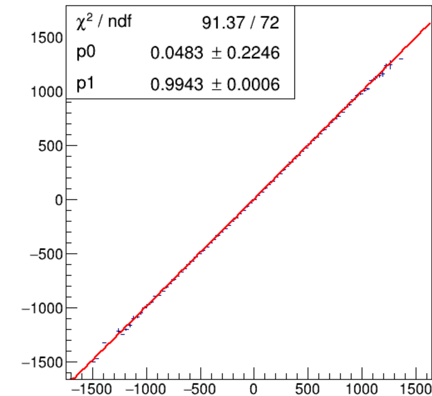
run7790_000_asym_bcm_dg_us_vs_asym_bcm_an_ds3_mul.png
