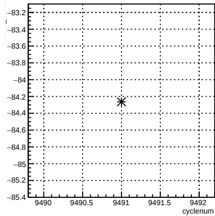
12X_coil7:cyclenum {run == 7808}
