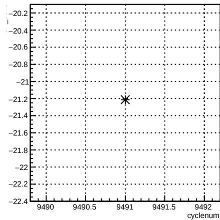
4eX_coil3:cyclenum {run == 7808}
