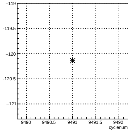
1X_coil1:cyclenum {run == 7808}
