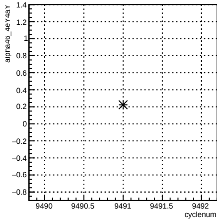
alpha46_4eY4aY:cyclenum {run == 7808}
