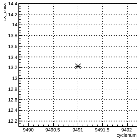
1X_coil3:cyclenum {run == 7808}
