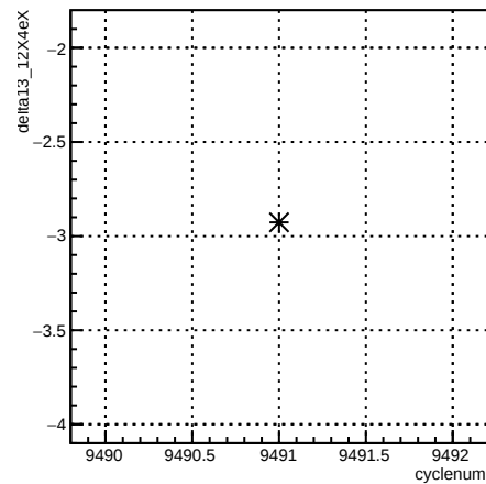
delta13_12X4eX:cyclenum {run == 7808}
