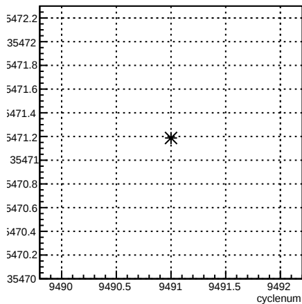
usr_coil7:cyclenum {run == 7808}
