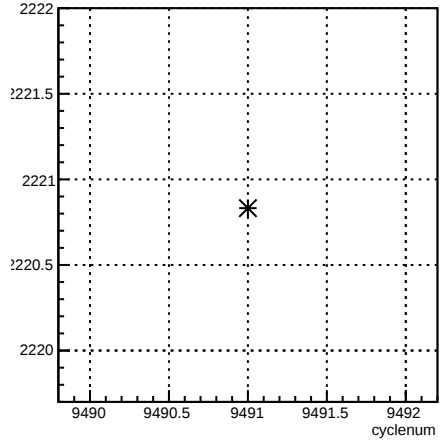
usl_coil7:cyclenum {run == 7808}
