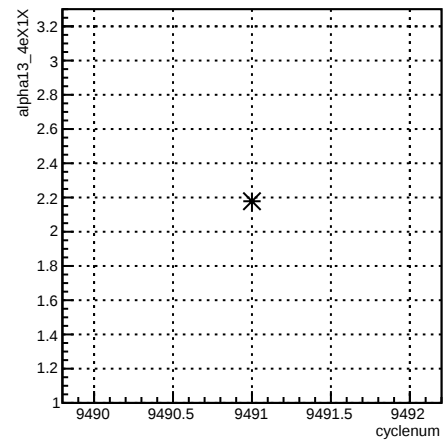
alpha13_4eX1X:cyclenum {run == 7808}
