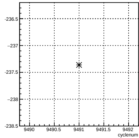
12X_coil6:cyclenum {run == 7808}
