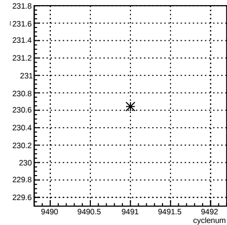
1X_coil7:cyclenum {run == 7808}
