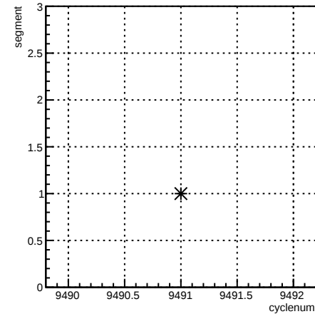
segment:cyclenum {run == 7808}
