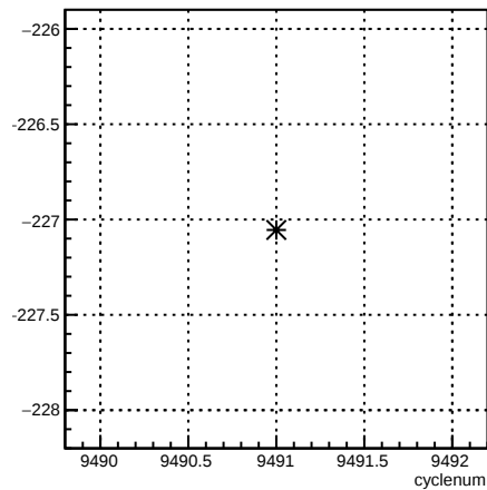
4eX_coil1:cyclenum {run == 7808}
