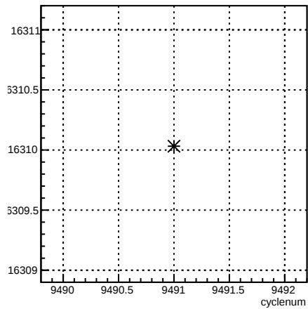
usl_coil6:cyclenum {run == 7808}
