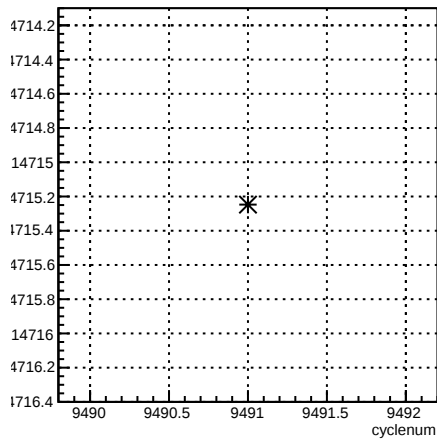
usr_coil6:cyclenum {run == 7808}
