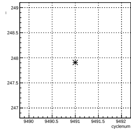
4eX_coil7:cyclenum {run == 7808}
