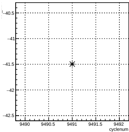
usr_12X:cyclenum {run == 7808}
