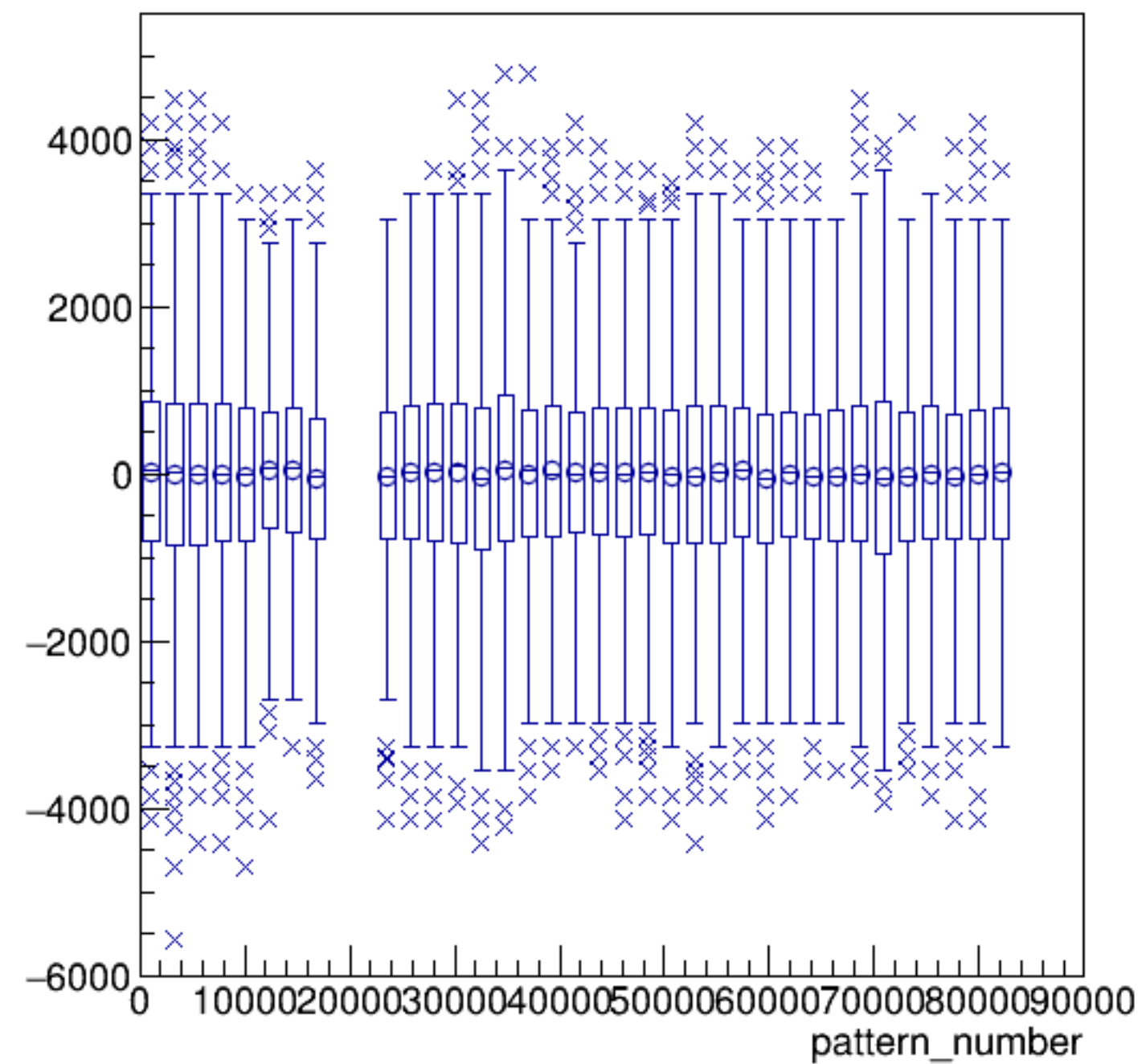
asym_sam7/ppm:pattern_number {ErrorFlag==0}
