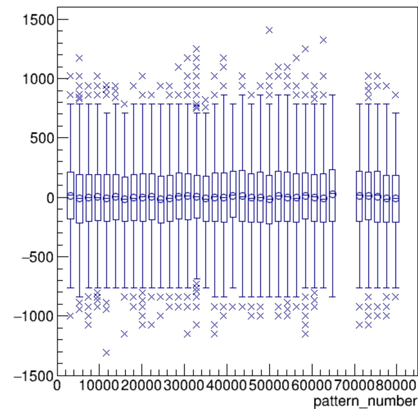
asym_dsl/ppm:pattern_number {ErrorFlag==0}
