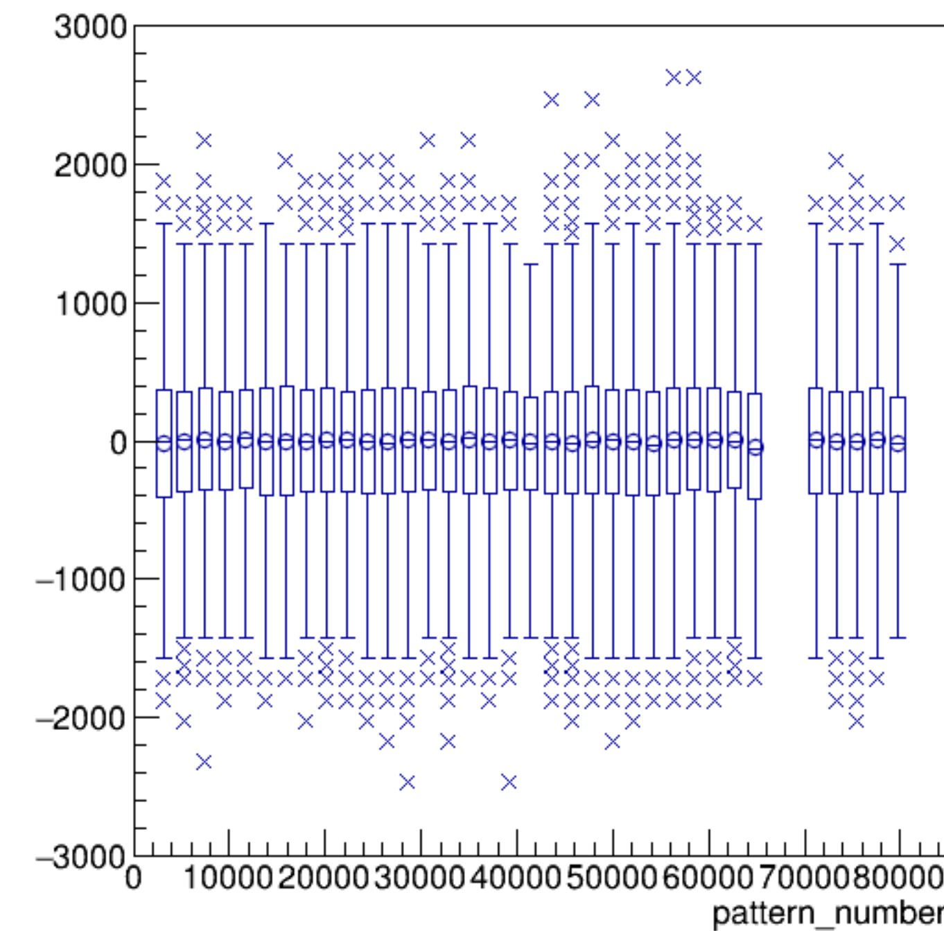
asym_dsr/ppm:pattern_number {ErrorFlag==0}
