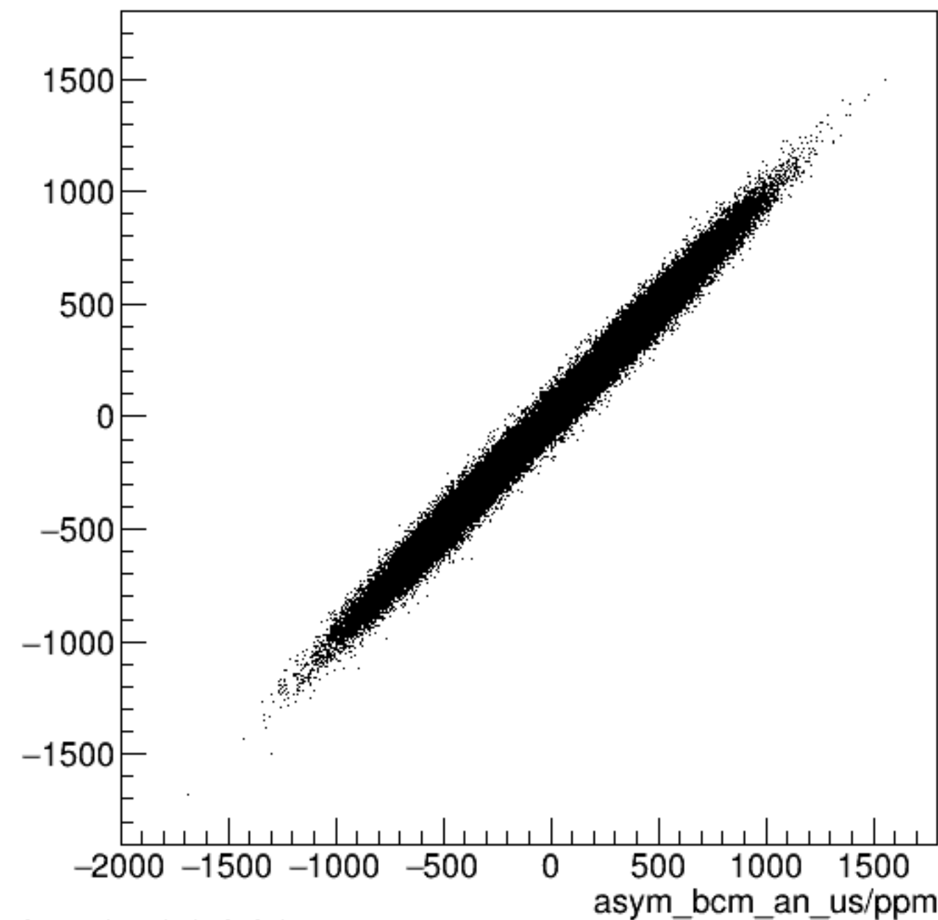
run7849_000_asym_bcm_dg_ds_vs_asym_bcm_an_us_pr.png
