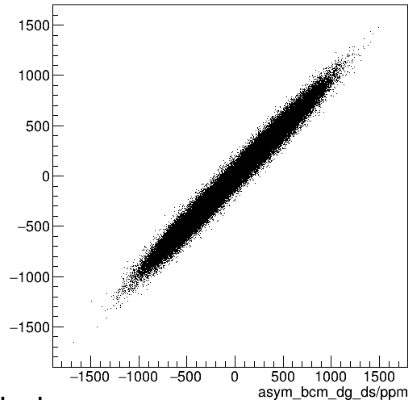
run7849_000_asym_bcm_dg_us_vs_asym_bcm_dg_ds_pr.png
