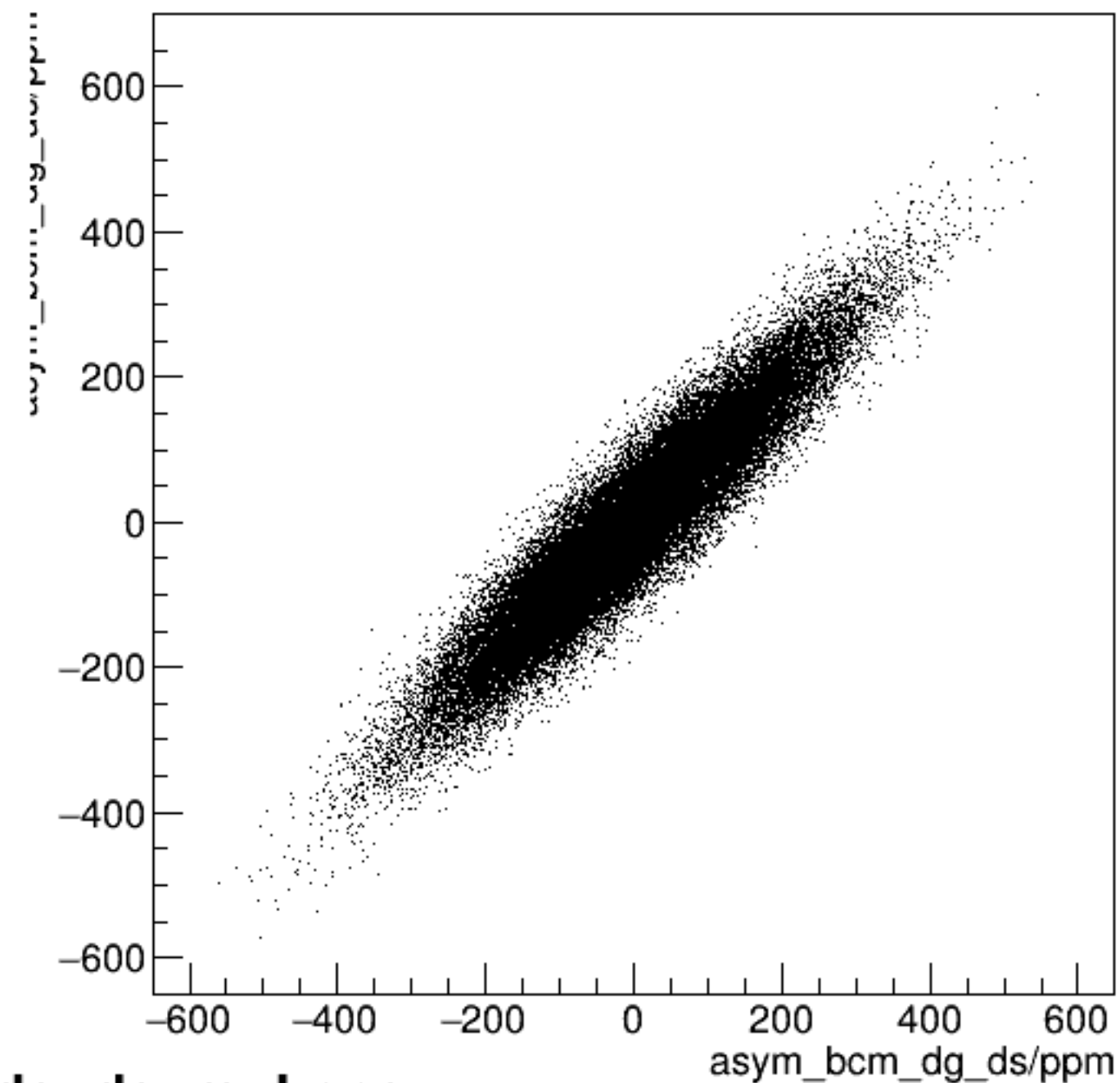
run7849_000_asym_bcm_dg_us_vs_asym_bcm_dg_ds_mul.png
