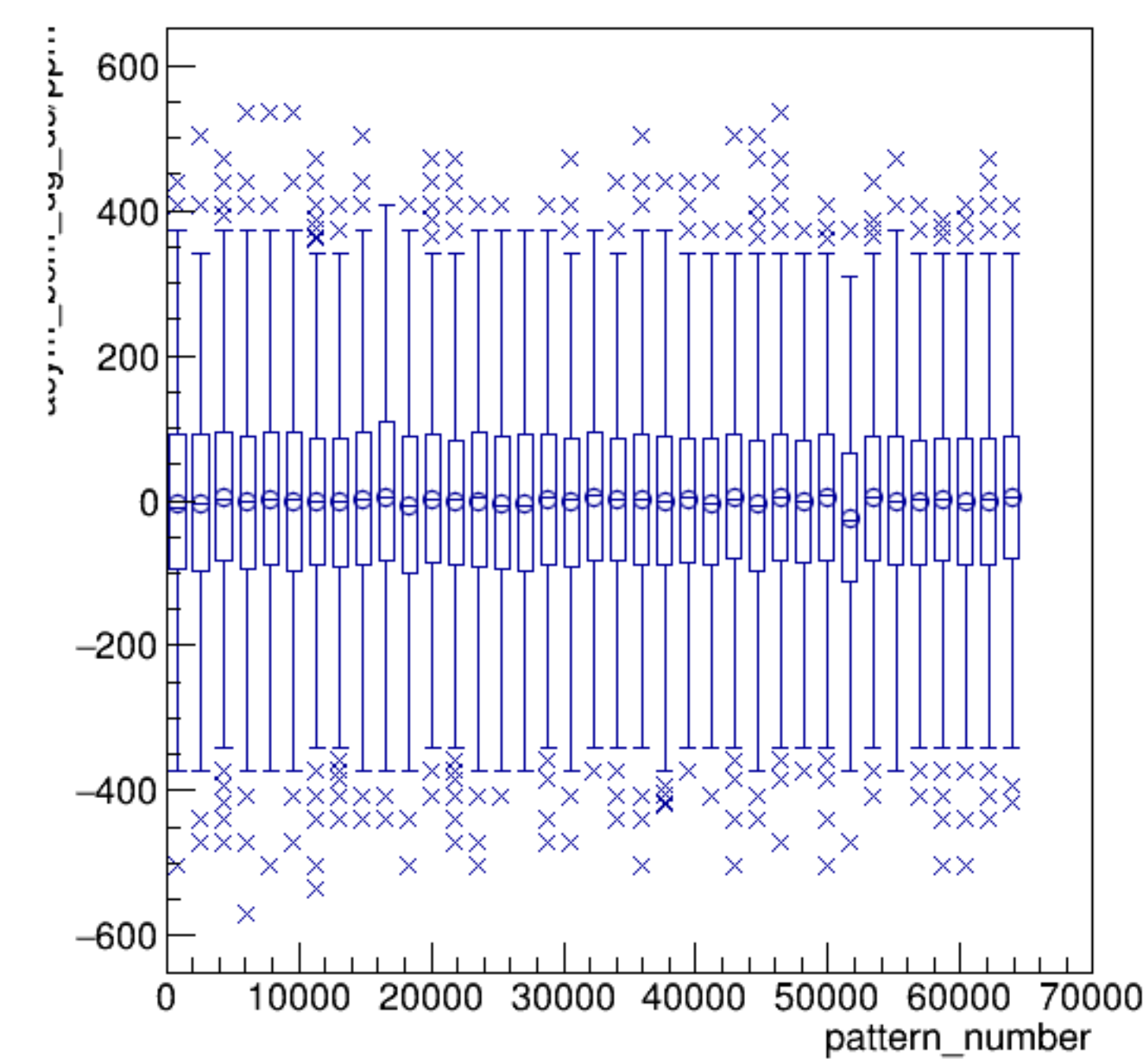
asym_bcm_dg_ds/ppm:pattern_number {ErrorFlag==0}
