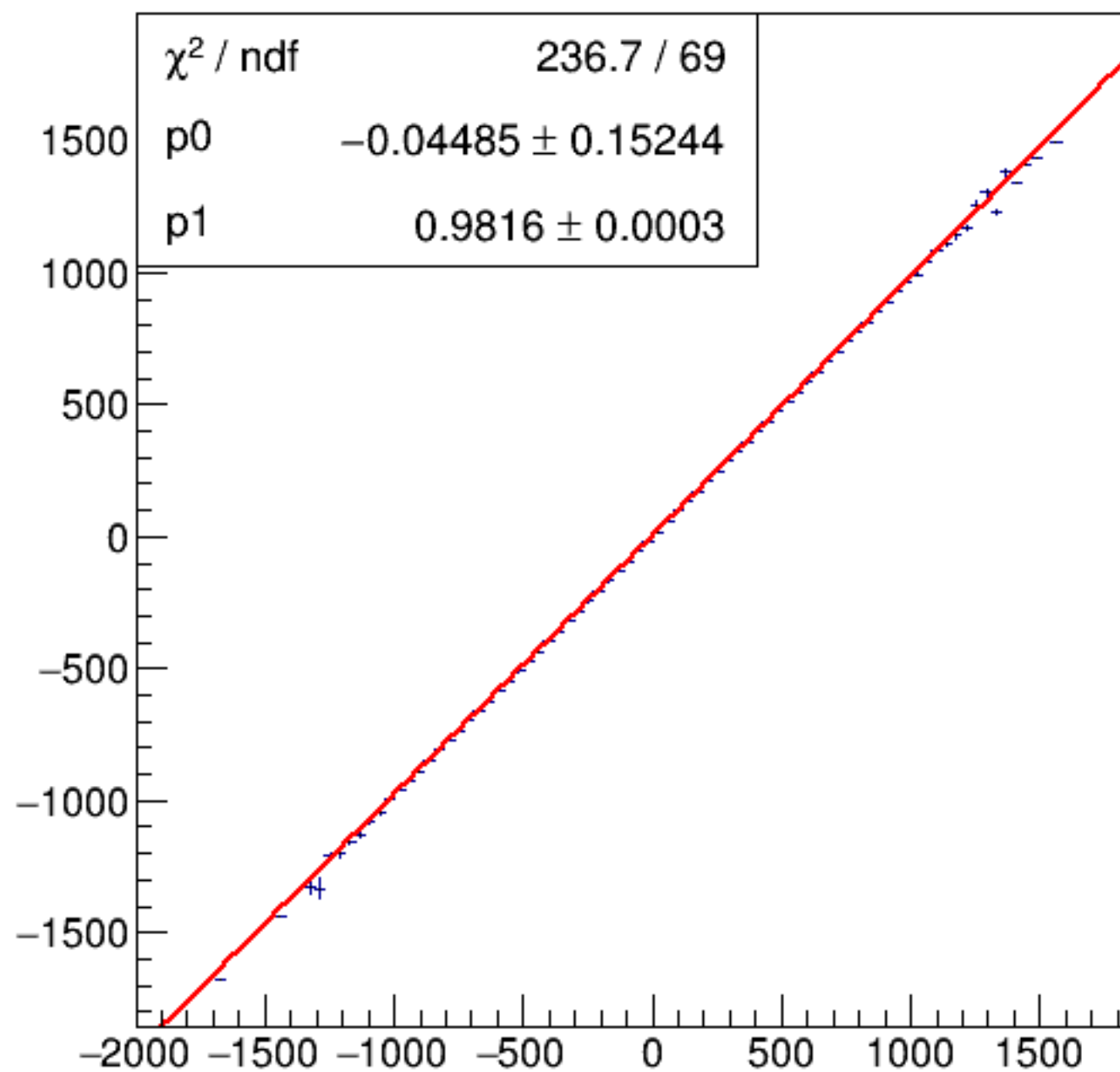
run7849_000_asym_bcm_dg_ds_vs_asym_bcm_an_us_pr.png
