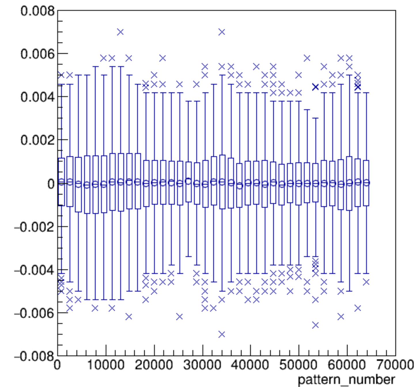
asym_bcm_an_diff*yield_bcm_an_diff:pattern_number {ErrorFlag==0}
