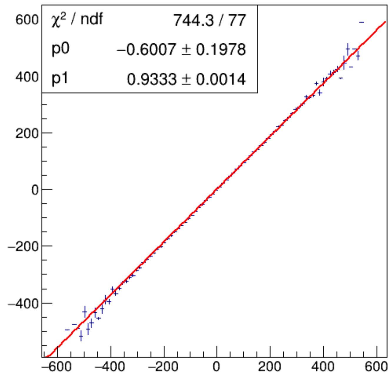
run7849_000_asym_bcm_dg_us_vs_asym_bcm_dg_ds_mul.png
