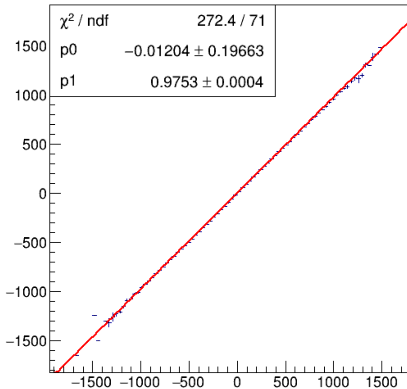
run7849_000_asym_bcm_dg_us_vs_asym_bcm_dg_ds_pr.png
