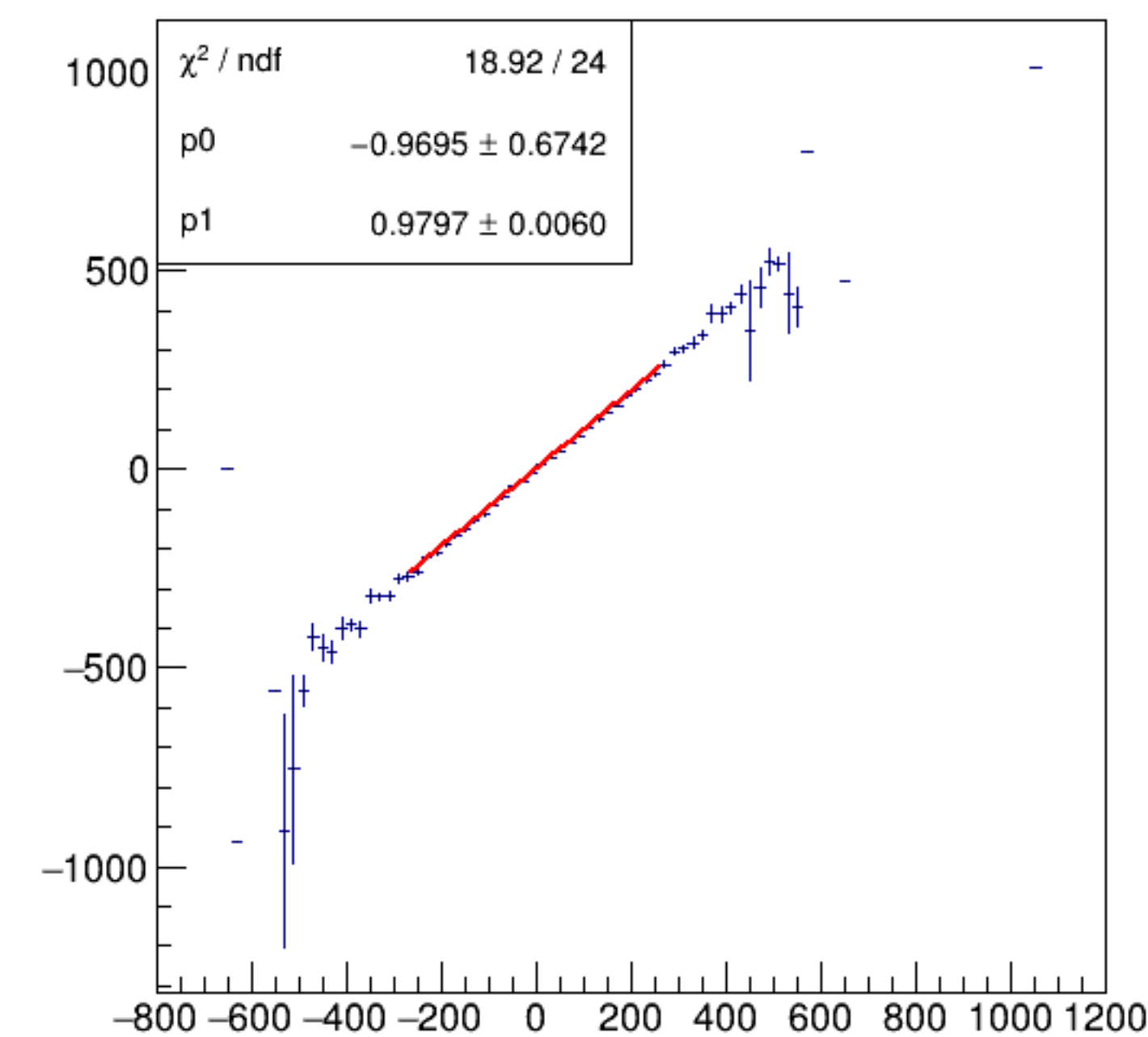
asym_bpm11WS/ppm:Aq/ppm {ErrorFlag==0}
