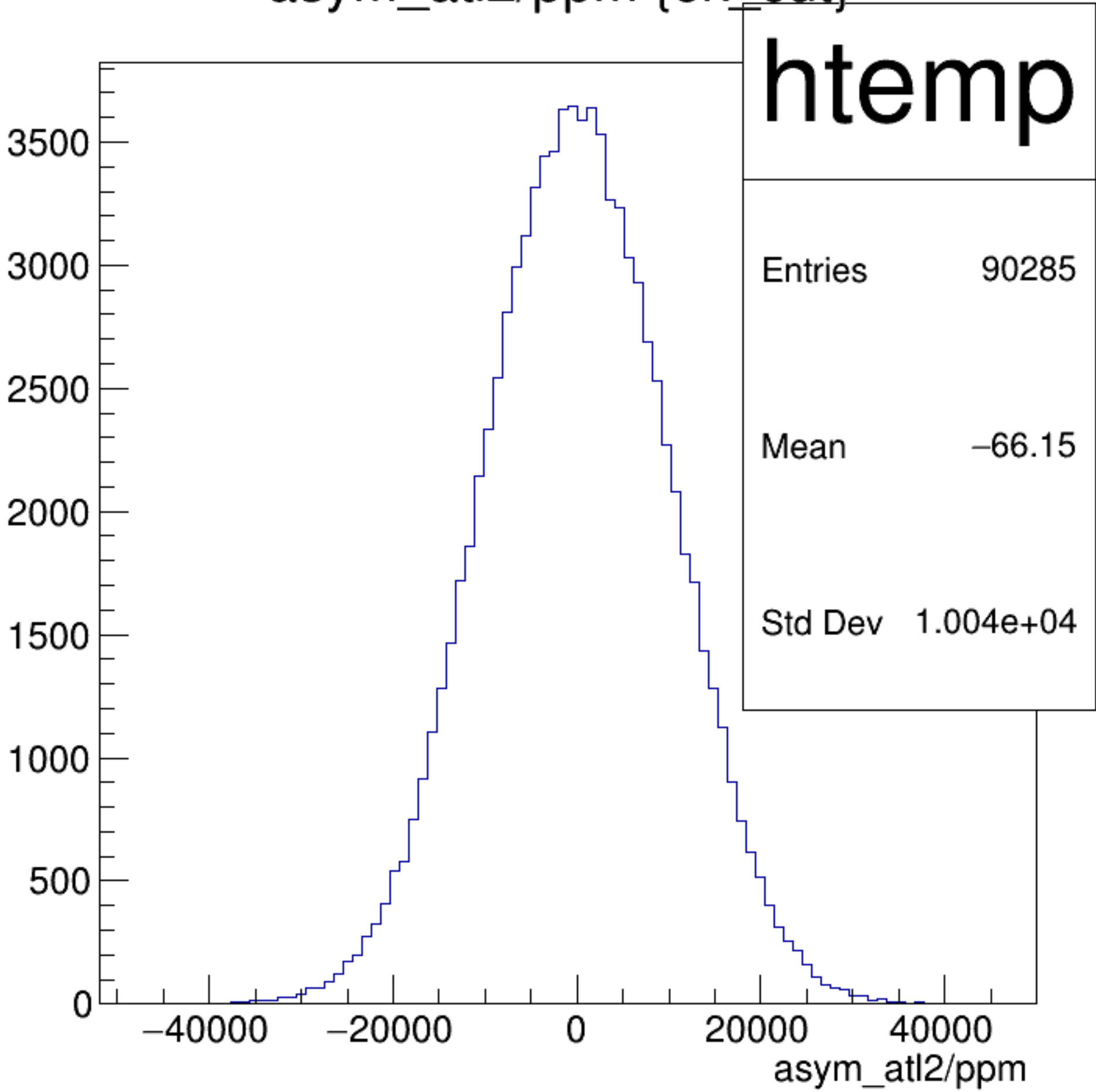
asym_atl2/ppm {ok_cut}
