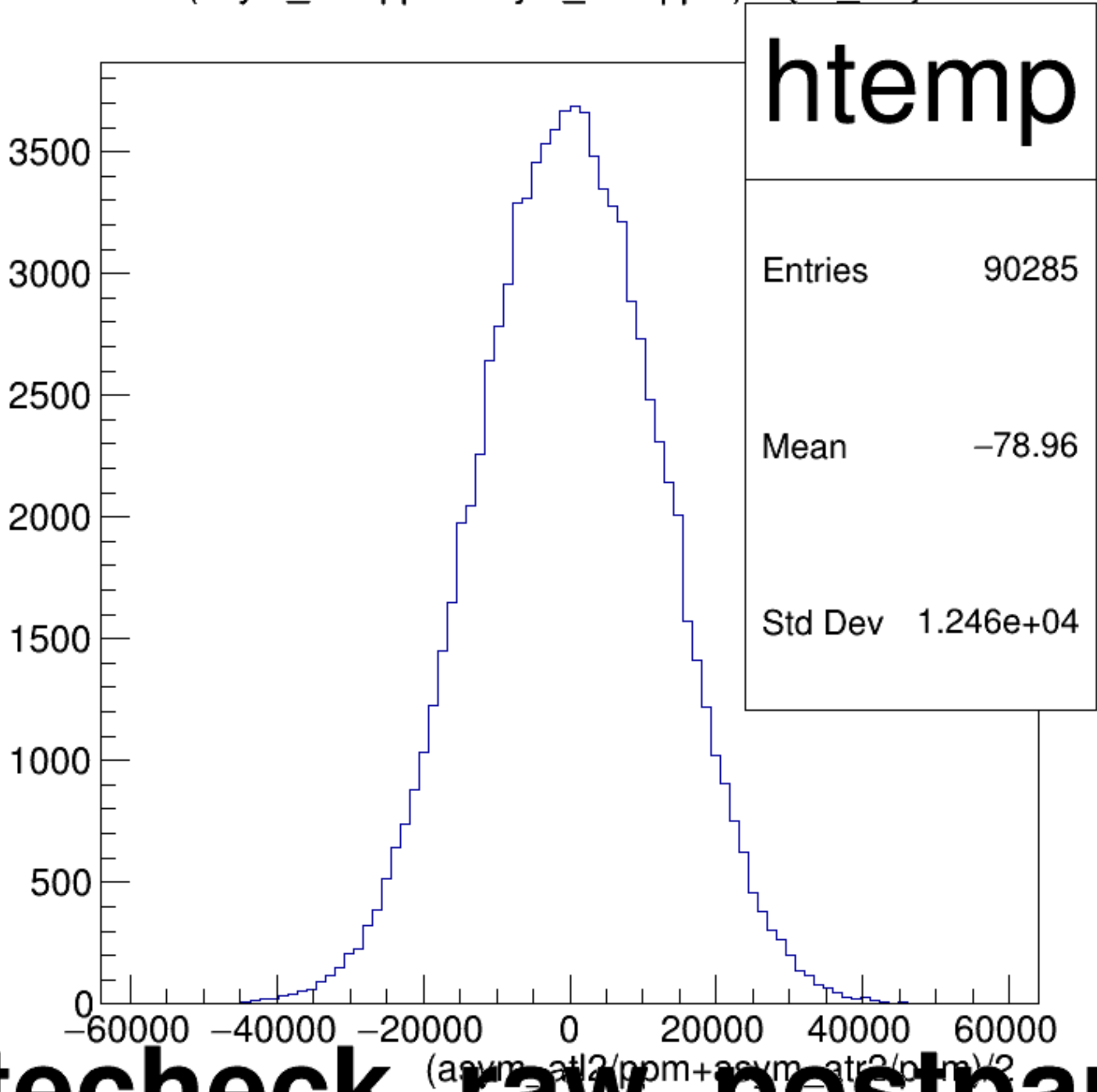
(asym_atl2/ppm+asym_atr2/ppm)/2 {ok_cut}
