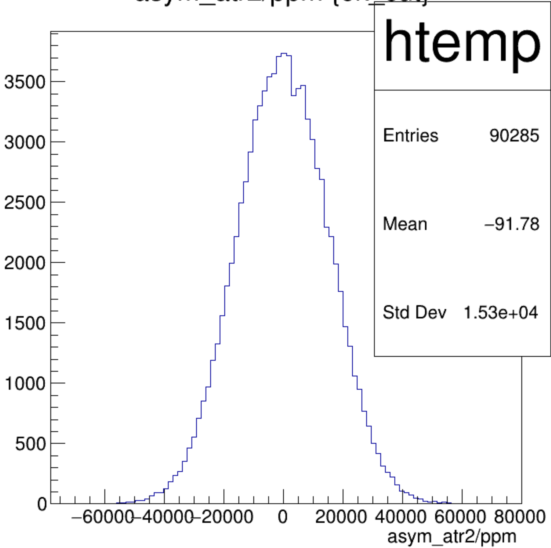
asym_atr2/ppm {ok_cut}
