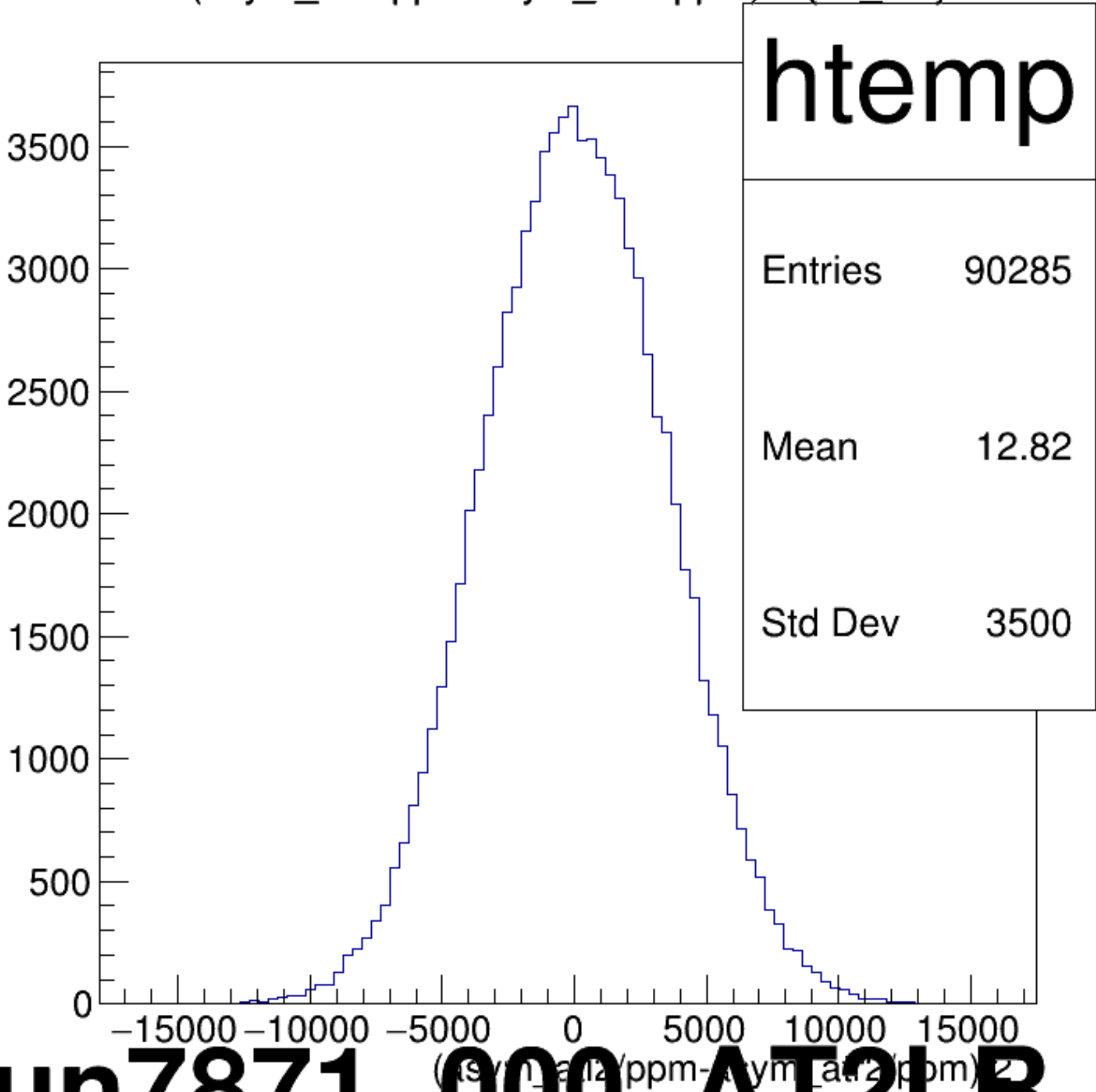
(asym_atl2/ppm-asym_atr2/ppm)/2 {ok_cut}
