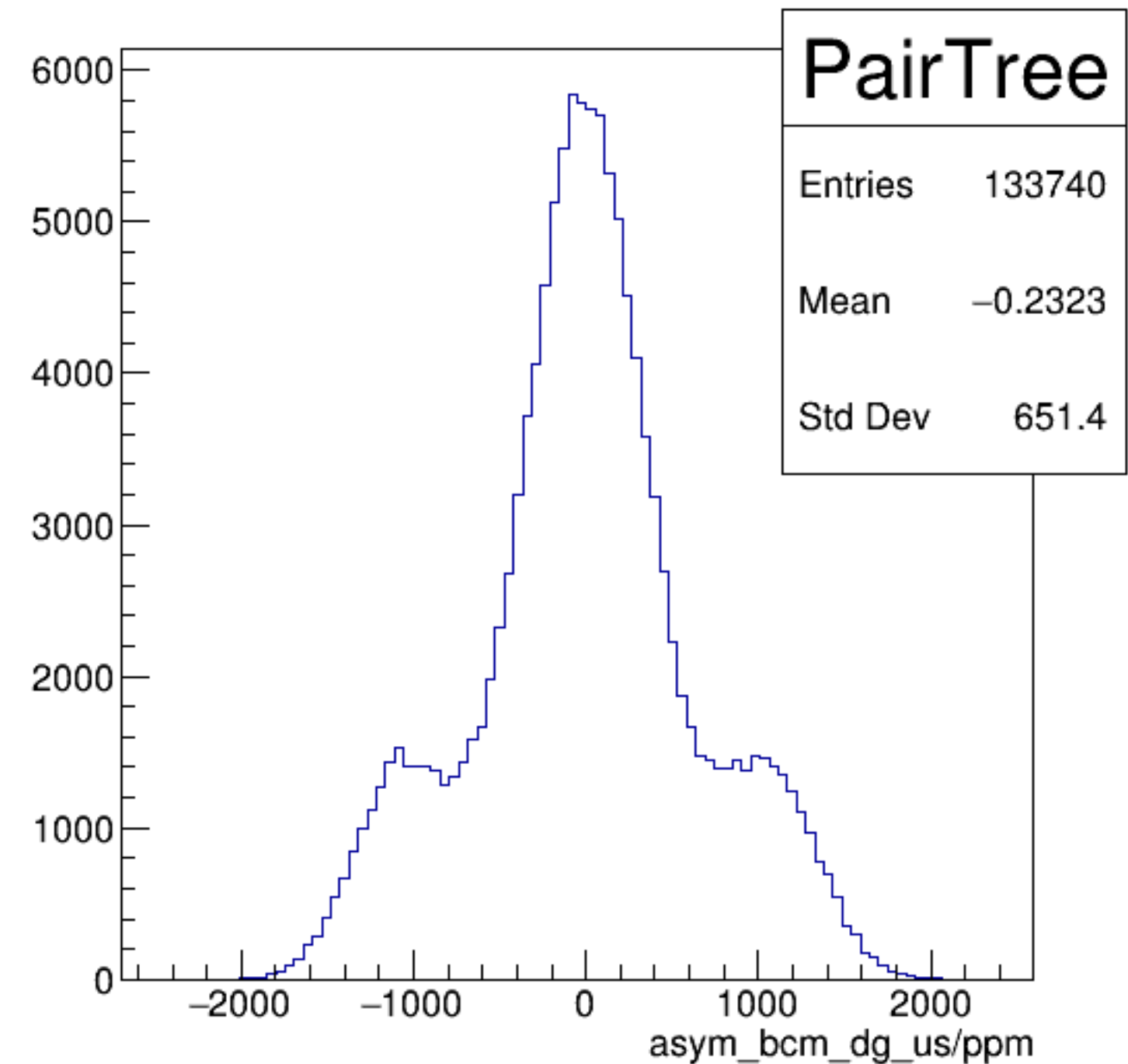
asym_bcm_dg_us/ppm {ErrorFlag==0}
