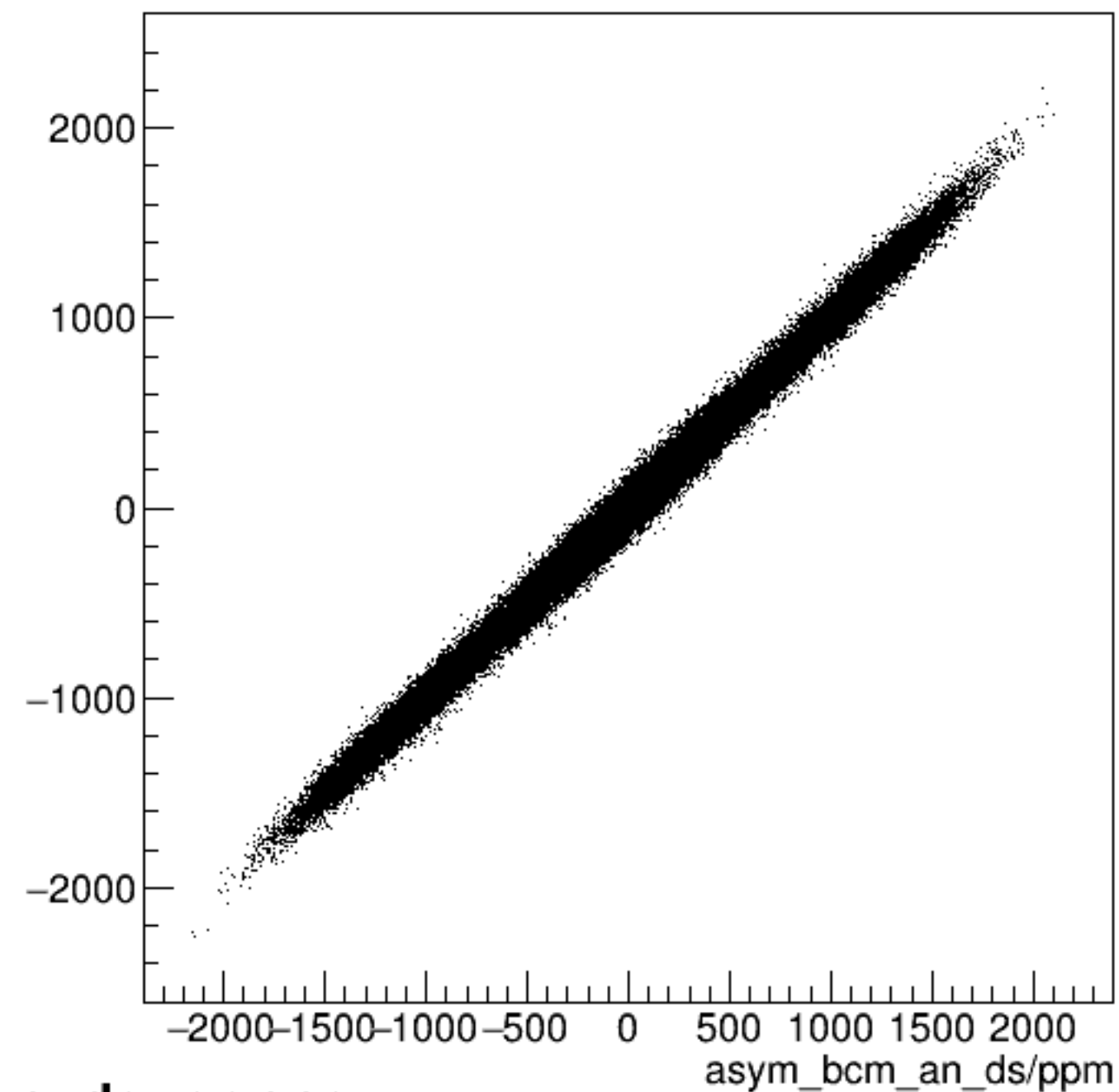
run7896_000_asym_bcm_dg_us_vs_asym_bcm_an_ds_pr.png
