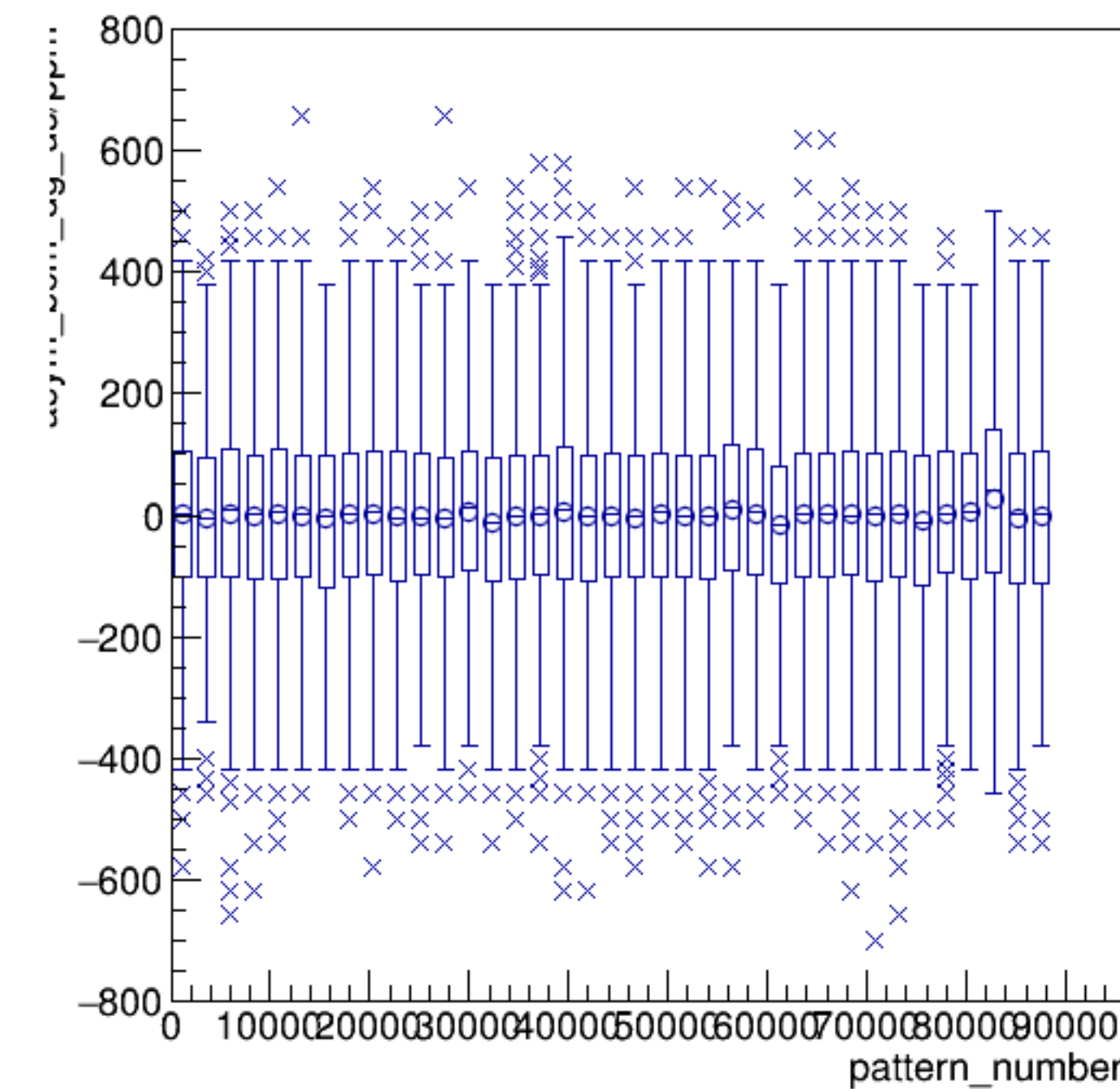
asym_bcm_dg_us/ppm:pattern_number {ErrorFlag==0}
