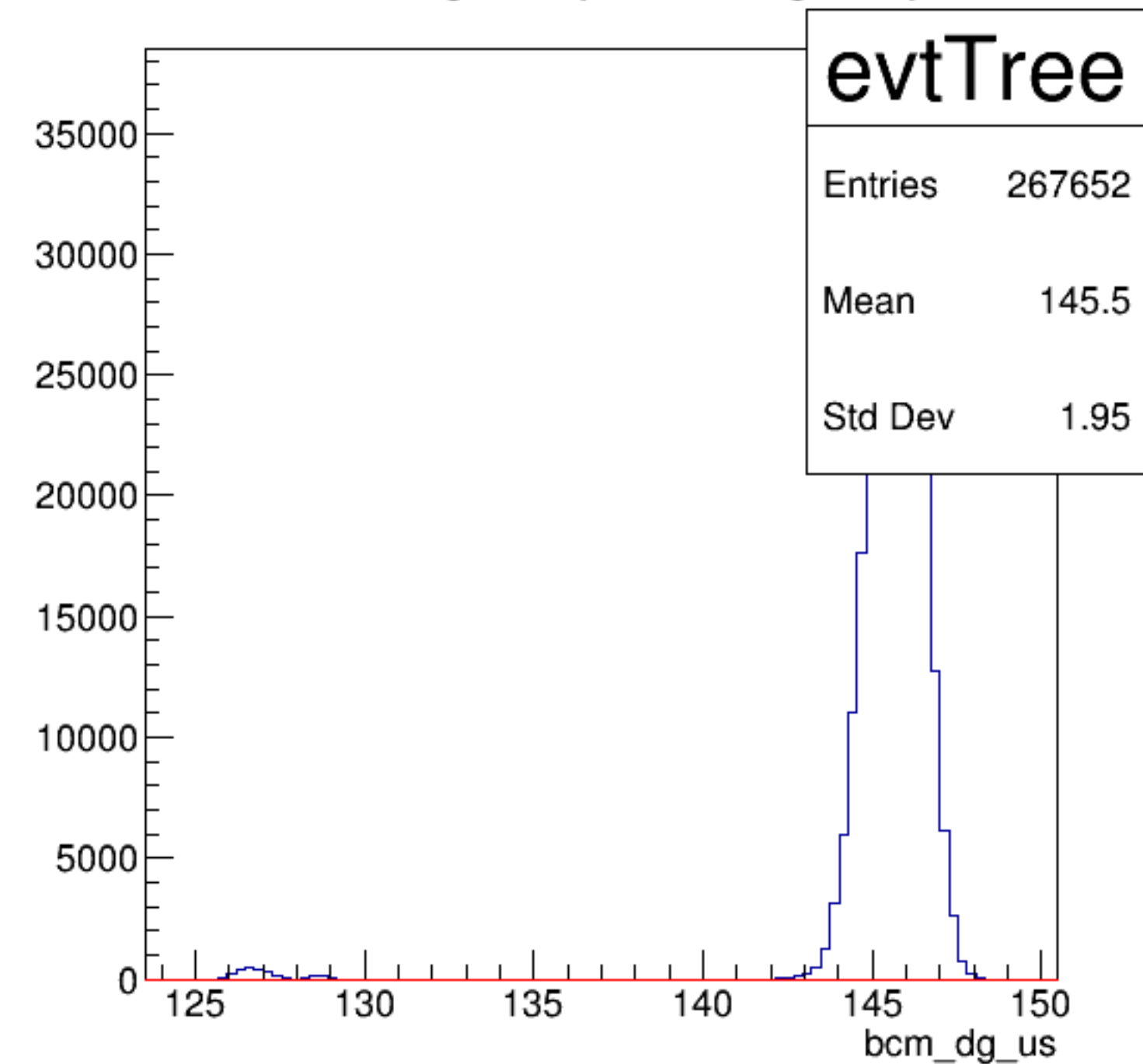
bcm_dg_us {ErrorFlag==0}
