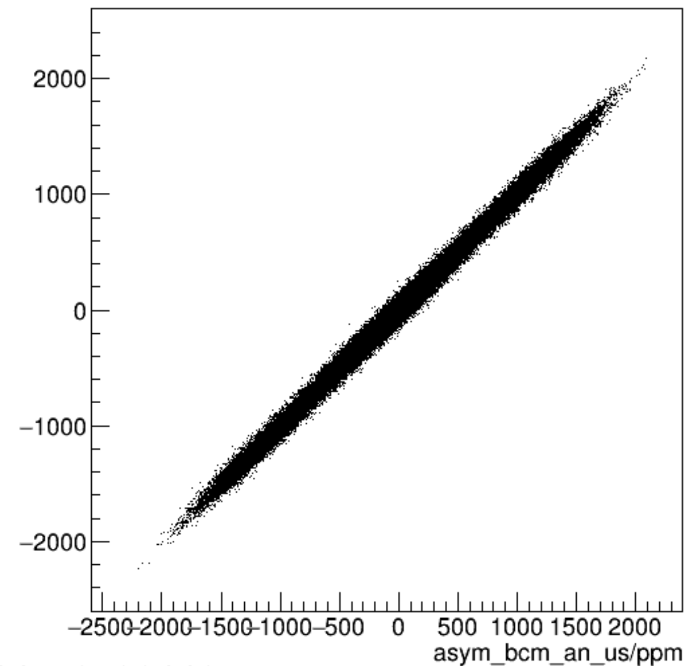
run7896_000_asym_bcm_dg_ds_vs_asym_bcm_an_us_pr.png
