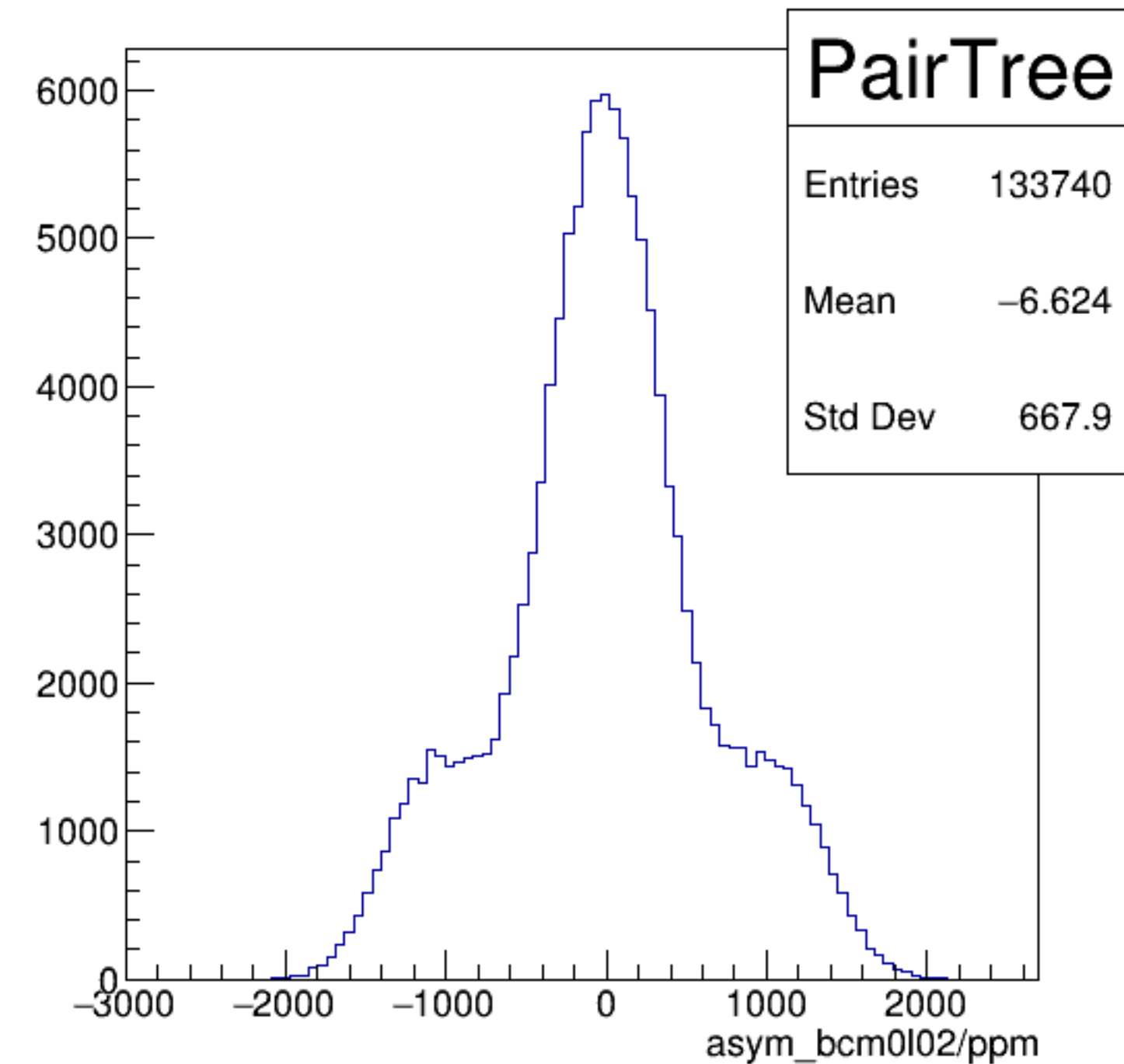
asym_bcm0l02/ppm {ErrorFlag==0}
