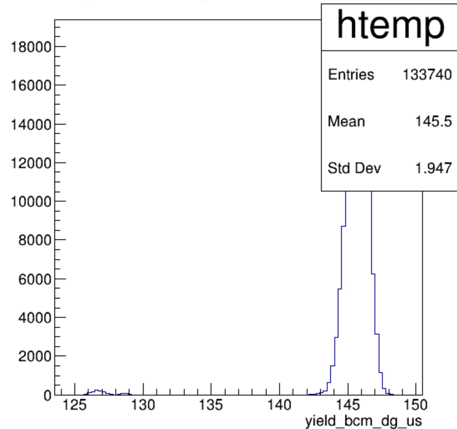
yield_bcm_dg_us {ErrorFlag==0}
