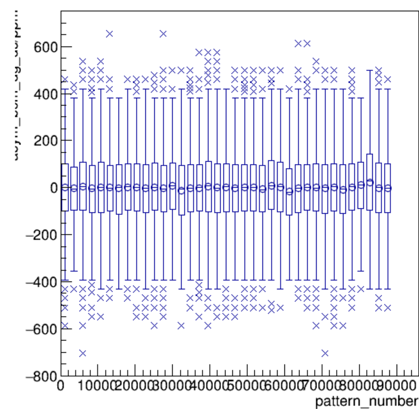
asym_bcm_dg_ds/ppm:pattern_number {ErrorFlag==0}
