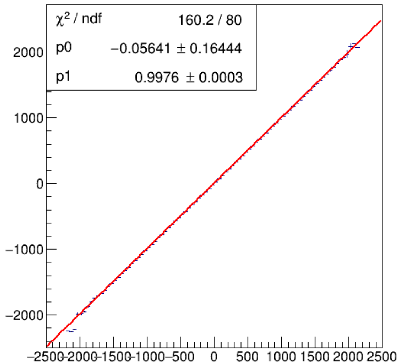
run7896_000_asym_bcm_dg_us_vs_asym_bcm_an_ds_pr.png
