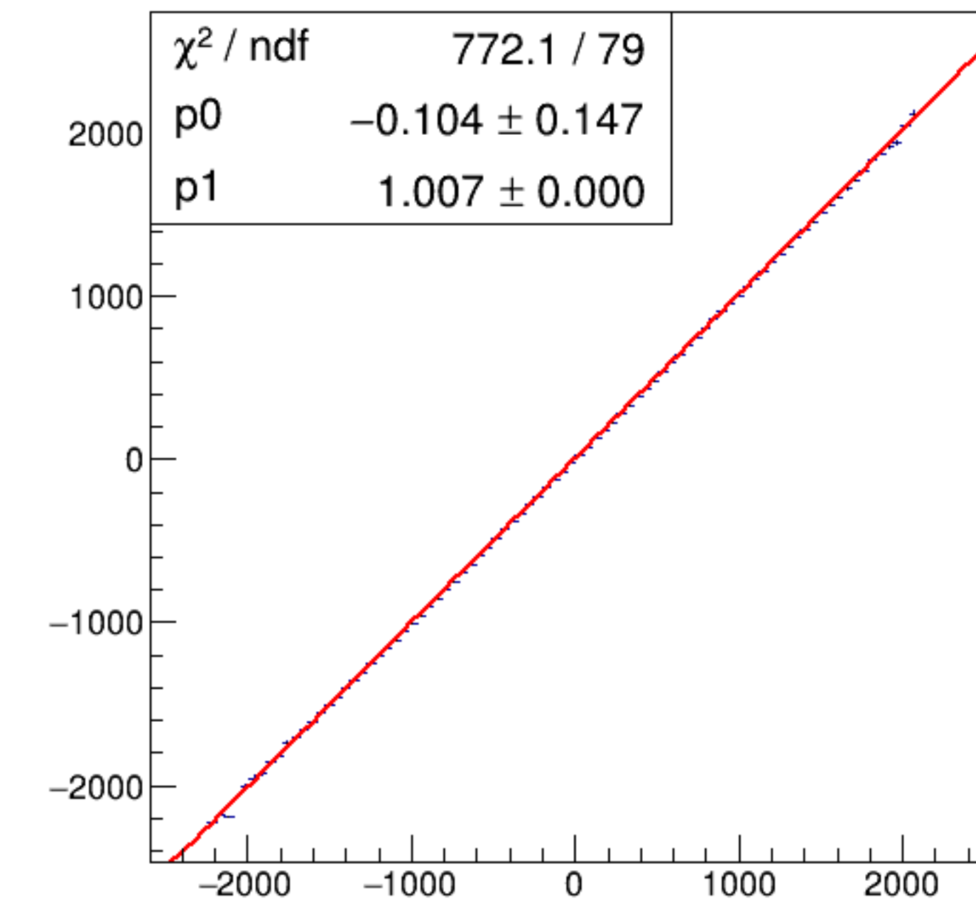
run7896_000_asym_bcm_dg_ds_vs_asym_bcm_an_us_pr.png
