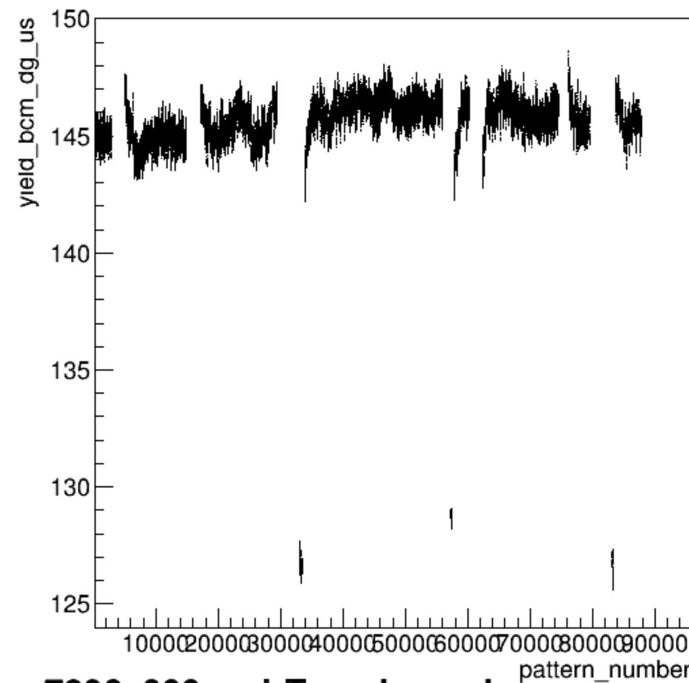
yield_bcm_dg_us:pattern_number {ErrorFlag==0}
