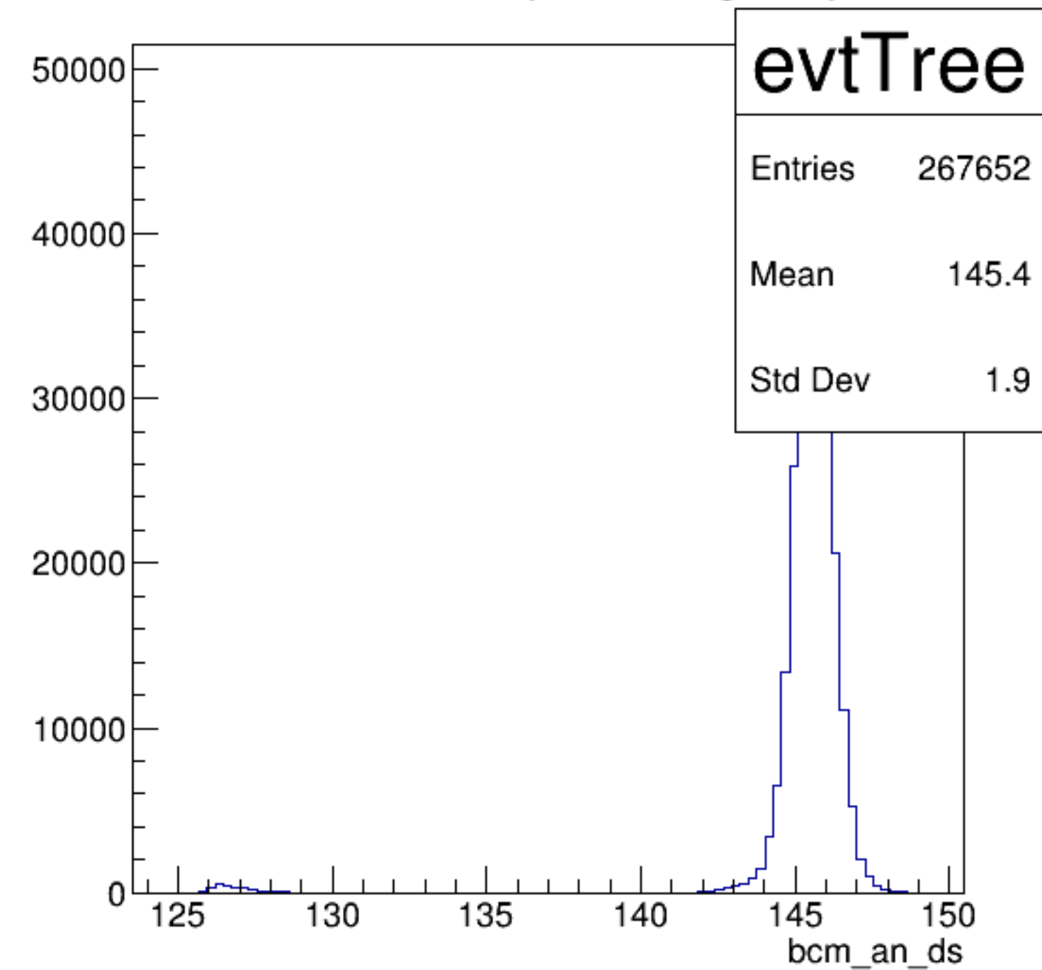
bcm_an_ds {ErrorFlag==0}
