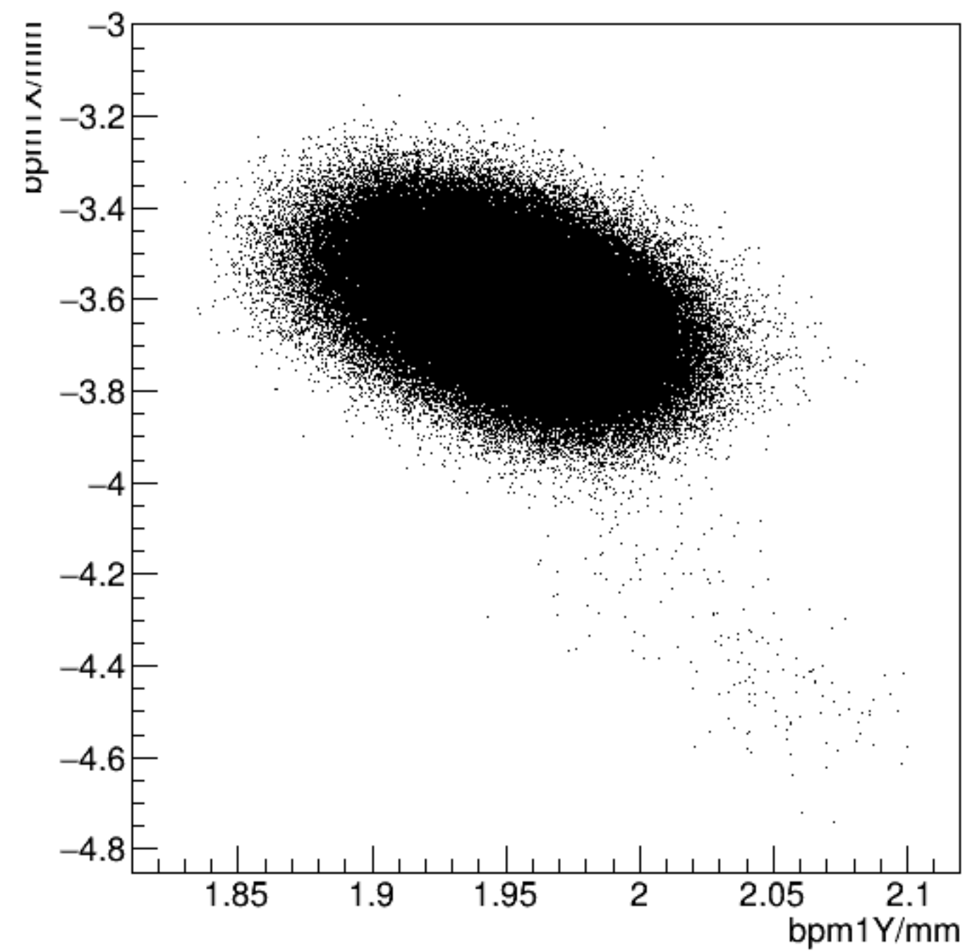
bpm1X/mm:bpm1Y/mm {ErrorFlag==0}
