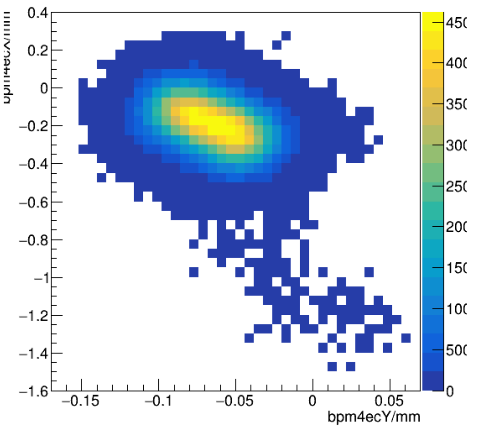
bpm4ecX/mm:bpm4ecY/mm {ErrorFlag==0}
