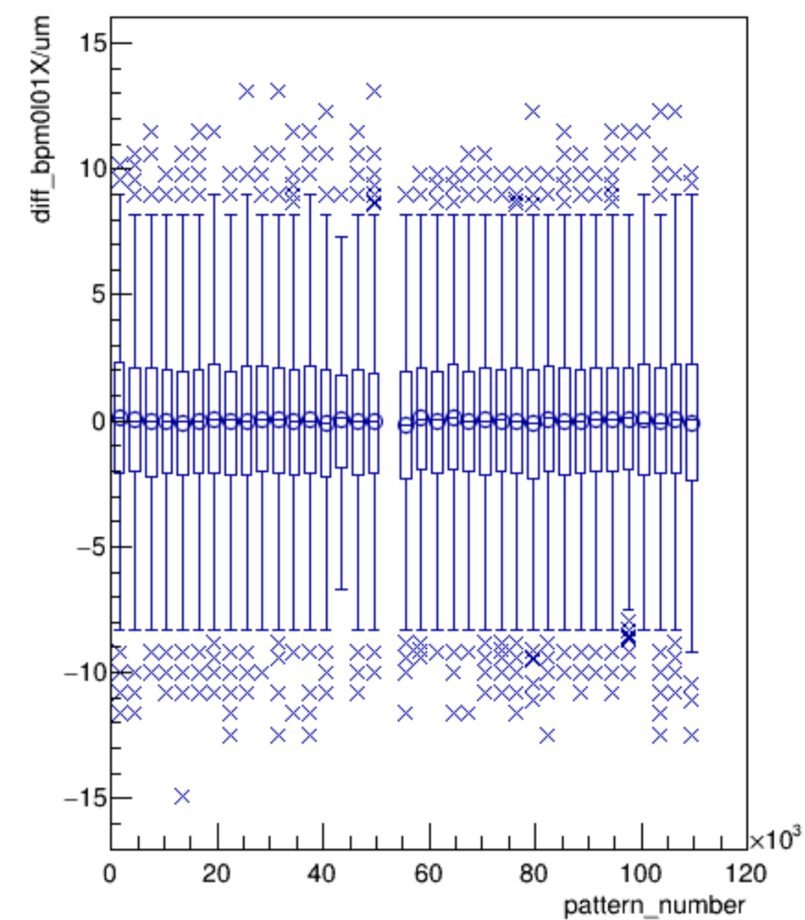
diff_bpm0I01X/um:pattern_number (ErrorFlag==0)
