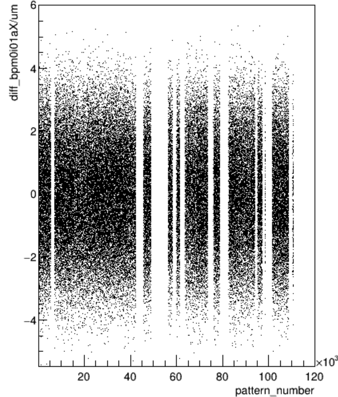
diff_bpm0i01aX/um:pattern_number (ErrorFlag==0)
