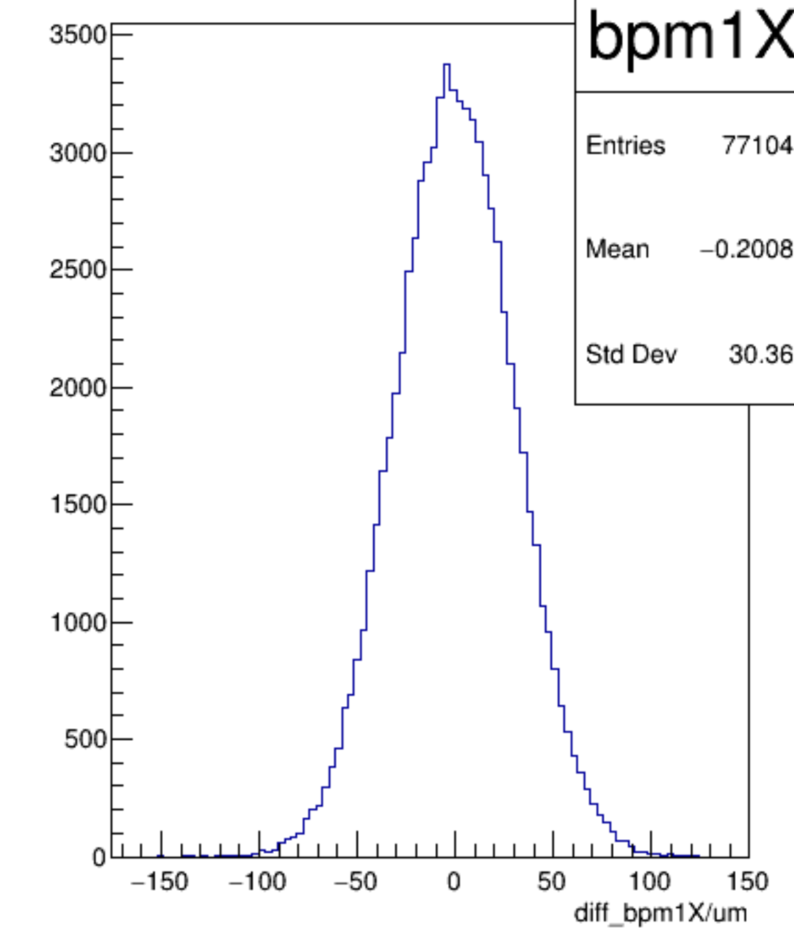
diff_bpm1X/um {ErrorFlag==0}
