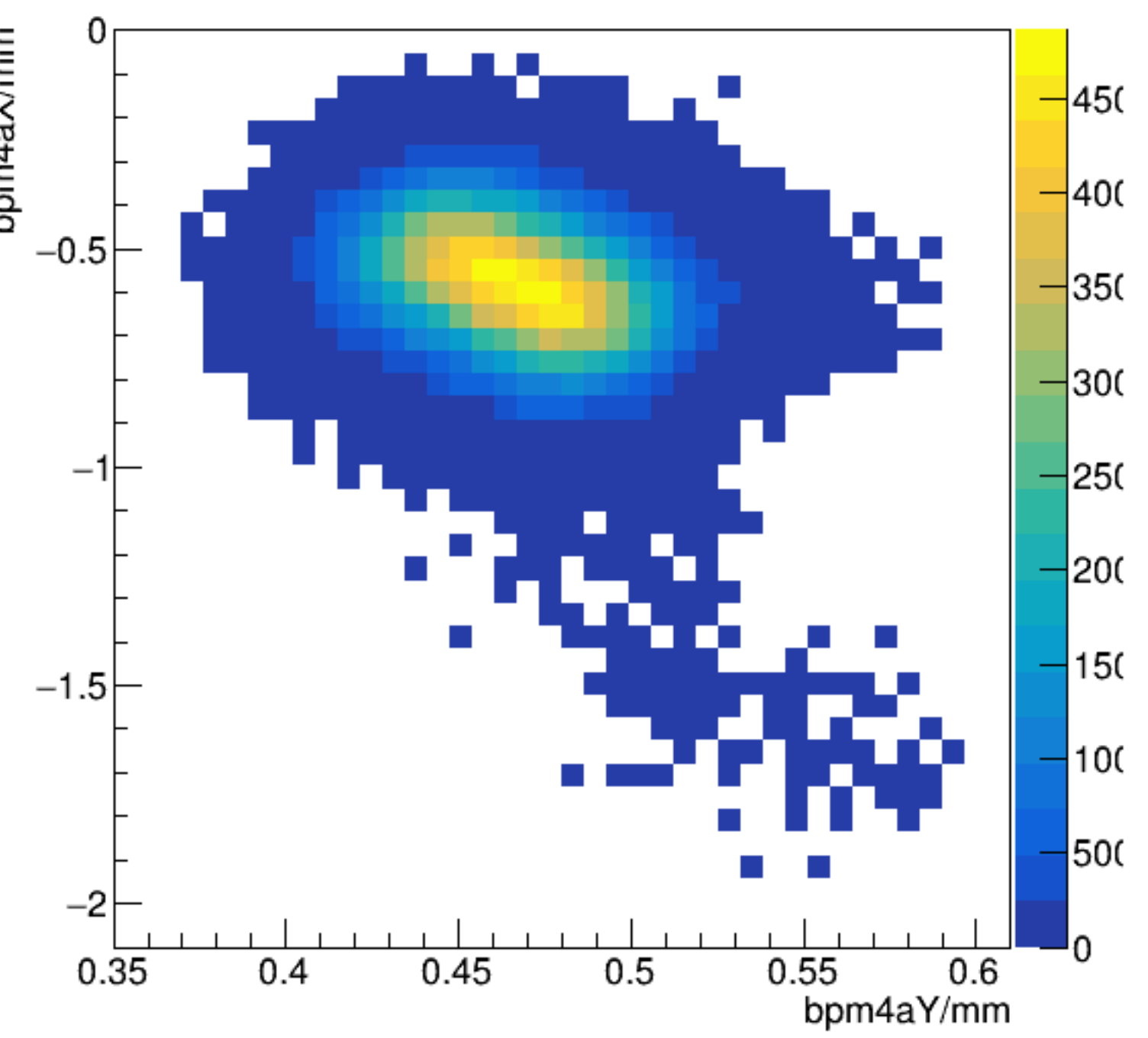
bpm4aX/mm:bpm4aY/mm {ErrorFlag==0}
