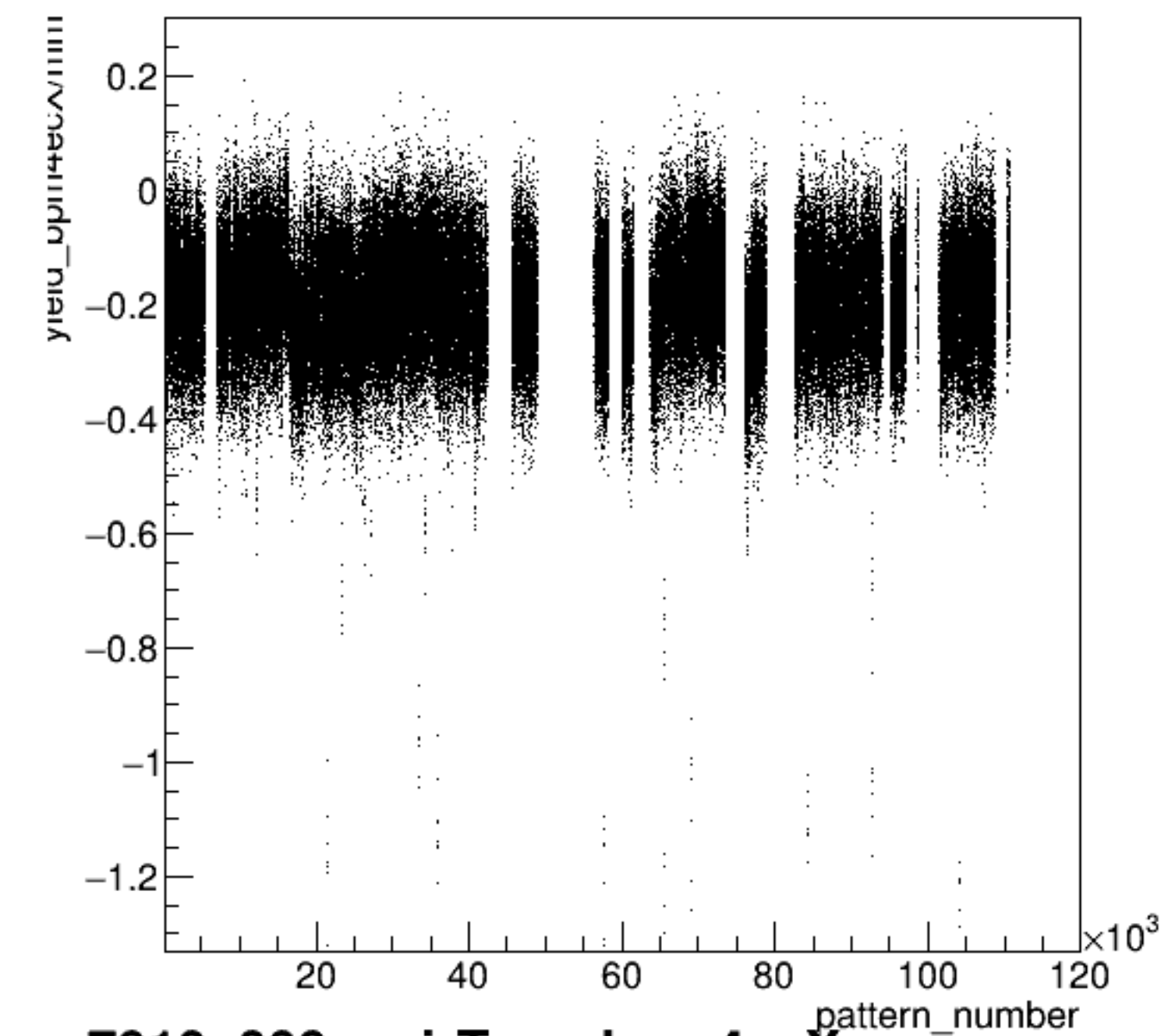
yield_bpm4ecX/mm:pattern_number {ErrorFlag==0}
