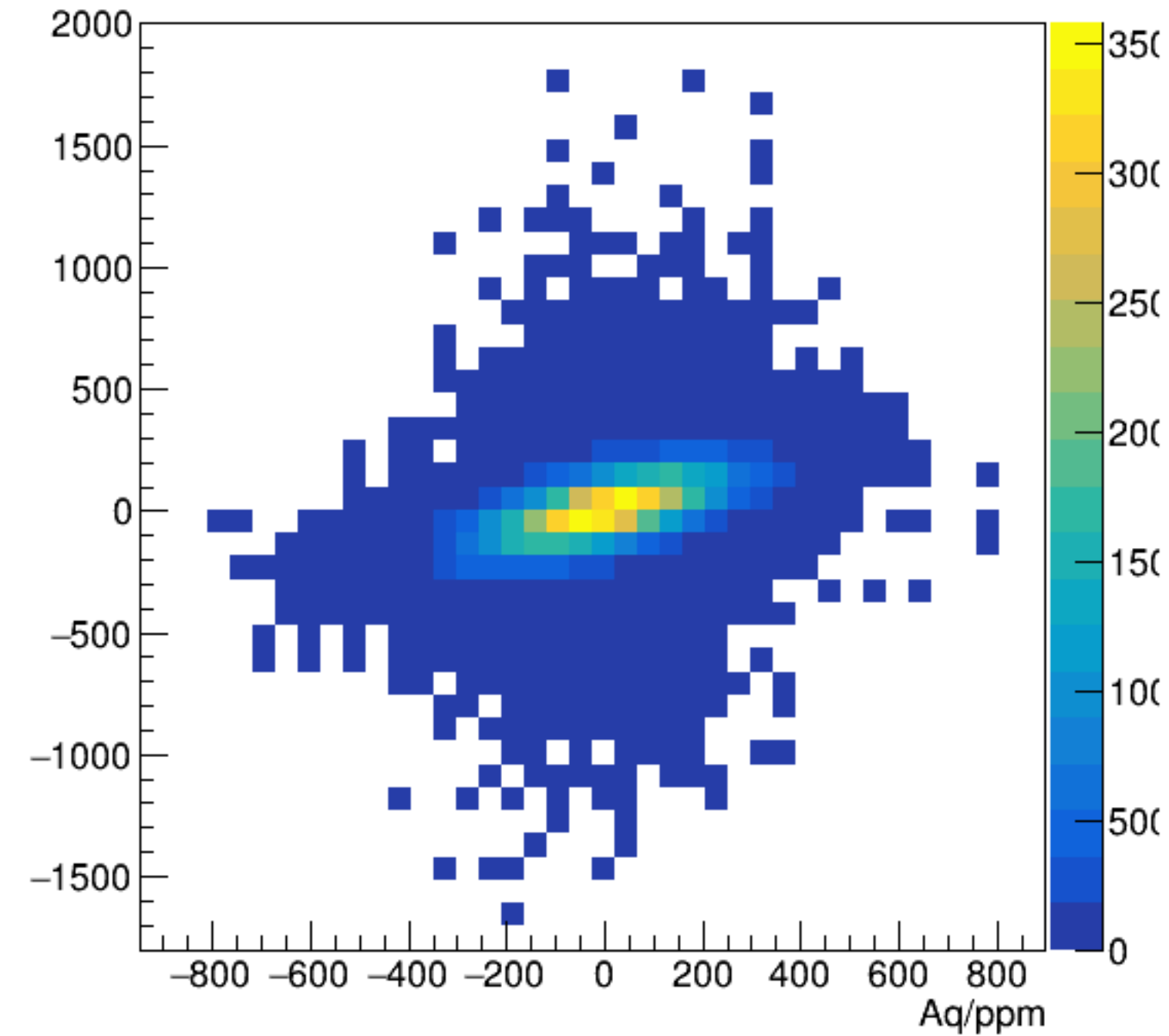
asym_bpm2i02WS/ppm:Aq/ppm {ErrorFlag==0}
