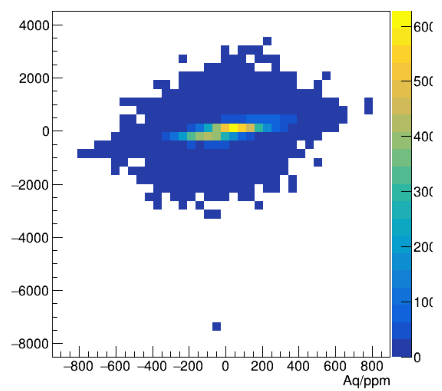
asym_bpm4aWS/ppm:Aq/ppm {ErrorFlag==0}
