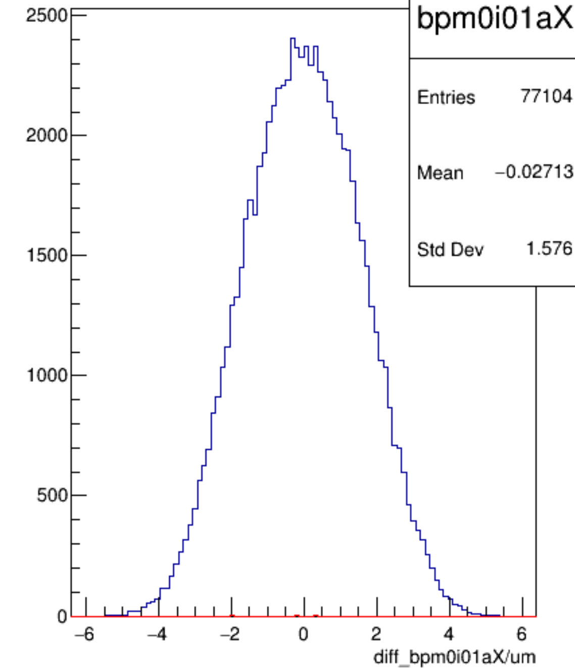
diff_bpm0i01aX/um {ErrorFlag==0}
