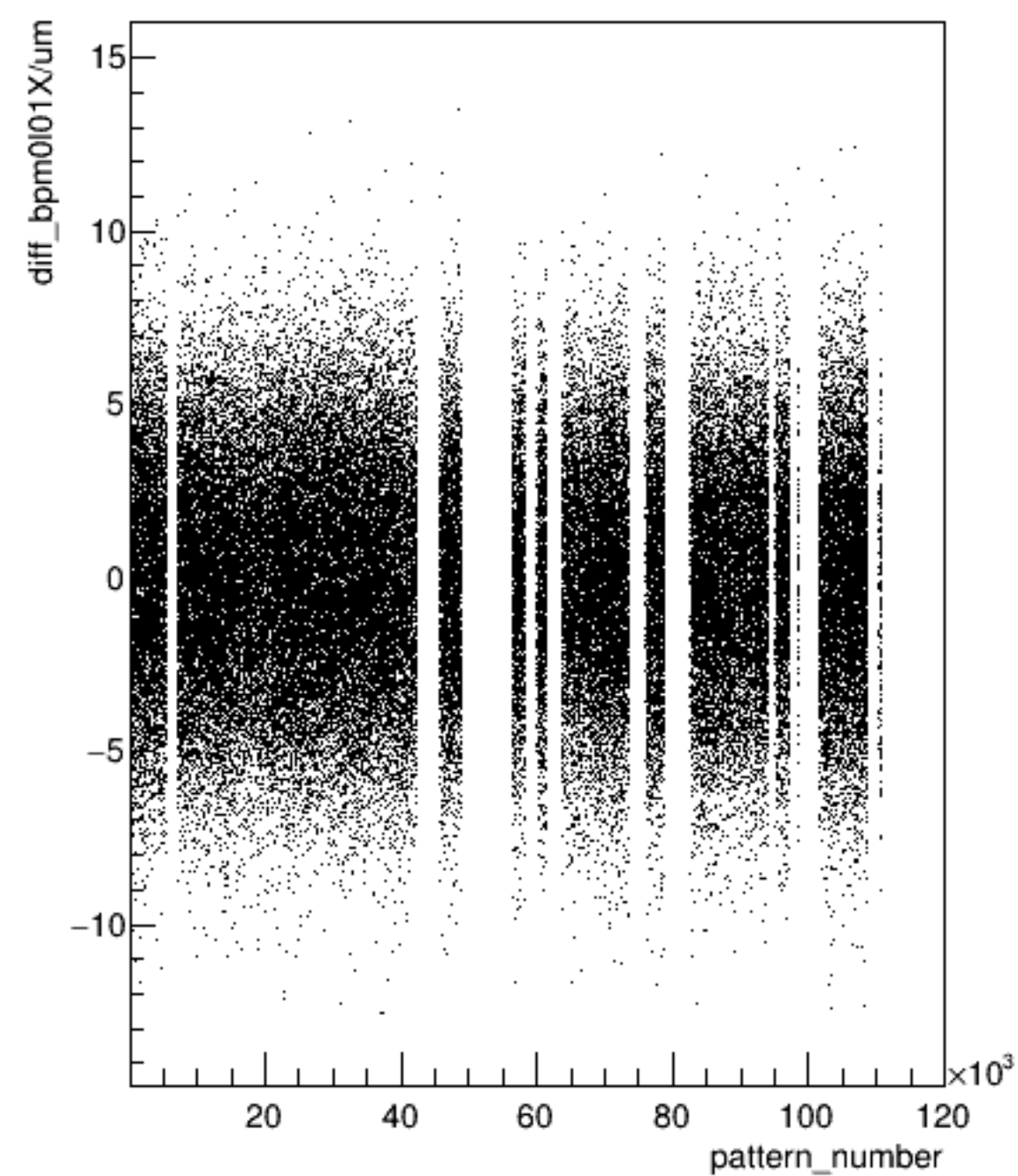
diff_bpm0I01X/um:pattern_number (ErrorFlag==0)
