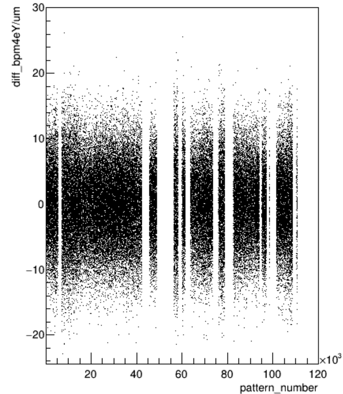
diff_bpm4eY/um:pattern_number {ErrorFlag==0}
