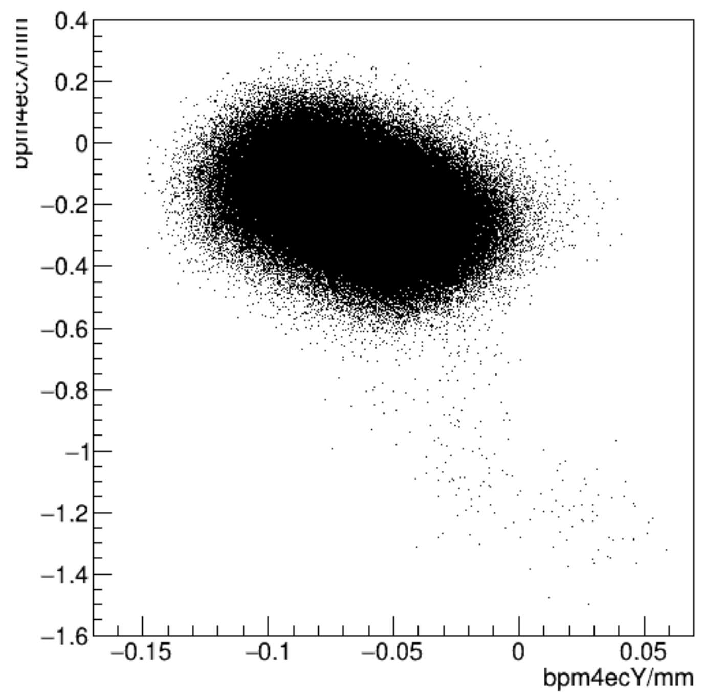
bpm4ecX/mm:bpm4ecY/mm {ErrorFlag==0}
