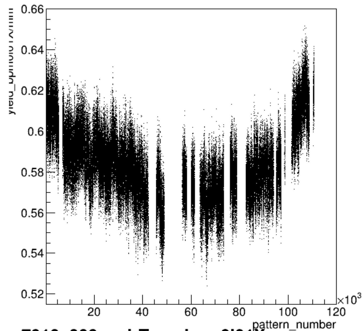
yield_bpm0l01X/mm:pattern_number {ErrorFlag==0}
