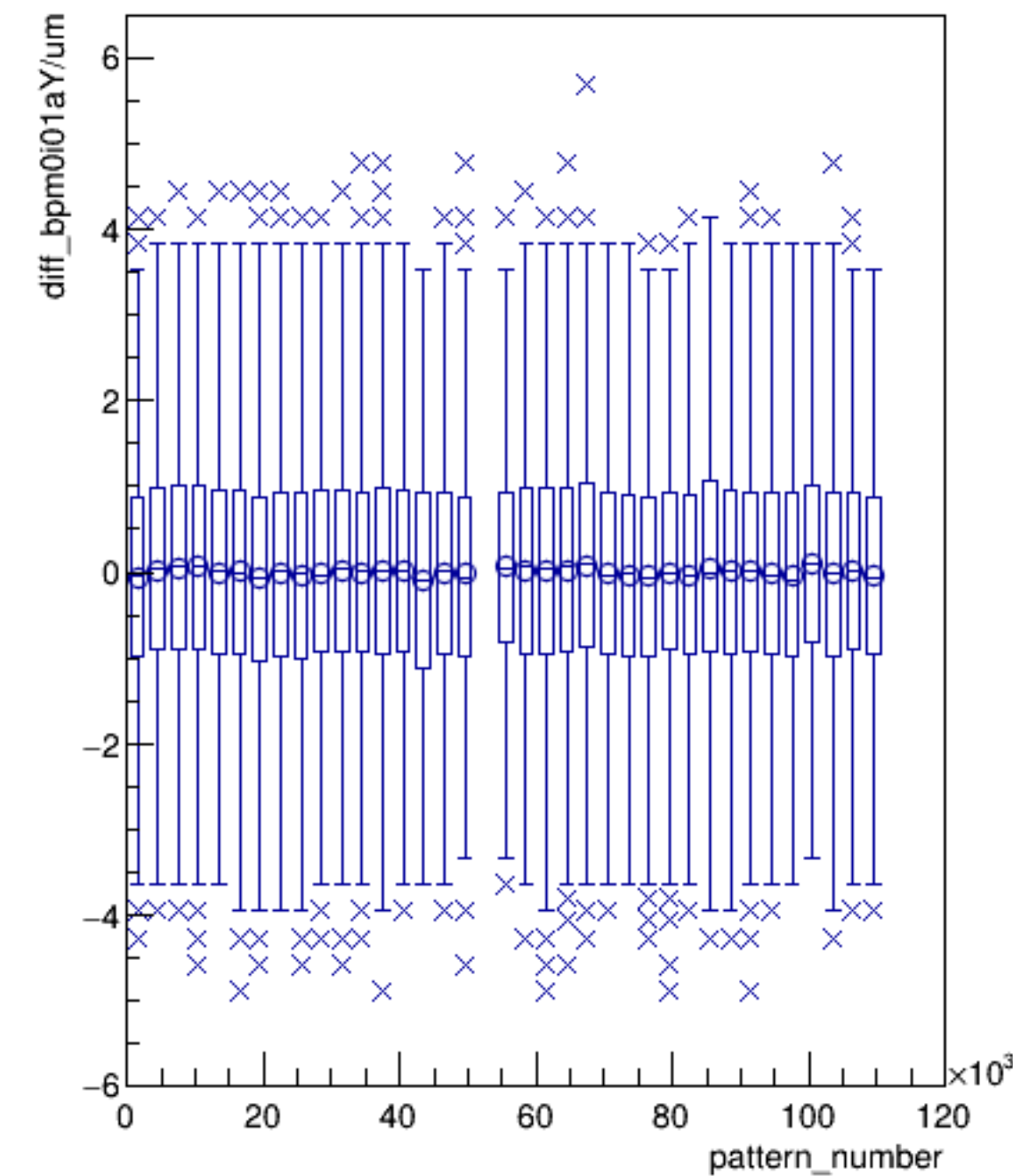
diff_bpm0i01aY/um:pattern_number (ErrorFlag==0)
