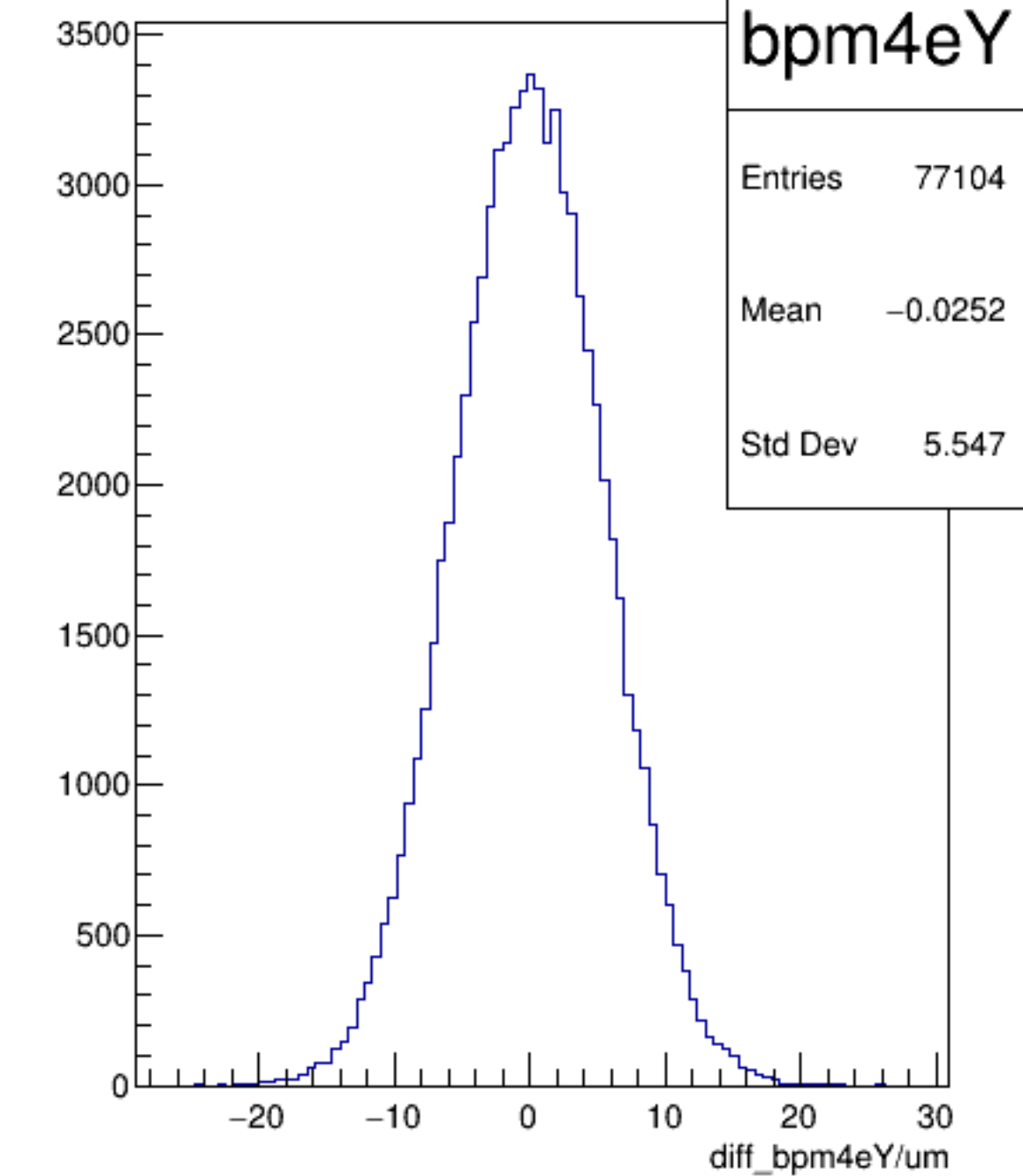
diff_bpm4eY/um {ErrorFlag==0}
