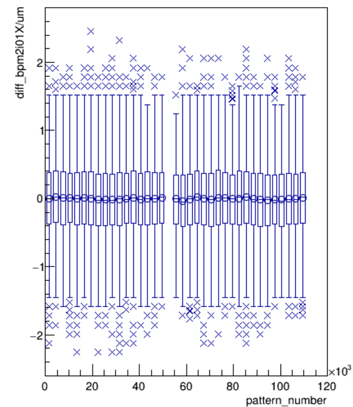
diff_bpm2i01X/um:pattern_number (ErrorFlag==0)
