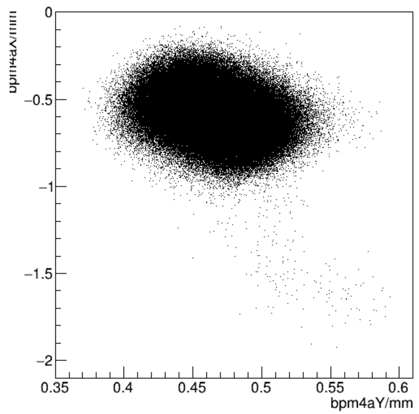
bpm4aX/mm:bpm4aY/mm {ErrorFlag==0}
