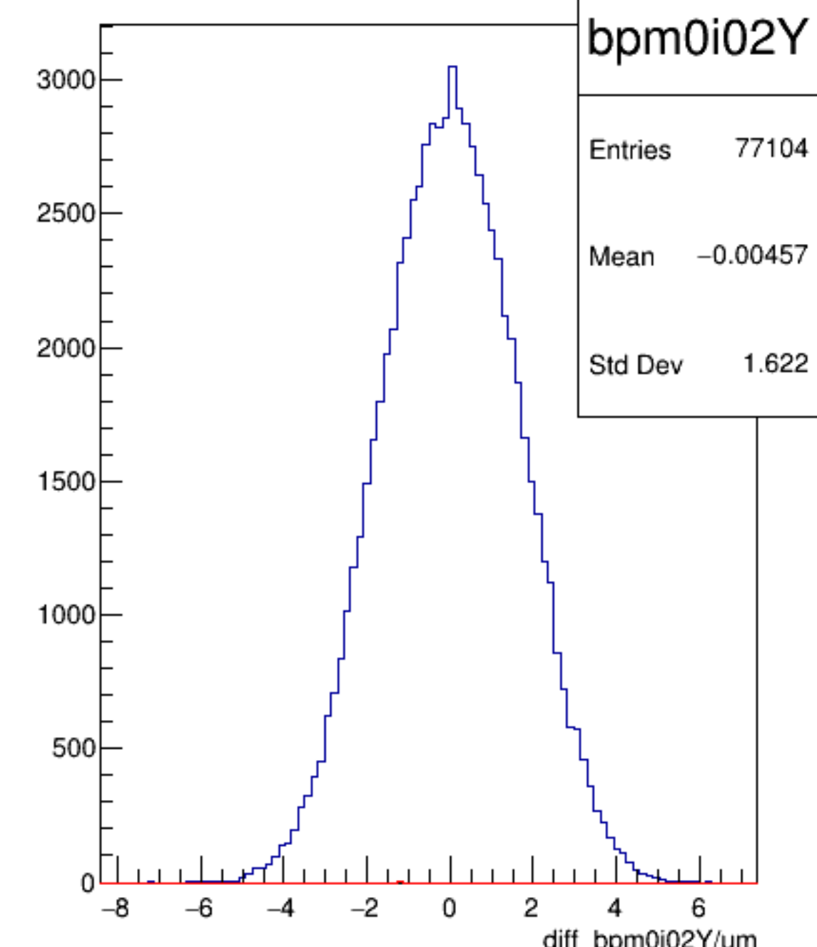
diff_bpm0i02Y/um {ErrorFlag==0}
