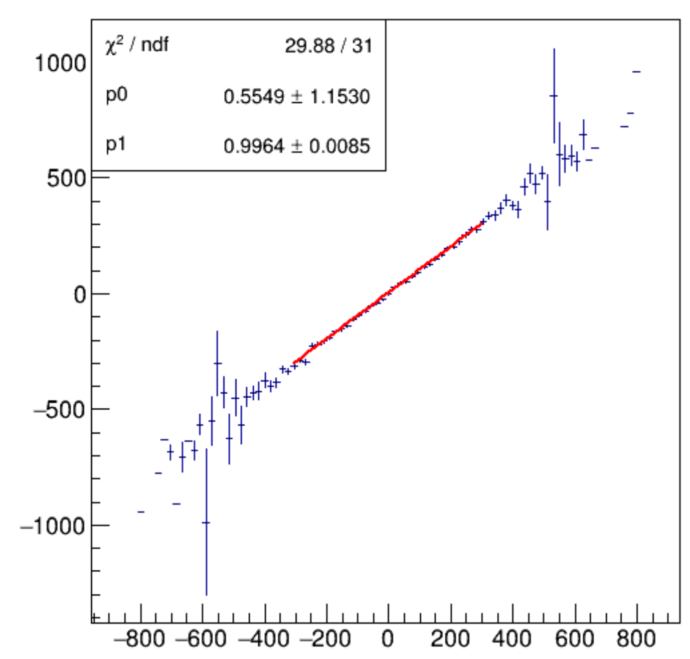
asym_bpm4ecWS/ppm:Aq/ppm {ErrorFlag==0}
