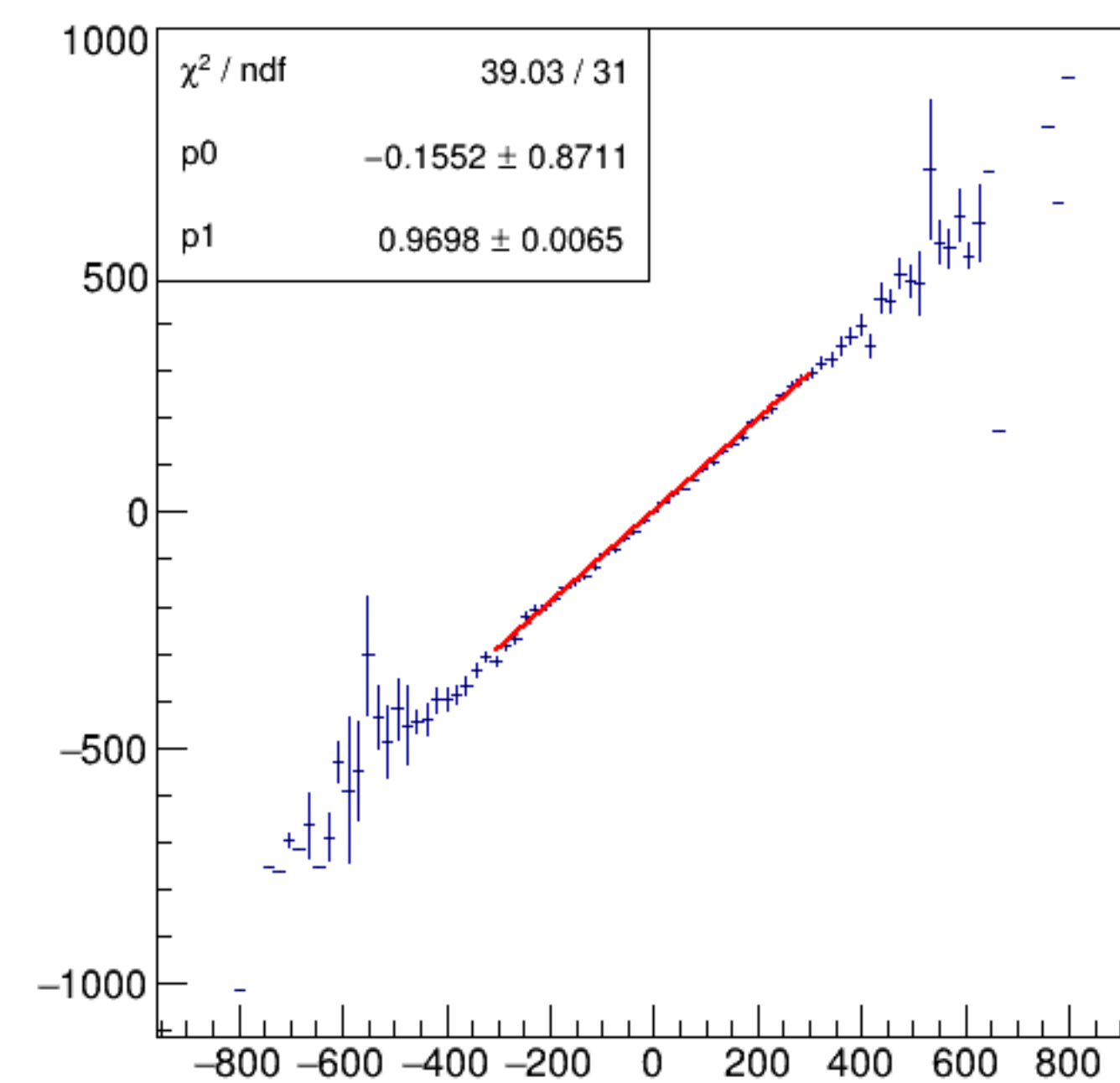
asym_bpm1WS/ppm:Aq/ppm {ErrorFlag==0}
