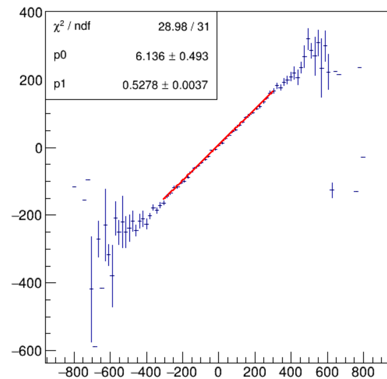
asym_bpm0i01aWS/ppm:Aq/ppm {ErrorFlag==0}
