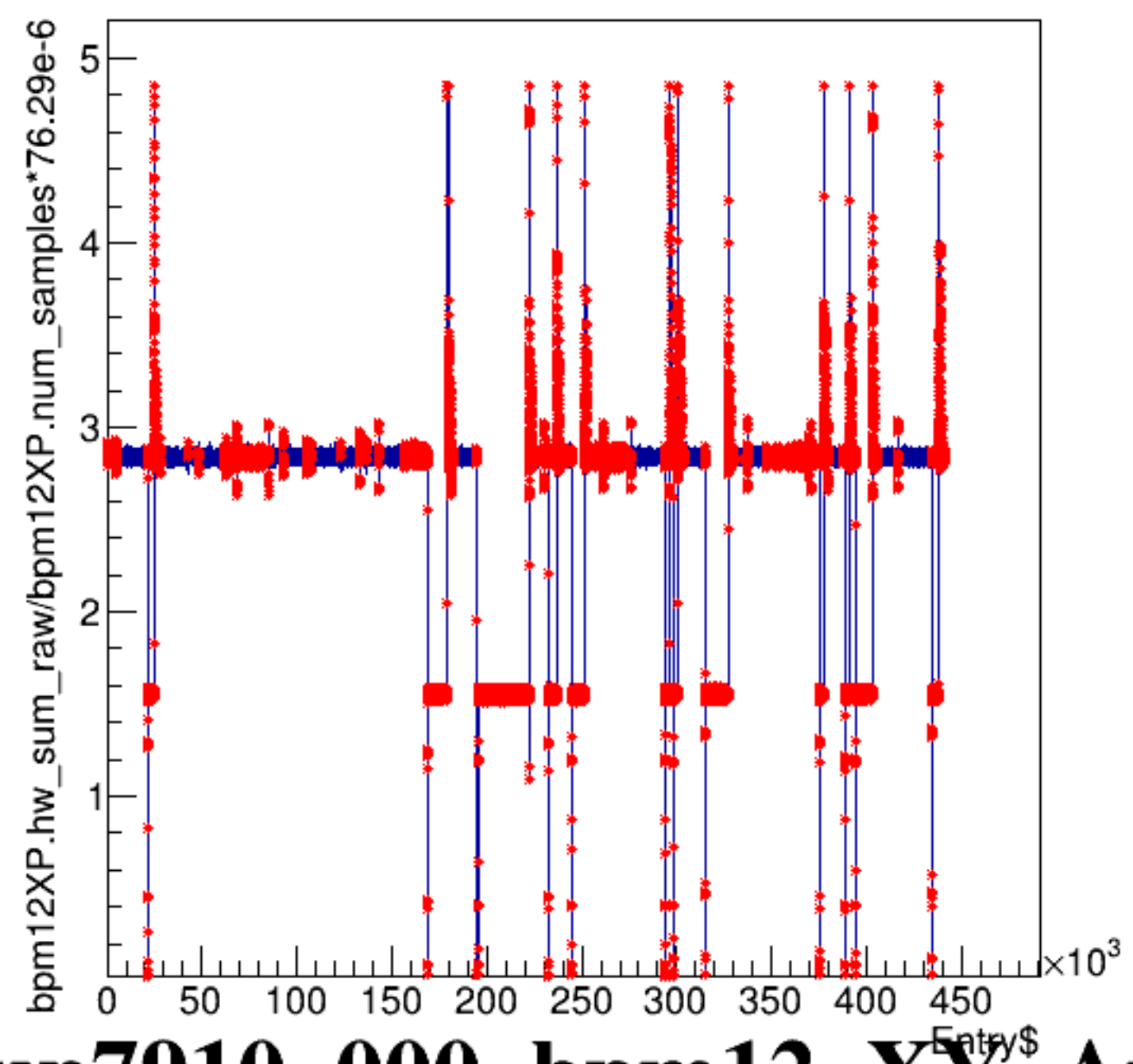
bpm12XP.hw_sum_raw/bpm12XP.num_samples*76.29e-6:Entry$
