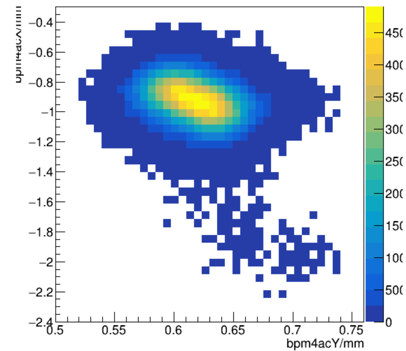
bpm4acX/mm:bpm4acY/mm {ErrorFlag==0}
