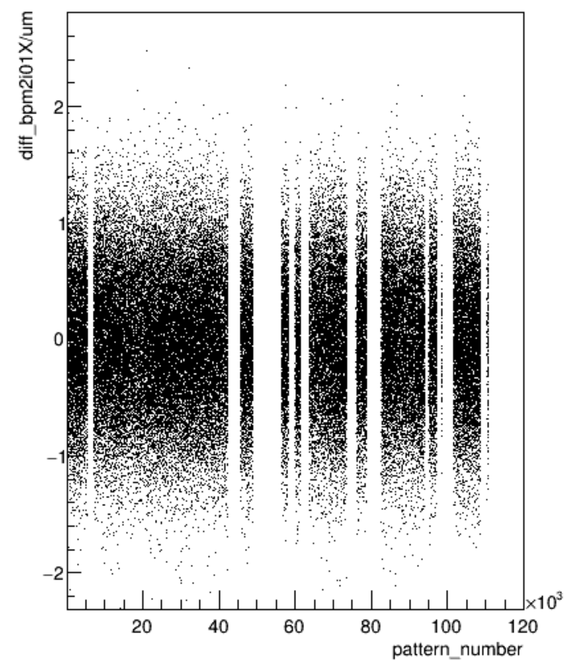
diff_bpm2i01X/um:pattern_number (ErrorFlag==0)
