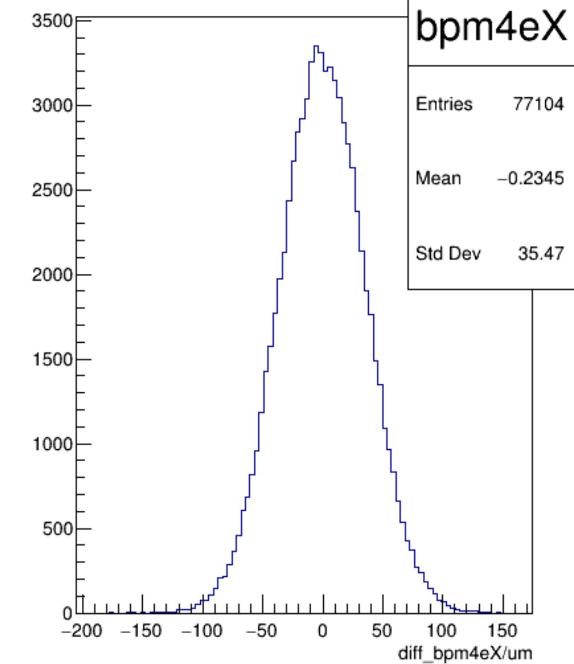
diff_bpm4eX/um {ErrorFlag==0}
