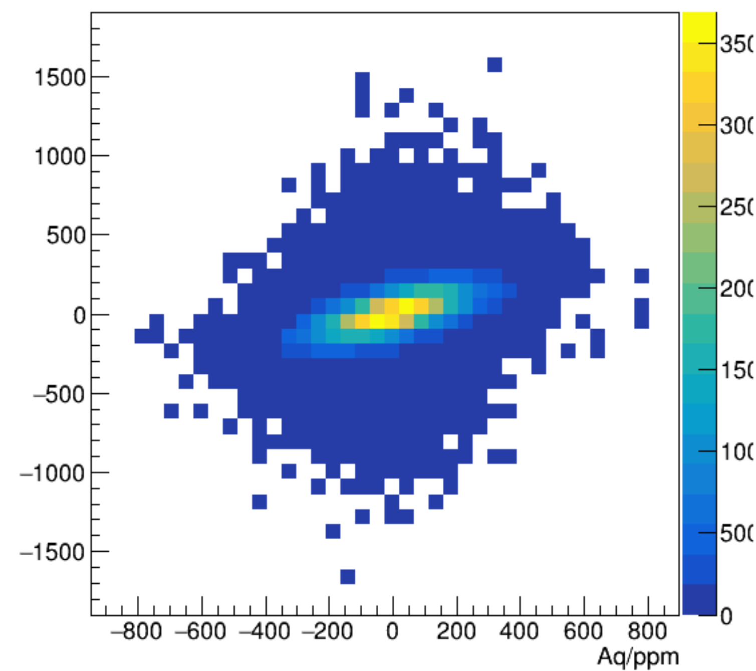
asym_bpm2i01WS/ppm:Aq/ppm {ErrorFlag==0}
