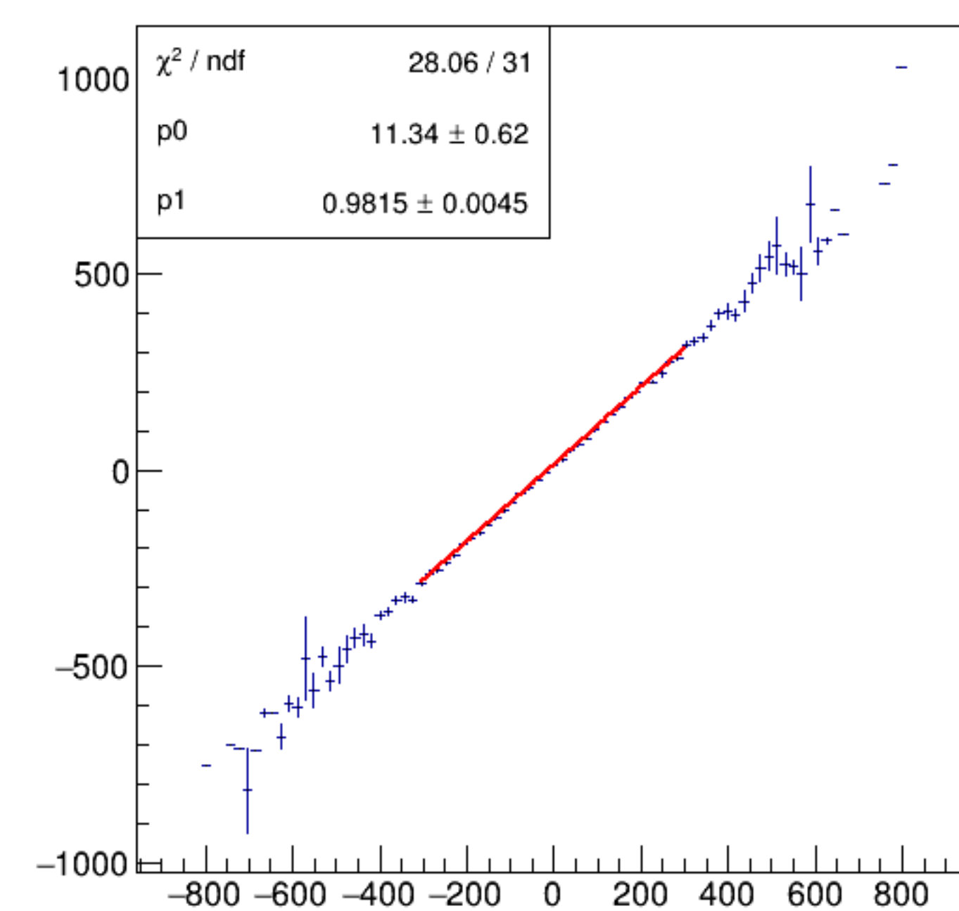
asym_bpm0l01WS/ppm:Aq/ppm {ErrorFlag==0}
