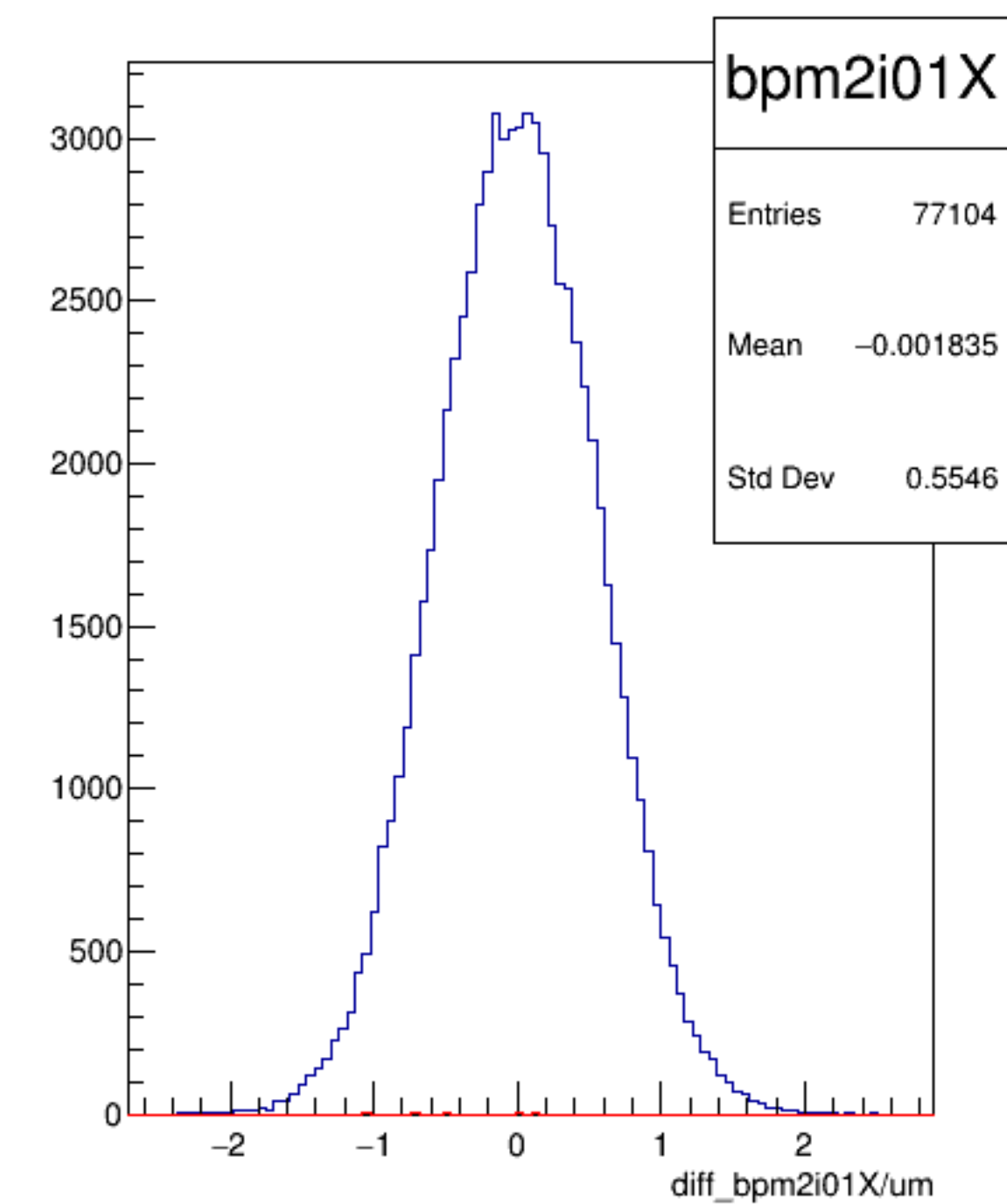
diff_bpm2i01X/um {ErrorFlag==0}
