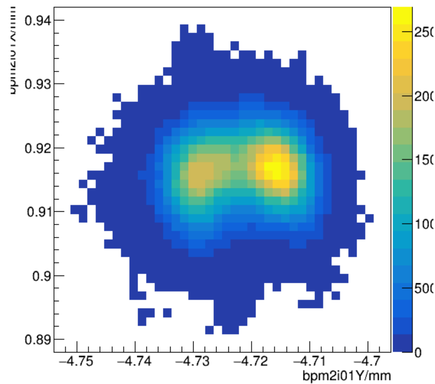
bpm2i01X/mm:bpm2i01Y/mm {ErrorFlag==0}
