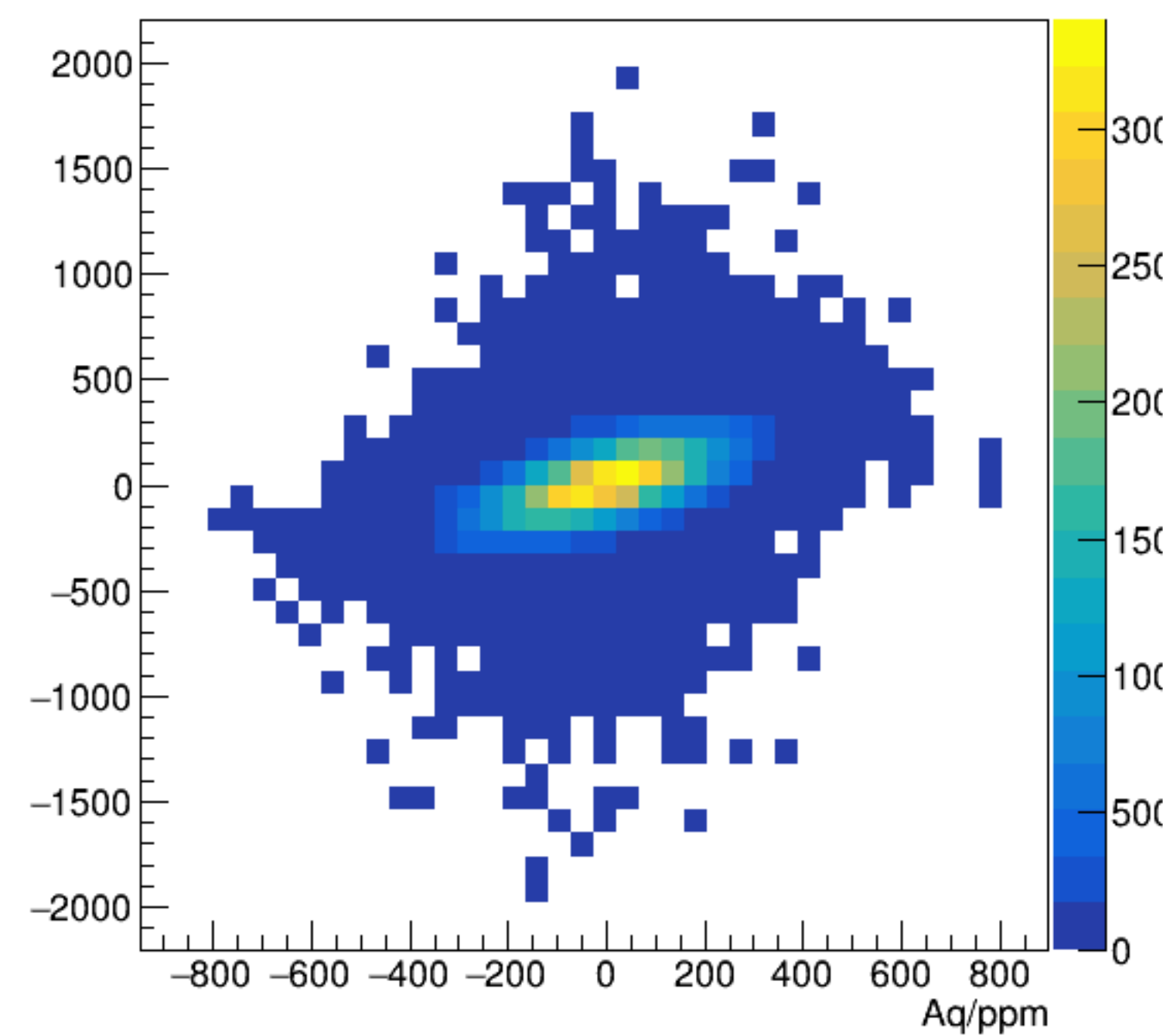
asym_bpm0i02WS/ppm:Aq/ppm {ErrorFlag==0}
