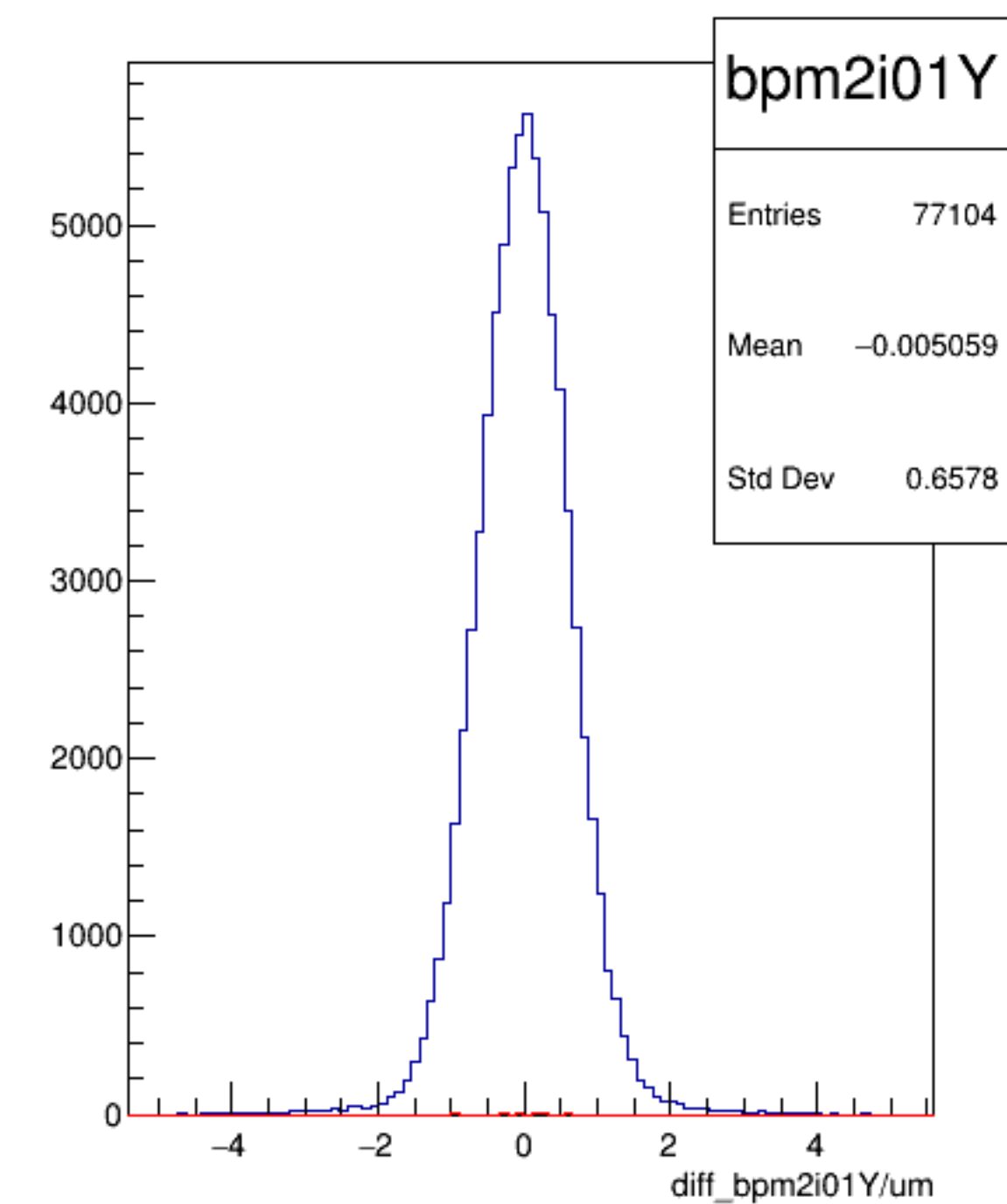
diff_bpm2i01Y/um {ErrorFlag==0}
