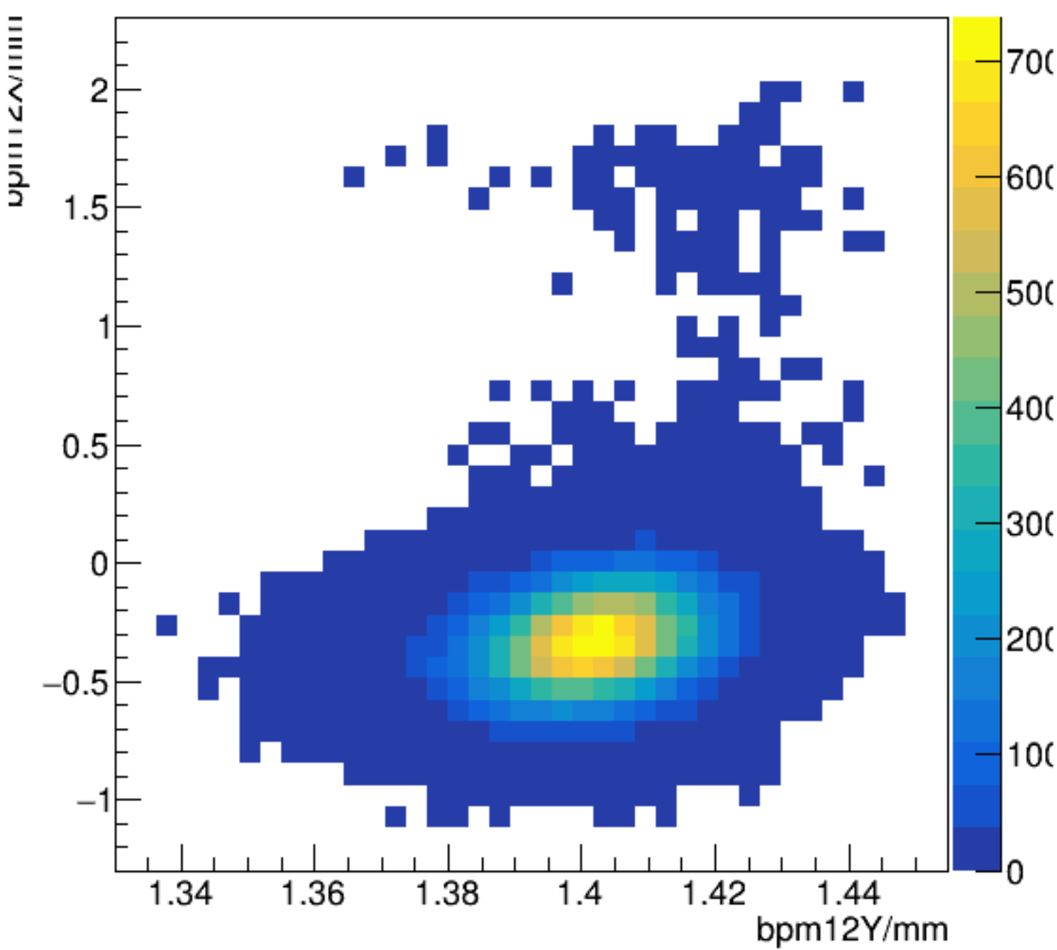
bpm12X/mm:bpm12Y/mm {ErrorFlag==0}
