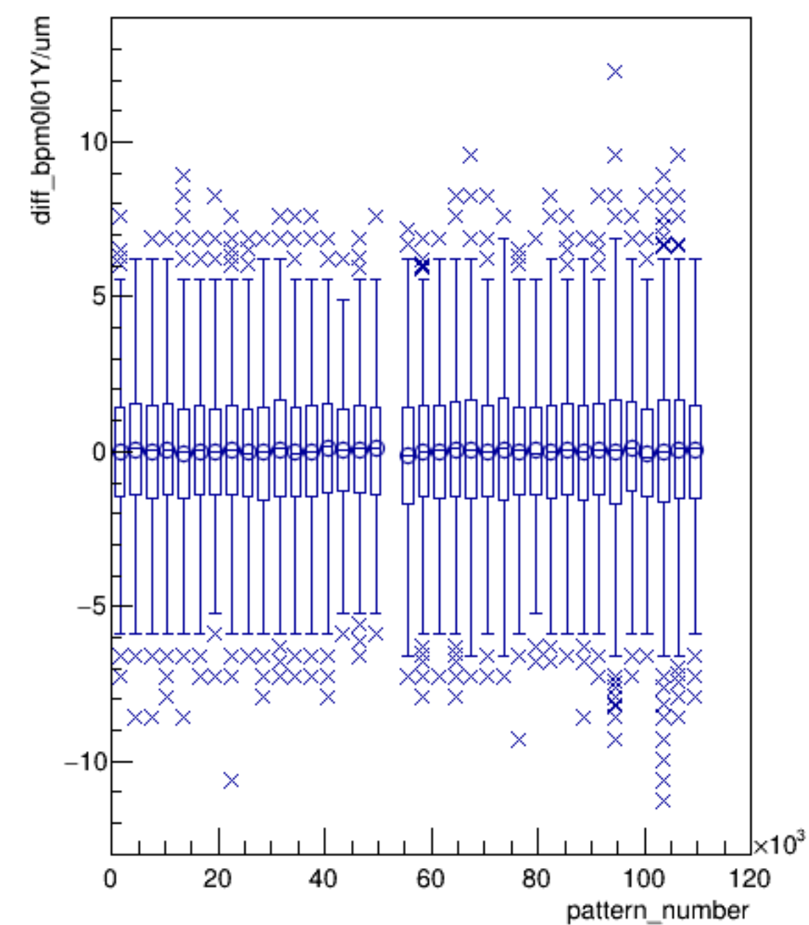
diff_bpm0I01Y/um:pattern_number (ErrorFlag==0)
