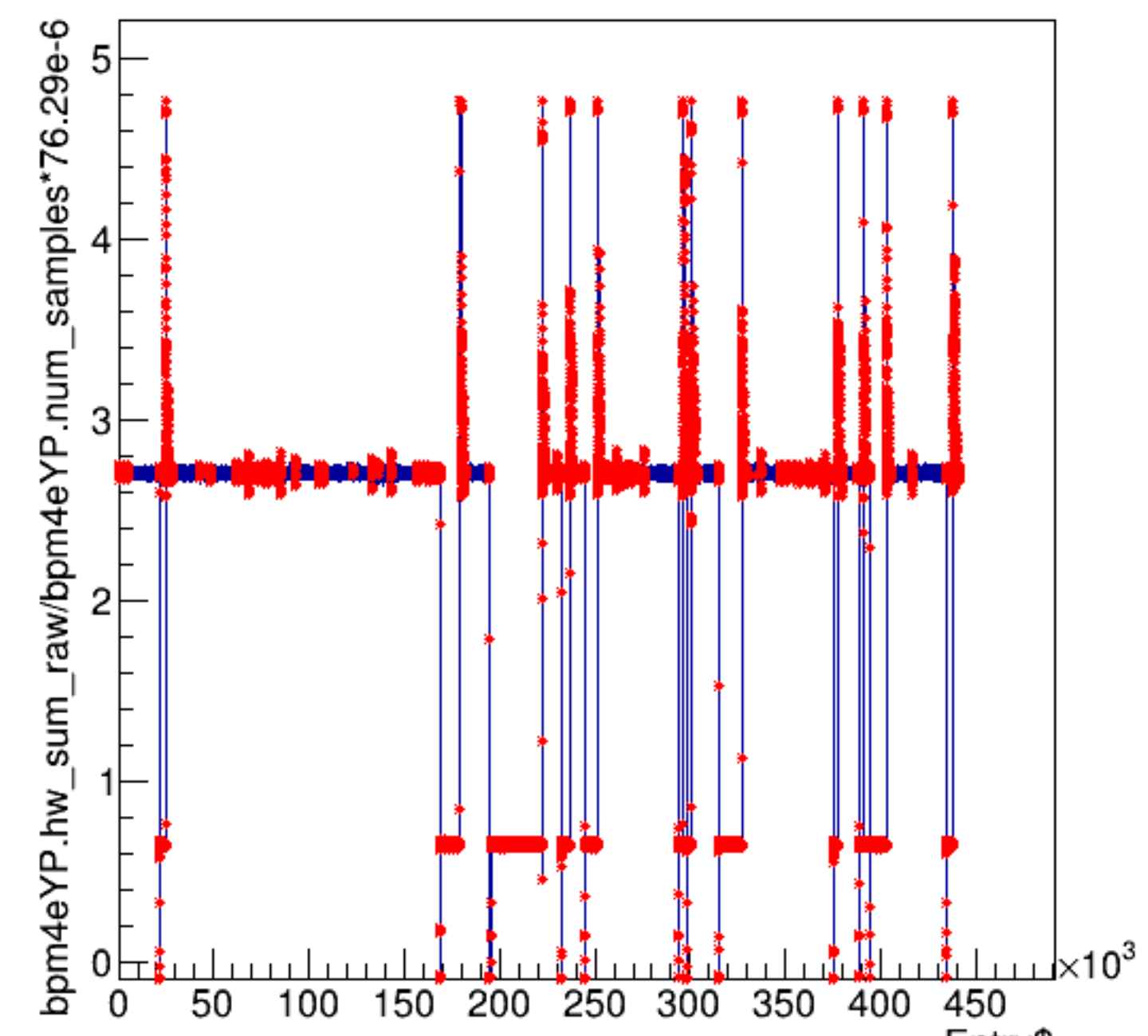
bpm4eYP.hw_sum_raw/bpm4eYP.num_samples*76.29e-6:Entry$
