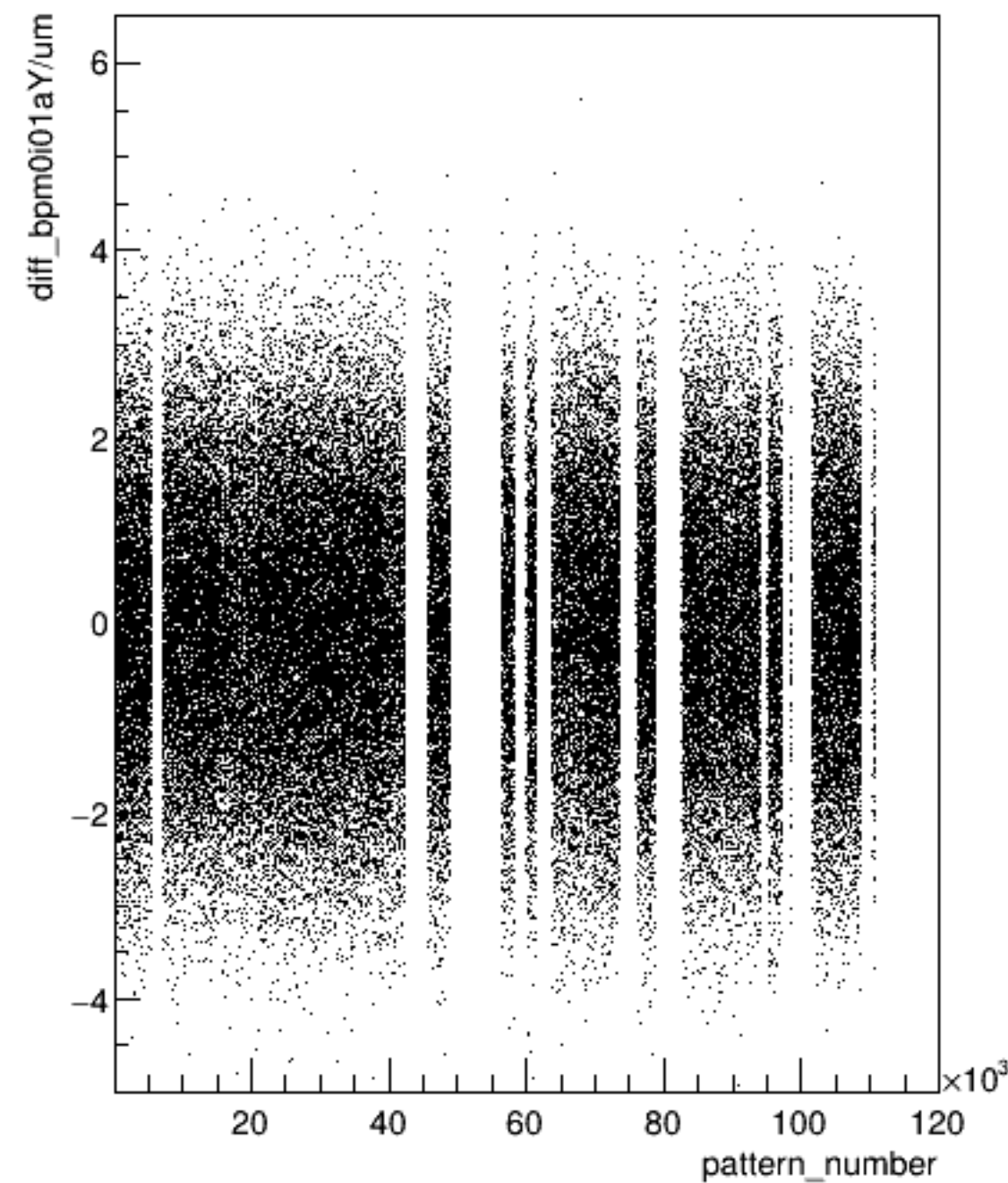
diff_bpm0i01aY/um:pattern_number (ErrorFlag==0)
