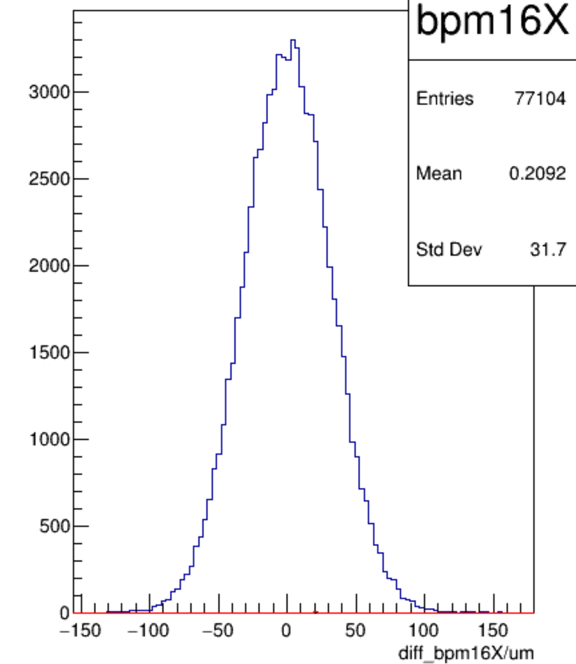
diff_bpm16X/um {ErrorFlag==0}
