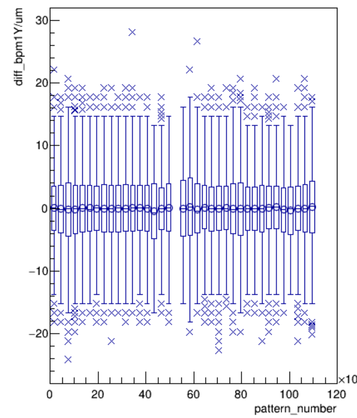
diff_bpm1Y/um:pattern_number {ErrorFlag==0}
